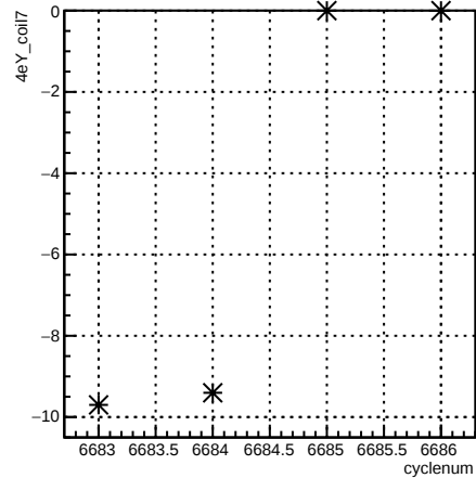
4eY_coil7:cyclenum {run == 6629}
