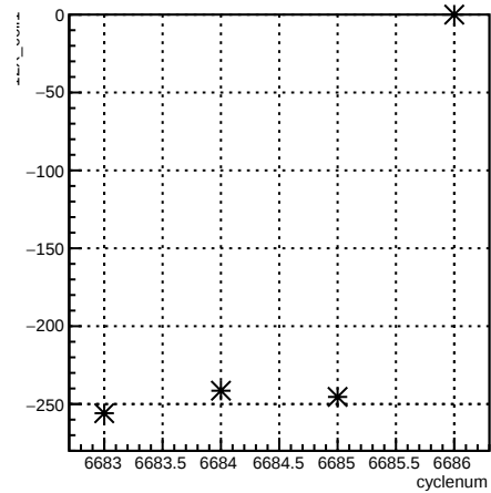
12X_coil1:cyclenum {run == 6629}
