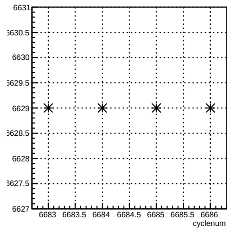
run:cyclenum {run == 6629}
