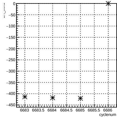
1X_coil1:cyclenum {run == 6629}
