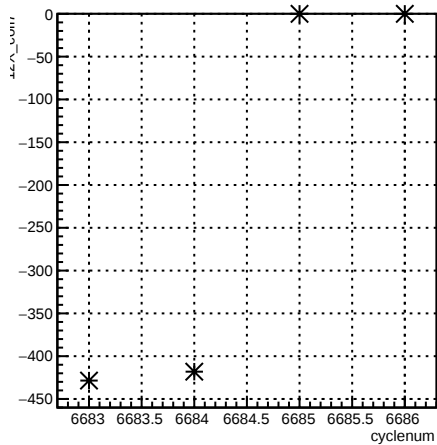
12X_coil7:cyclenum {run == 6629}
