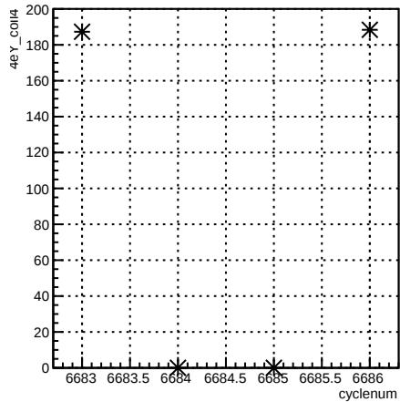
4eY_coil4:cyclenum {run == 6629}
