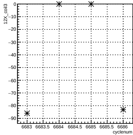
12X_coil3:cyclenum {run == 6629}
