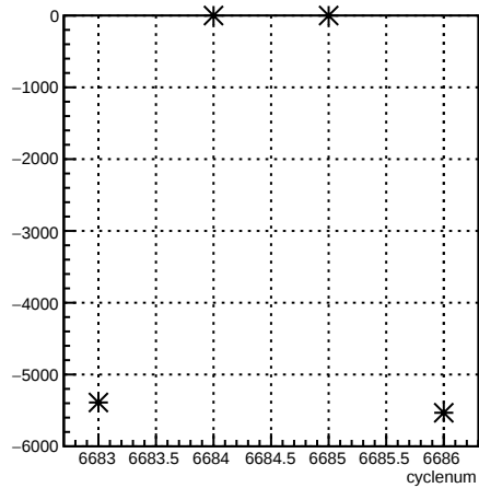
usr_coil3:cyclenum {run == 6629}
