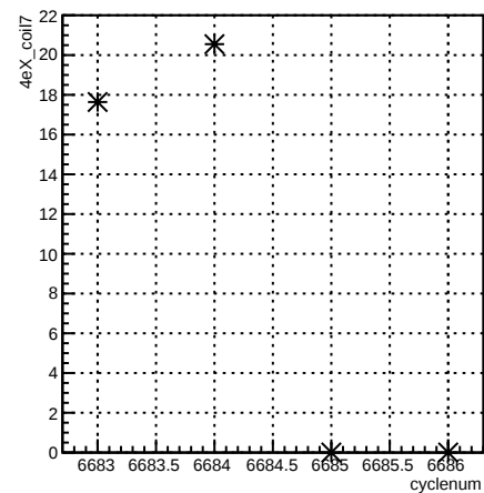
4eX_coil7:cyclenum {run == 6629}
