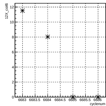
12X_coil6:cyclenum {run == 6629}
