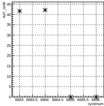
4aY_coil6:cyclenum {run == 6629}
