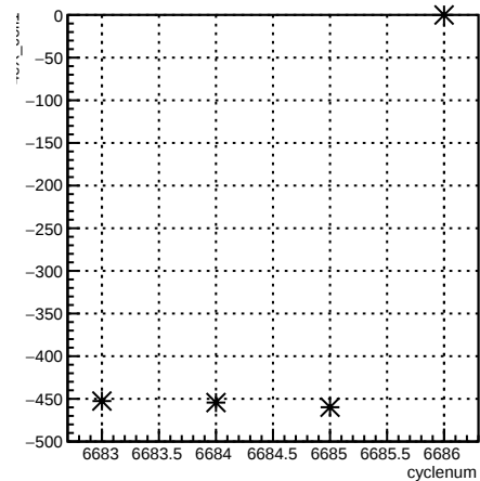
4eX_coil1:cyclenum {run == 6629}
