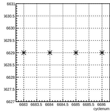
run:cyclenum {run == 6629}
