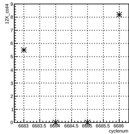
12X_coil4:cyclenum {run == 6629}
