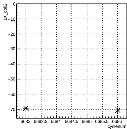
1X_coil3:cyclenum {run == 6629}
