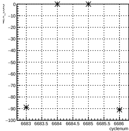
4eX_coil3:cyclenum {run == 6629}
