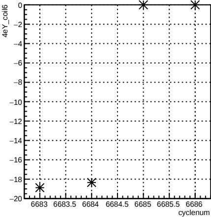
4eY_coil6:cyclenum {run == 6629}
