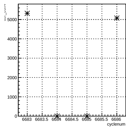
usr_coil4:cyclenum {run == 6629}
