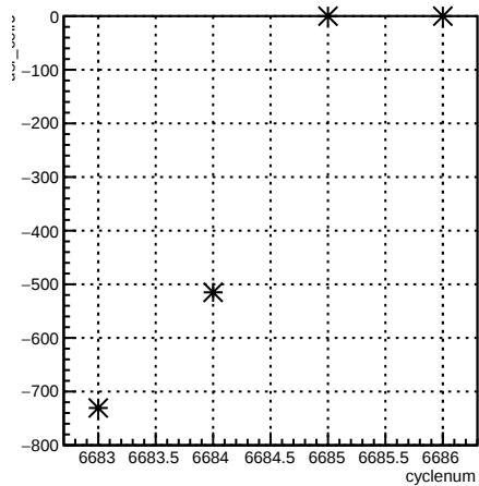
usr_coil6:cyclenum {run == 6629}
