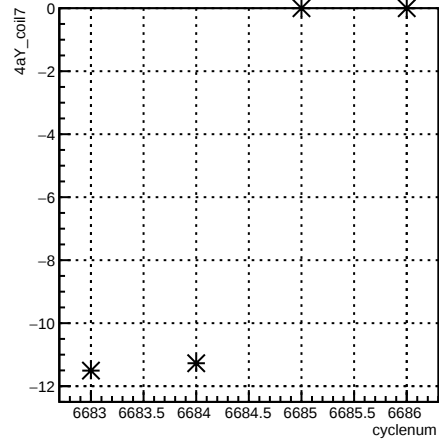
4aY_coil7:cyclenum {run == 6629}
