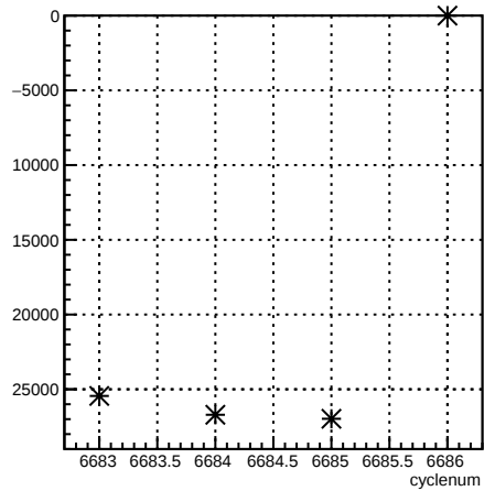
usr_coil1:cyclenum {run == 6629}
