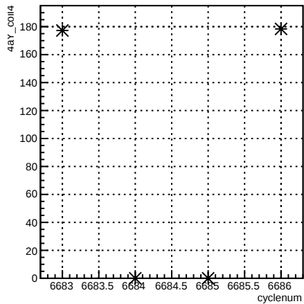
4aY_coil4:cyclenum {run == 6629}
