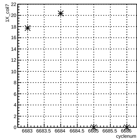
1X_coil7:cyclenum {run == 6629}
