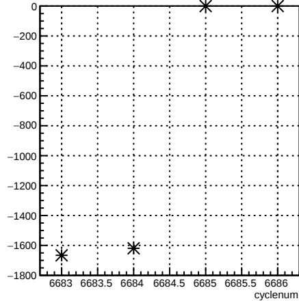
usl_coil6:cyclenum {run == 6629}
