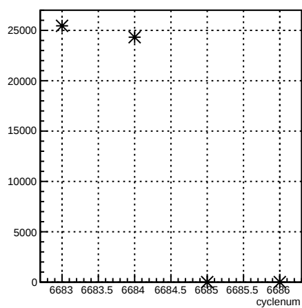
usr_coil7:cyclenum {run == 6629}
