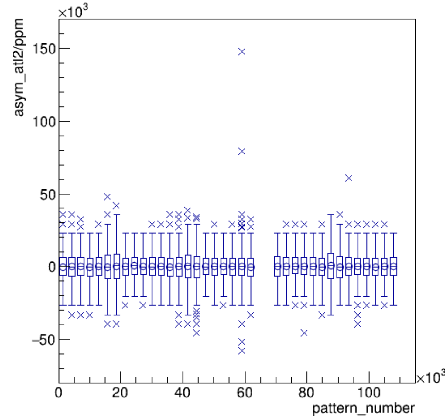
asym_atl2/ppm:pattern_number {ErrorFlag==0}
