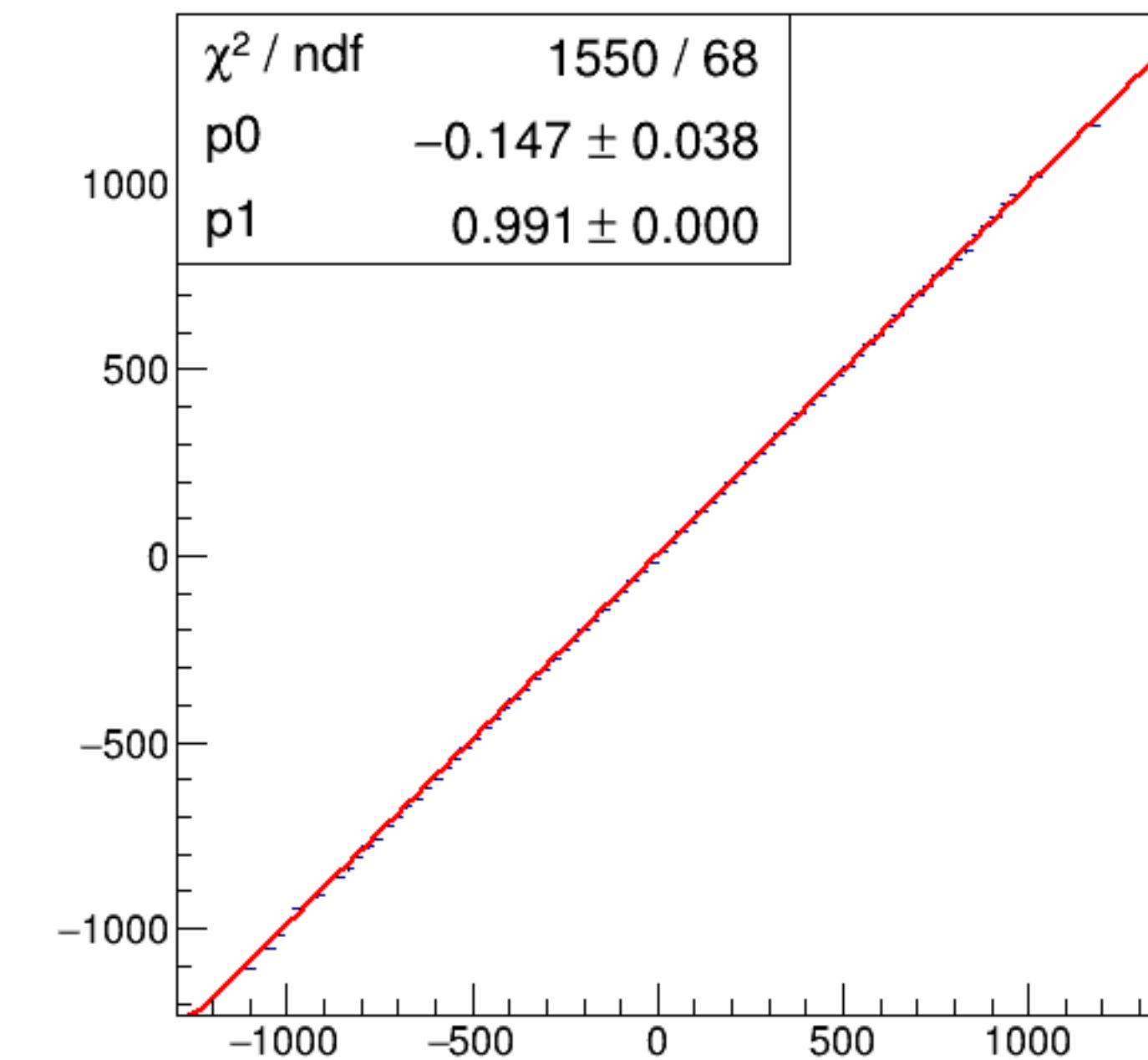
run6629_000_asym_bcm_an_ds_vs_asym_bcm_an_ds3_mul.png
