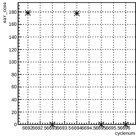
4aY_coil4:cyclenum {run == 6631}
