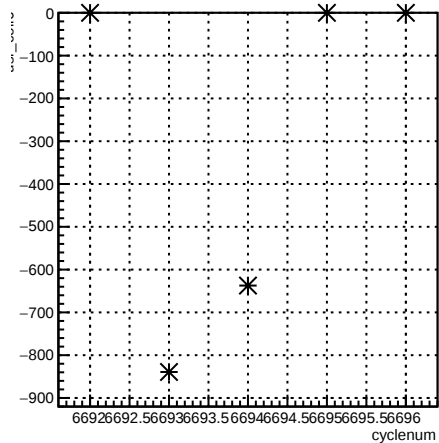
usr_coil6:cyclenum {run == 6631}
