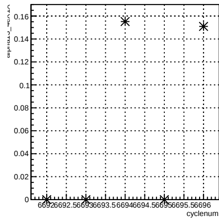
alpha13_4eX1X:cyclenum {run == 6631}
