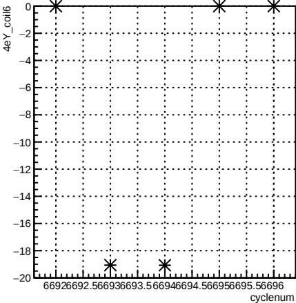
4eY_coil6:cyclenum {run == 6631}
