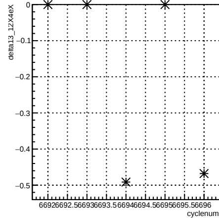
delta13_12X4eX:cyclenum {run == 6631}
