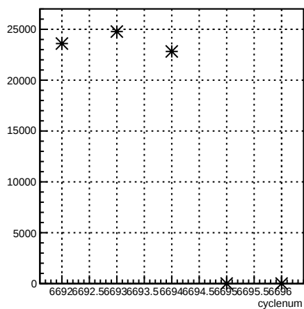
usr_coil7:cyclenum {run == 6631}
