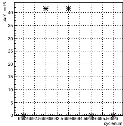
4aY_coil6:cyclenum {run == 6631}
