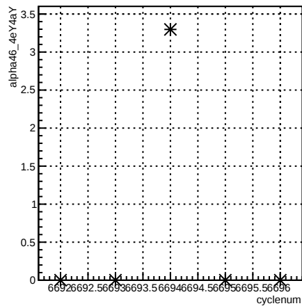
alpha46_4eY4aY:cyclenum {run == 6631}
