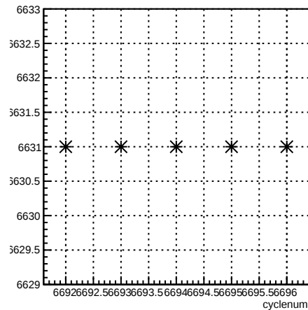
run:cyclenum {run == 6631}
