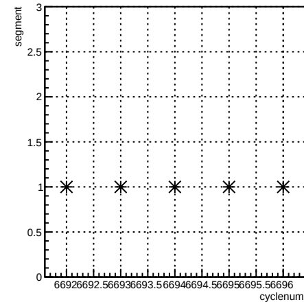
segment:cyclenum {run == 6631}
