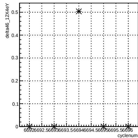
delta46_12X4eY:cyclenum {run == 6631}
