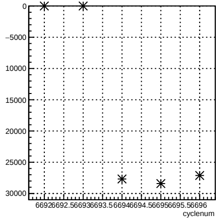
usr_coil1:cyclenum {run == 6631}
