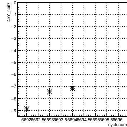
4eY_coil7:cyclenum {run == 6631}
