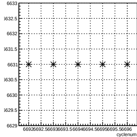
run:cyclenum {run == 6631}
