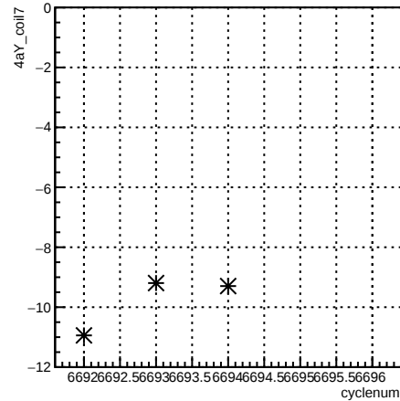
4aY_coil7:cyclenum {run == 6631}
