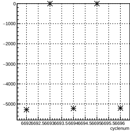
usr_coil3:cyclenum {run == 6631}
