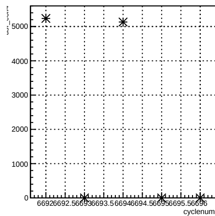
usr_coil4:cyclenum {run == 6631}
