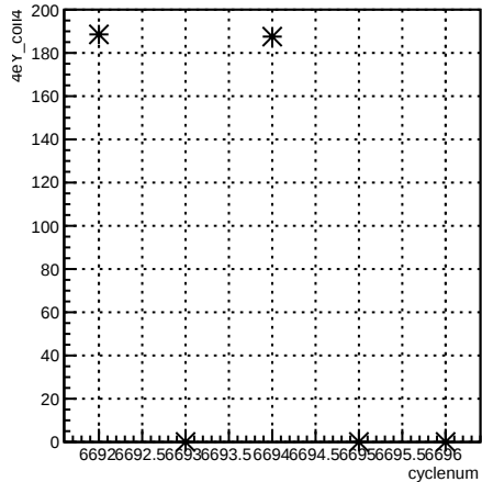
4eY_coil4:cyclenum {run == 6631}
