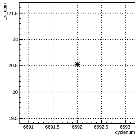
4eX_coil7:cyclenum {run == 6631}
