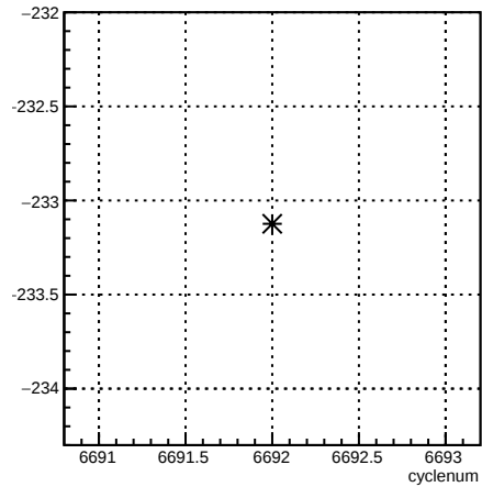
12X_coil1:cyclenum {run == 6631}
