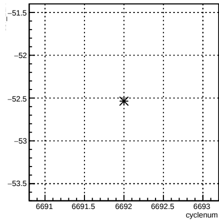
usr_12X:cyclenum {run == 6631}
