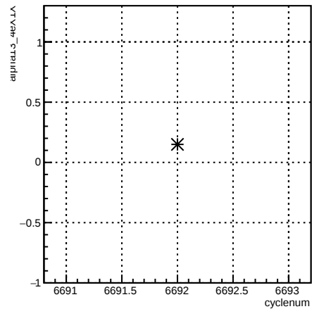
alpha13_4eX1X:cyclenum {run == 6631}
