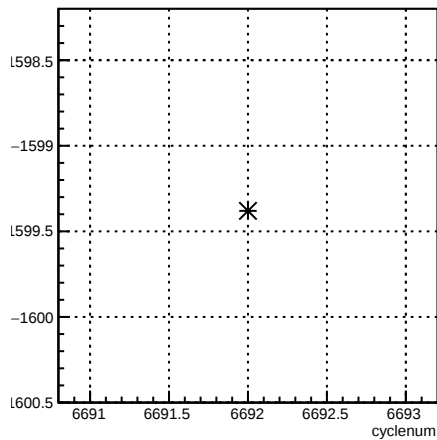
usl_coil6:cyclenum {run == 6631}
