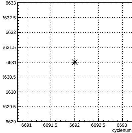
run:cyclenum {run == 6631}
