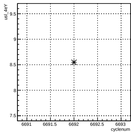
usl_4eY:cyclenum {run == 6631}
