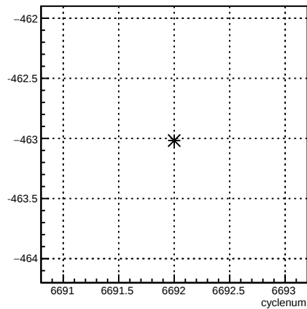
4eX_coil1:cyclenum {run == 6631}
