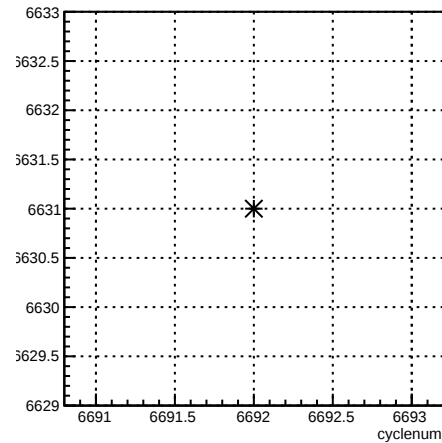
run:cyclenum {run == 6631}
