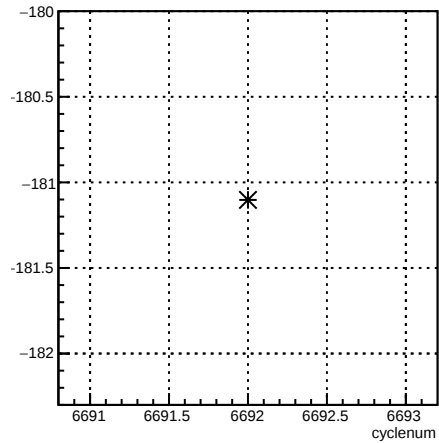
usl_1X:cyclenum {run == 6631}
