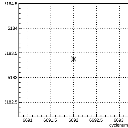
usr_coil4:cyclenum {run == 6631}
