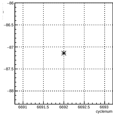
12X_coil3:cyclenum {run == 6631}
