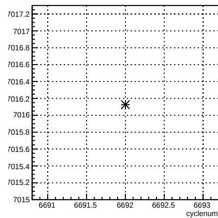
usl_coil4:cyclenum {run == 6631}
