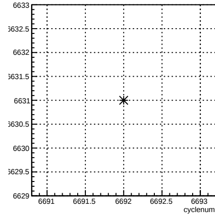
run:cyclenum {run == 6631}
