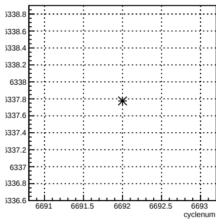
usl_coil3:cyclenum {run == 6631}
