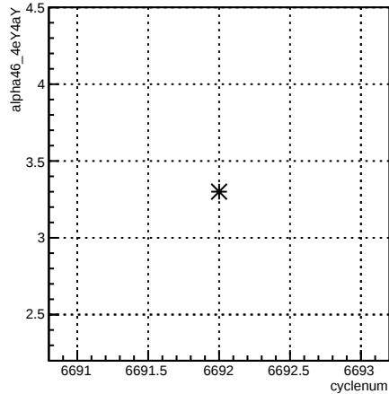
alpha46_4eY4aY:cyclenum {run == 6631}
