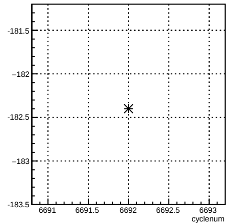
usr_4eY:cyclenum {run == 6631}
