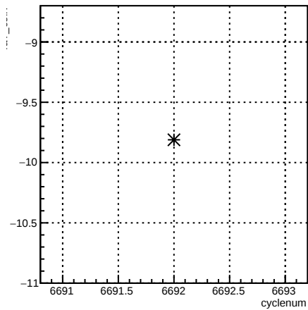
4eY_coil7:cyclenum {run == 6631}
