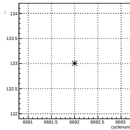
usl_4eX:cyclenum {run == 6631}
