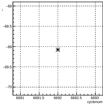
4eX_coil3:cyclenum {run == 6631}
