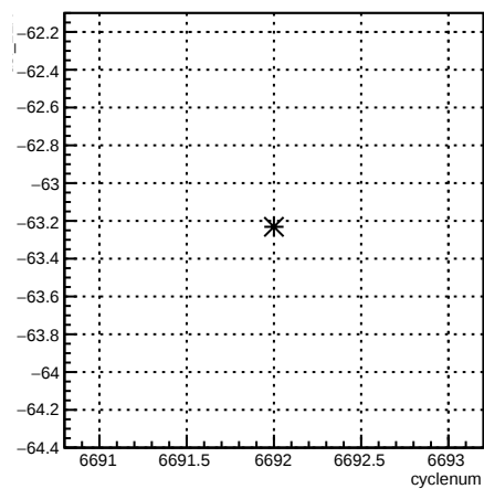
usl_12X:cyclenum {run == 6631}
