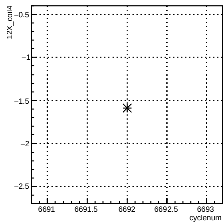
12X_coil4:cyclenum {run == 6631}
