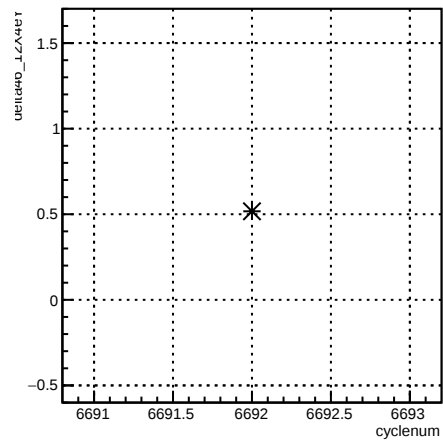
delta46_12X4eY:cyclenum {run == 6631}
