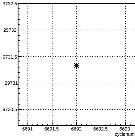
usl_coil1:cyclenum {run == 6631}
