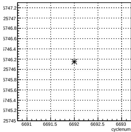
usl_coil7:cyclenum {run == 6631}
