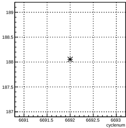
4eY_coil4:cyclenum {run == 6631}
