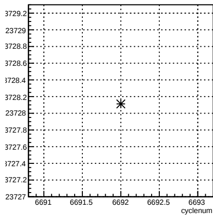
usr_coil7:cyclenum {run == 6631}
