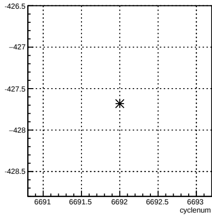
12X_coil7:cyclenum {run == 6631}
