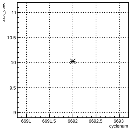
12X_coil6:cyclenum {run == 6631}
