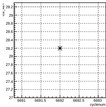
usl_4aY:cyclenum {run == 6631}
