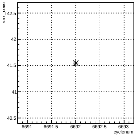
4eY_coil6:cyclenum {run == 6631}
