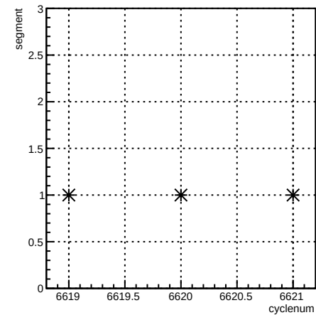
segment:cyclenum {run == 6613}
