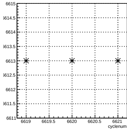
run:cyclenum {run == 6613}
