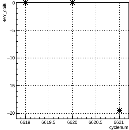
4eY_coil6:cyclenum {run == 6613}
