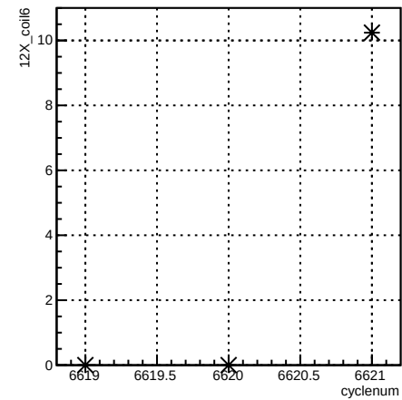
12X_coil6:cyclenum {run == 6613}
