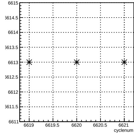
run:cyclenum {run == 6613}
