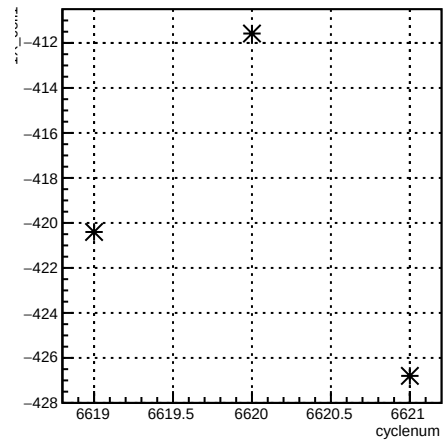
4eX_coil1:cyclenum {run == 6613}
