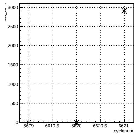
usl_coil4:cyclenum {run == 6613}
