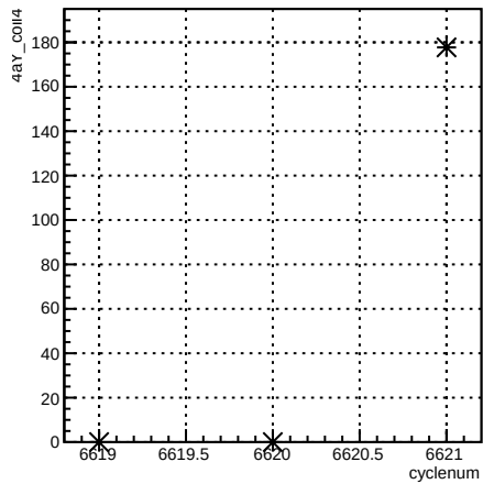
4eY_coil4:cyclenum {run == 6613}
