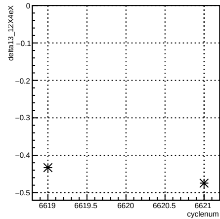
delta13_12X4eX:cyclenum {run == 6613}
