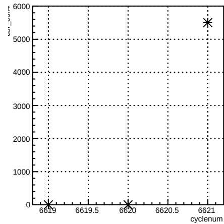
usr_coil4:cyclenum {run == 6613}
