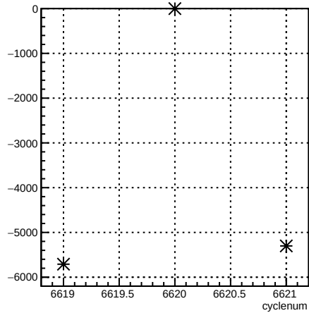
usr_coil3:cyclenum {run == 6613}
