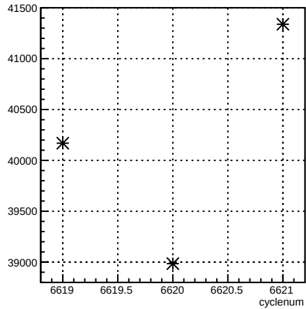
usl_coil1:cyclenum {run == 6613}
