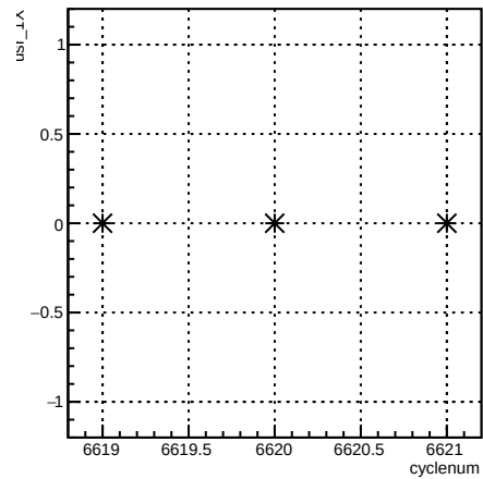
usr_4eY:cyclenum {run == 6613}
