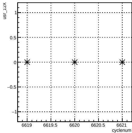
usr_12X:cyclenum {run == 6613}
