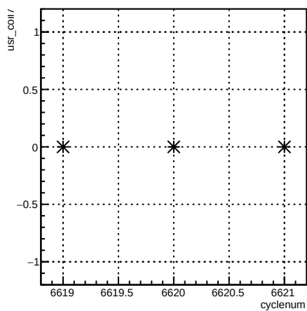
usr_coil7:cyclenum {run == 6613}
