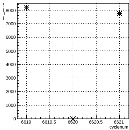
usl_coil3:cyclenum {run == 6613}
