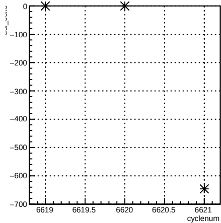
usl_coil6:cyclenum {run == 6613}
