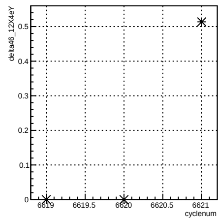
delta46_12X4eY:cyclenum {run == 6613}
