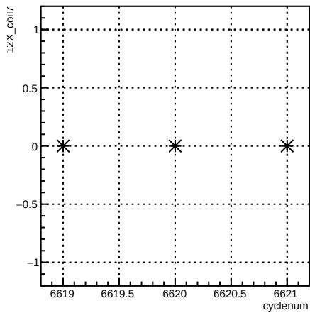
12X_coil7:cyclenum {run == 6613}
