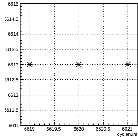
run:cyclenum {run == 6613}
