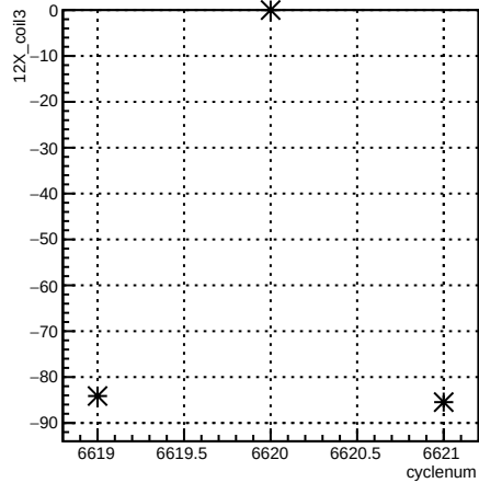
12X_coil3:cyclenum {run == 6613}
