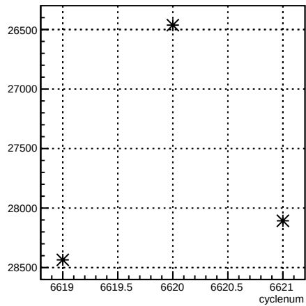
usr_coil6:cyclenum {run == 6613}
