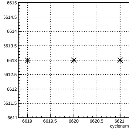
run:cyclenum {run == 6613}
