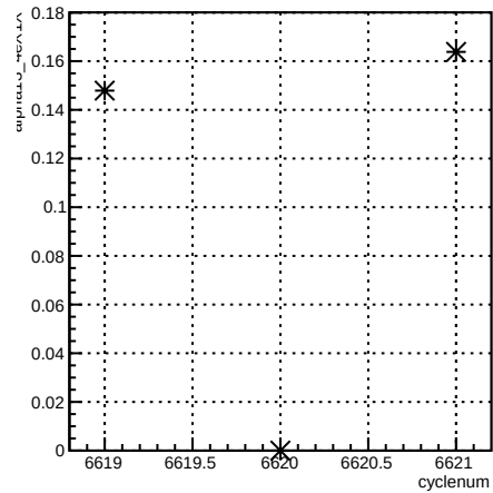
alpha13_4eX1X:cyclenum {run == 6613}
