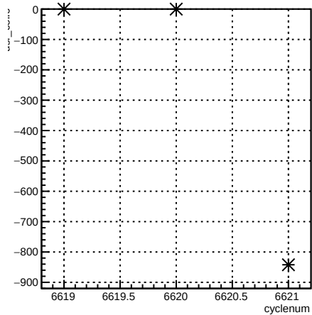
usr_coil6:cyclenum {run == 6613}
