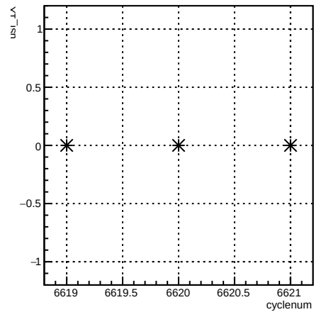
usl_4eY:cyclenum {run == 6613}
