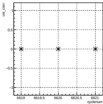
usl_coil7:cyclenum {run == 6613}
