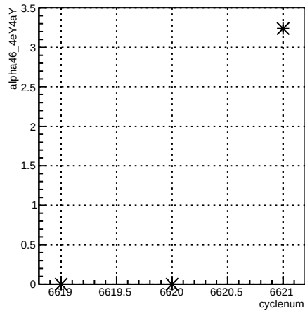
alpha46_4eY4aY:cyclenum {run == 6613}
