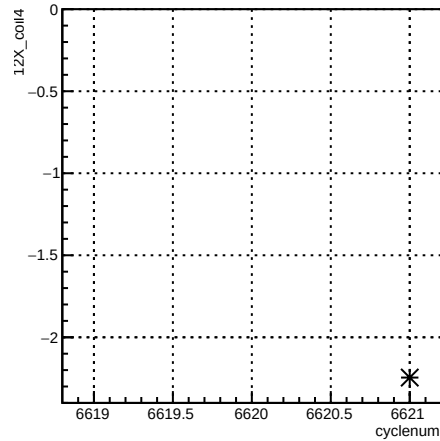
12X_coil4:cyclenum {run == 6613}
