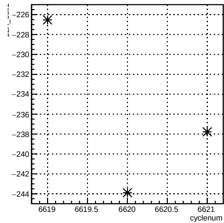
12X_coil1:cyclenum {run == 6613}
