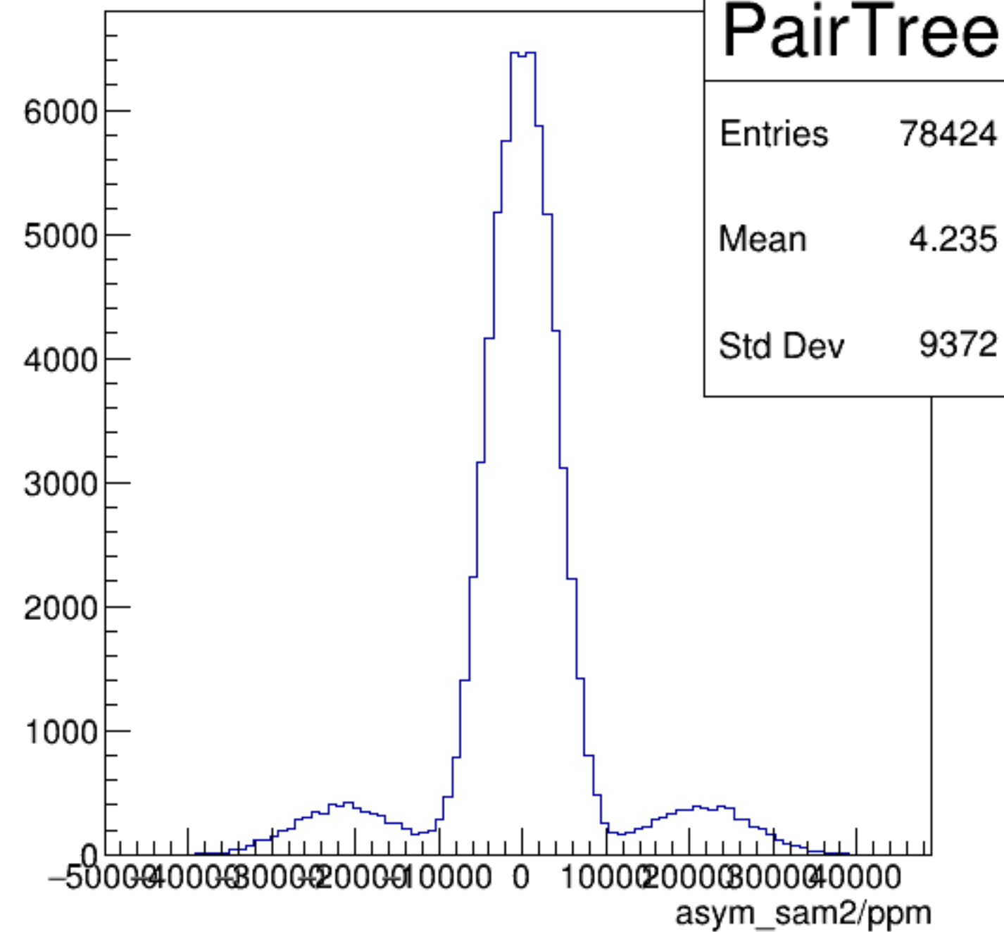
asym_sam2/ppm {ErrorFlag==0}
