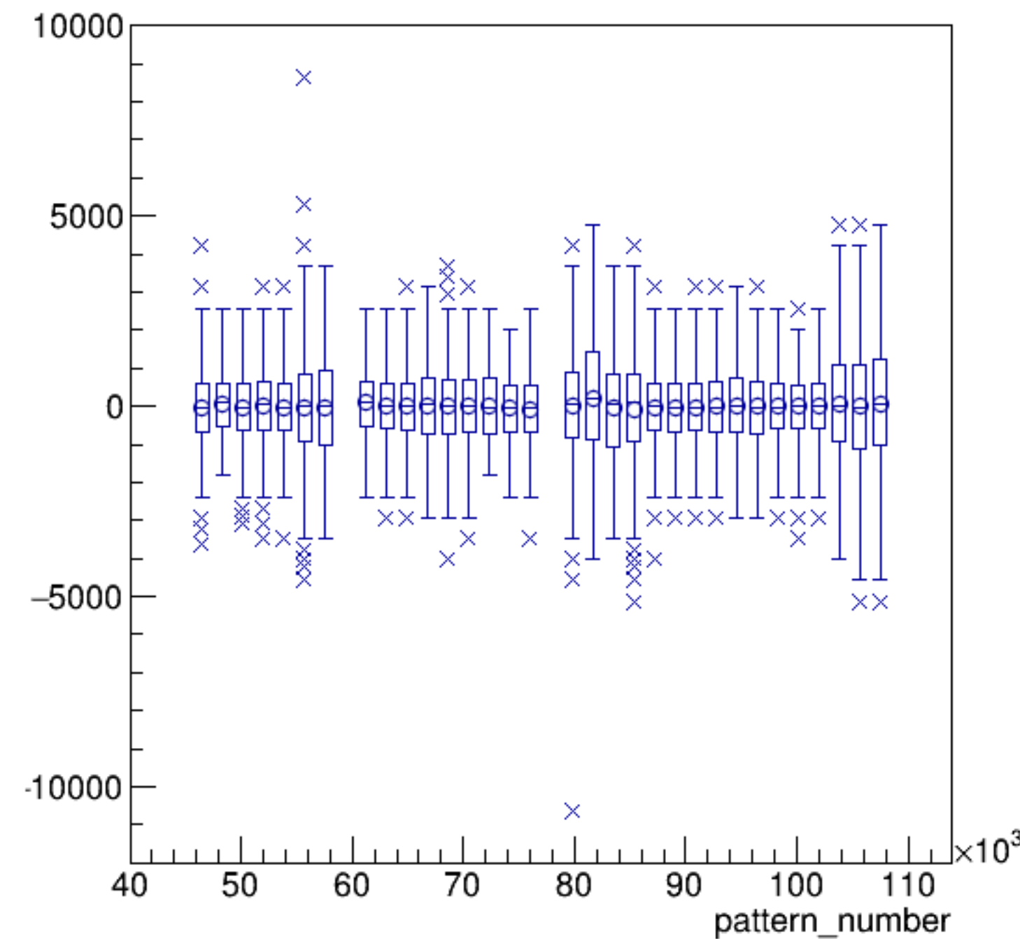
asym_sam3/ppm:pattern_number {ErrorFlag==0}
