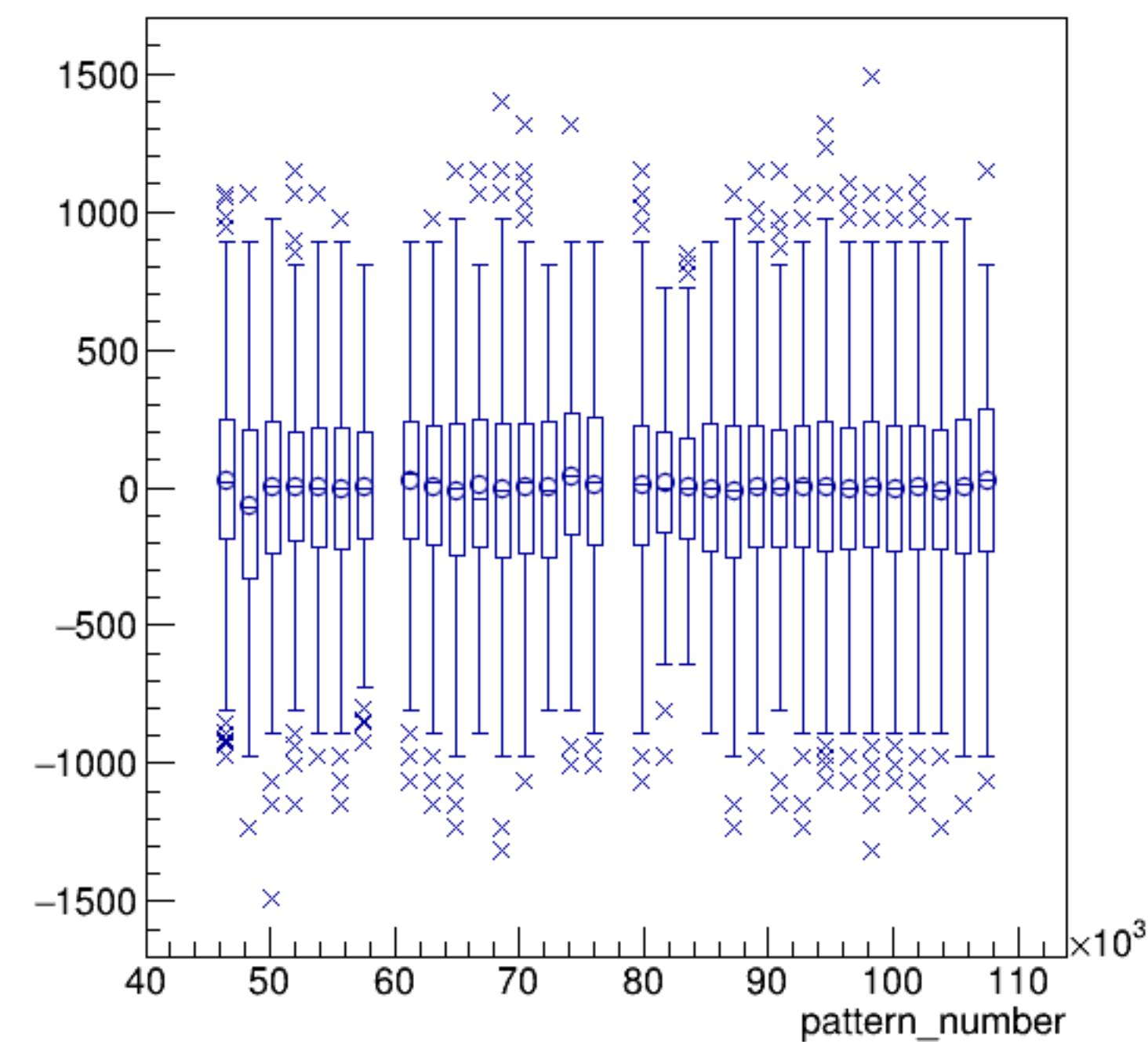
asym_sam1/ppm:pattern_number {ErrorFlag==0}
