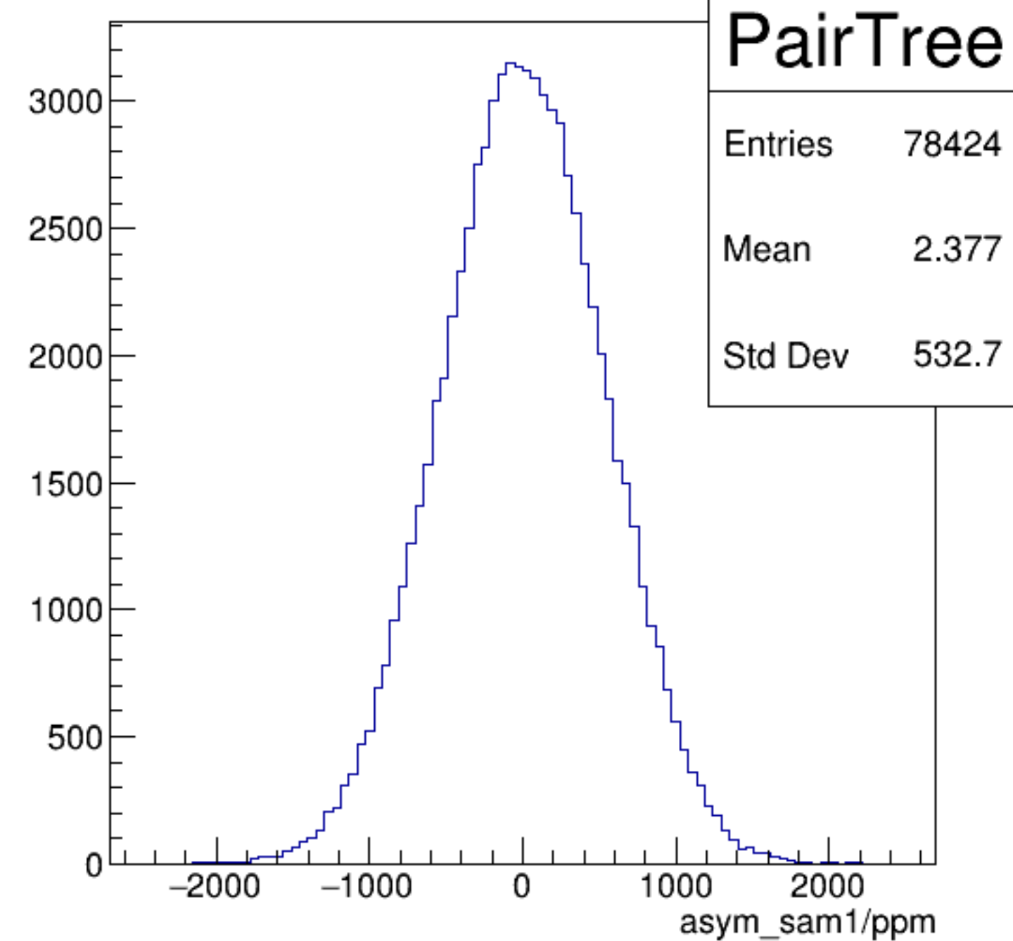
asym_sam1/ppm {ErrorFlag==0}
