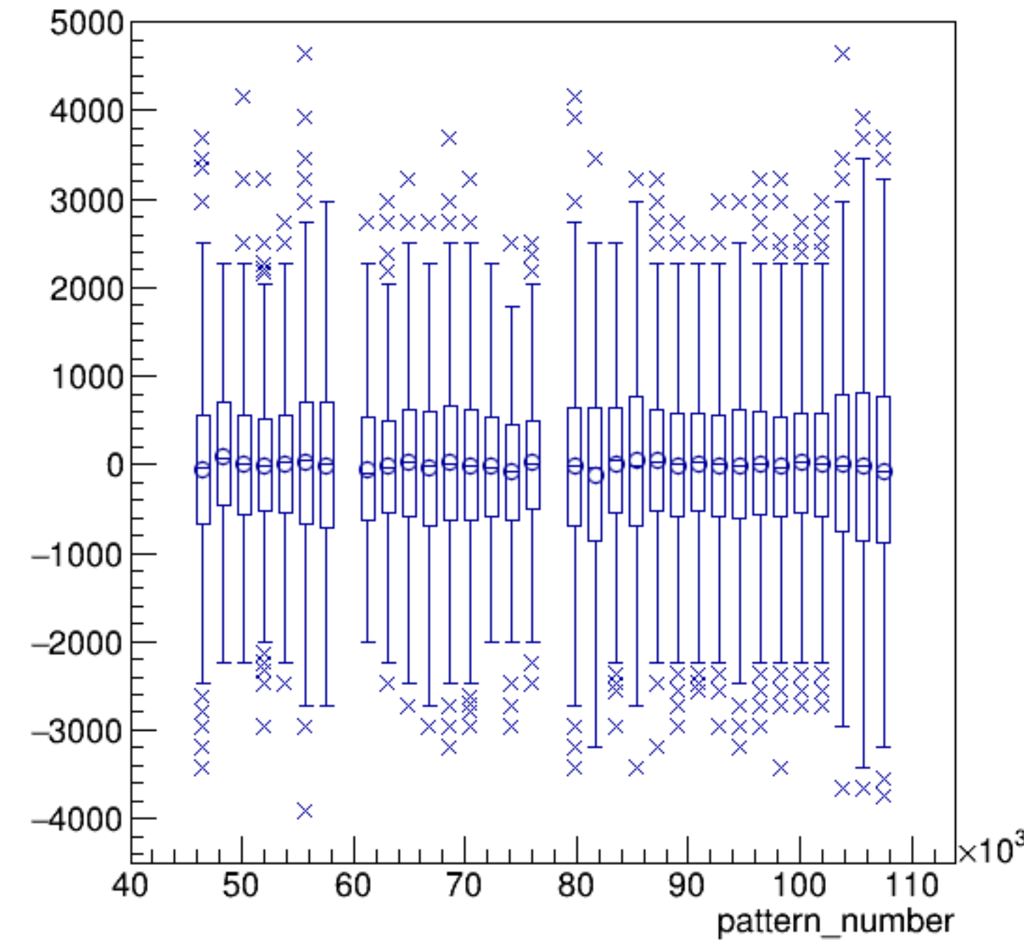
asym_sam6/ppm:pattern_number {ErrorFlag==0}
