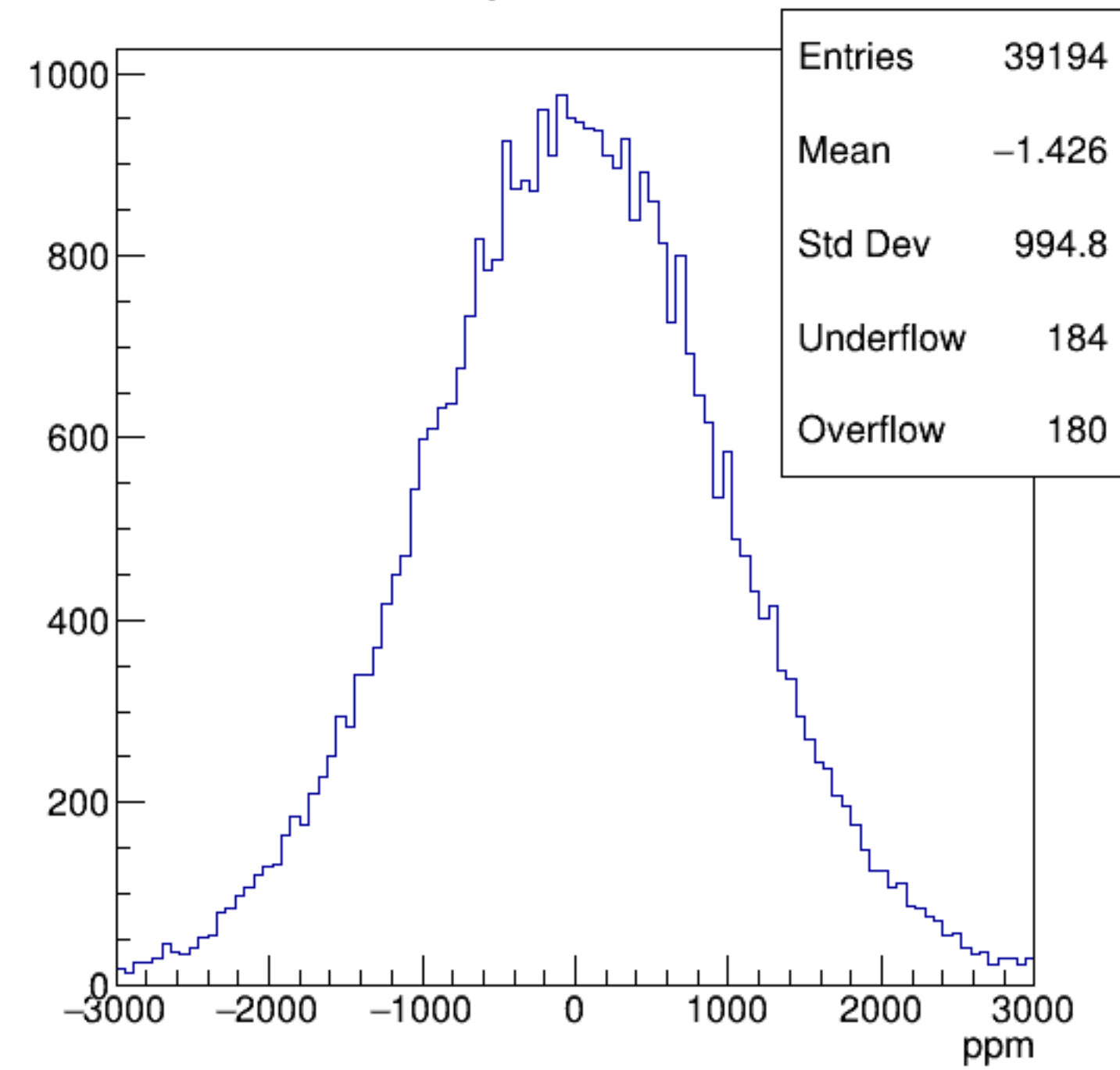
asym_sam3
