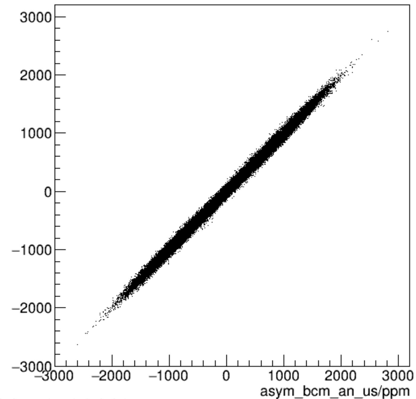
run6614_000_asym_bcm_dg_ds_vs_asym_bcm_an_us_pr.png
