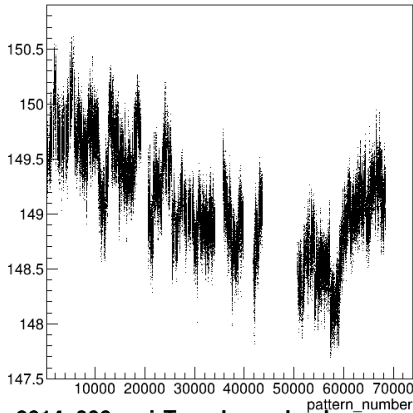
yield_bcm_dg_ds:pattern_number {ErrorFlag==0}
