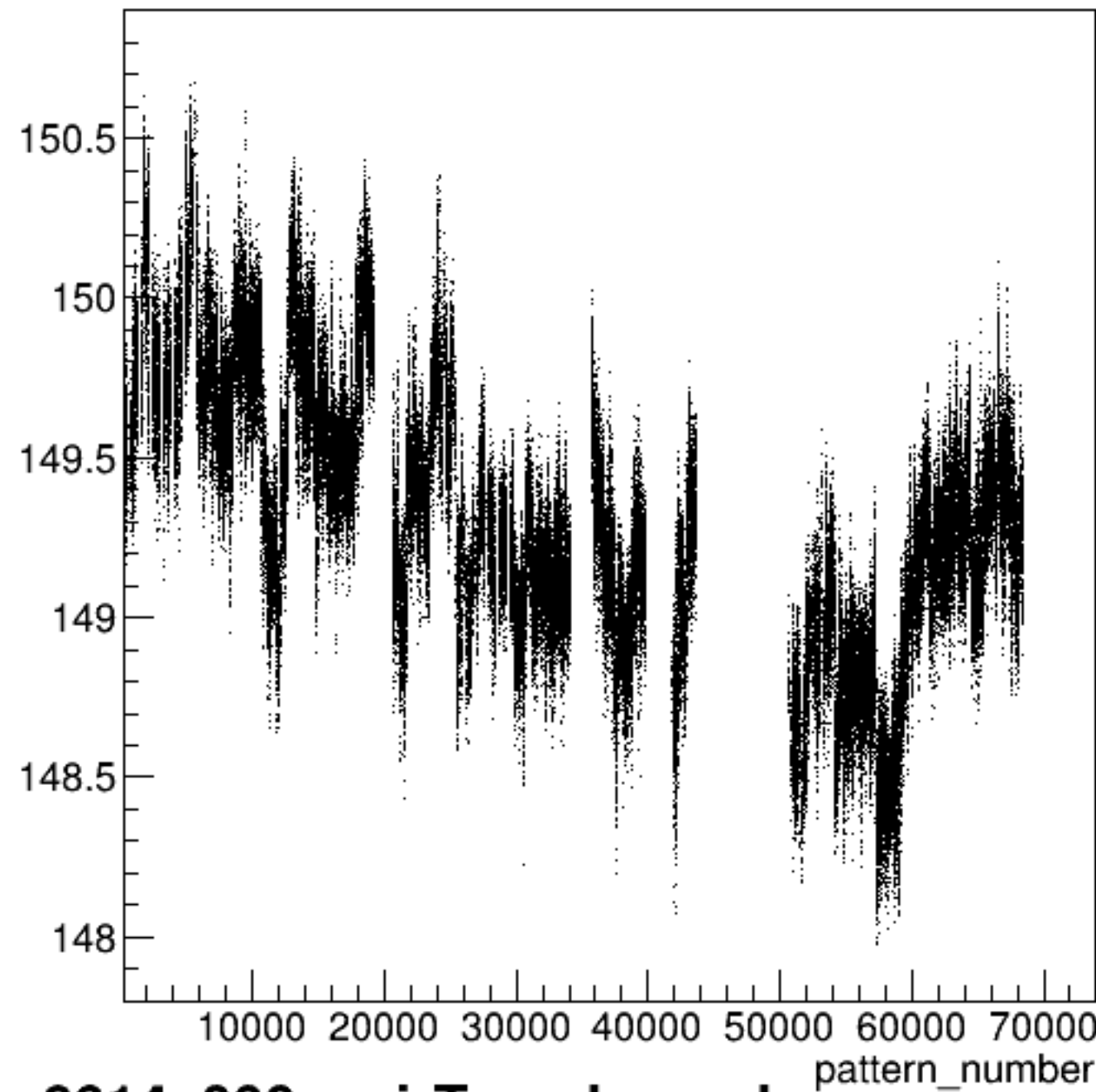
yield_bcm_dg_us:pattern_number {ErrorFlag==0}
