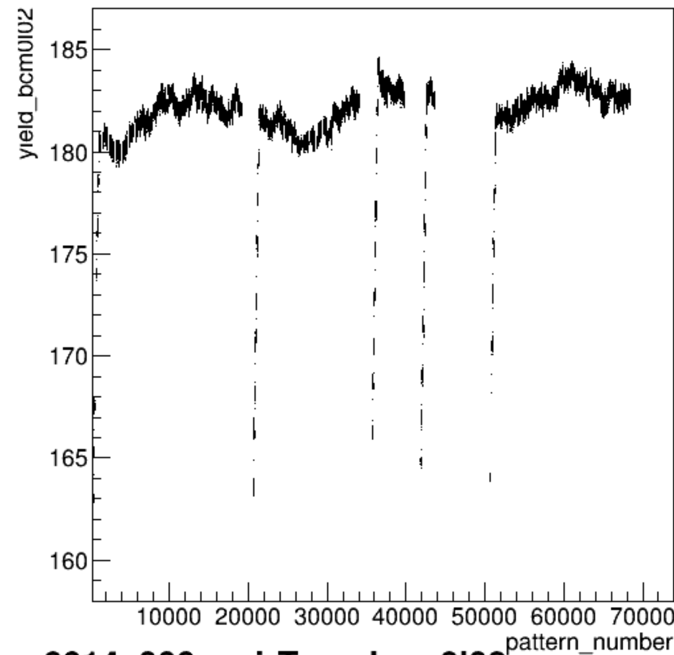
yield_bcm0l02:pattern_number {ErrorFlag==0}
