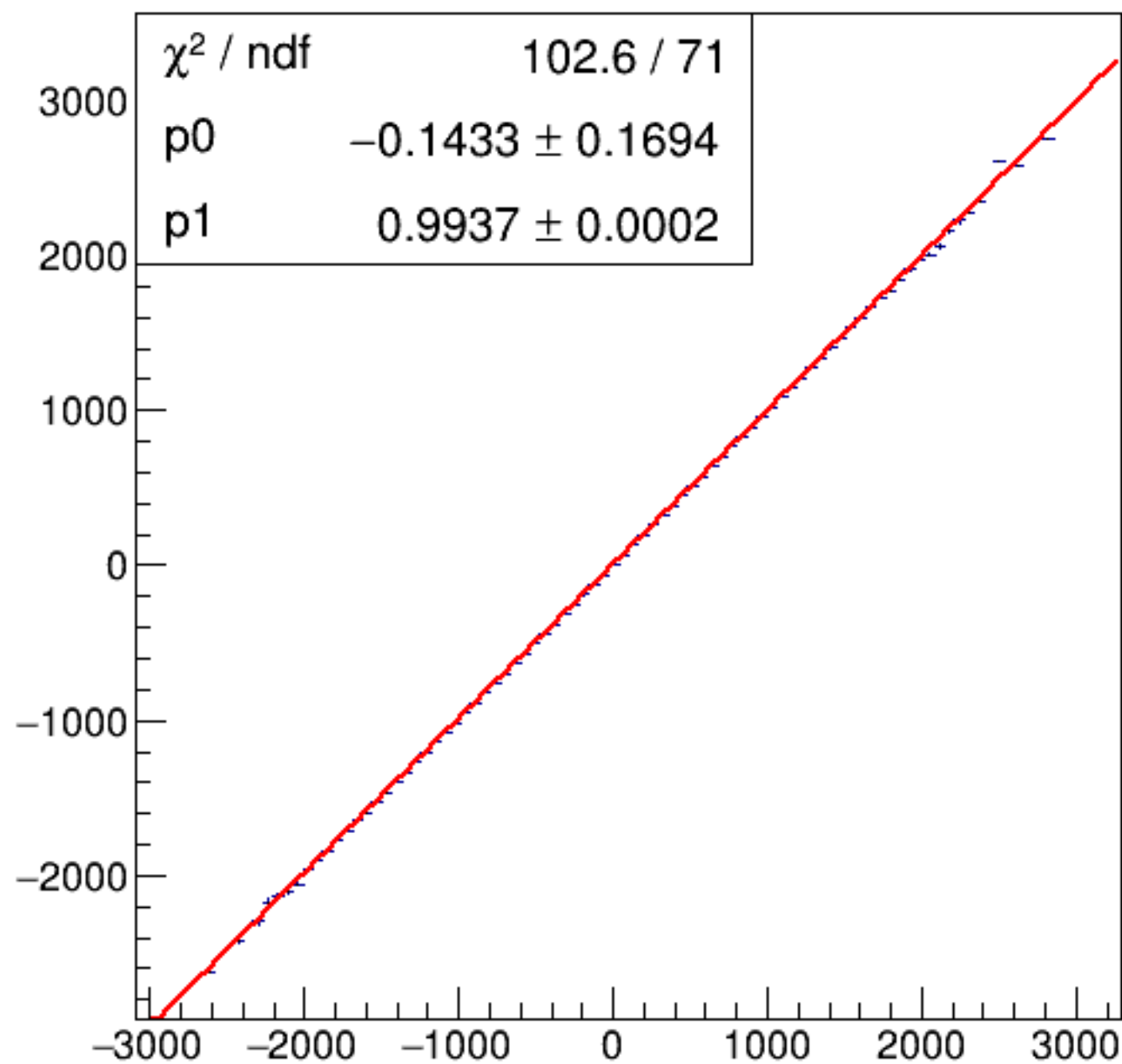
run6614_000_asym_bcm_dg_ds_vs_asym_bcm_an_us_pr.png
