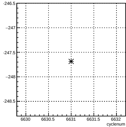
12X_coil1:cyclenum {run == 6616}
