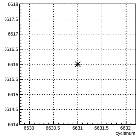
run:cyclenum {run == 6616}
