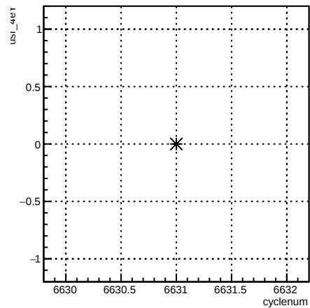
usr_4eY:cyclenum {run == 6616}
