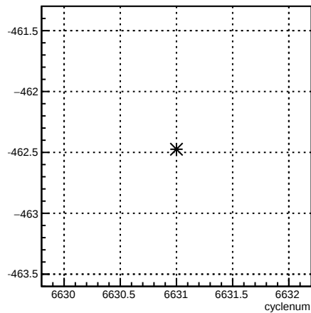
4eX_coil1:cyclenum {run == 6616}
