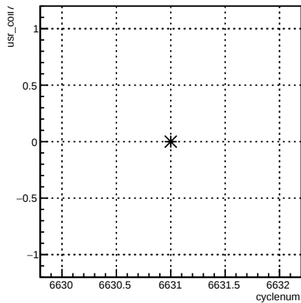
usr_coil7:cyclenum {run == 6616}
