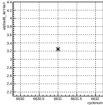
alpha46_4eY4aY:cyclenum {run == 6616}
