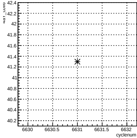
4eY_coil6:cyclenum {run == 6616}
