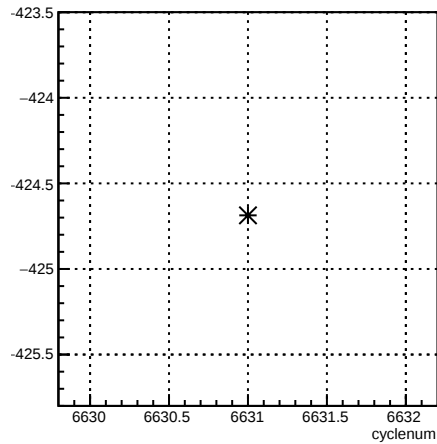
1X_coil1:cyclenum {run == 6616}
