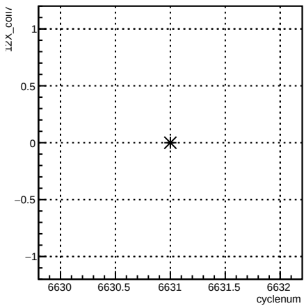
12X_coil7:cyclenum {run == 6616}
