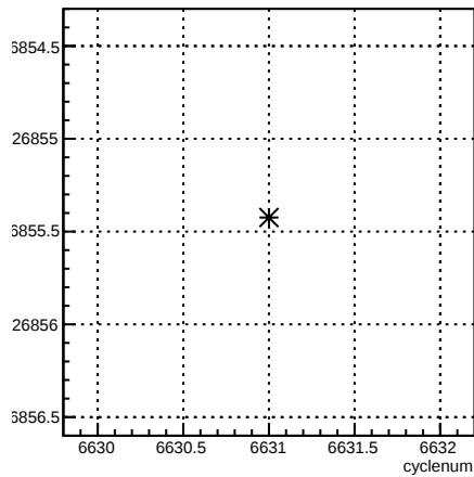
usr_coil6:cyclenum {run == 6616}
