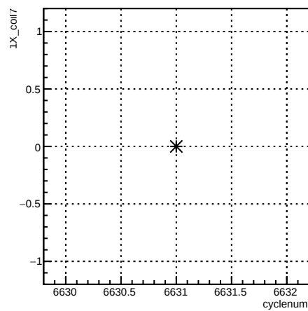
1X_coil7:cyclenum {run == 6616}
