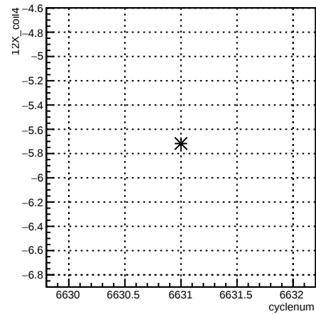
12X_coil4:cyclenum {run == 6616}
