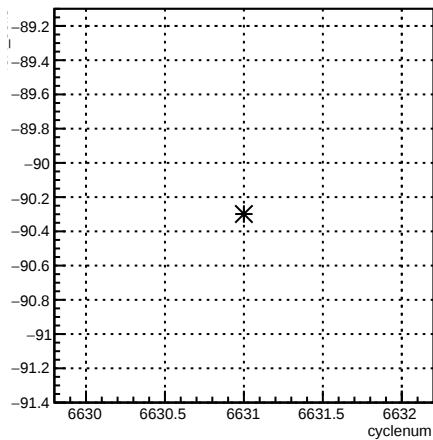
4eX_coil3:cyclenum {run == 6616}
