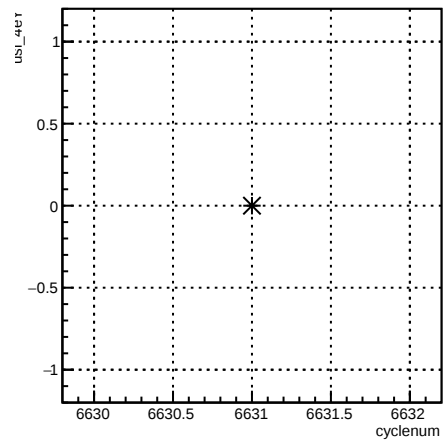
usl_4eY:cyclenum {run == 6616}
