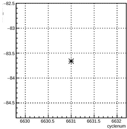
12X_coil3:cyclenum {run == 6616}
