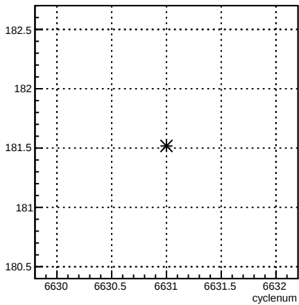
4eY_coil4:cyclenum {run == 6616}
