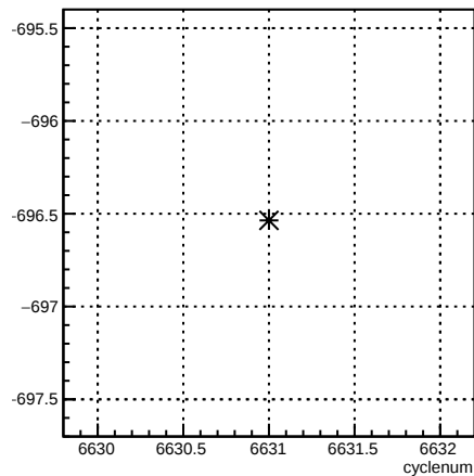
usl_coil6:cyclenum {run == 6616}
