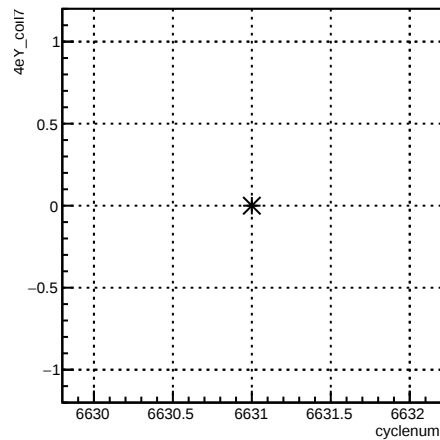
4eY_coil7:cyclenum {run == 6616}
