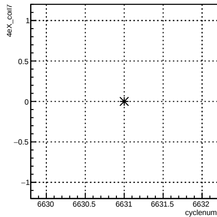
4eX_coil7:cyclenum {run == 6616}
