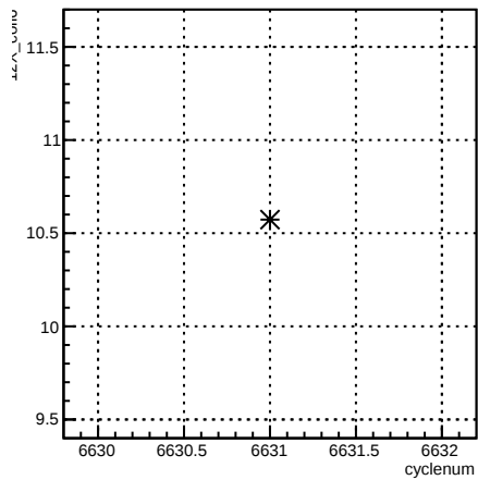
12X_coil6:cyclenum {run == 6616}
