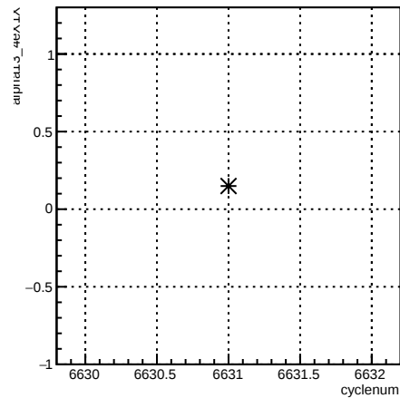
alpha13_4eX1X:cyclenum {run == 6616}
