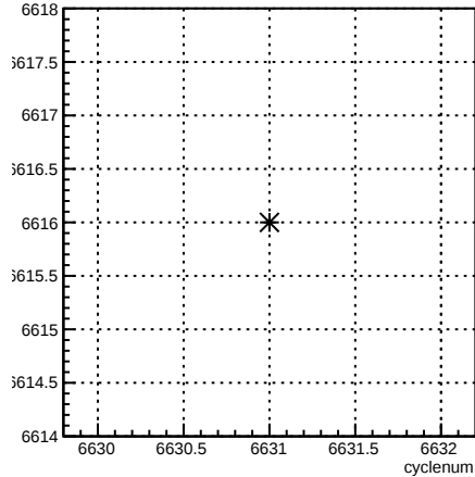
run:cyclenum {run == 6616}
