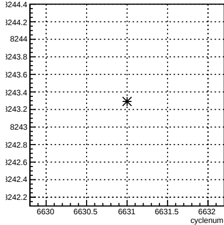
usl_coil7:cyclenum {run == 6616}
