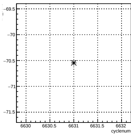
1X_coil3:cyclenum {run == 6616}
