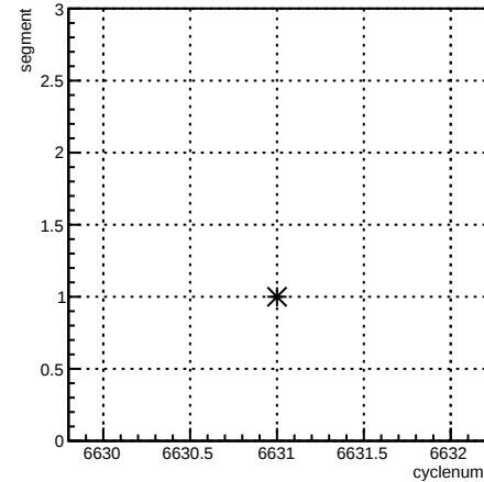
segment:cyclenum {run == 6616}
