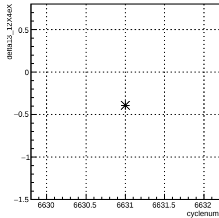
delta13_12X4eX:cyclenum {run == 6616}
