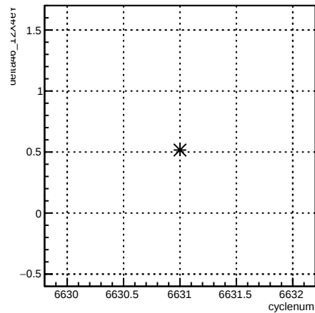
delta46_12X4eY:cyclenum {run == 6616}
