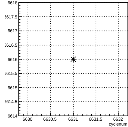
run:cyclenum {run == 6616}
