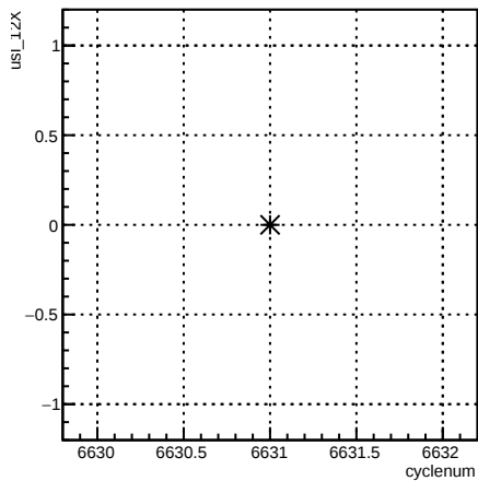
usl_12X:cyclenum {run == 6616}
