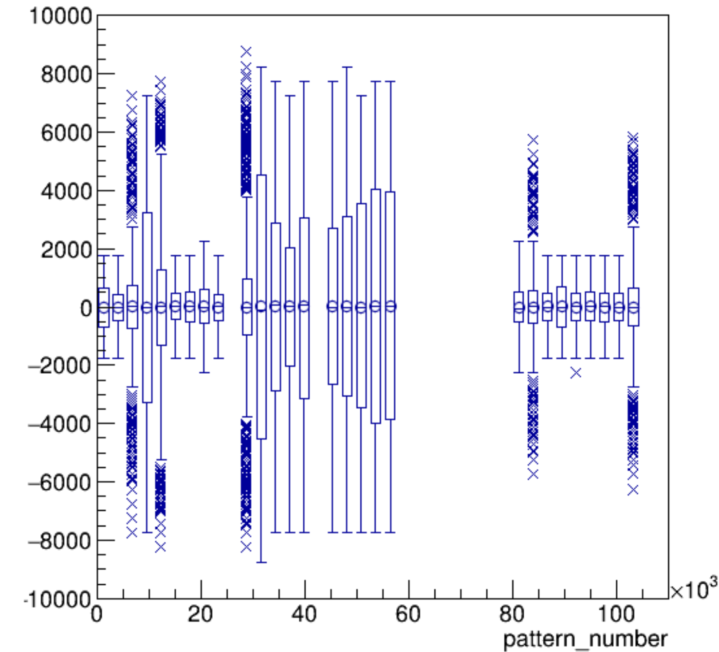
asym_sam7/ppm:pattern_number {ErrorFlag==0}
