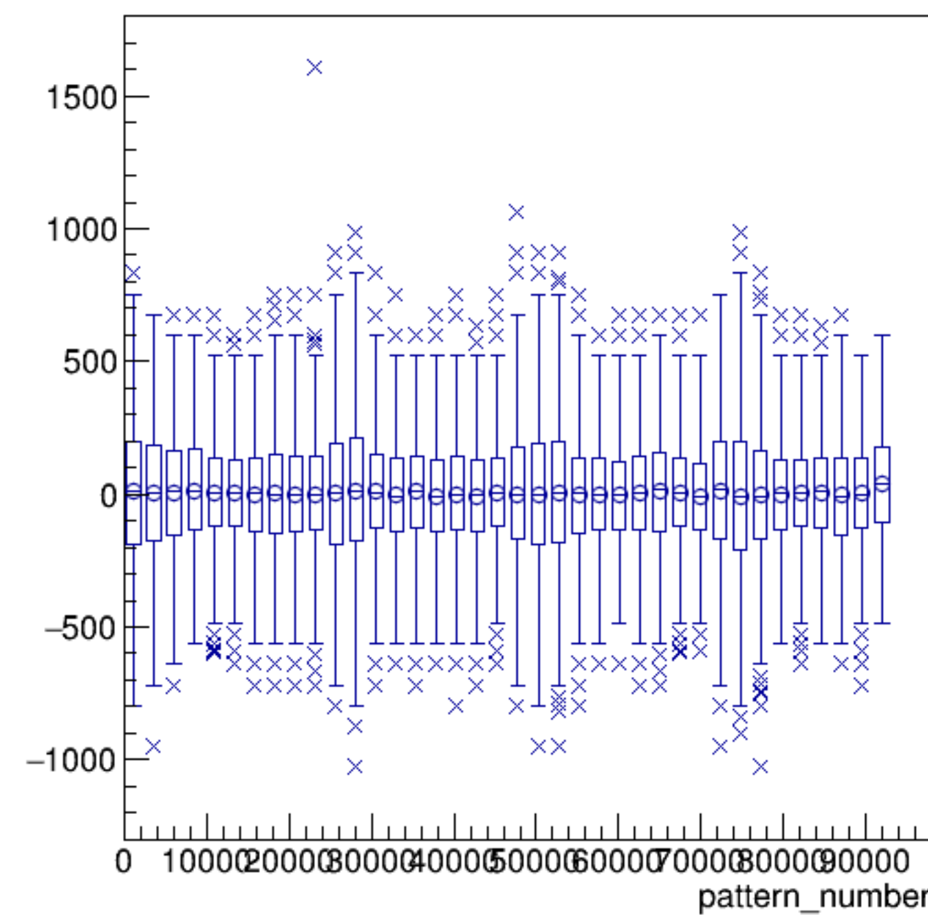
asym_sam8/ppm:pattern_number {ErrorFlag==0}
