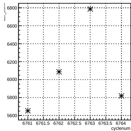
usr_coil4:cyclenum {run == 6664}
