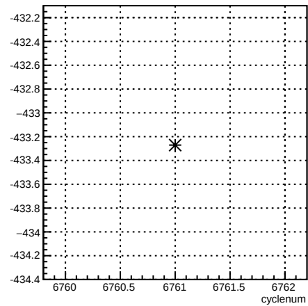
4eX_coil1:cyclenum {run == 6664}
