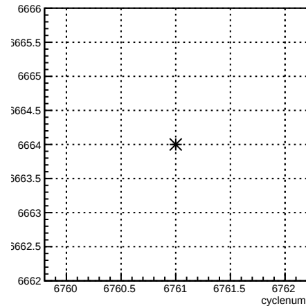
run:cyclenum {run == 6664}
