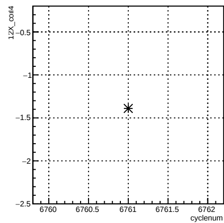
12X_coil4:cyclenum {run == 6664}
