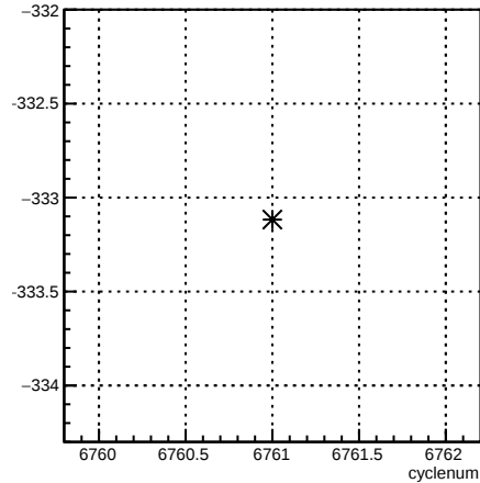
usr_coil6:cyclenum {run == 6664}
