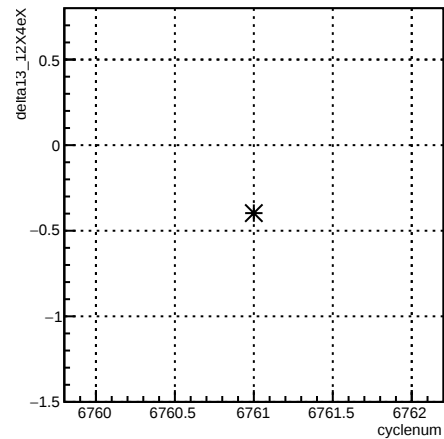
delta13_12X4eX:cyclenum {run == 6664}
