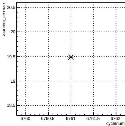
alpha46_4eY4aY:cyclenum {run == 6664}
