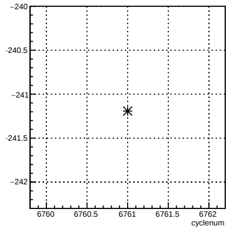
12X_coil1:cyclenum {run == 6664}
