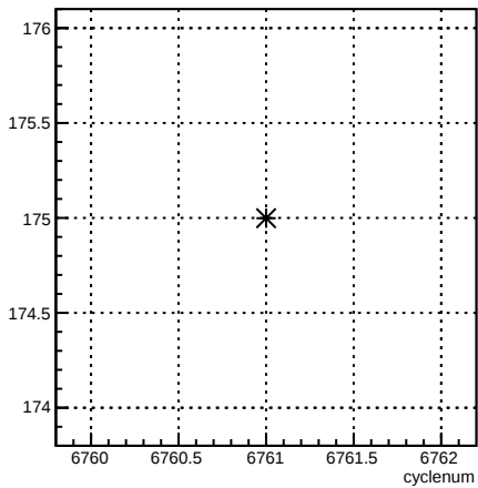
4eY_coil4:cyclenum {run == 6664}
