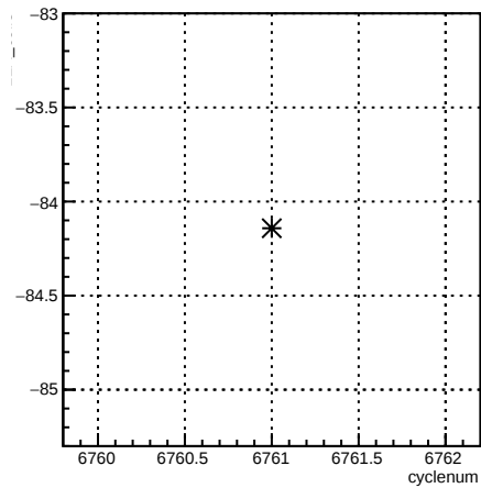
12X_coil3:cyclenum {run == 6664}
