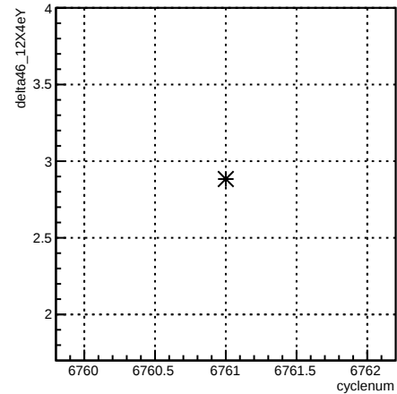
delta46_12X4eY:cyclenum {run == 6664}
