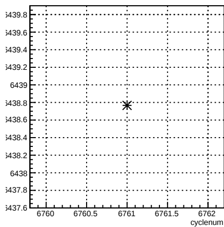
usl_coil3:cyclenum {run == 6664}
