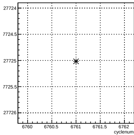
usr_coil1:cyclenum {run == 6664}
