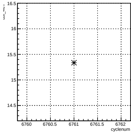
usl_4eY:cyclenum {run == 6664}
