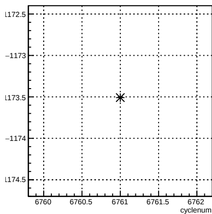
usl_coil6:cyclenum {run == 6664}
