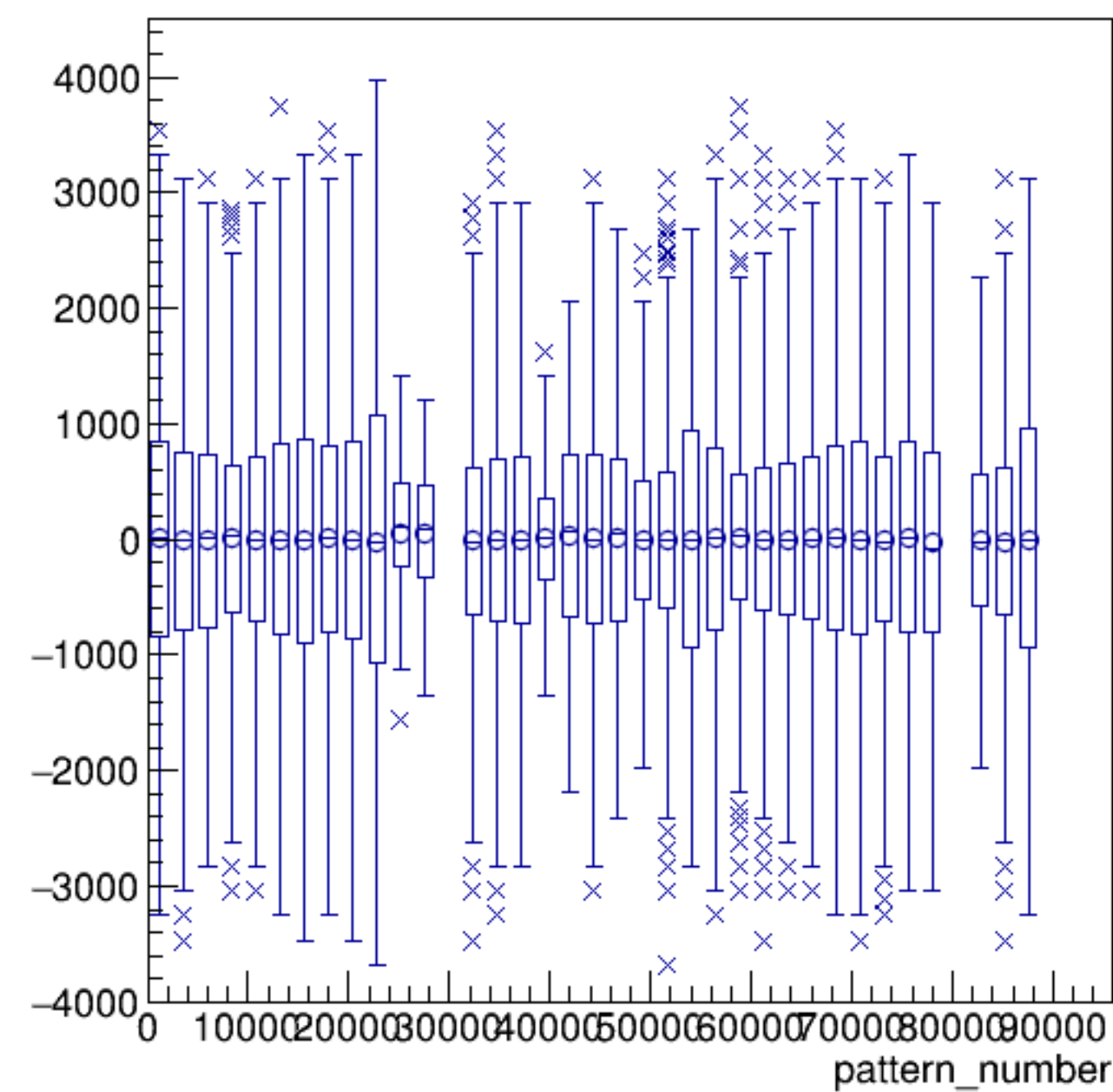
asym_sam1/ppm:pattern_number {ErrorFlag==0}
