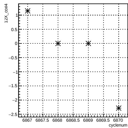
12X_coil4:cyclenum {run == 6726}
