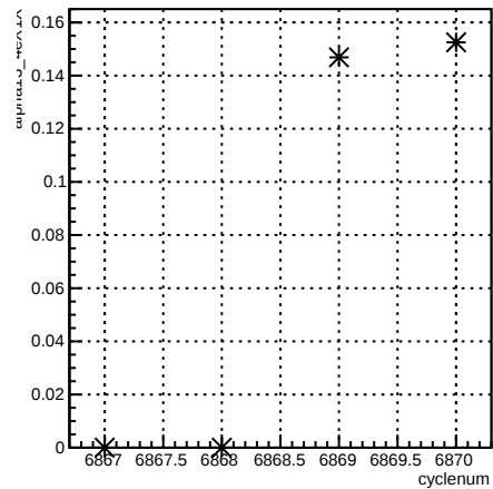
alpha13_4eX1X:cyclenum {run == 6726}
