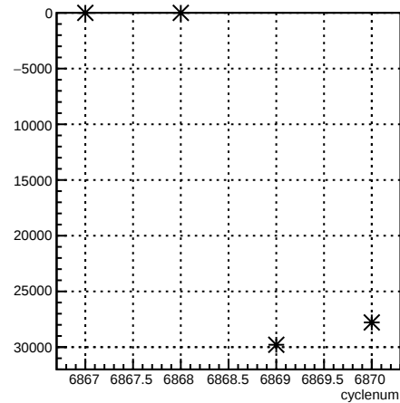
usr_coil1:cyclenum {run == 6726}
