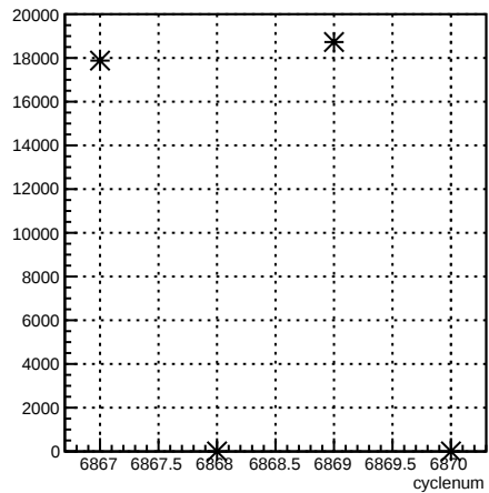
usl_coil7:cyclenum {run == 6726}
