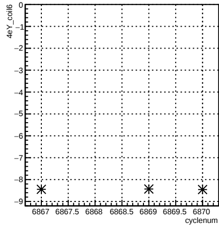
4eY_coil6:cyclenum {run == 6726}
