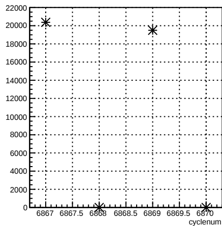
usr_coil7:cyclenum {run == 6726}
