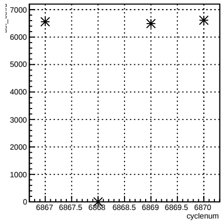
usl_coil7:cyclenum {run == 6726}
