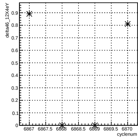
delta46_12X4eY:cyclenum {run == 6726}
