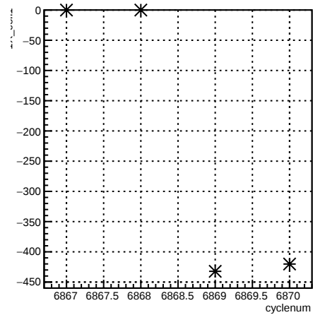
1X_coil1:cyclenum {run == 6726}
