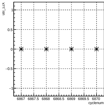
usl_12X:cyclenum {run == 6726}
