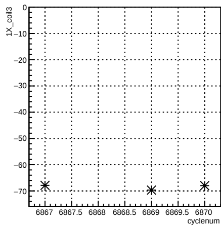
1X_coil3:cyclenum {run == 6726}
