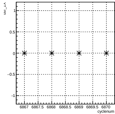
usr_4eY:cyclenum {run == 6726}
