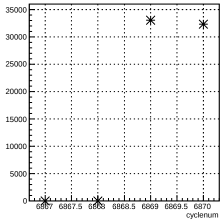
usl_coil6:cyclenum {run == 6726}
