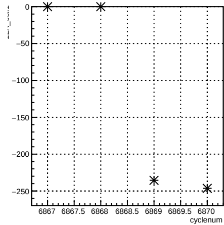
12X_coil1:cyclenum {run == 6726}
