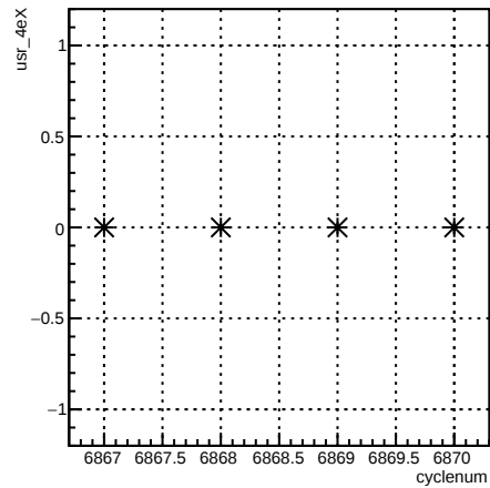
run:cyclenum {run == 6726}
