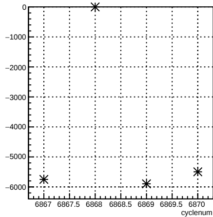
usr_coil3:cyclenum {run == 6726}
