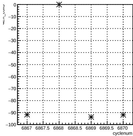
4eX_coil3:cyclenum {run == 6726}
