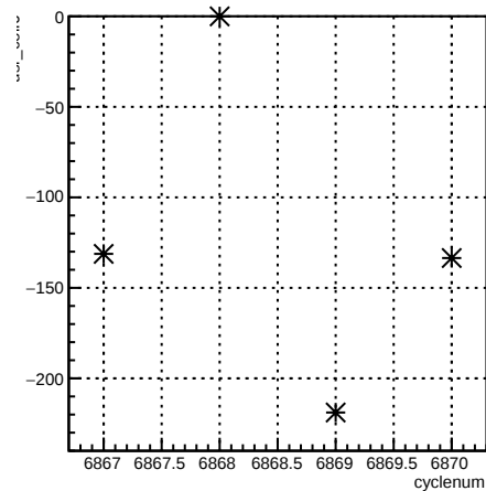
usr_coil6:cyclenum {run == 6726}
