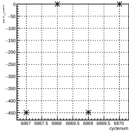
12X_coil7:cyclenum {run == 6726}
