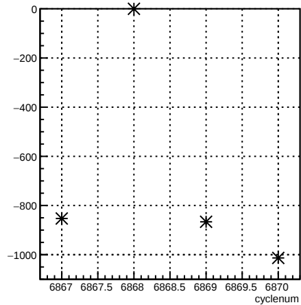
usl_coil6:cyclenum {run == 6726}
