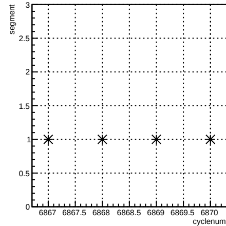
segment:cyclenum {run == 6726}
