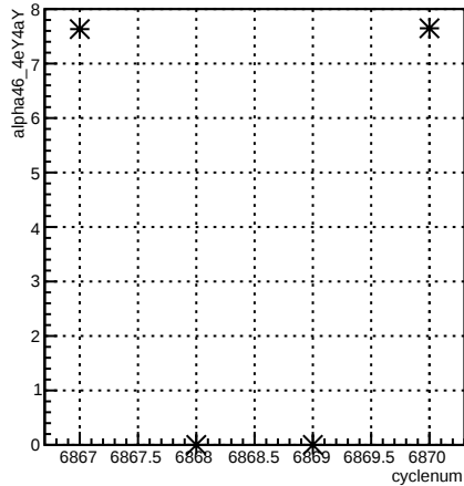
alpha46_4eY4aY:cyclenum {run == 6726}
