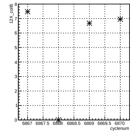
12X_coil6:cyclenum {run == 6726}
