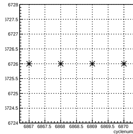
run:cyclenum {run == 6726}
