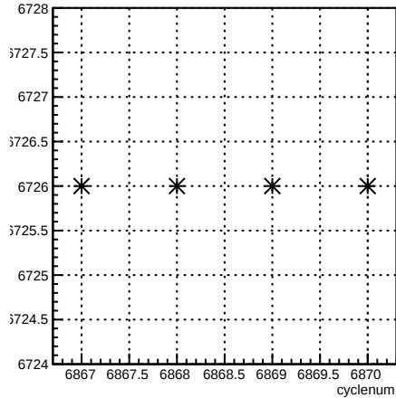
run:cyclenum {run == 6726}
