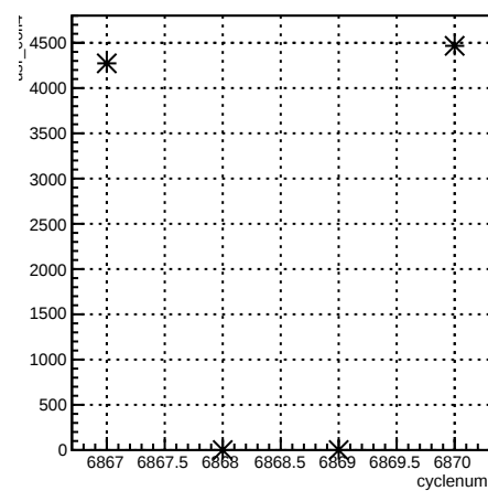
usr_coil4:cyclenum {run == 6726}
