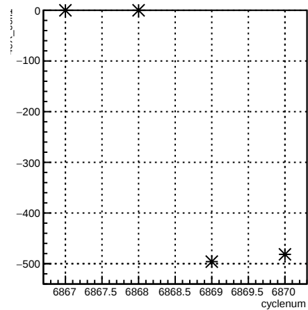
4eX_coil1:cyclenum {run == 6726}
