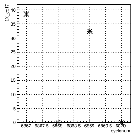
1X_coil7:cyclenum {run == 6726}
