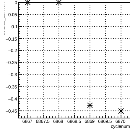
delta13_12X4eX:cyclenum {run == 6726}
