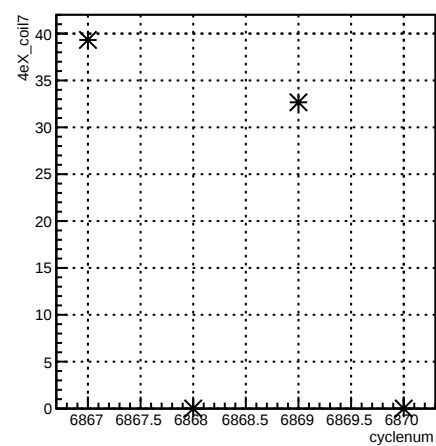
4eX_coil7:cyclenum {run == 6726}
