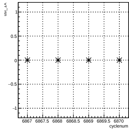
usl_4eY:cyclenum {run == 6726}
