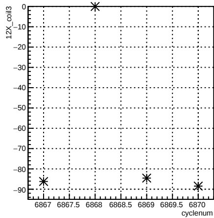
12X_coil3:cyclenum {run == 6726}
