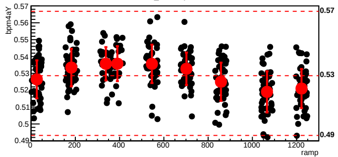
bmod_trim3,cyc=6927
