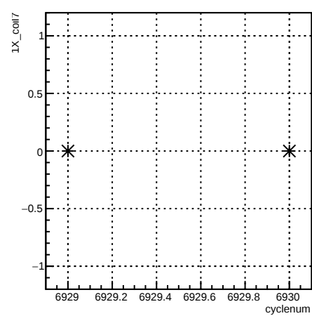
1X_coil7:cyclenum {run == 6782}
