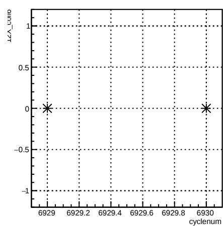
12X_coil6:cyclenum {run == 6782}
