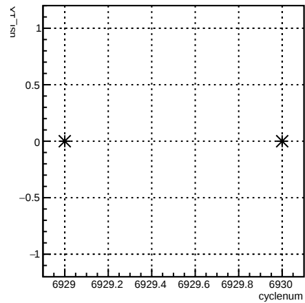
usl_4eY:cyclenum {run == 6782}
