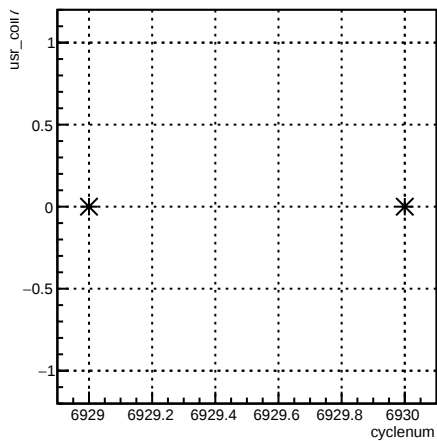
usr_coil7:cyclenum {run == 6782}
