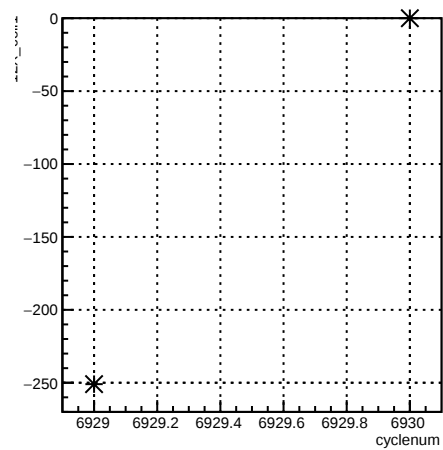
12X_coil1:cyclenum {run == 6782}
