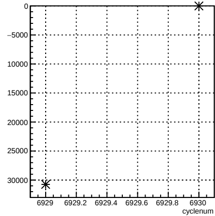
usr_coil1:cyclenum {run == 6782}
