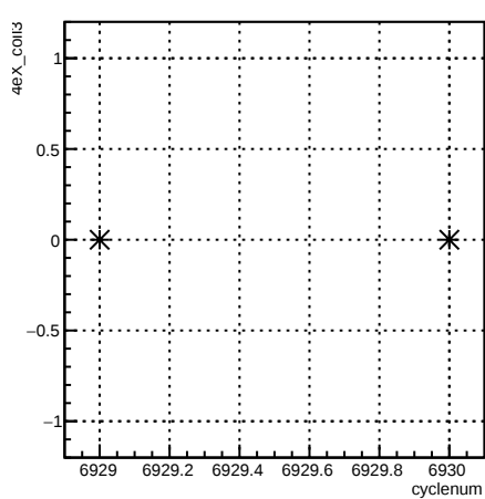
4eX_coil3:cyclenum {run == 6782}
