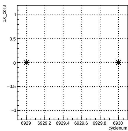
1X_coil3:cyclenum {run == 6782}
