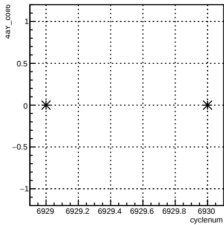
4eY_coil6:cyclenum {run == 6782}
