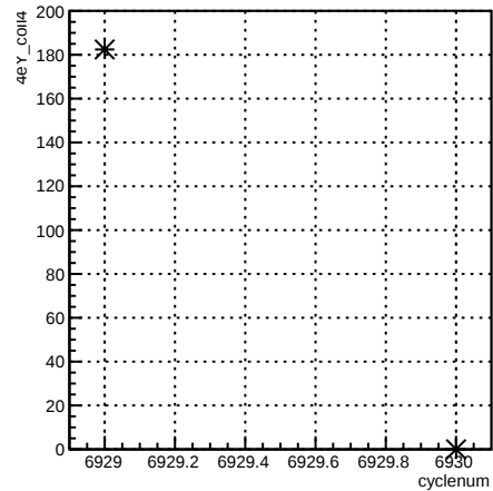
4eY_coil4:cyclenum {run == 6782}
