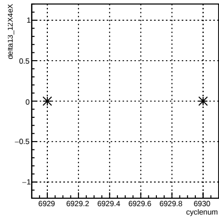
delta13_12X4eX:cyclenum {run == 6782}
