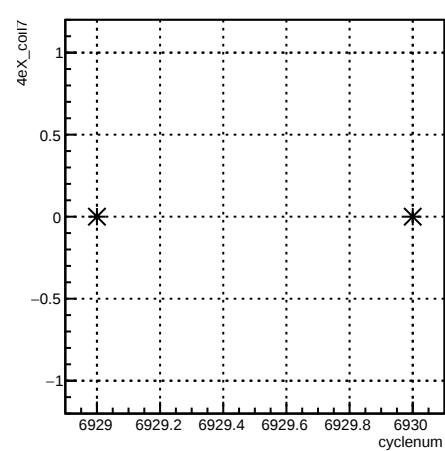
4eX_coil7:cyclenum {run == 6782}
