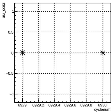
usr_coil3:cyclenum {run == 6782}
