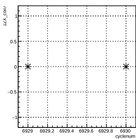
12X_coil7:cyclenum {run == 6782}
