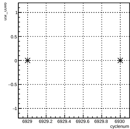
usr_coil6:cyclenum {run == 6782}
