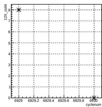
12X_coil4:cyclenum {run == 6782}
