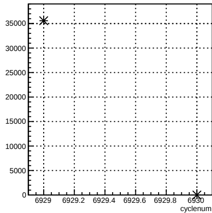
usl_coil6:cyclenum {run == 6782}
