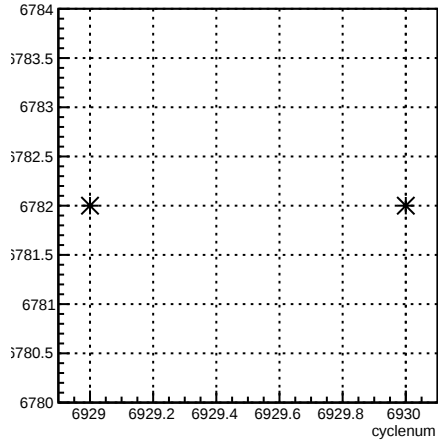
run:cyclenum {run == 6782}
