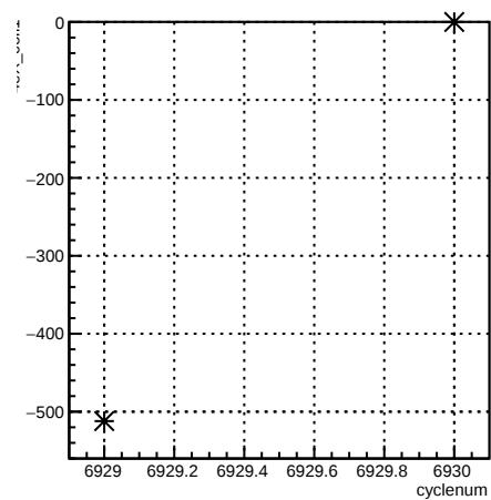
4eX_coil1:cyclenum {run == 6782}
