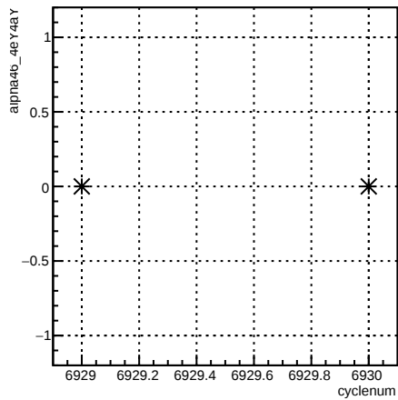
alpha46_4eY4aY:cyclenum {run == 6782}
