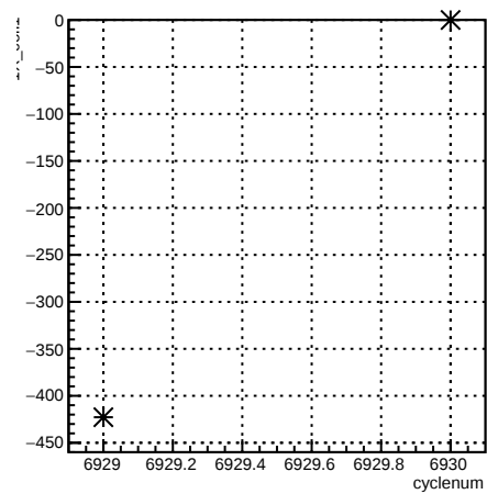
1X_coil1:cyclenum {run == 6782}
