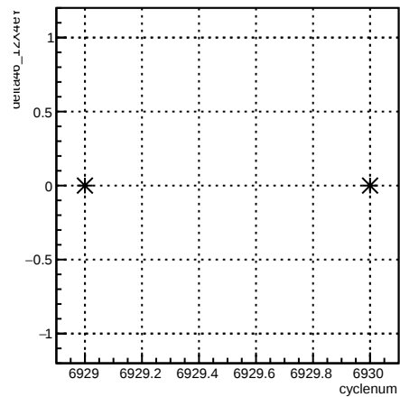
delta46_12X4eY:cyclenum {run == 6782}
