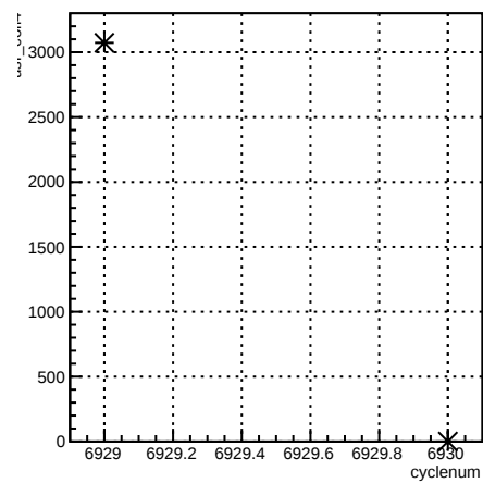
usr_coil4:cyclenum {run == 6782}
