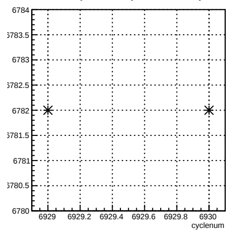
run:cyclenum {run == 6782}
