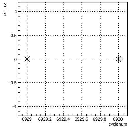
usr_4eY:cyclenum {run == 6782}
