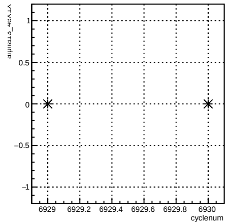
alpha13_4eX1X:cyclenum {run == 6782}
