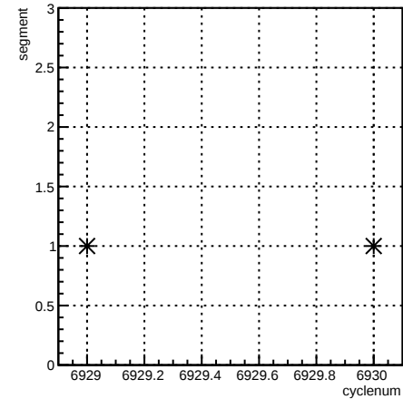
segment:cyclenum {run == 6782}
