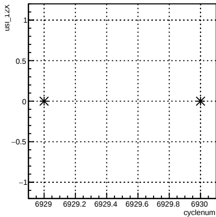
usl_12X:cyclenum {run == 6782}
