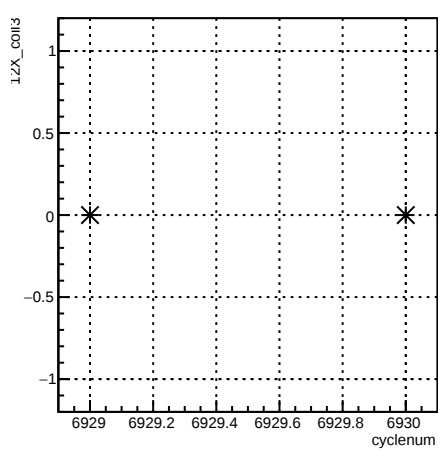
12X_coil3:cyclenum {run == 6782}
