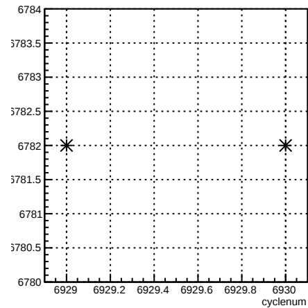
run:cyclenum {run == 6782}
