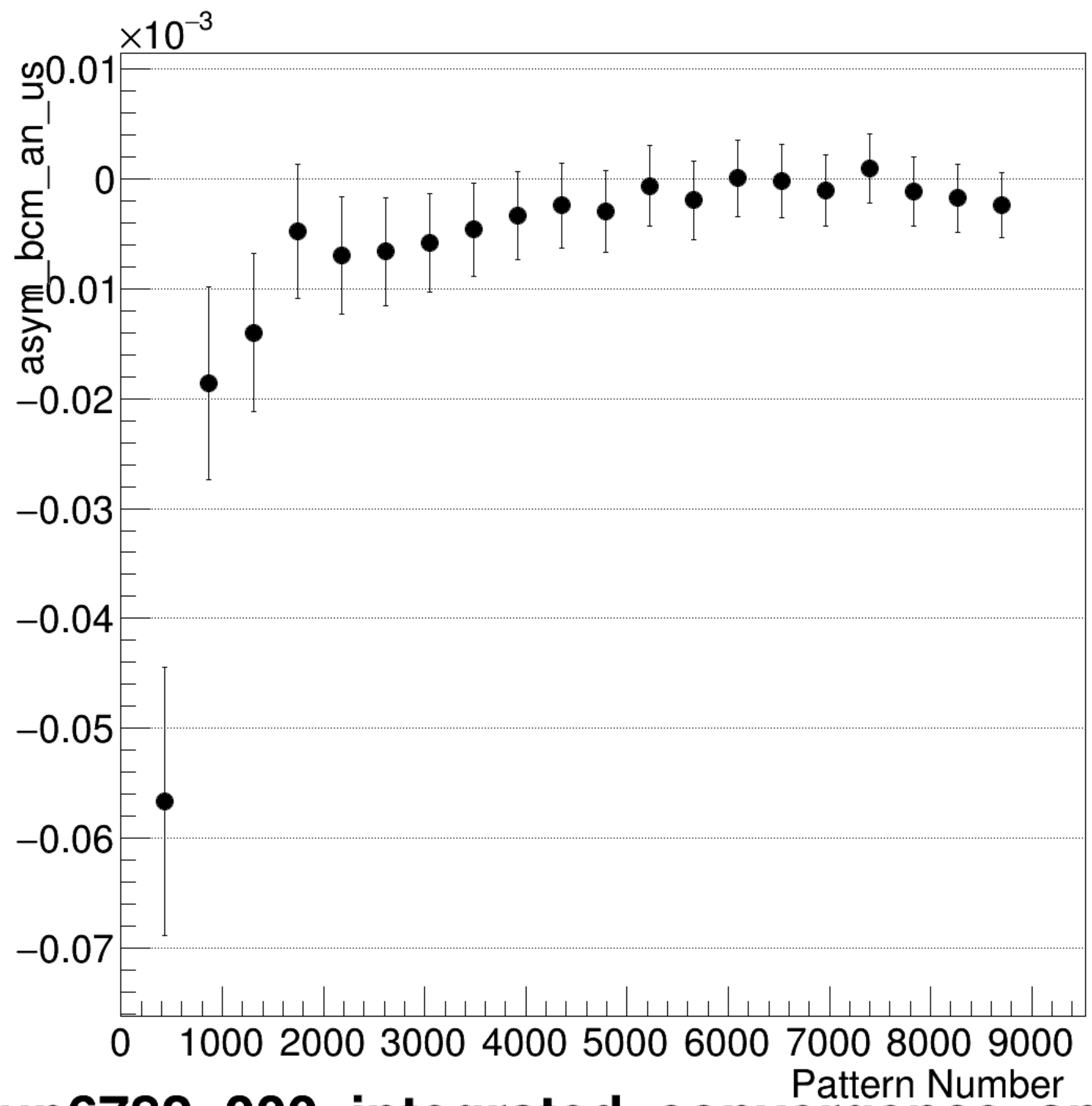
asym_bcm_an_us Integrated Convergence
