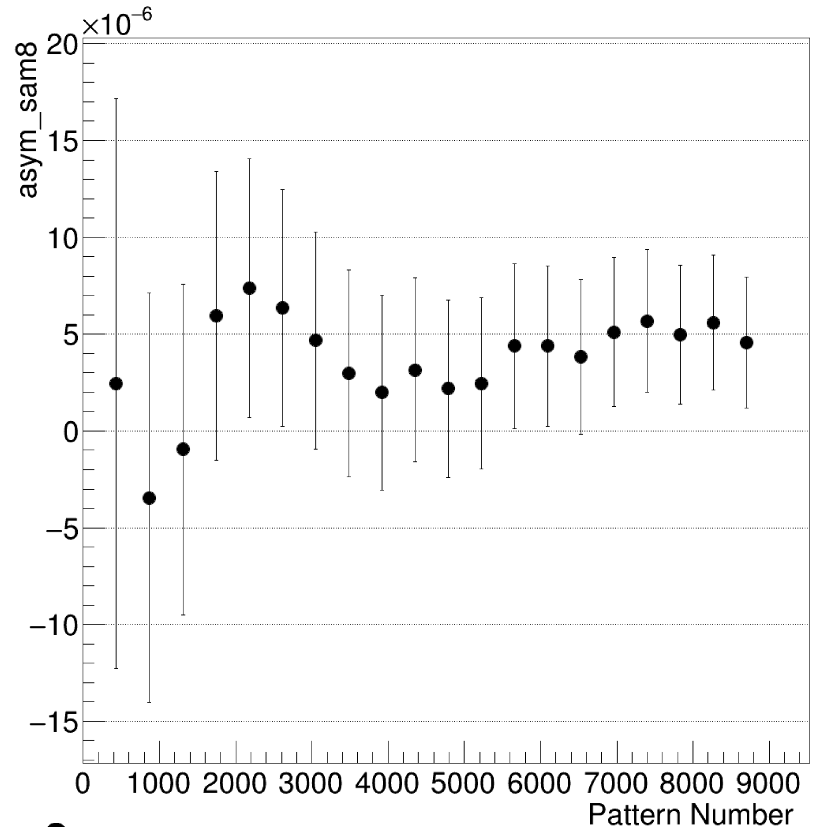
asym_sam8 Integrated Convergence
