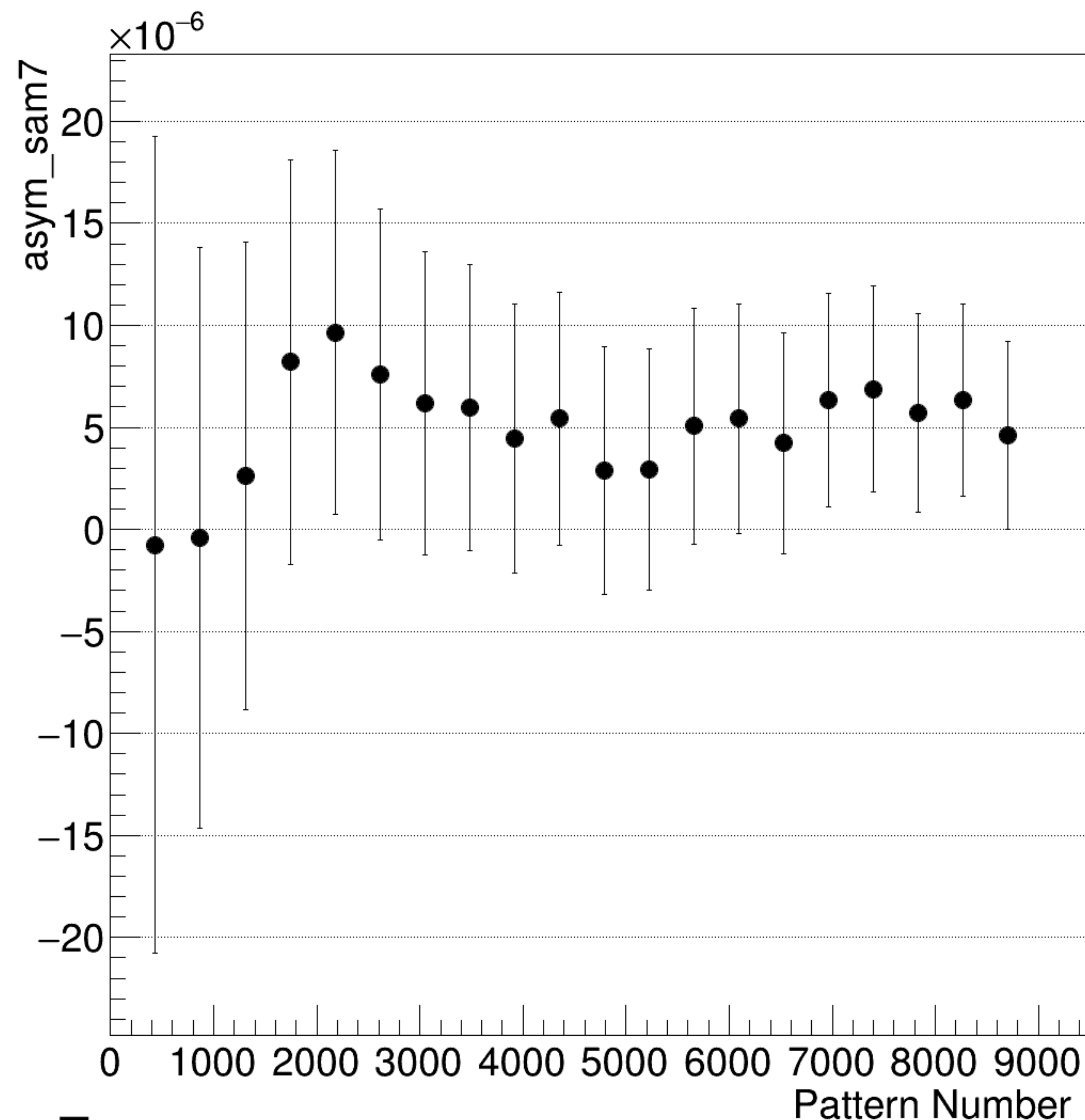
asym_sam7 Integrated Convergence
