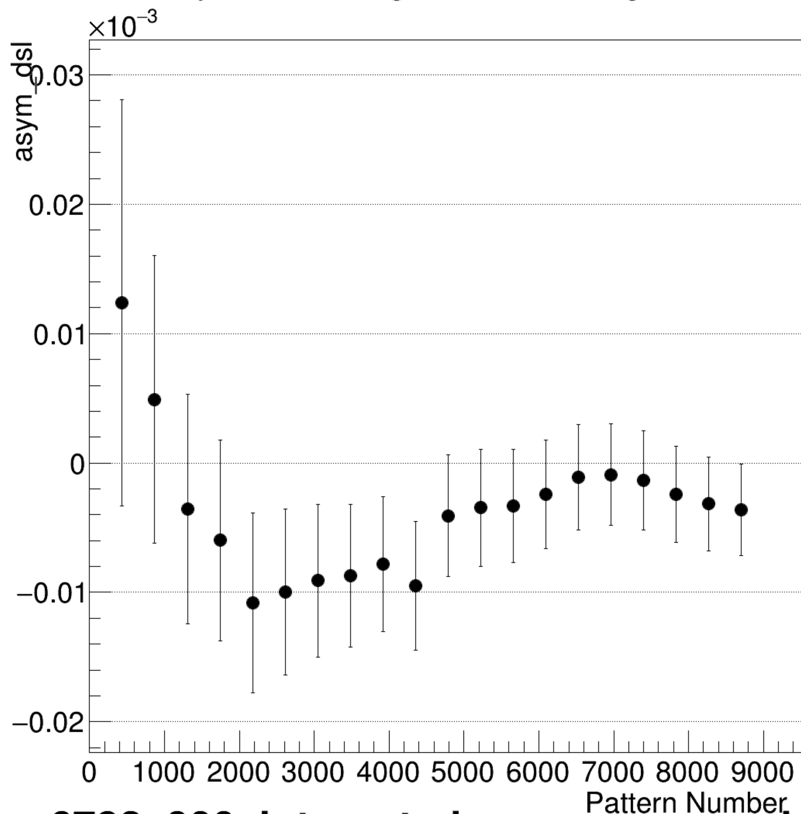
asym_dsl Integrated Convergence
