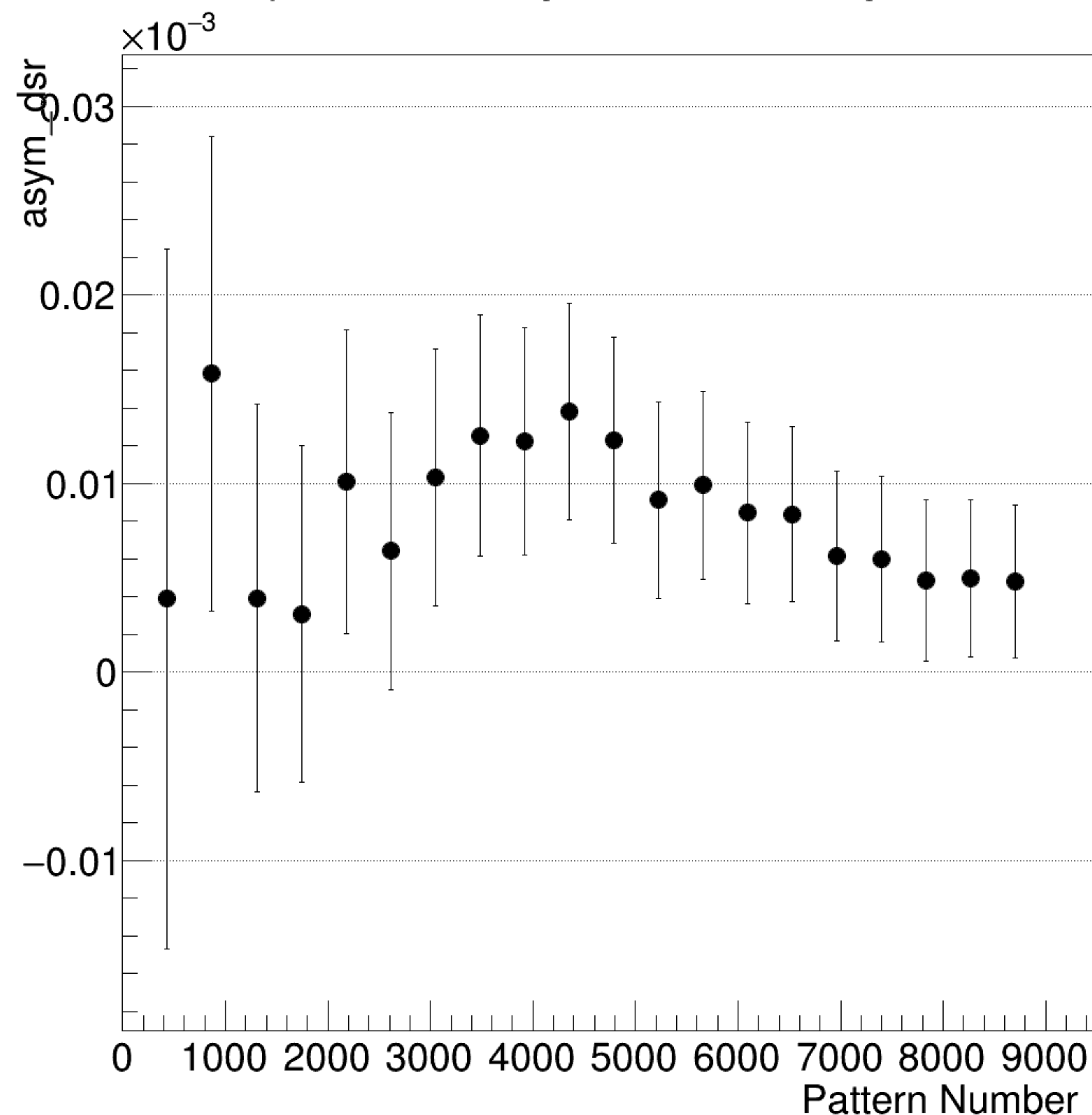
asym_dsr Integrated Convergence
