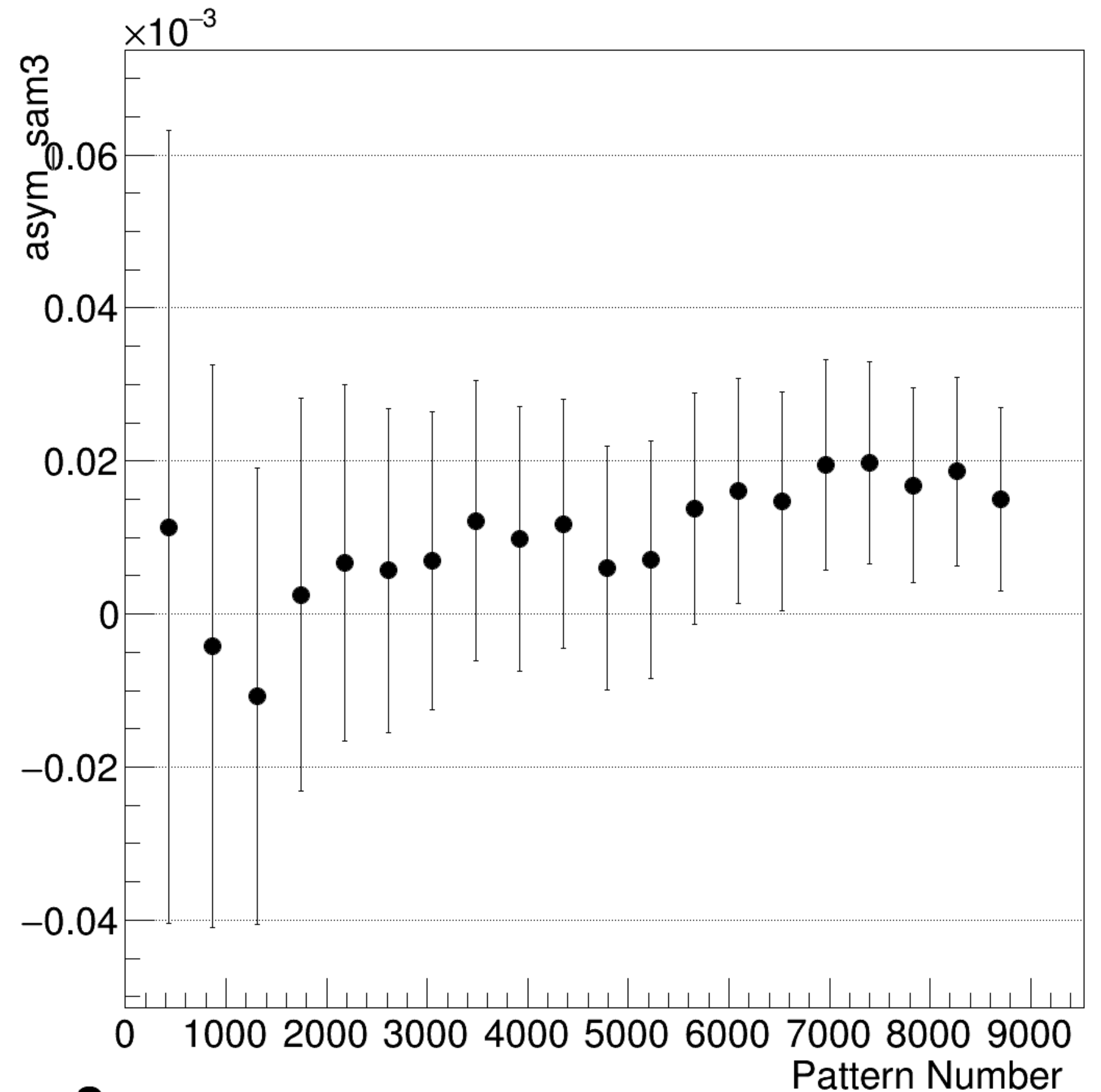
asym_sam3 Integrated Convergence
