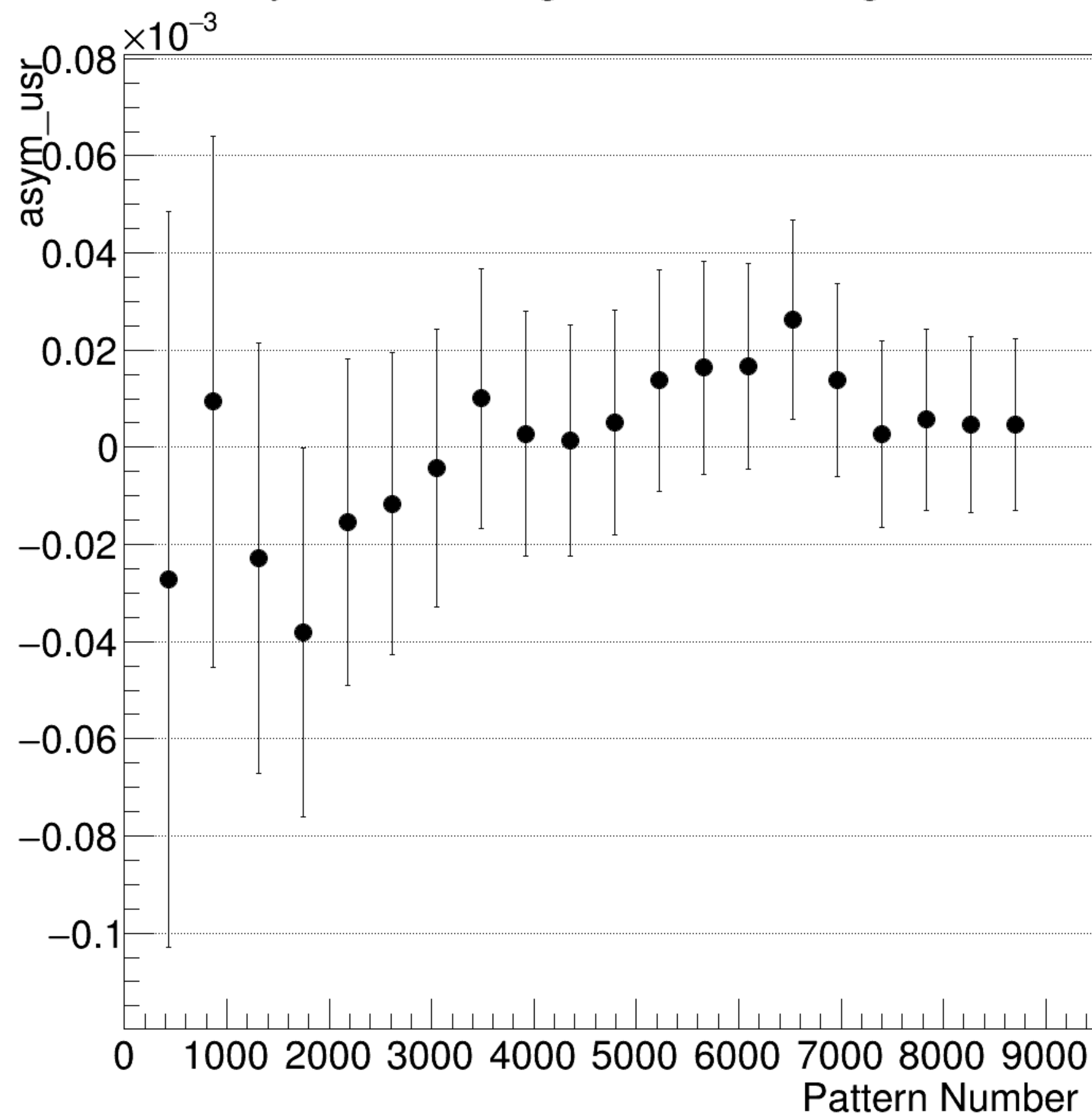
asym_usr Integrated Convergence
