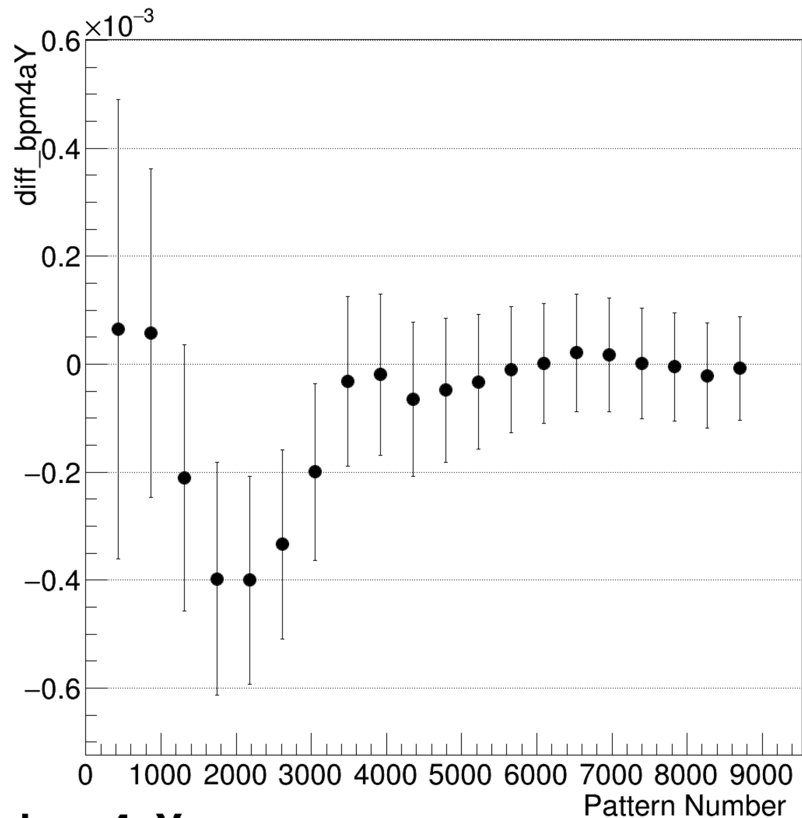
diff_bpm4aY Integrated Convergence
