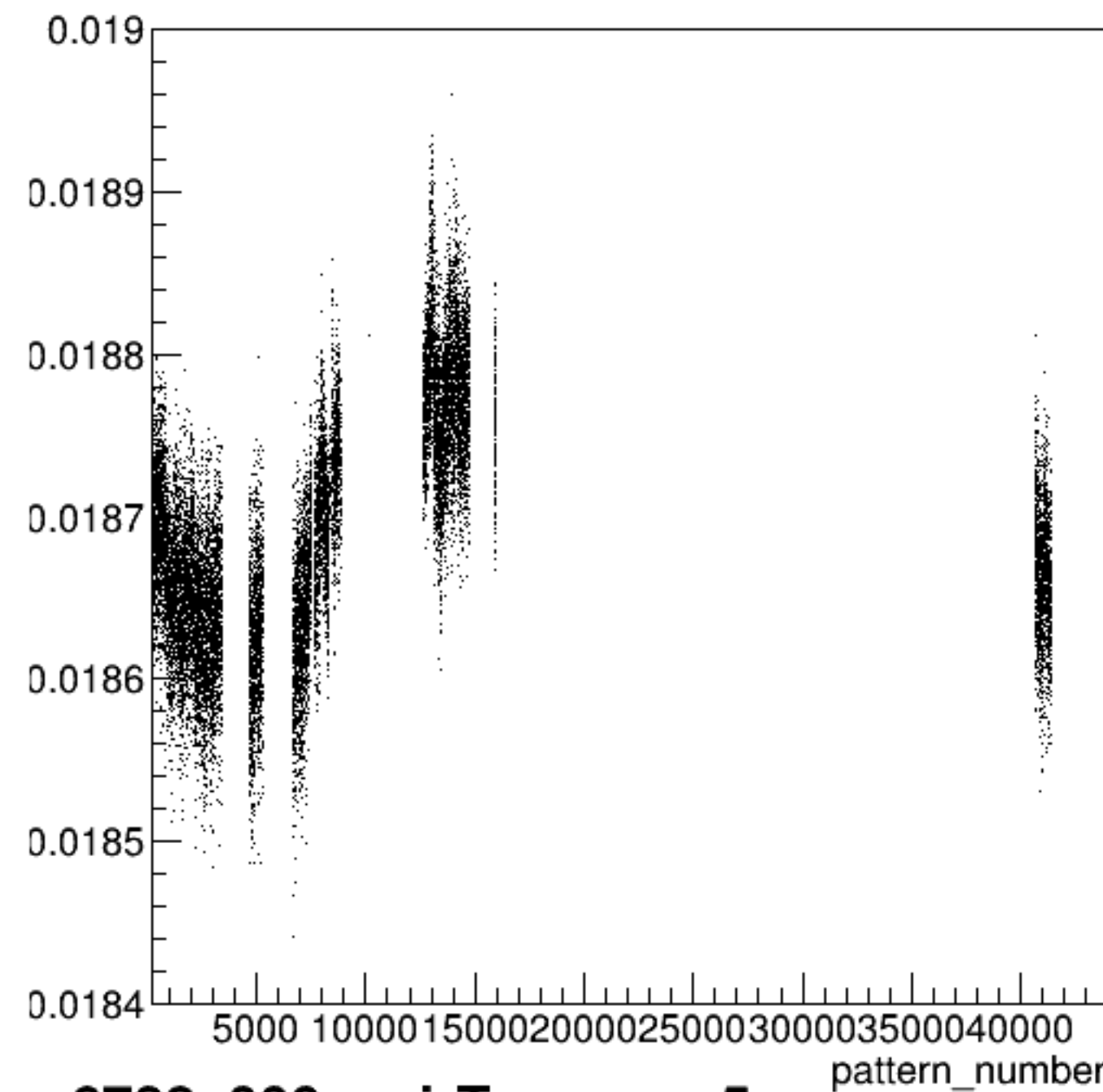
yield_sam5:pattern_number {ErrorFlag==0}
