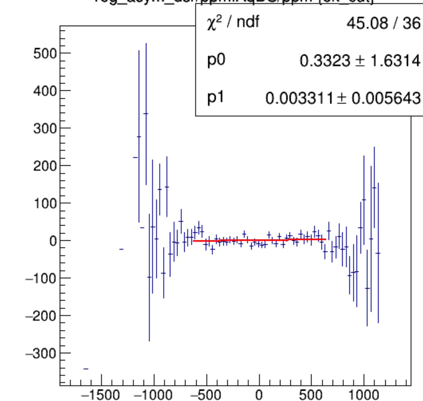
reg_asym_dsr/ppm:AqDS/ppm {ok_cut}
