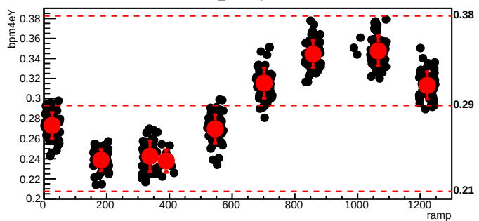
bmod_trim6,cyc=6963
