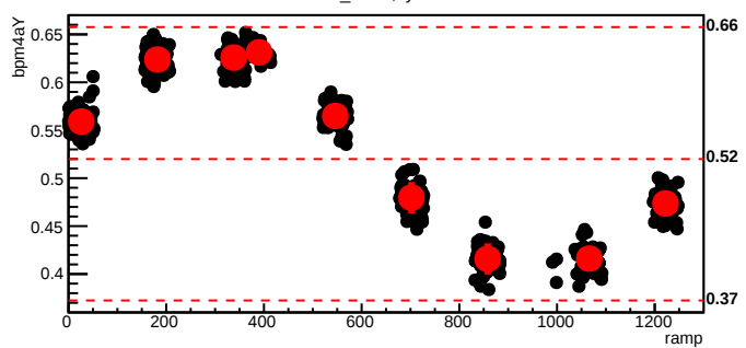
bmod_trim4,cyc=6963
