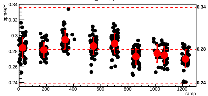
bmod_trim3,cyc=6963
