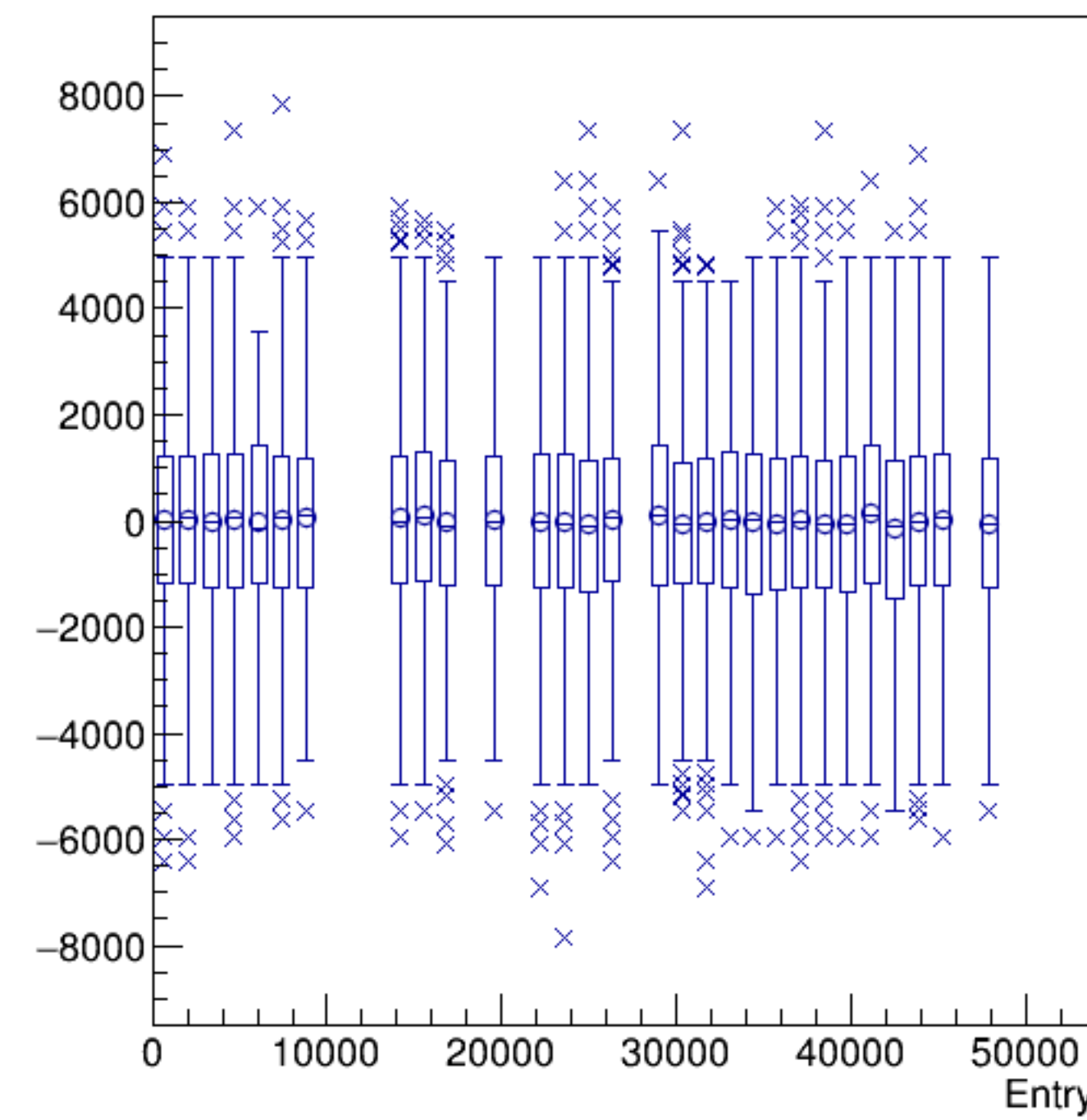
(reg_asym_atl1/ppm+reg_asym_atr1/ppm)/2:Entry$ {ok_cut}
