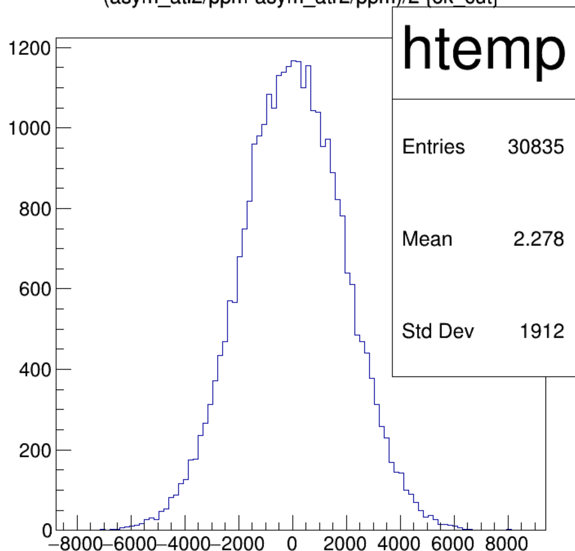
(asym_atl2/ppm-asym_atr2/ppm)/2 {ok_cut}
