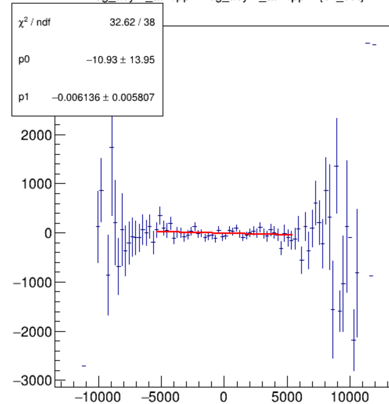
reg_asym_atl1/ppm:reg_asym_atr1/ppm {ok_cut}
