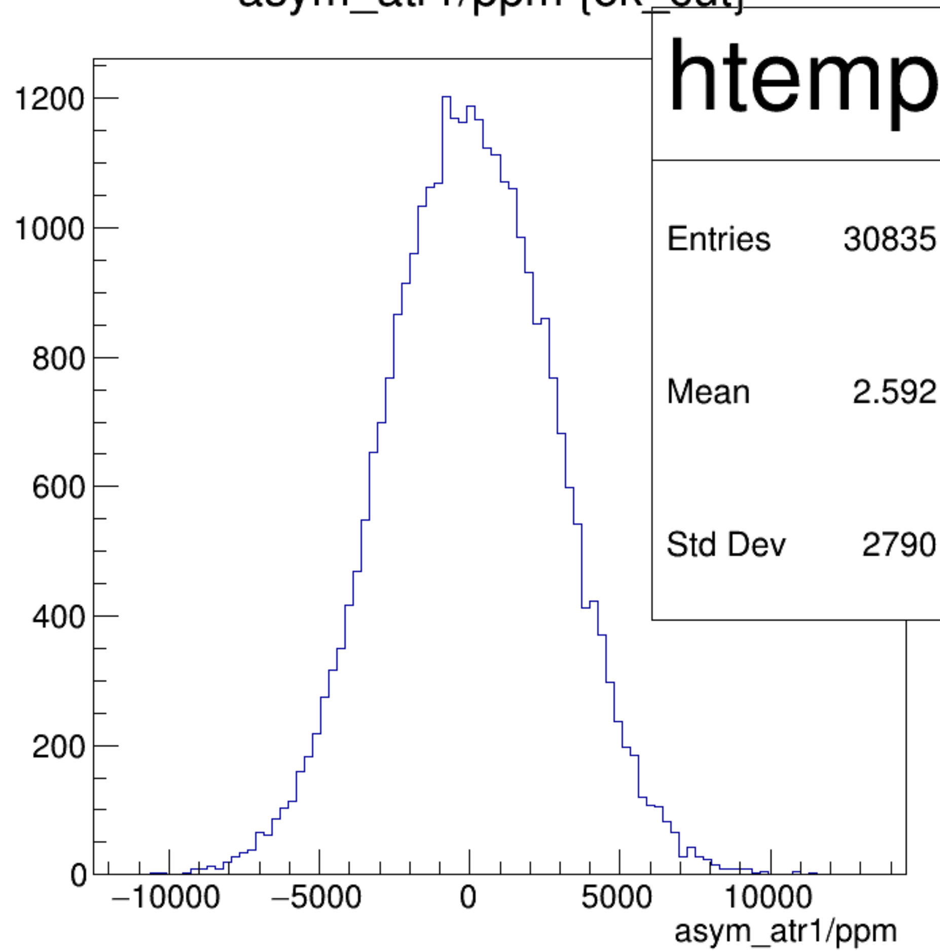
asym_atr1/ppm {ok_cut}
