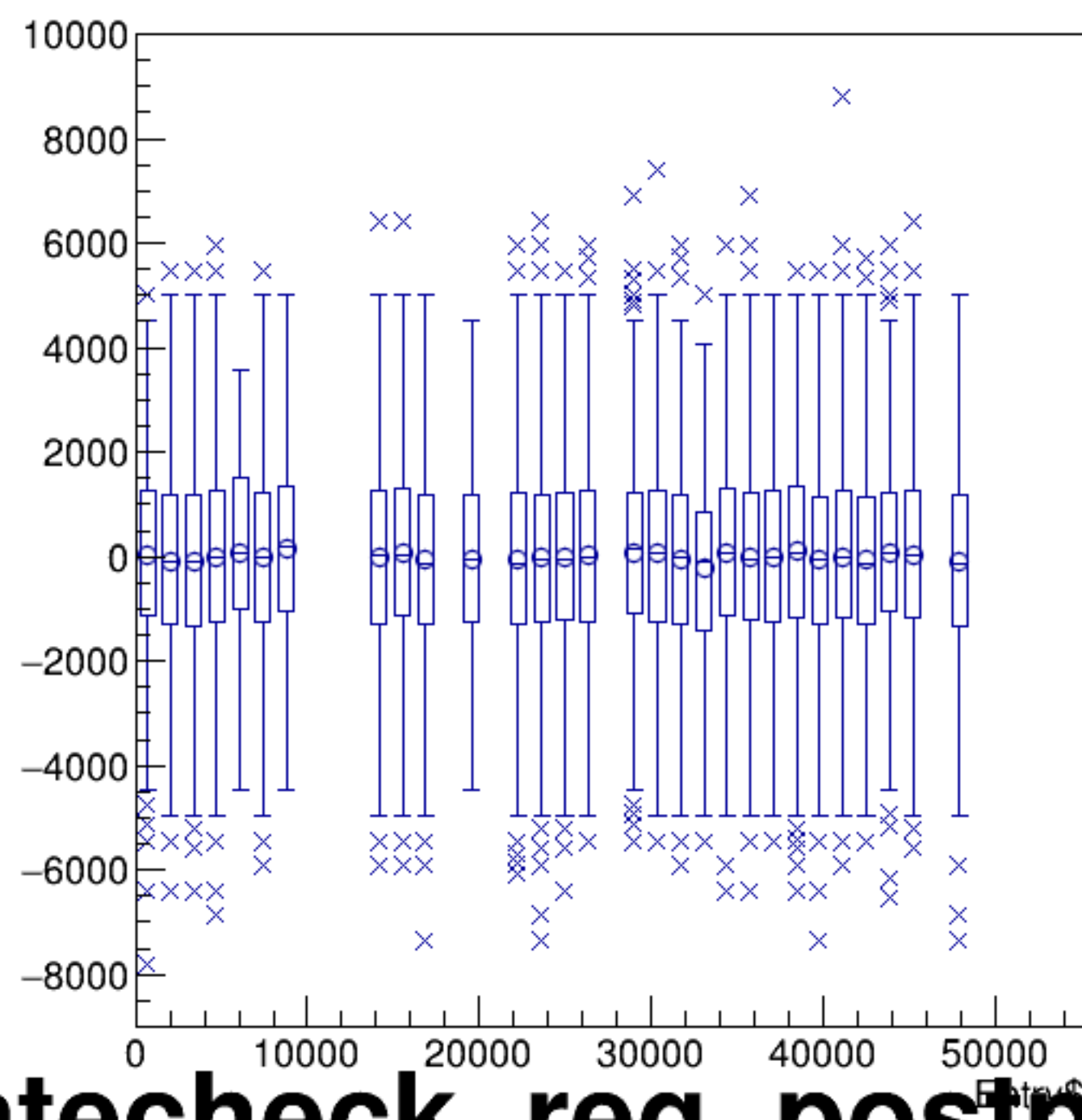
(reg_asym_atl1/ppm-reg_asym_atr1/ppm)/2:Entry$ {ok_cut}
