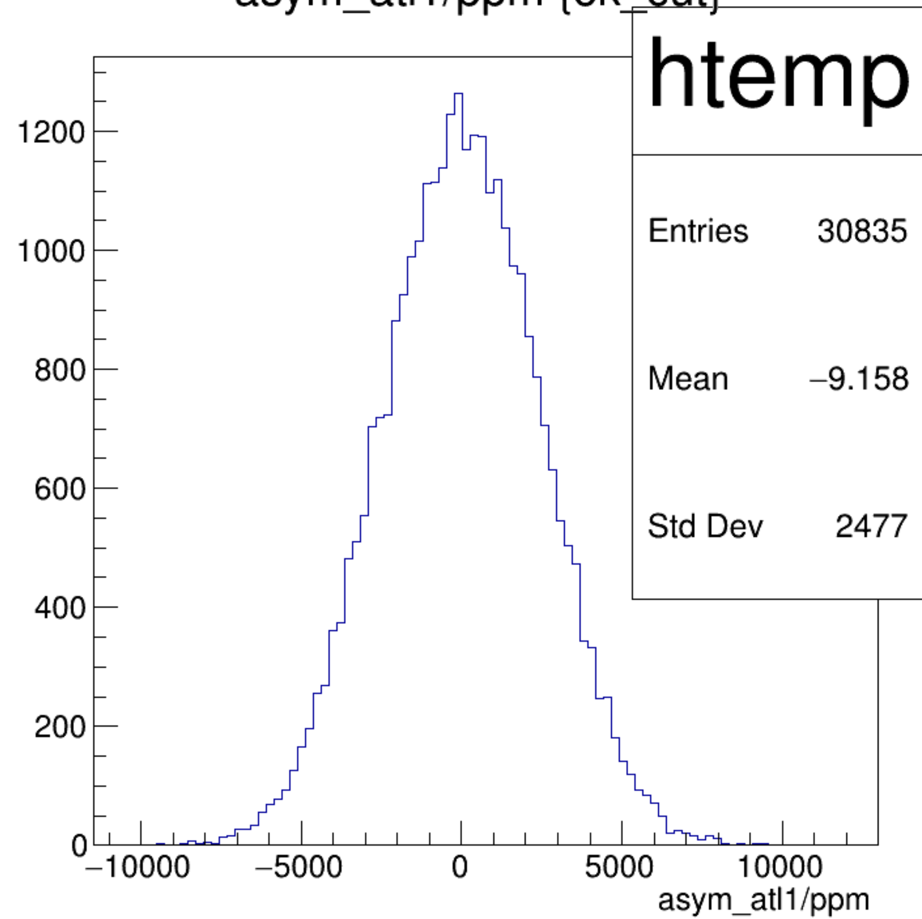
asym_atl1/ppm {ok_cut}
