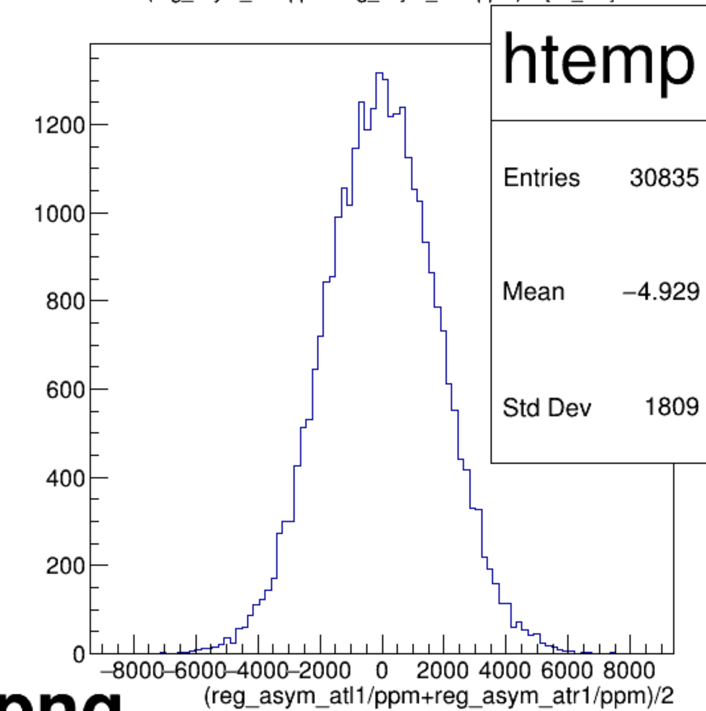
(reg_asym_atl1/ppm+reg_asym_atr1/ppm)/2 {ok_cut}
