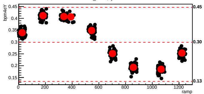
bmod_trim4,cyc=7048
