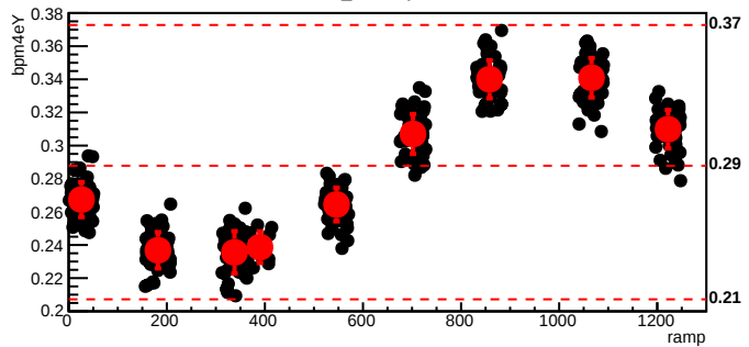
bmod_trim6,cyc=7048
