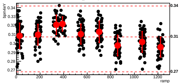
bmod_trim3,cyc=7048
