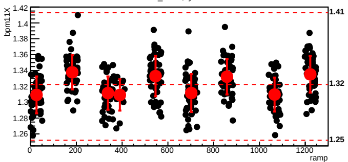
bmod_trim4,cyc=7048
