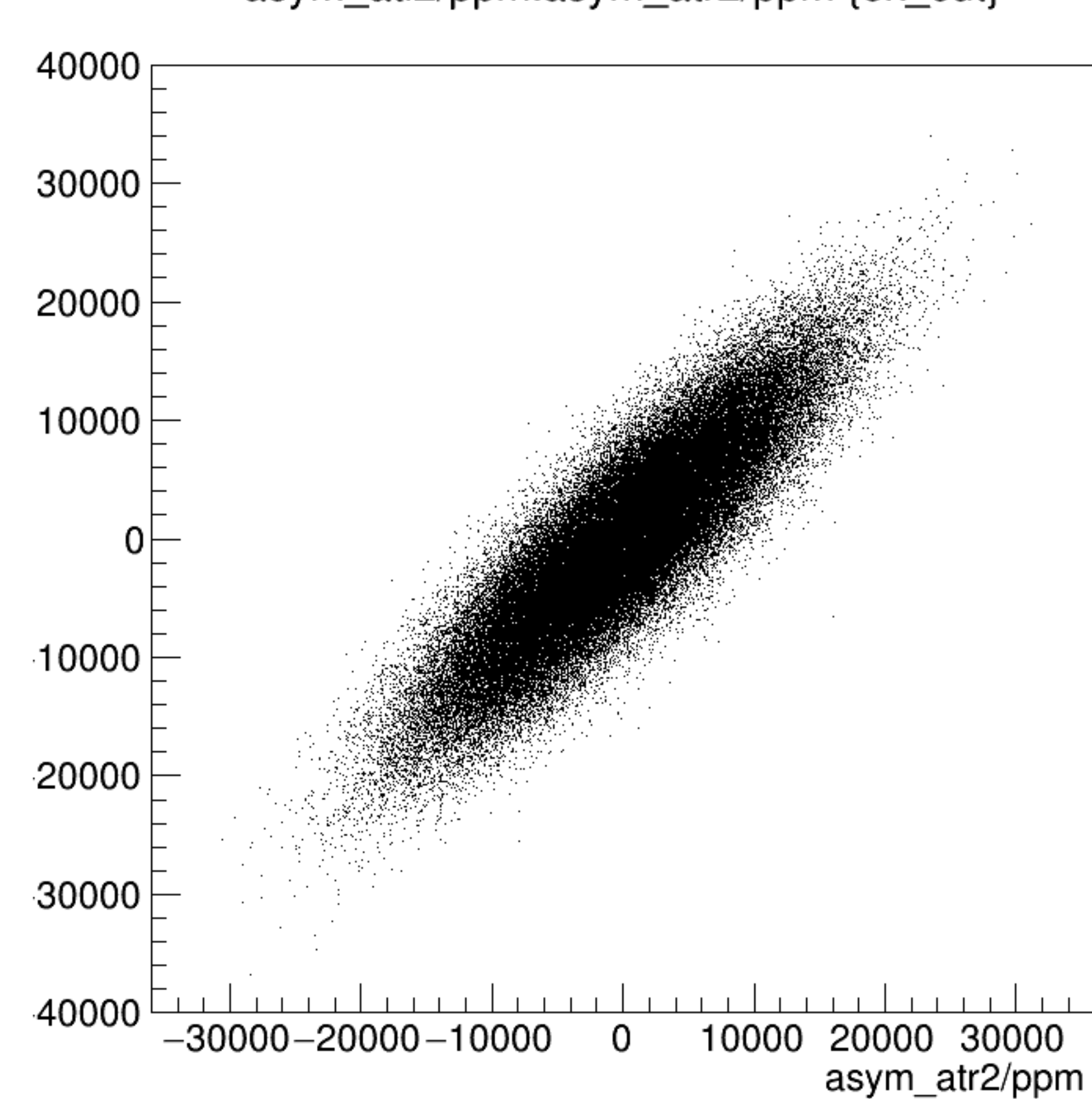
asym_atl2/ppm:asym_atr2/ppm {ok_cut}
