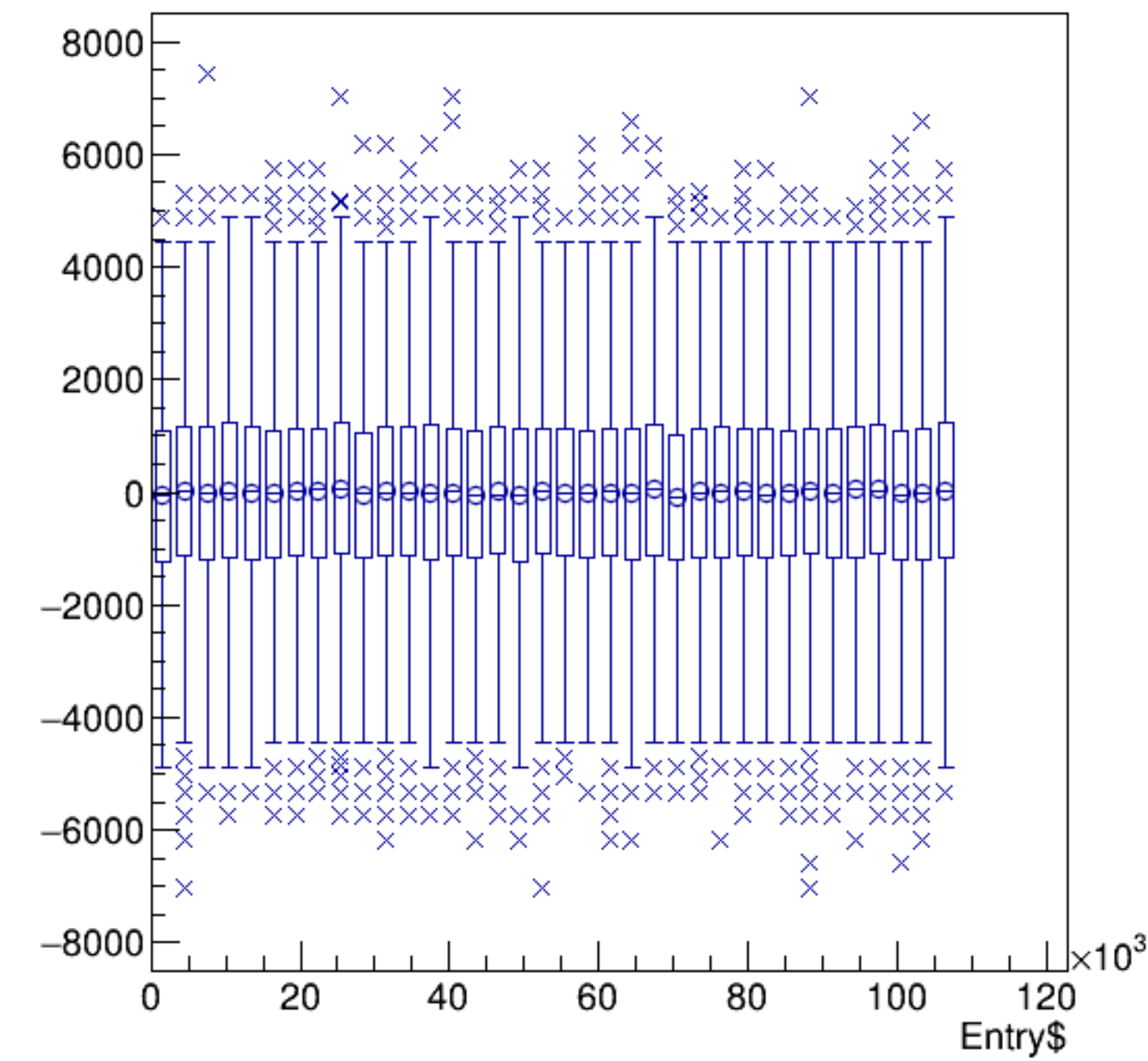
(reg_asym_atl2/ppm-reg_asym_atr2/ppm)/2:Entry$ {ok_cut}
