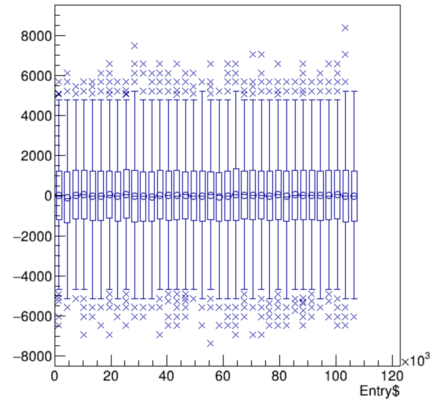
(reg_asym_atl1/ppm+reg_asym_atr1/ppm)/2:Entry$ {ok_cut}
