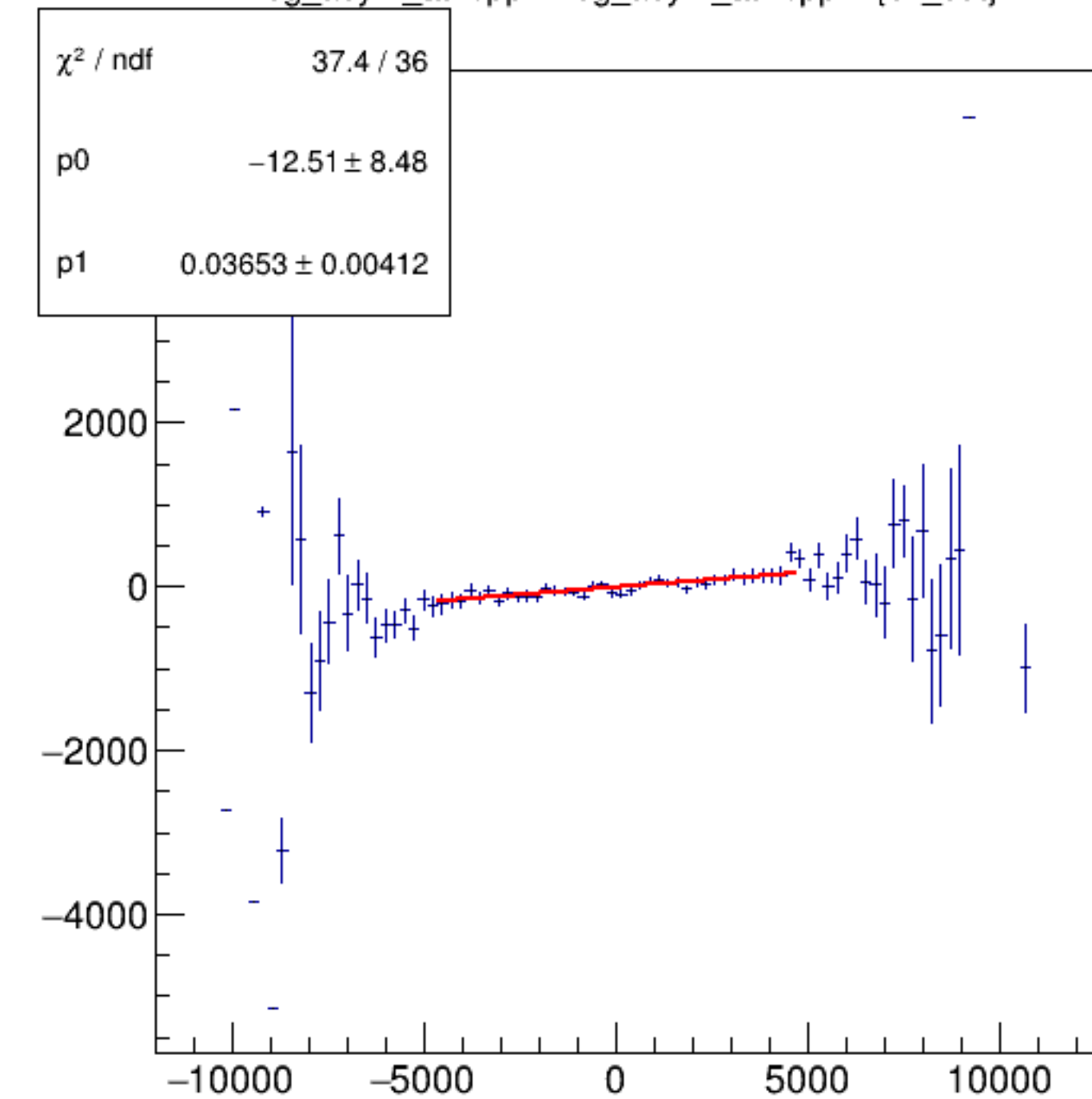
reg_asym_atl2/ppm:reg_asym_atr2/ppm {ok_cut}
