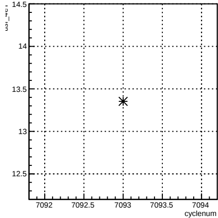
usr_4eY:cyclenum {run == 6818}
