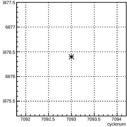
usl_coil7:cyclenum {run == 6818}
