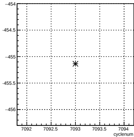
12X_coil7:cyclenum {run == 6818}
