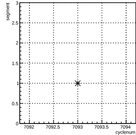
segment:cyclenum {run == 6818}
