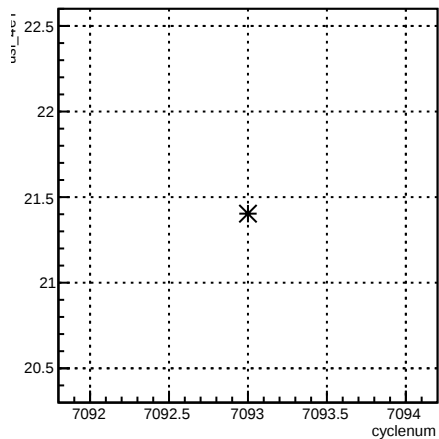
usl_4eY:cyclenum {run == 6818}
