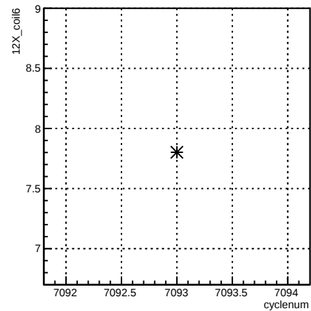
12X_coil6:cyclenum {run == 6818}
