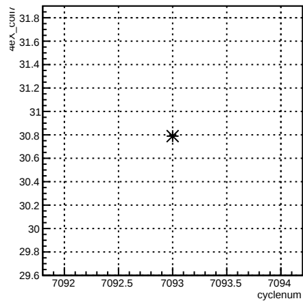
4eX_coil7:cyclenum {run == 6818}
