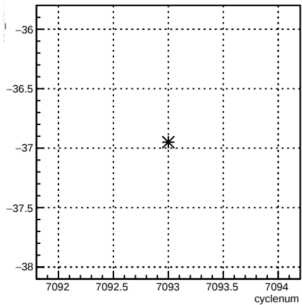
usr_12X:cyclenum {run == 6818}
