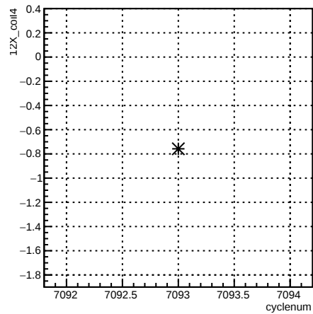
12X_coil4:cyclenum {run == 6818}
