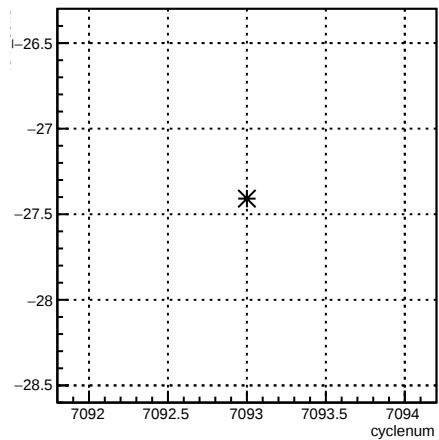
4eY_coil6:cyclenum {run == 6818}
