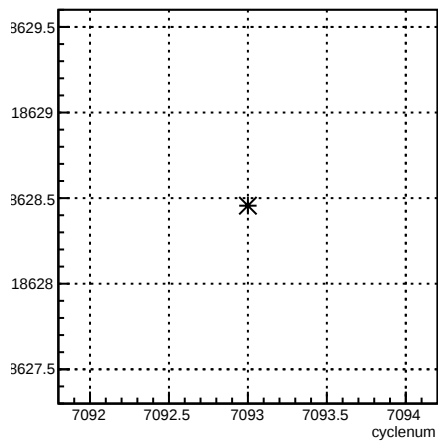
usr_coil7:cyclenum {run == 6818}
