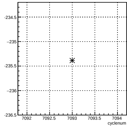
12X_coil6:cyclenum {run == 6818}
