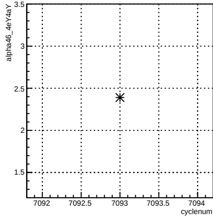
alpha46_4eY4aY:cyclenum {run == 6818}
