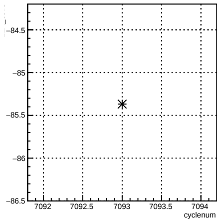
12X_coil7:cyclenum {run == 6818}
