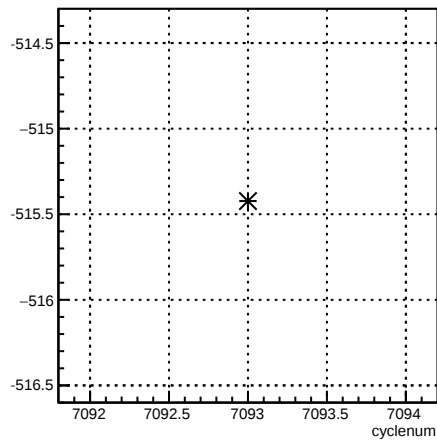
4eX_coil1:cyclenum {run == 6818}
