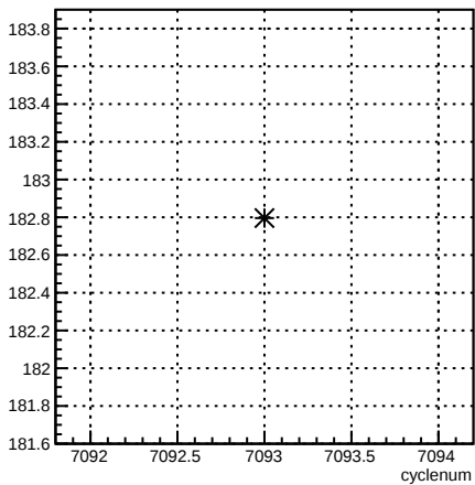
4eY_coil4:cyclenum {run == 6818}
