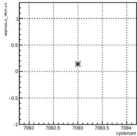
alpha13_4eX1X:cyclenum {run == 6818}
