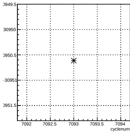
usr_coil1:cyclenum {run == 6818}
