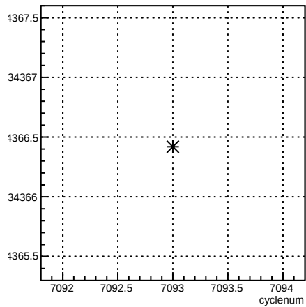
usl_coil6:cyclenum {run == 6818}
