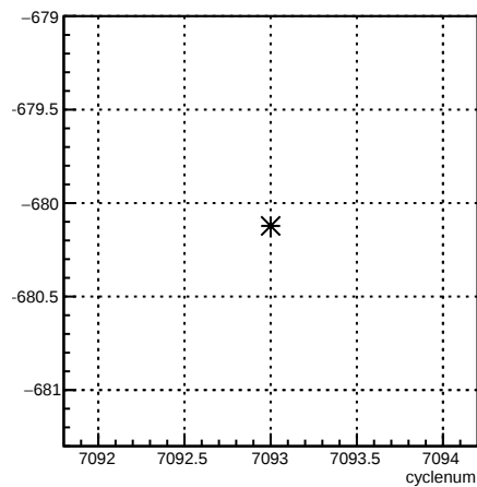
usr_coil6:cyclenum {run == 6818}
