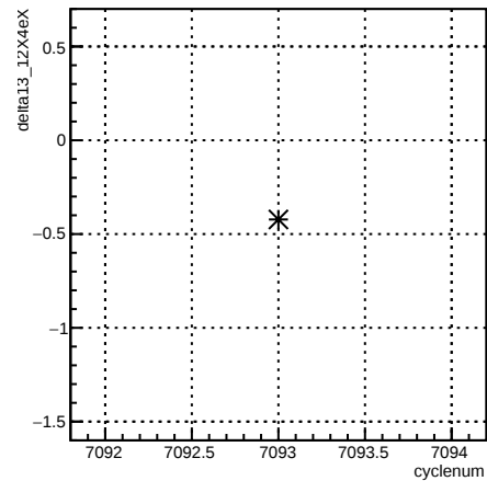
delta13_12X4eX:cyclenum {run == 6818}
