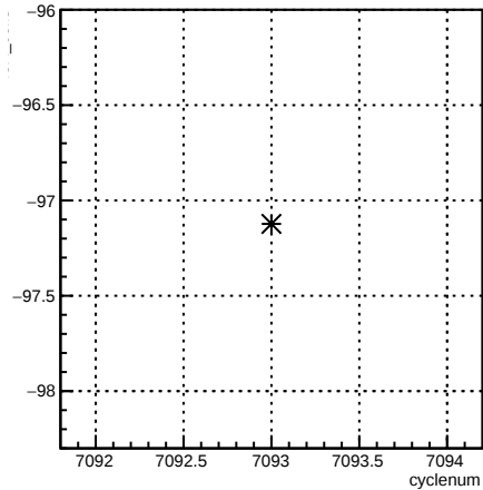
4eX_coil3:cyclenum {run == 6818}
