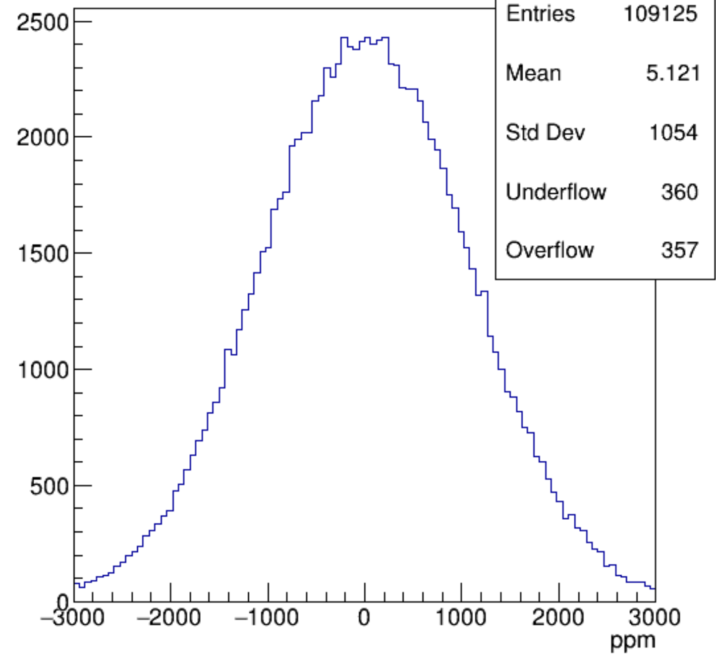
asym_sam3
