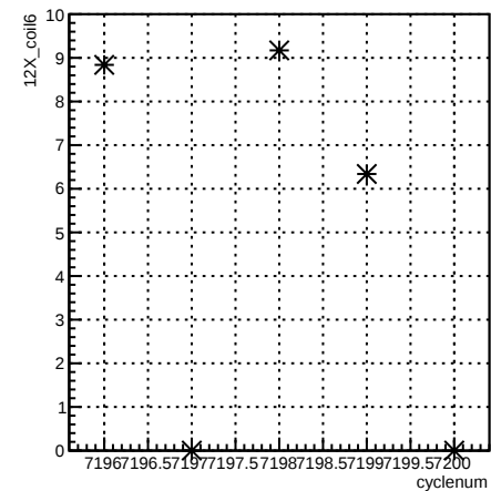
12X_coil6:cyclenum {run == 6867}
