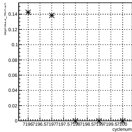
alpha13_4eX1X:cyclenum {run == 6867}
