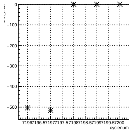
4eX_coil1:cyclenum {run == 6867}
