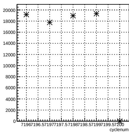
usr_coil7:cyclenum {run == 6867}
