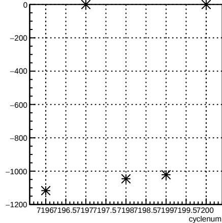
usl_coil6:cyclenum {run == 6867}
