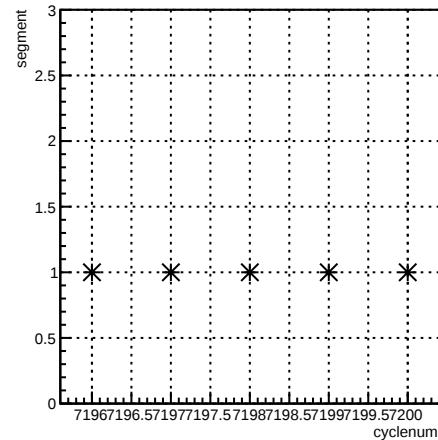
segment:cyclenum {run == 6867}
