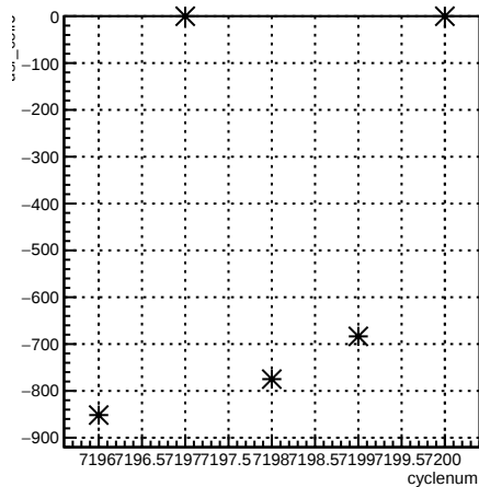
usr_coil6:cyclenum {run == 6867}
