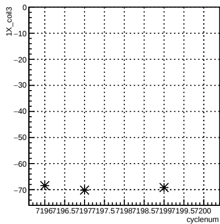
1X_coil3:cyclenum {run == 6867}
