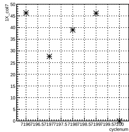
1X_coil7:cyclenum {run == 6867}
