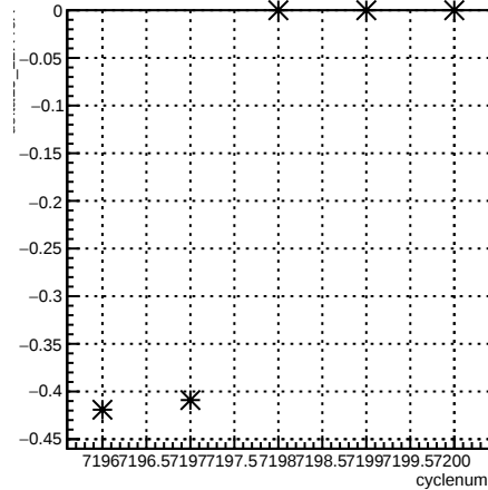
delta13_12X4eX:cyclenum {run == 6867}
