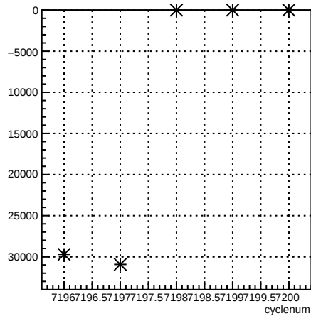
usr_coil1:cyclenum {run == 6867}
