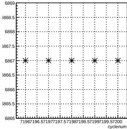
run:cyclenum {run == 6867}
