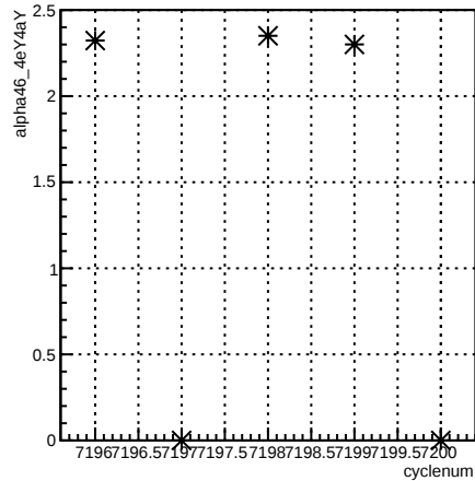
alpha46_4eY4aY:cyclenum {run == 6867}
