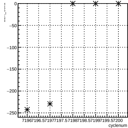
12X_coil1:cyclenum {run == 6867}
