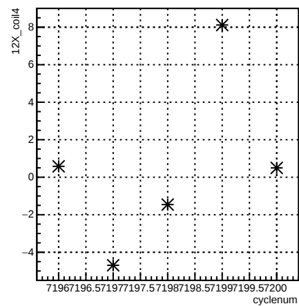
12X_coil4:cyclenum {run == 6867}
