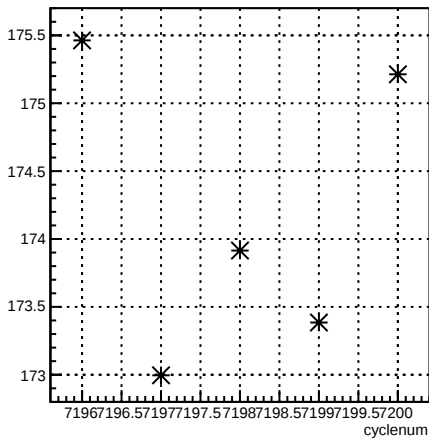
4eY_coil4:cyclenum {run == 6867}
