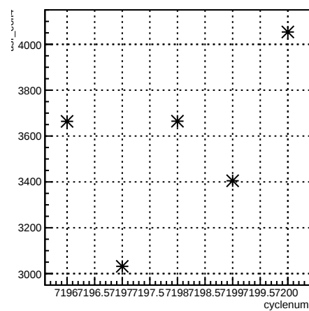
usr_coil4:cyclenum {run == 6867}
