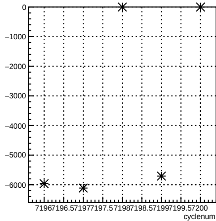
usr_coil3:cyclenum {run == 6867}
