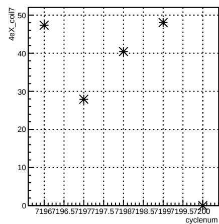
4eX_coil7:cyclenum {run == 6867}
