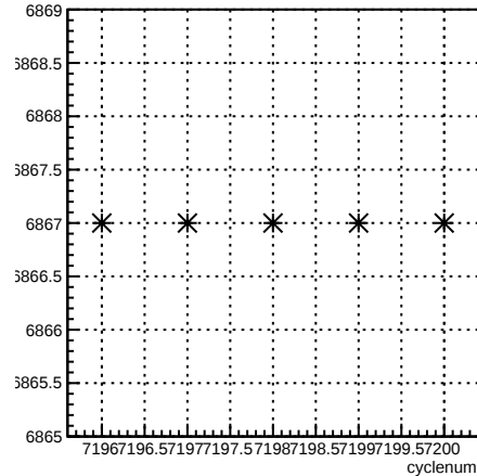
run:cyclenum {run == 6867}
