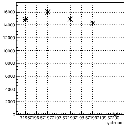
usl_coil7:cyclenum {run == 6867}
