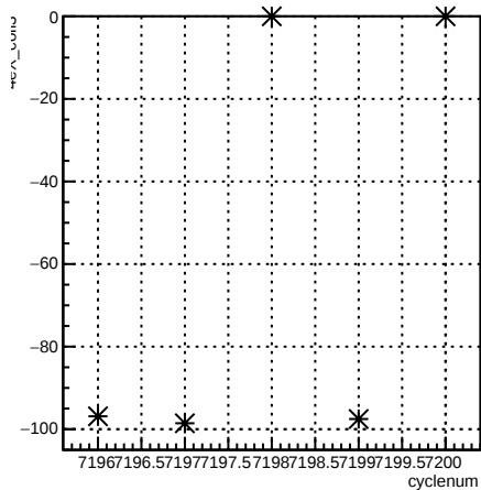
4eX_coil3:cyclenum {run == 6867}
