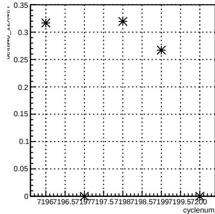
delta46_12X4eY:cyclenum {run == 6867}
