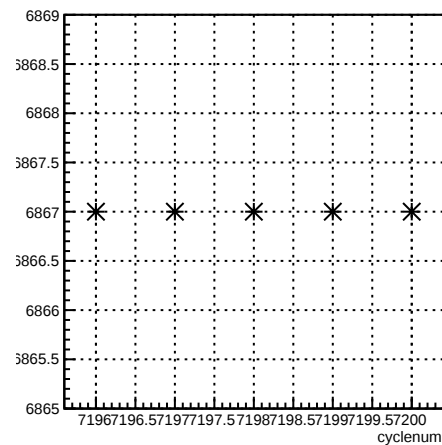
run:cyclenum {run == 6867}
