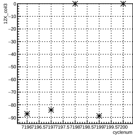
12X_coil3:cyclenum {run == 6867}
