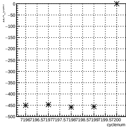
12X_coil7:cyclenum {run == 6867}
