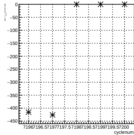
1X_coil1:cyclenum {run == 6867}
