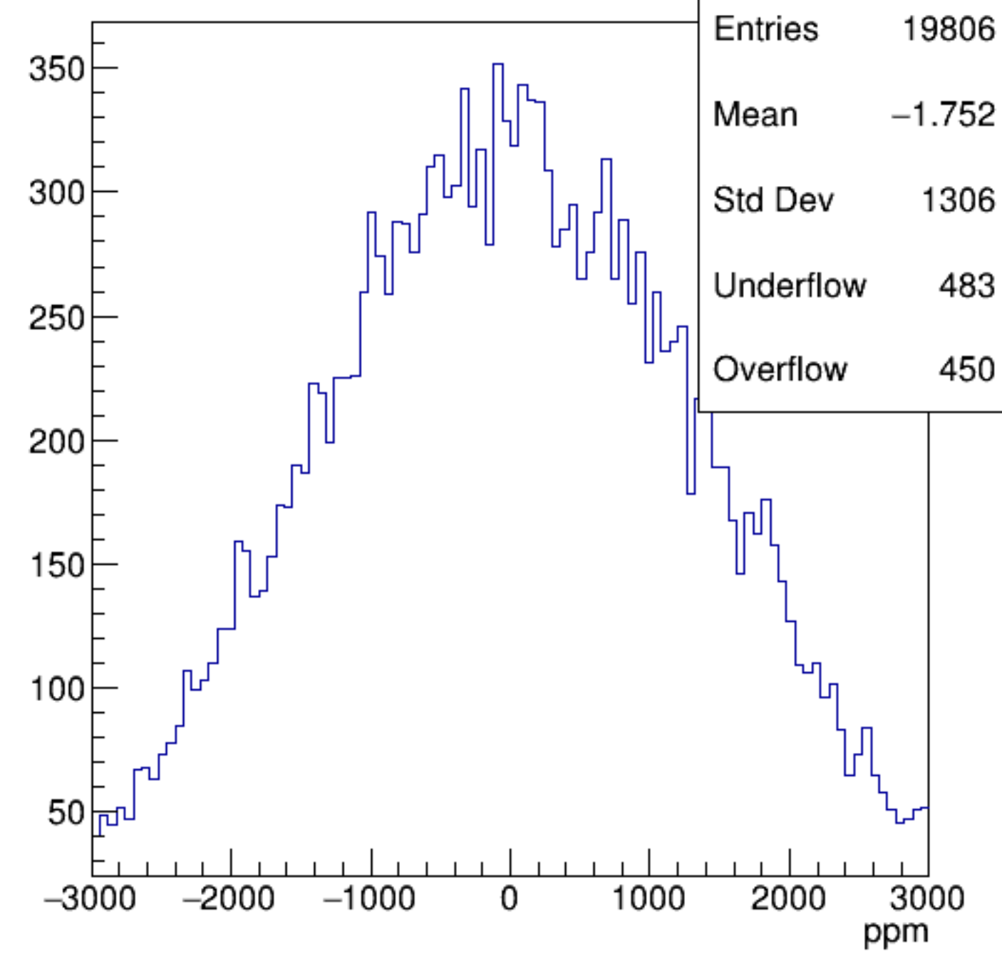
asym_sam6
