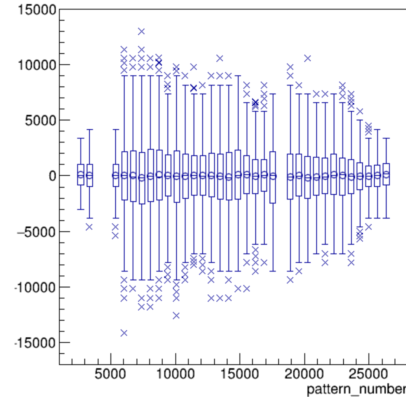
asym_sam5/ppm:pattern_number {ErrorFlag==0}
