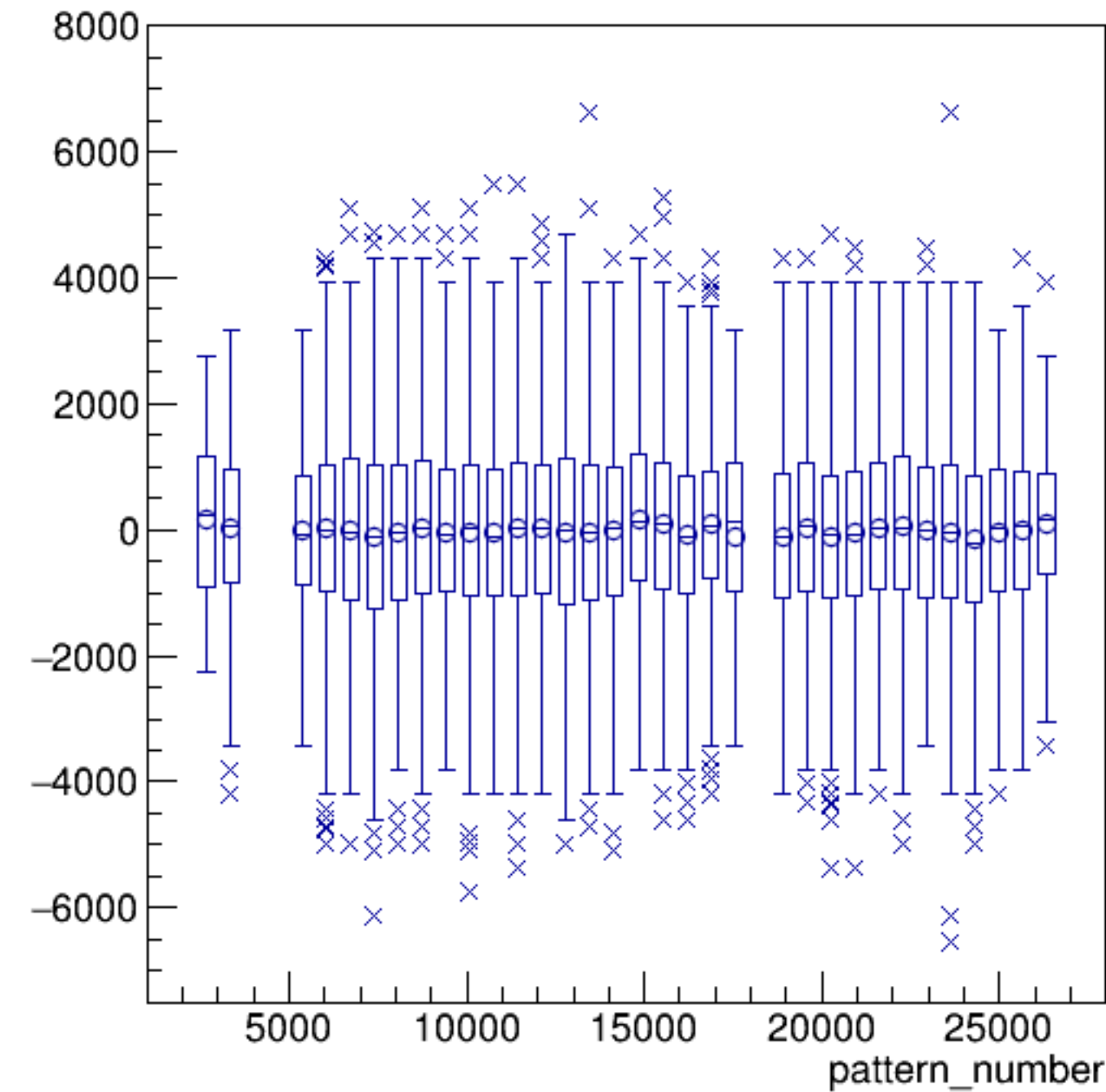
asym_sam6/ppm:pattern_number {ErrorFlag==0}
