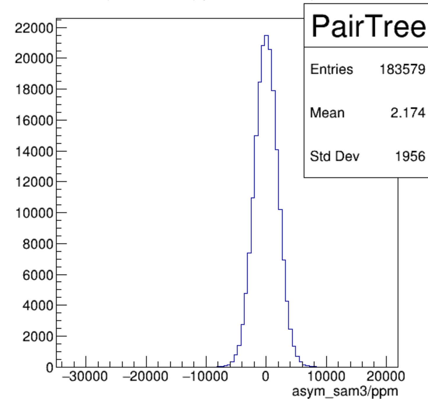
asym_sam3/ppm {ErrorFlag==0}
