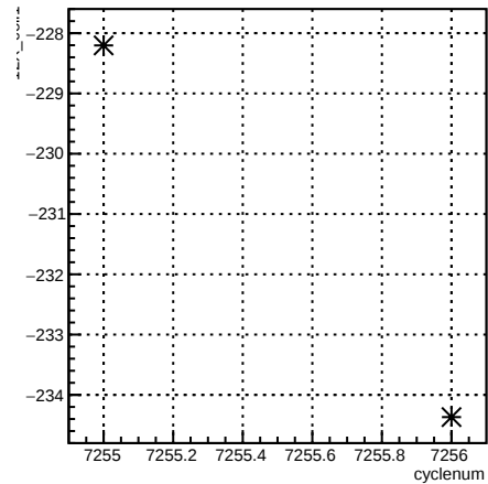
12X_coil6:cyclenum {run == 6893}
