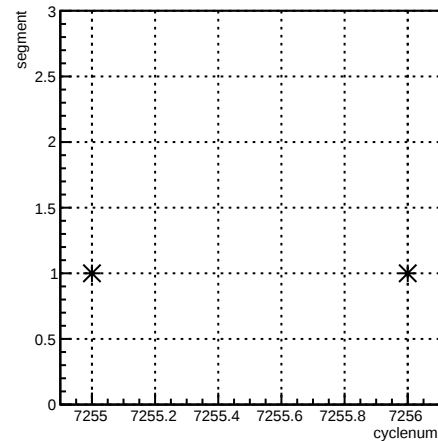
segment:cyclenum {run == 6893}
