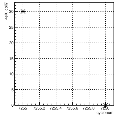
4eX_coil7:cyclenum {run == 6893}
