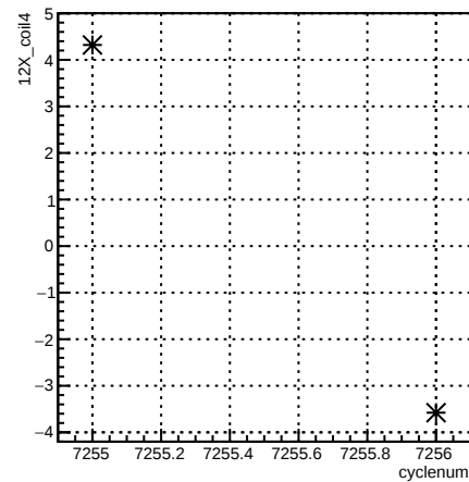
12X_coil4:cyclenum {run == 6893}
