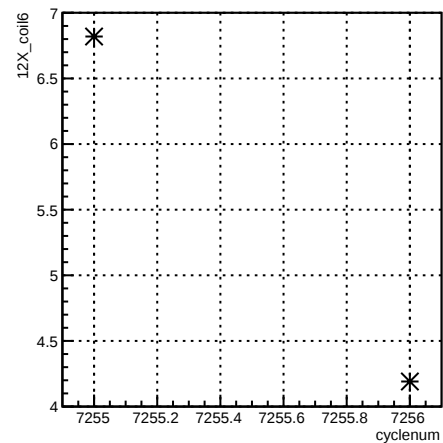
12X_coil6:cyclenum {run == 6893}
