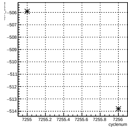
4eX_coil1:cyclenum {run == 6893}
