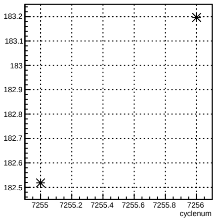
4eY_coil4:cyclenum {run == 6893}
