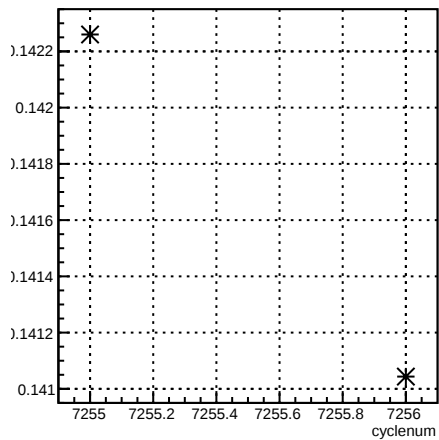
delta46_12X4eY:cyclenum {run == 6893}
