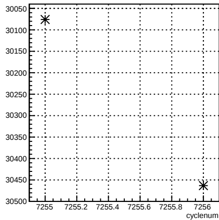
usr_coil6:cyclenum {run == 6893}
