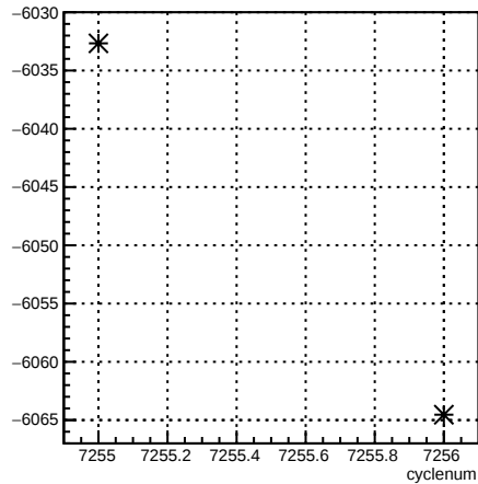
usr_coil3:cyclenum {run == 6893}
