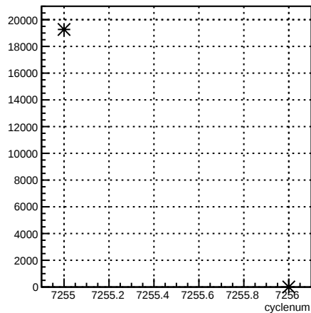
usr_coil7:cyclenum {run == 6893}
