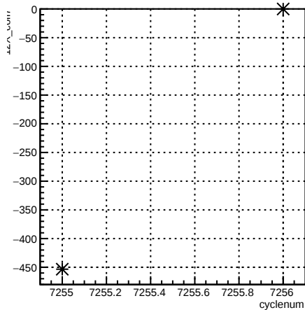
12X_coil7:cyclenum {run == 6893}
