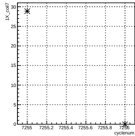
1X_coil7:cyclenum {run == 6893}
