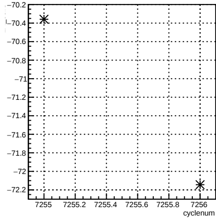
1X_coil3:cyclenum {run == 6893}
