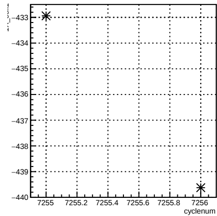
1X_coil1:cyclenum {run == 6893}
