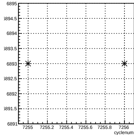
run:cyclenum {run == 6893}
