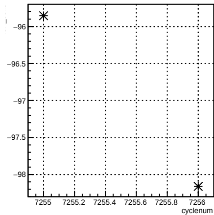
4eX_coil3:cyclenum {run == 6893}
