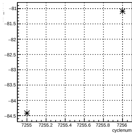
12X_coil7:cyclenum {run == 6893}
