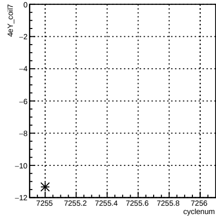
4eY_coil7:cyclenum {run == 6893}
