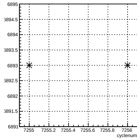
run:cyclenum {run == 6893}
