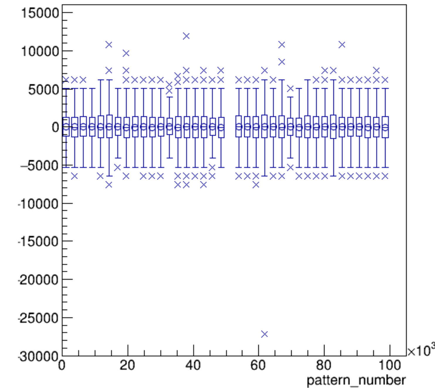
asym_sam6/ppm:pattern_number {ErrorFlag==0}
