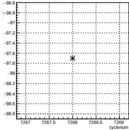
4eX_coil3:cyclenum {run == 6909}
