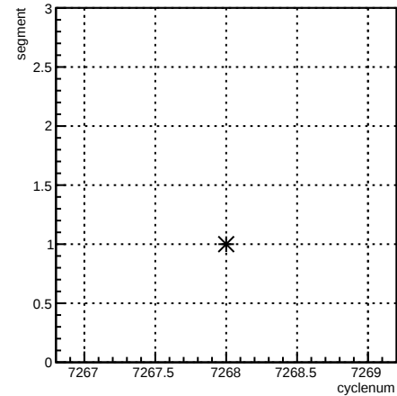
segment:cyclenum {run == 6909}
