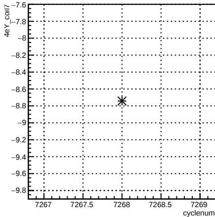
4eY_coil7:cyclenum {run == 6909}
