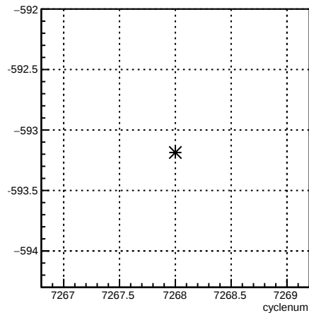
usr_coil6:cyclenum {run == 6909}
