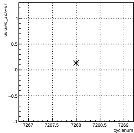
delta46_12X4eY:cyclenum {run == 6909}
