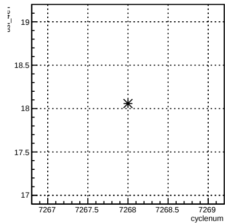
usl_4eY:cyclenum {run == 6909}
