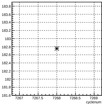
4eY_coil4:cyclenum {run == 6909}
