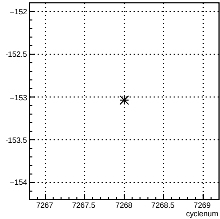
usr_4eY:cyclenum {run == 6909}
