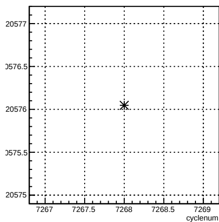
usr_coil7:cyclenum {run == 6909}
