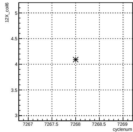
12X_coil6:cyclenum {run == 6909}
