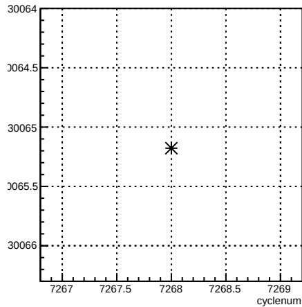
usr_coil1:cyclenum {run == 6909}
