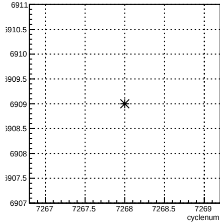
run:cyclenum {run == 6909}
