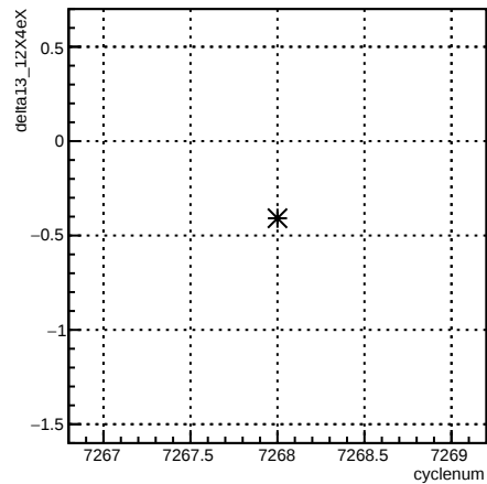
delta13_12X4eX:cyclenum {run == 6909}
