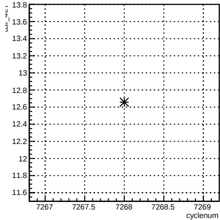
usr_4eY:cyclenum {run == 6909}
