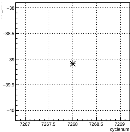
usr_12X:cyclenum {run == 6909}
