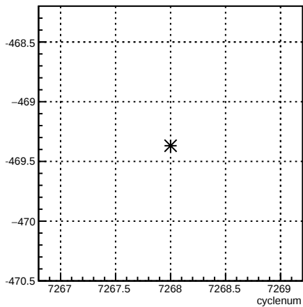
12X_coil7:cyclenum {run == 6909}
