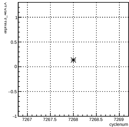
alpha13_4eX1X:cyclenum {run == 6909}
