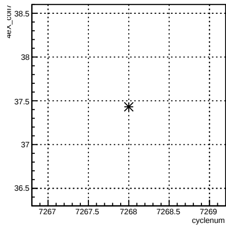
4eX_coil7:cyclenum {run == 6909}
