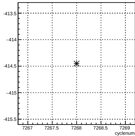
4eX_coil1:cyclenum {run == 6909}
