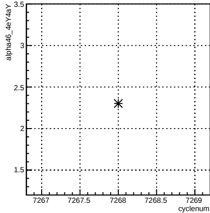
alpha46_4eY4aY:cyclenum {run == 6909}
