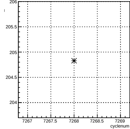
run:cyclenum {run == 6909}
