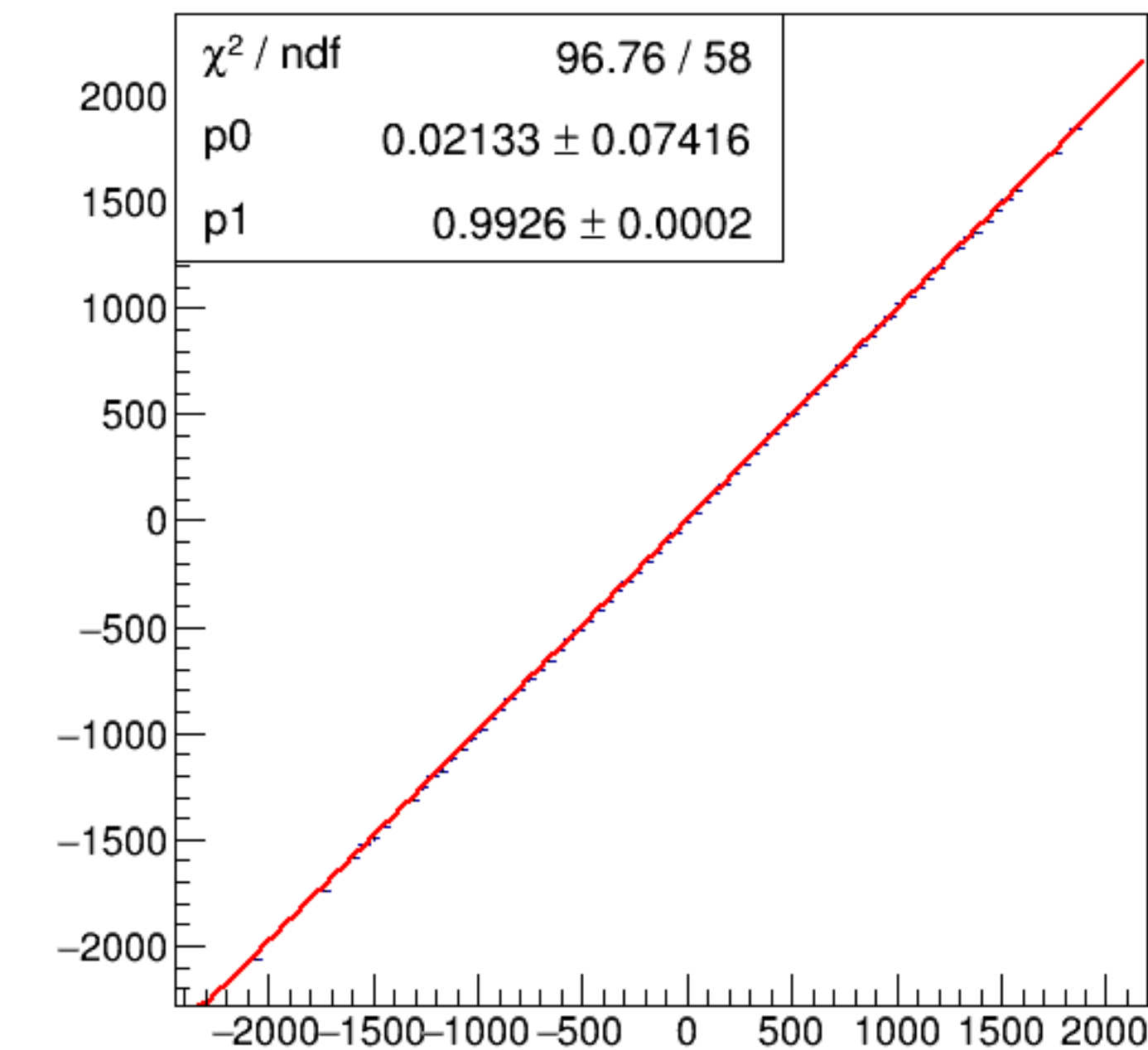
run6910_000_asym_bcm_an_ds_vs_asym_bcm_an_ds3_mul.png
