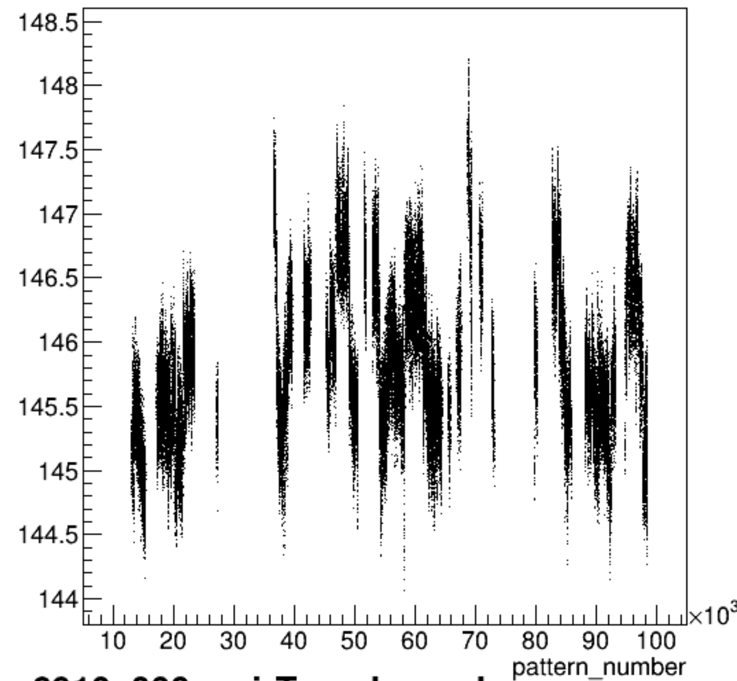
yield_bcm_dg_us:pattern_number {ErrorFlag==0}
