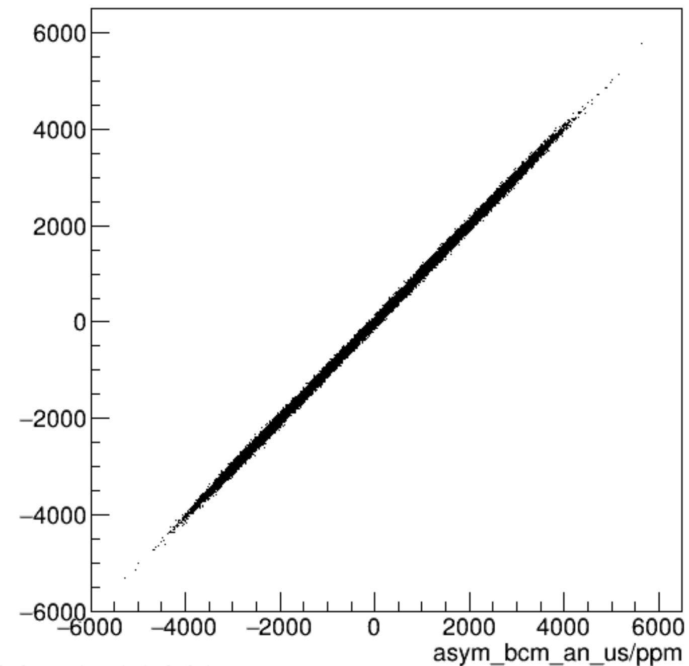
run6910_000_asym_bcm_dg_ds_vs_asym_bcm_an_us_pr.png
