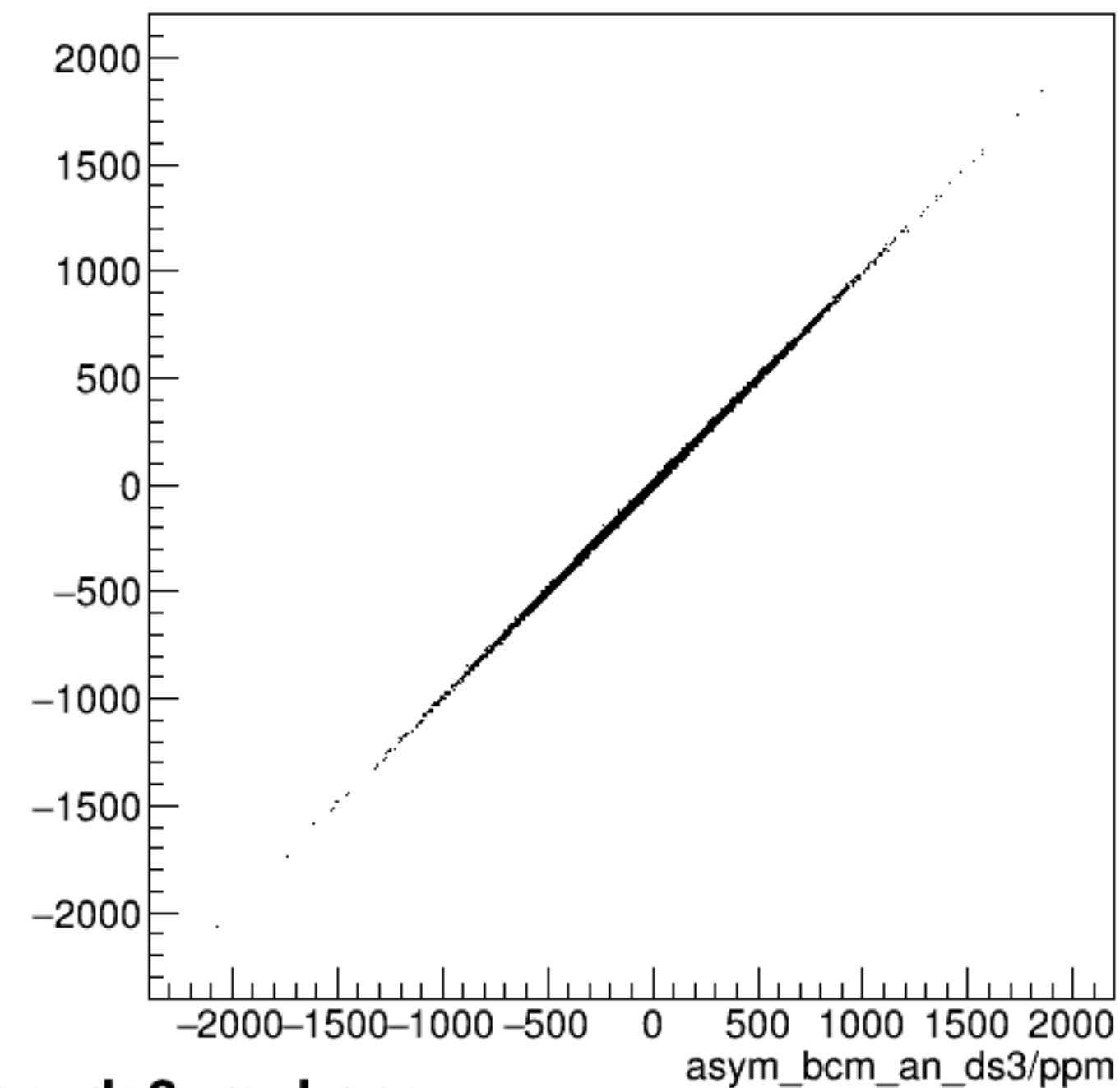
run6910_000_asym_bcm_an_ds_vs_asym_bcm_an_ds3_mul.png
