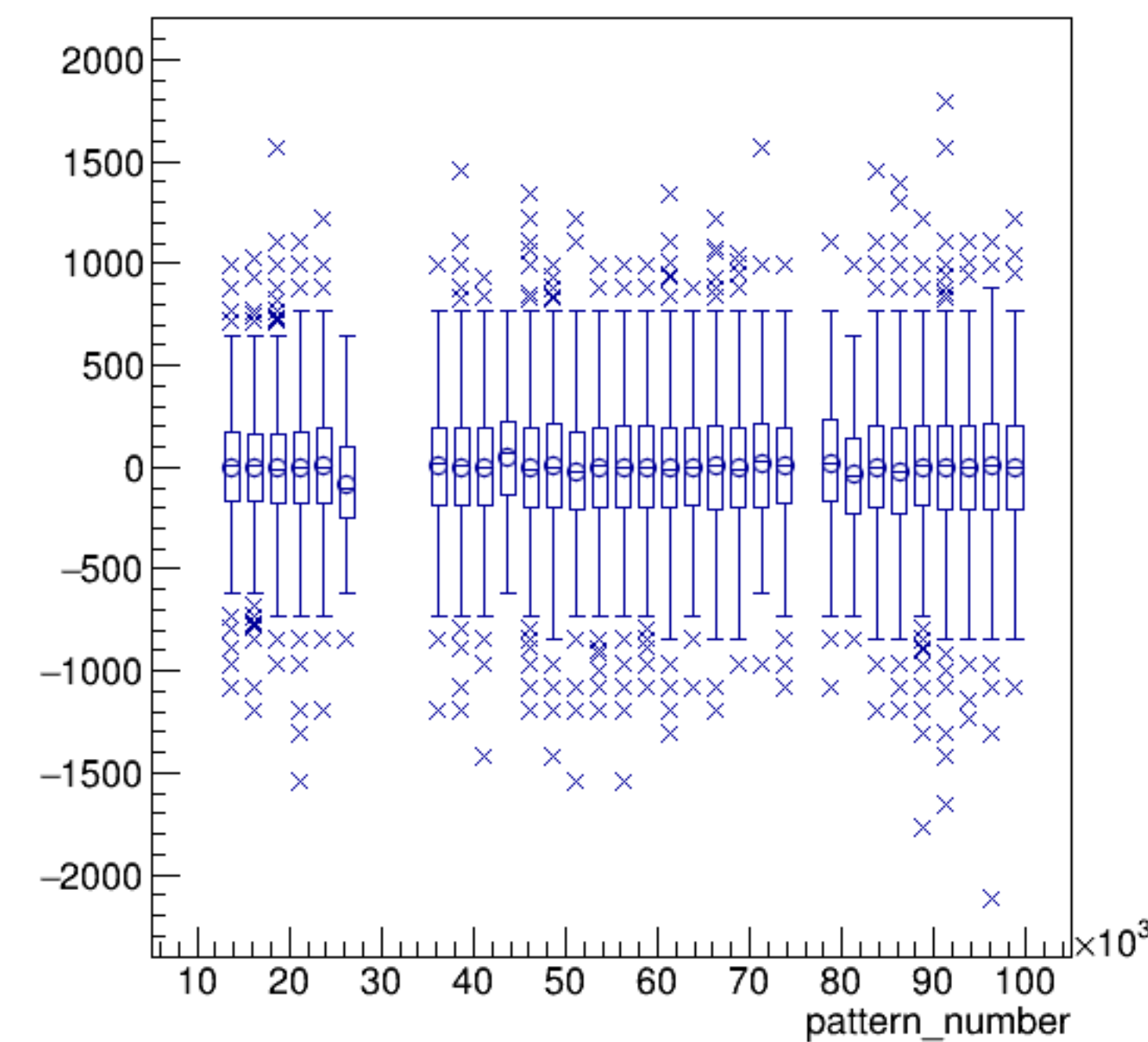
asym_bcm_an_us/ppm:pattern_number {ErrorFlag==0}
