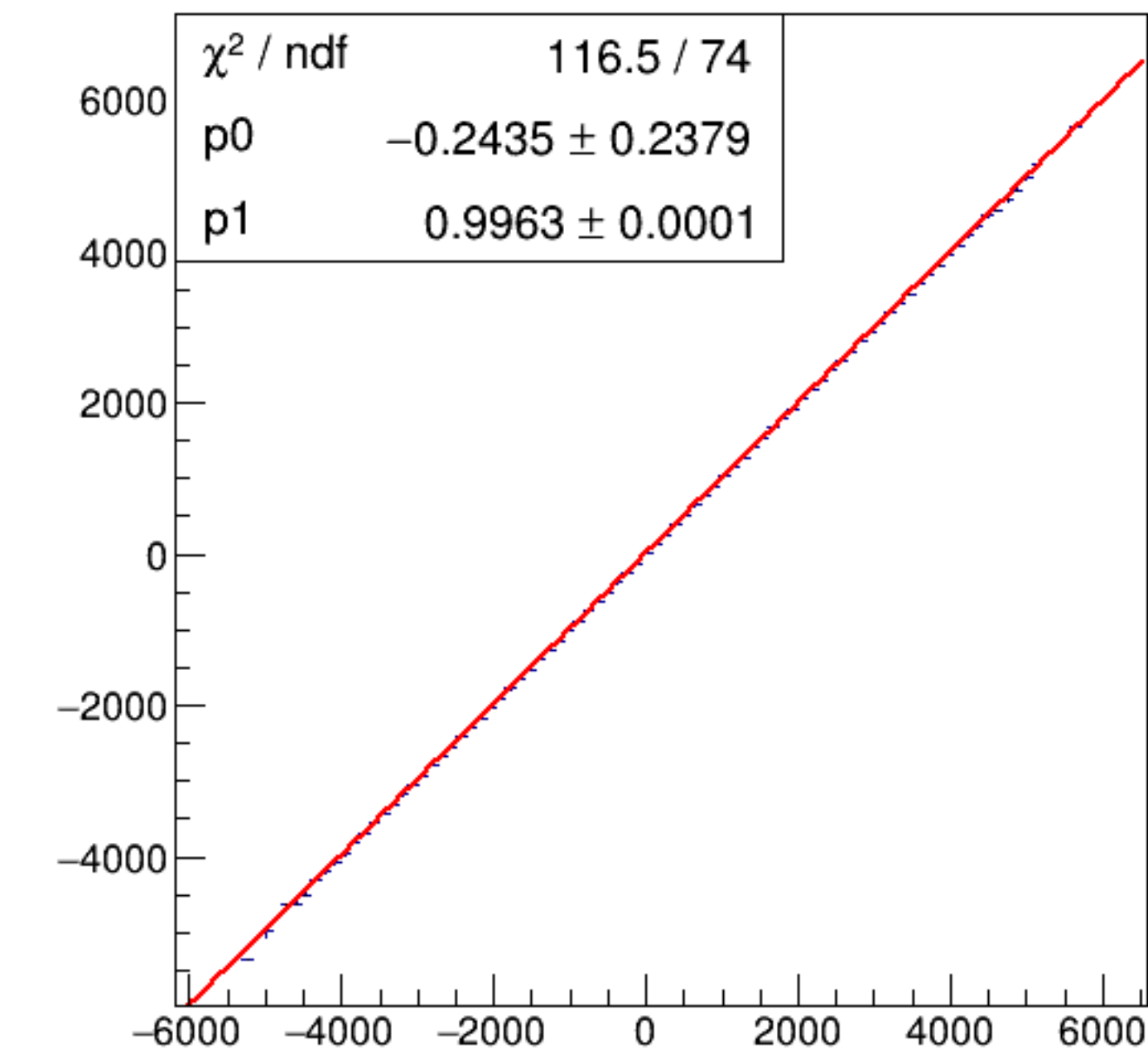
run6910_000_asym_bcm_dg_us_vs_asym_bcm_an_ds3_pr.png
