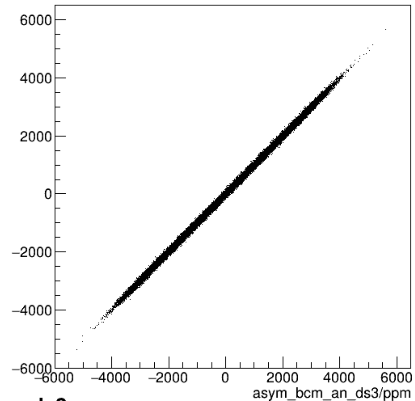
run6910_000_asym_bcm_dg_us_vs_asym_bcm_an_ds3_pr.png
