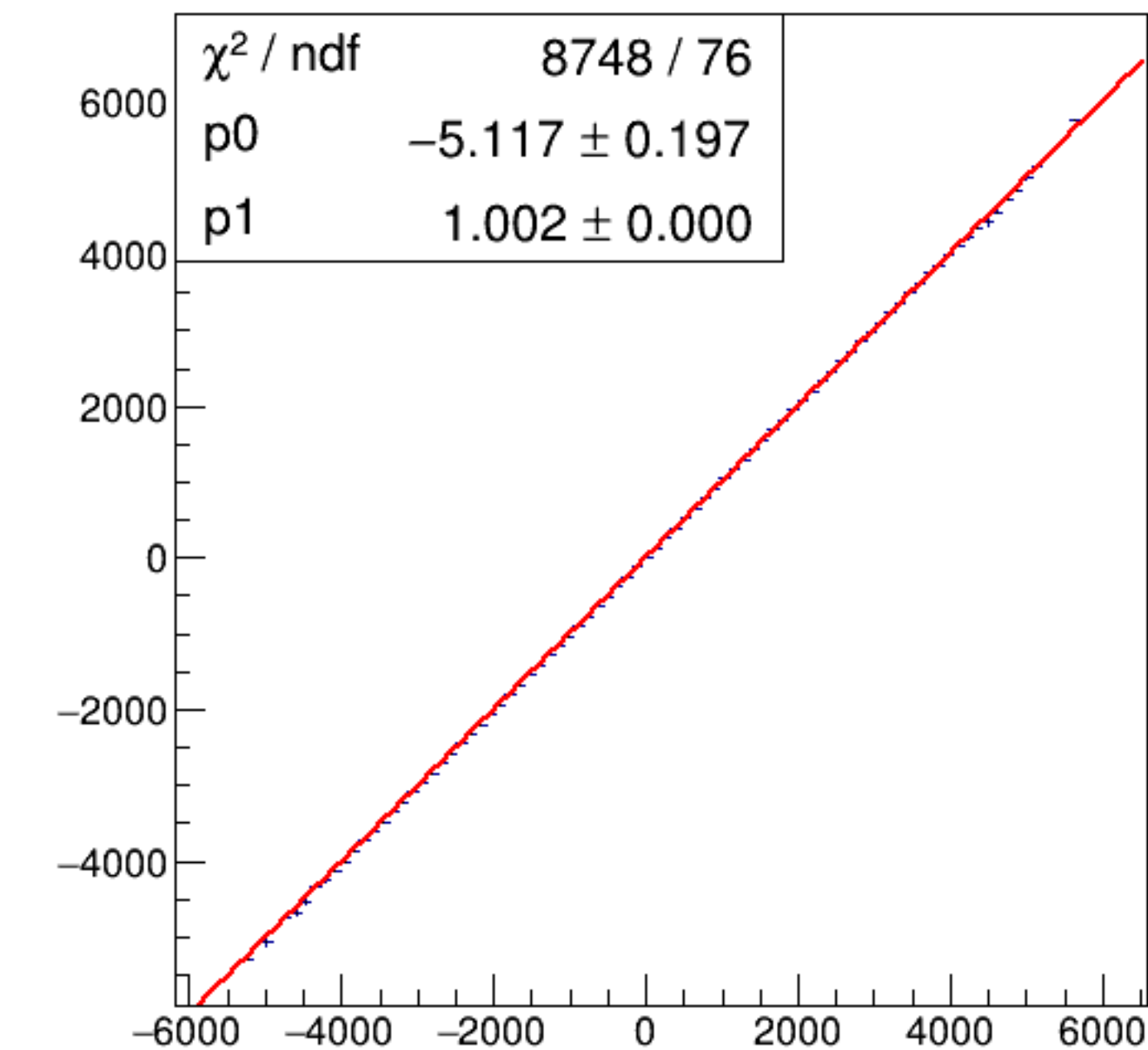
run6910_000_asym_bcm_dg_ds_vs_asym_bcm_an_us_pr.png
