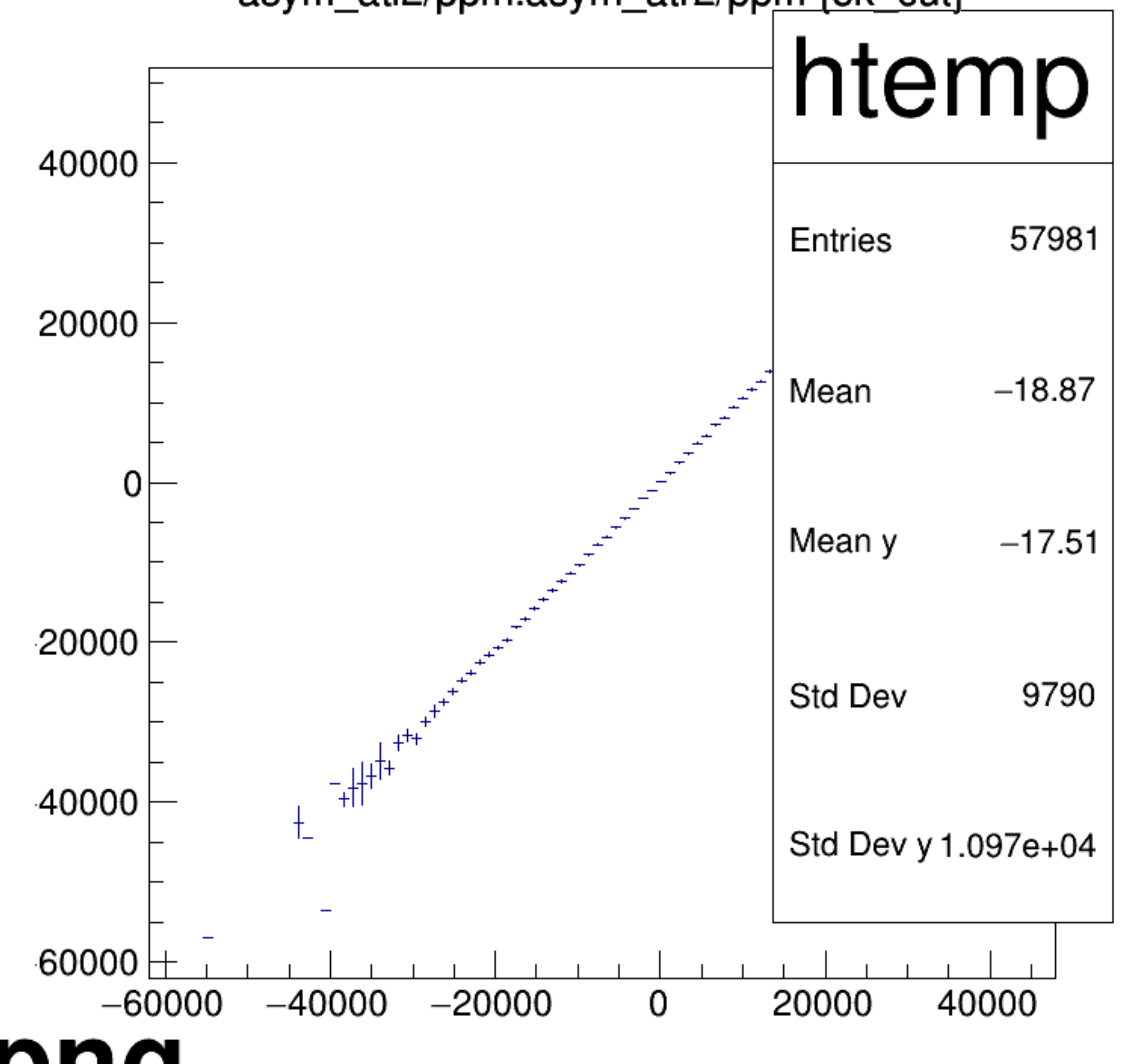
asym_atl2/ppm:asym_atr2/ppm {ok_cut}
