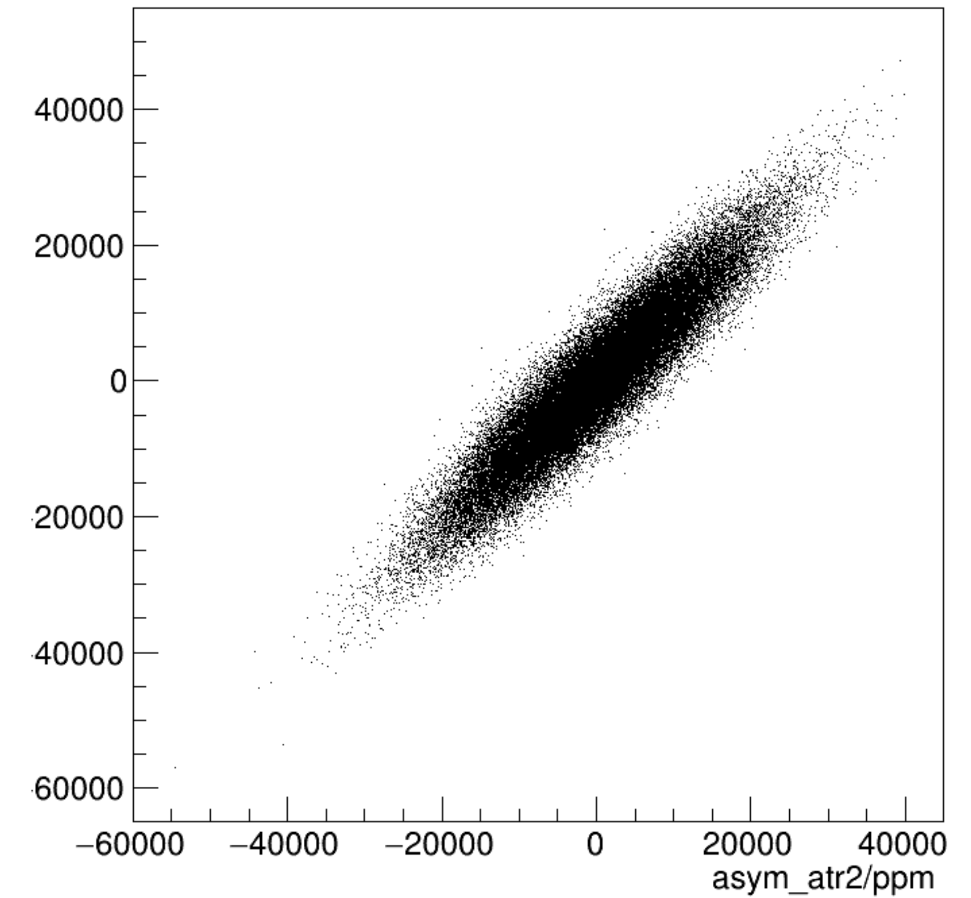
asym_atl2/ppm:asym_atr2/ppm {ok_cut}
