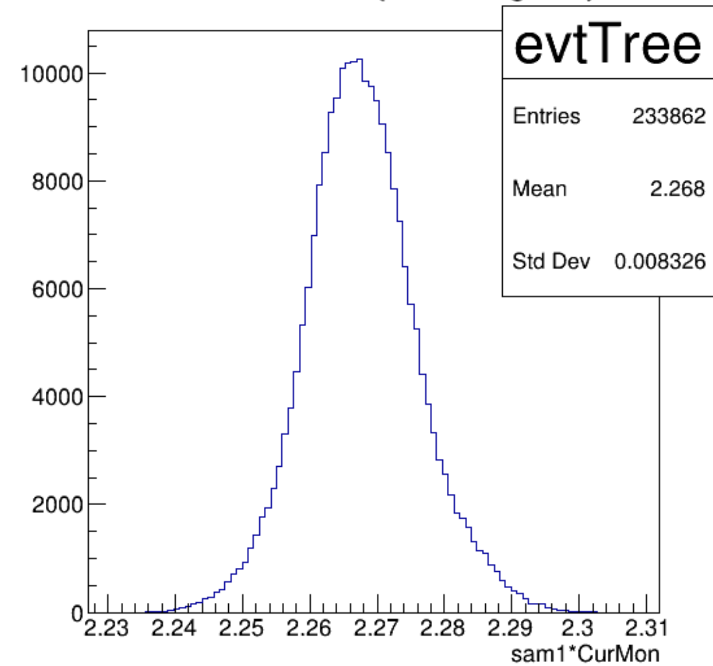
sam1*CurMon {ErrorFlag==0}
