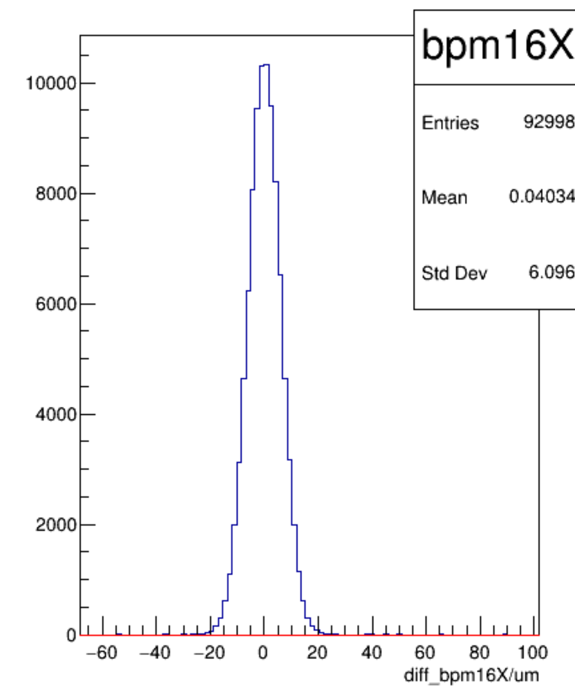
diff_bpm16X/um {ErrorFlag==0}
