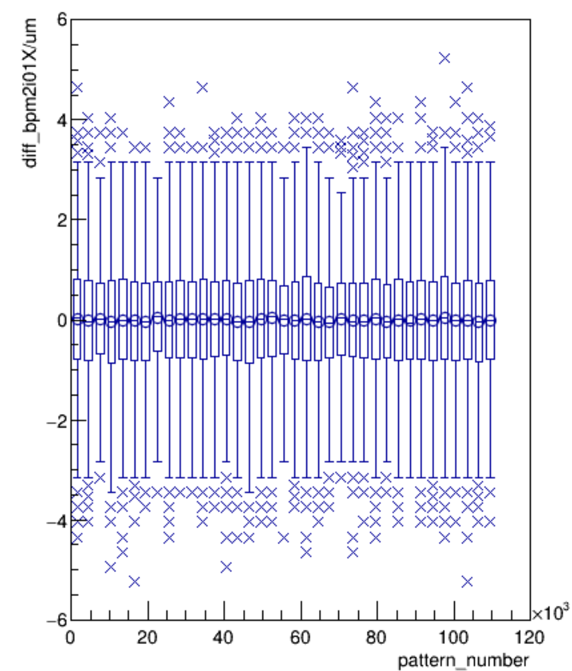
diff_bpm2i01X/um:pattern_number (ErrorFlag==0)
