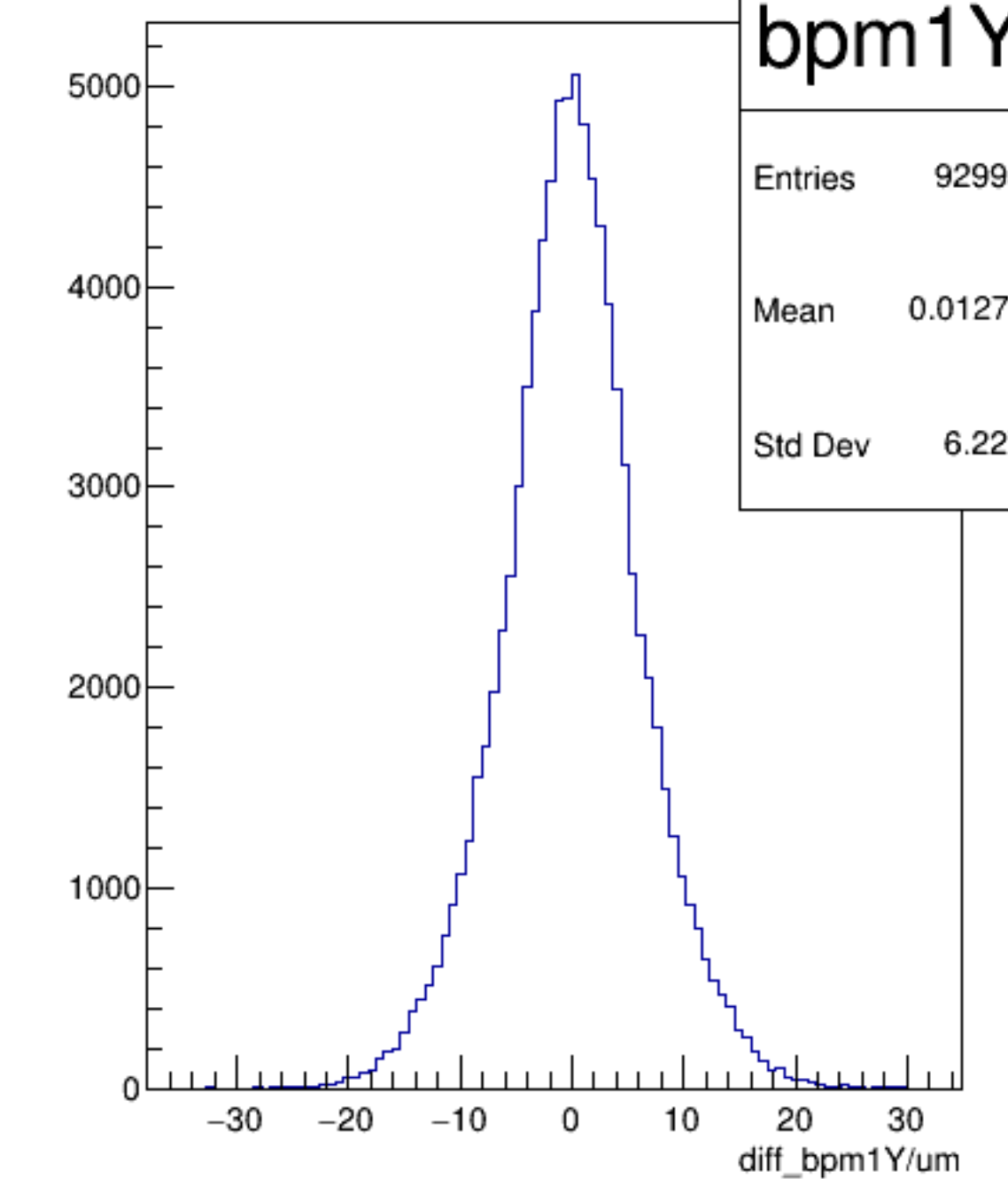
diff_bpm1Y/um {ErrorFlag==0}
