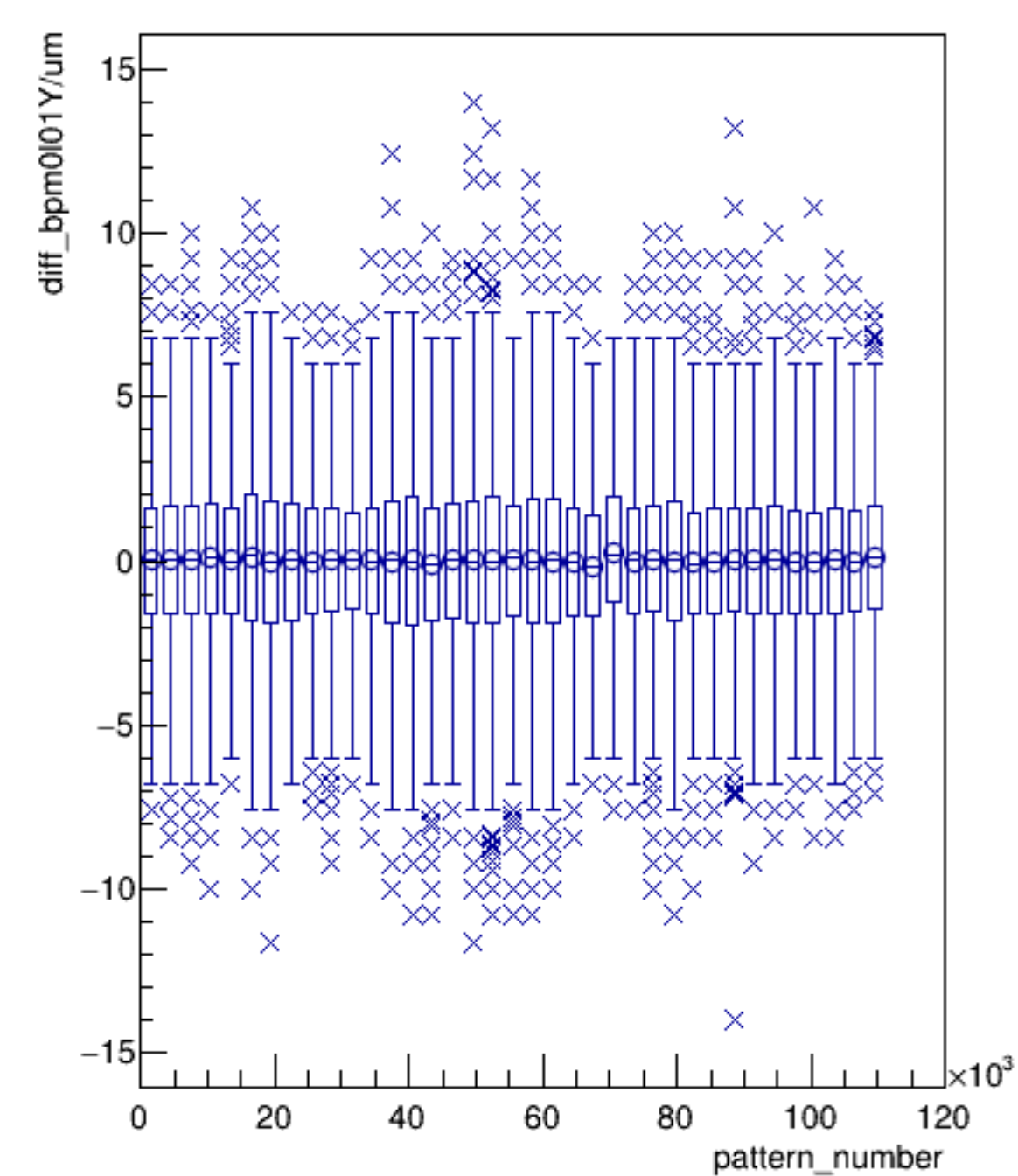
diff_bpm0I01Y/um:pattern_number (ErrorFlag==0)
