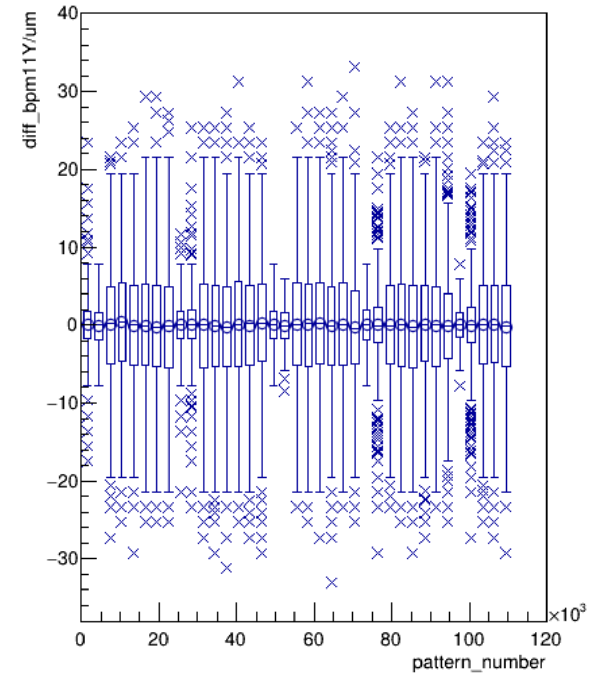
diff_bpm11Y/um:pattern_number {ErrorFlag==0}
