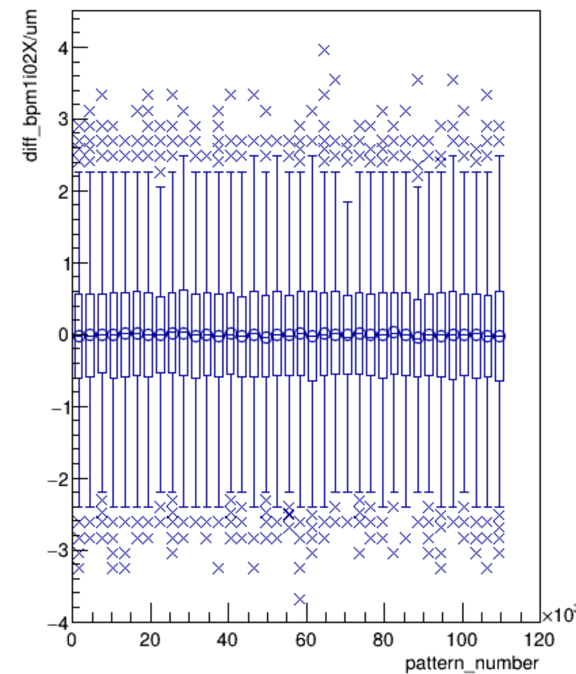
diff_bpm1i02X/um:pattern_number (ErrorFlag==0)
