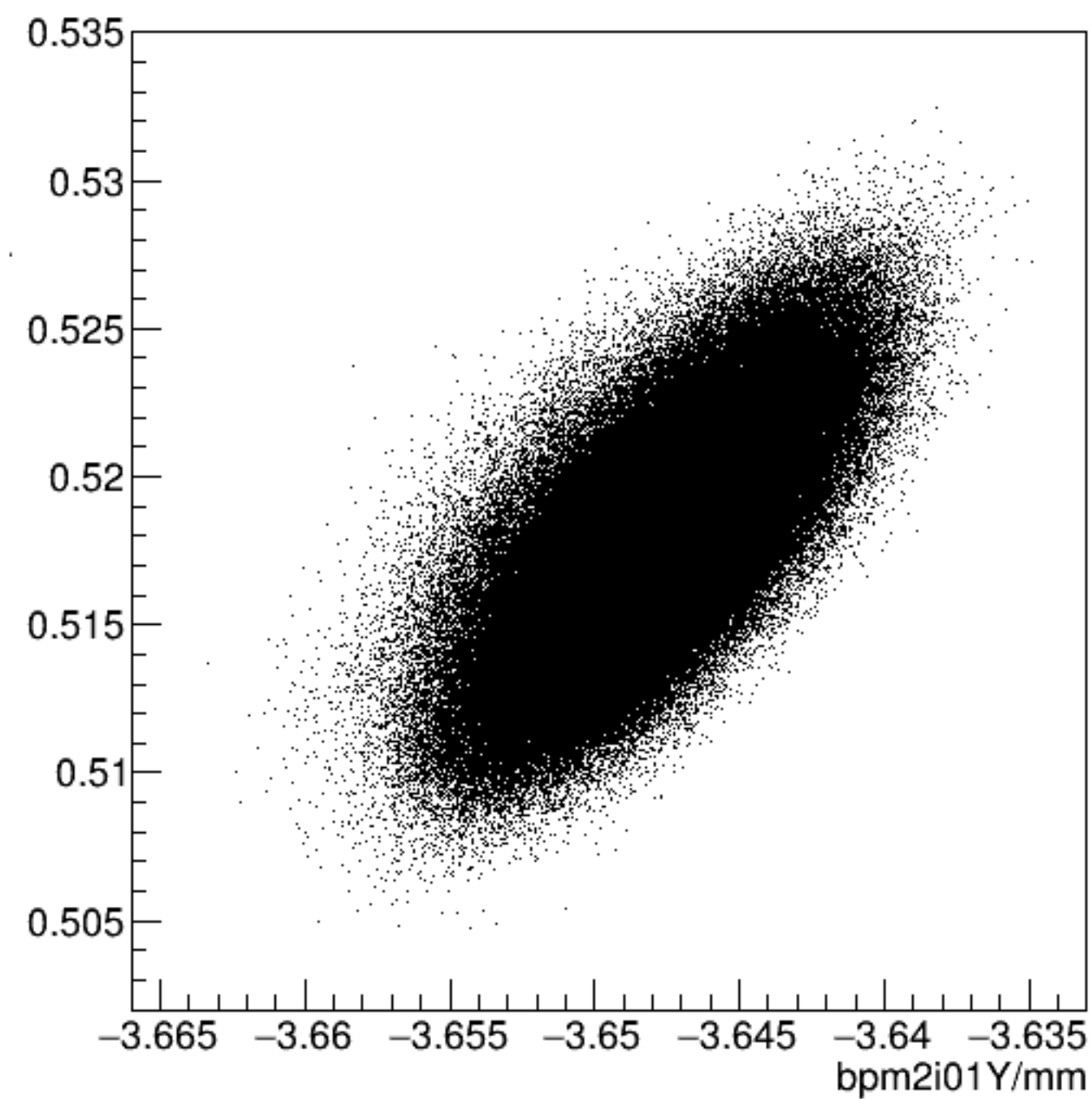
bpm2i01X/mm:bpm2i01Y/mm {ErrorFlag==0}
