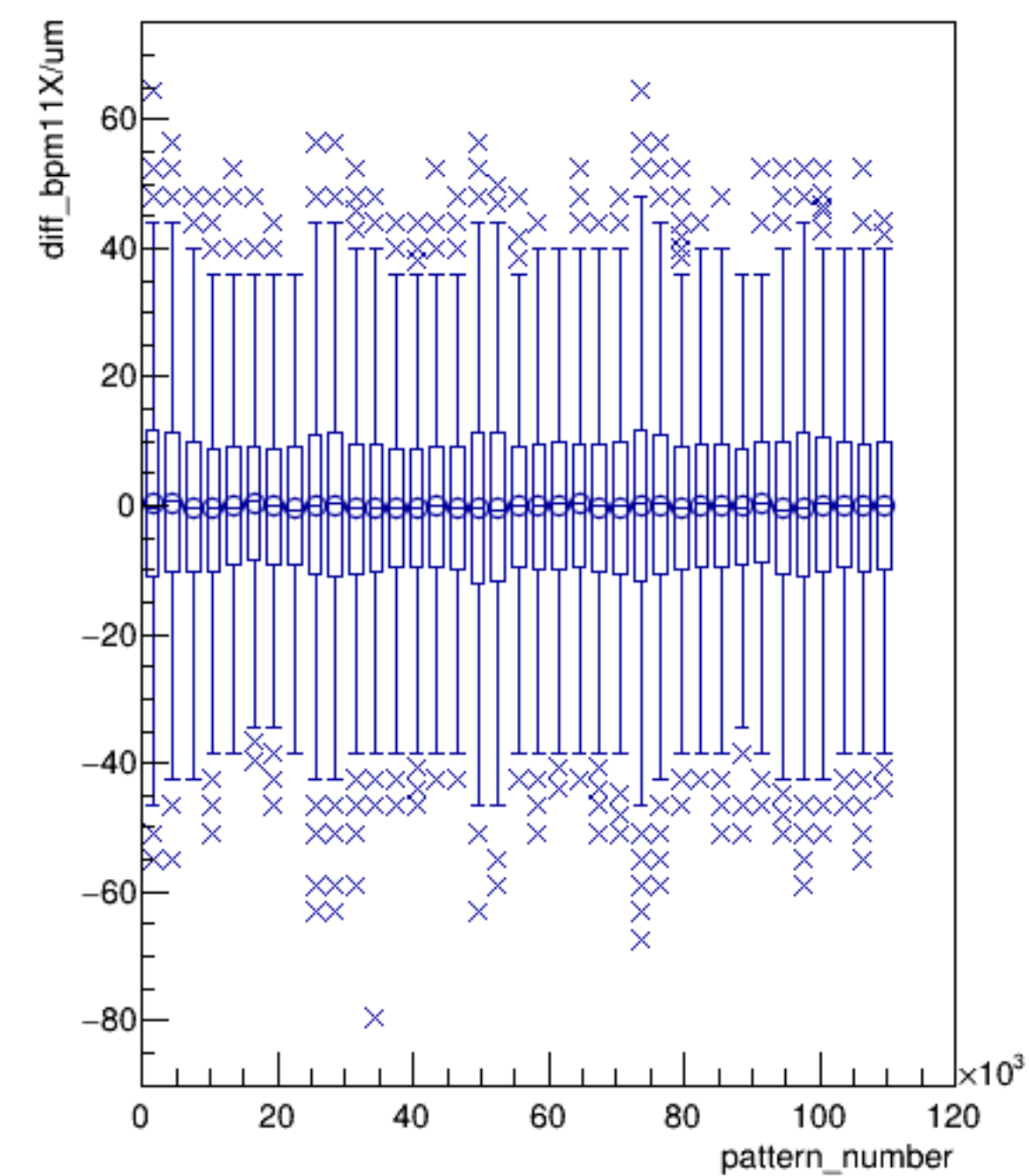
diff_bpm11X/um:pattern_number {ErrorFlag==0}
