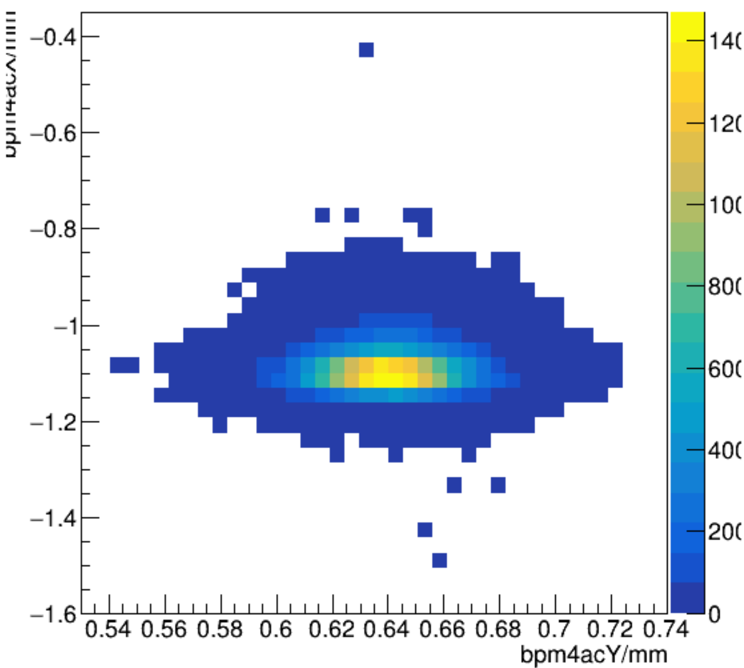
bpm4acX/mm:bpm4acY/mm {ErrorFlag==0}
