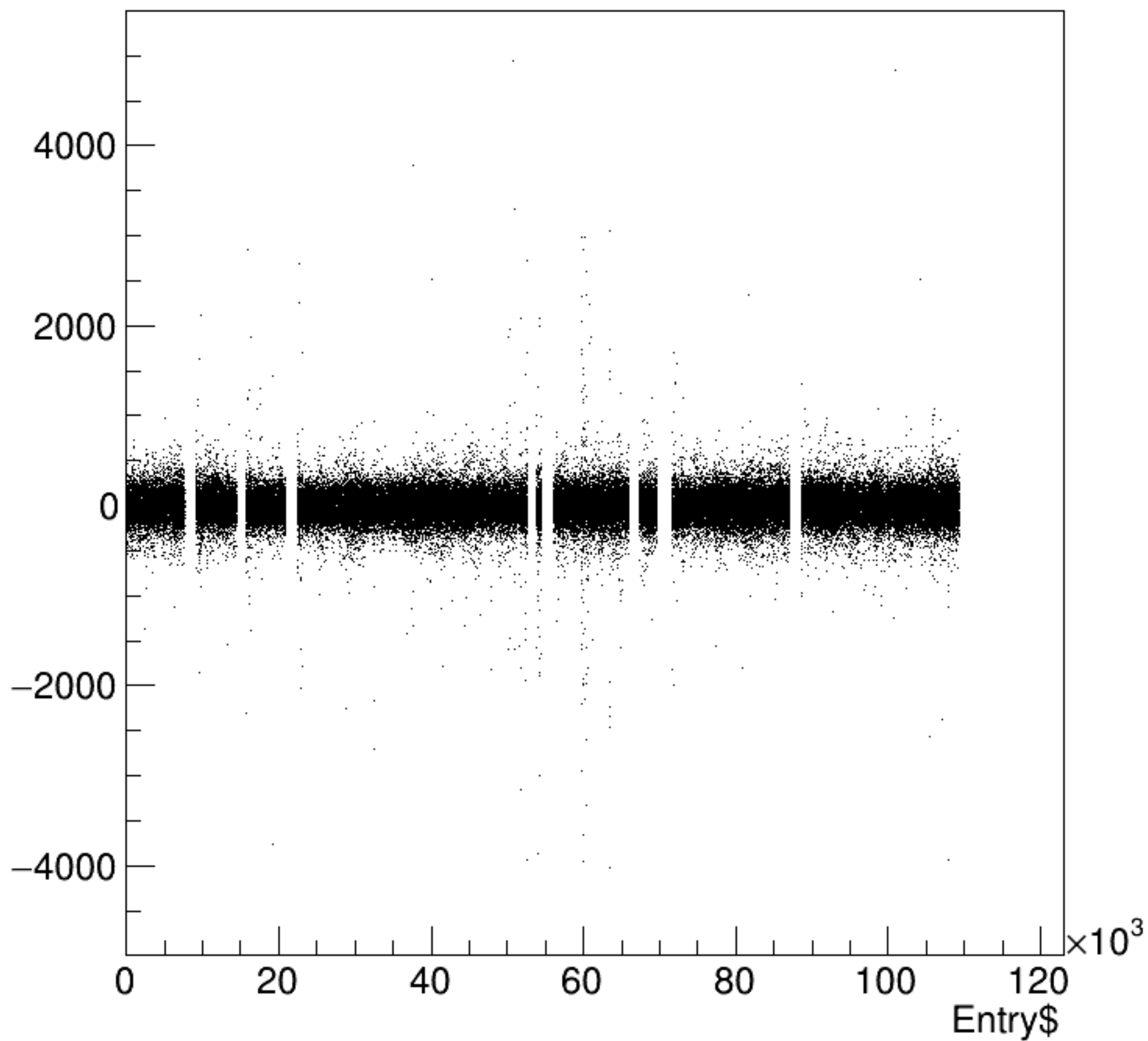
asym_bpm0l01WS/ppm:Entry$ {ErrorFlag==0}
