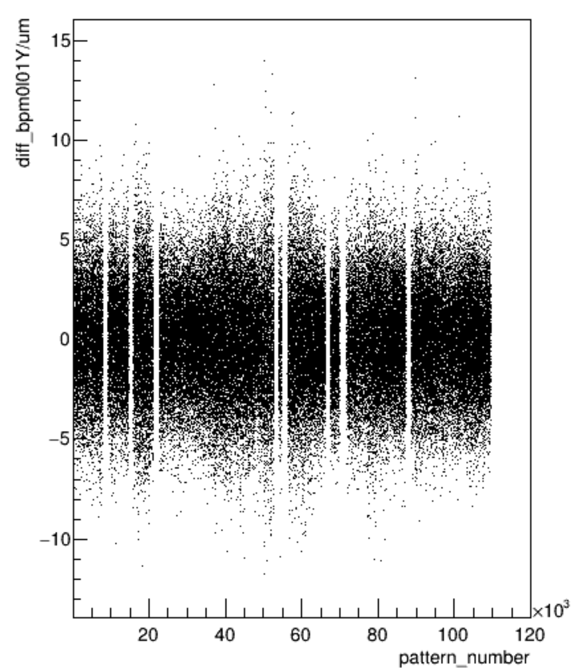
diff_bpm0I01Y/um:pattern_number (ErrorFlag==0)
