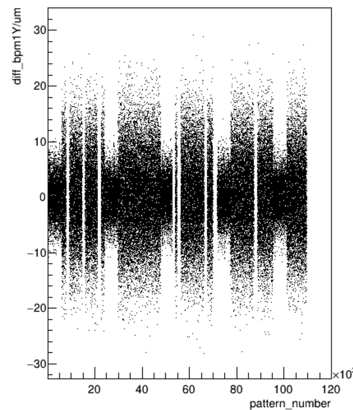
diff_bpm1Y/um:pattern_number {ErrorFlag==0}
