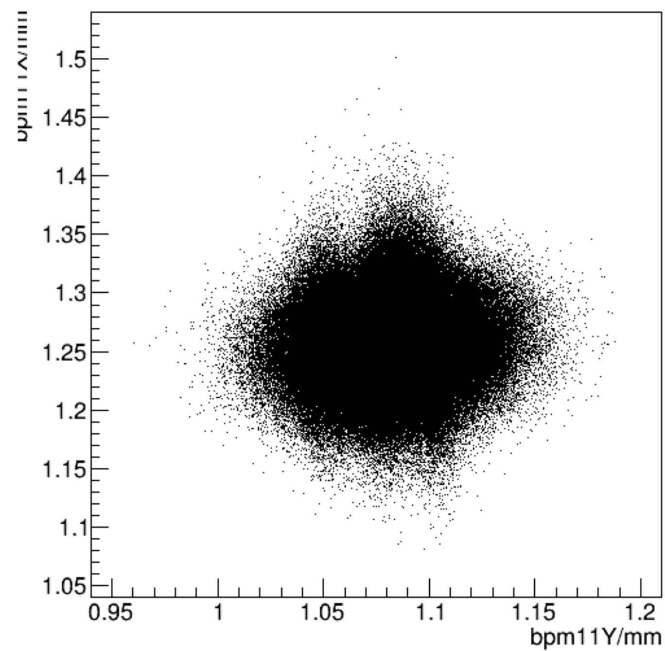
bpm11X/mm:bpm11Y/mm {ErrorFlag==0}
