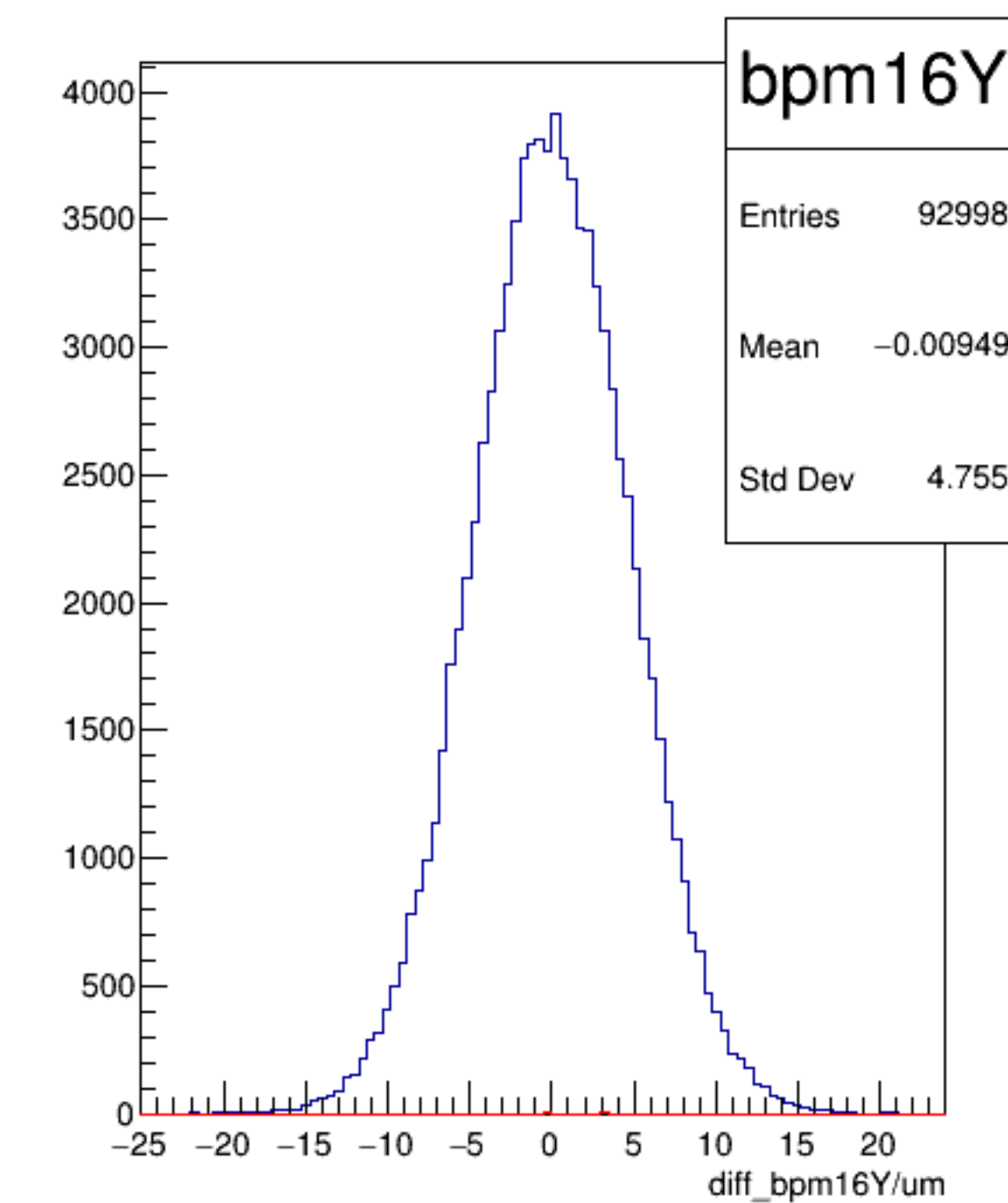
diff_bpm16Y/um {ErrorFlag==0}
