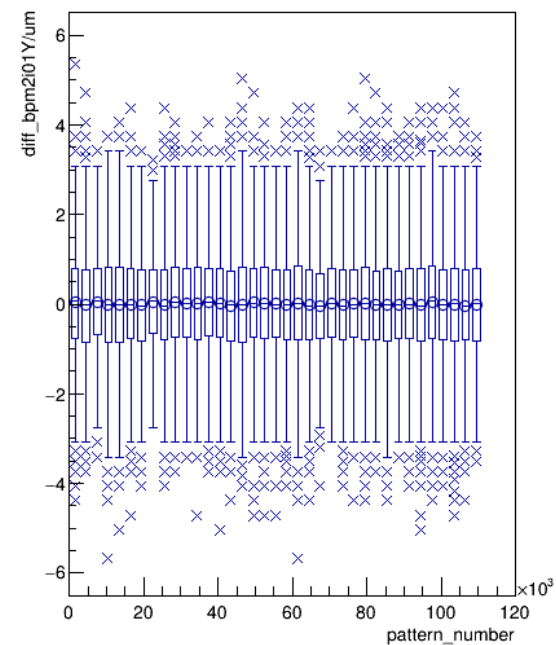
diff_bpm2i01Y/um:pattern_number (ErrorFlag==0)
