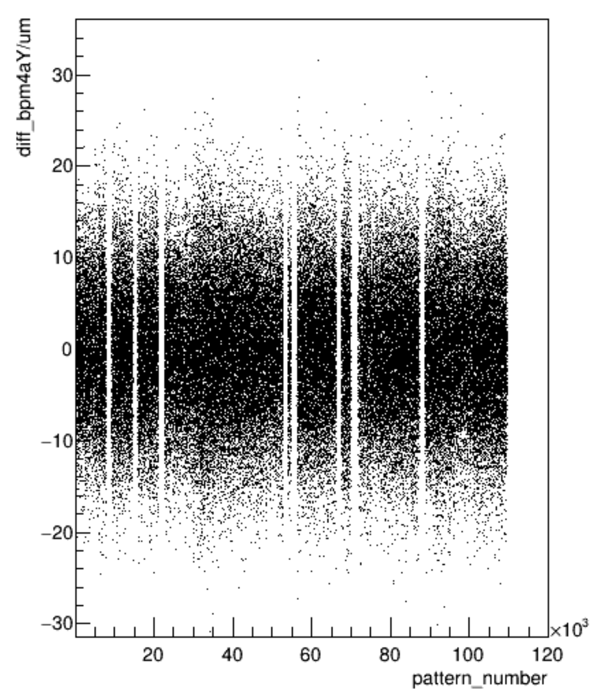
diff_bpm4aY/um:pattern_number {ErrorFlag==0}
