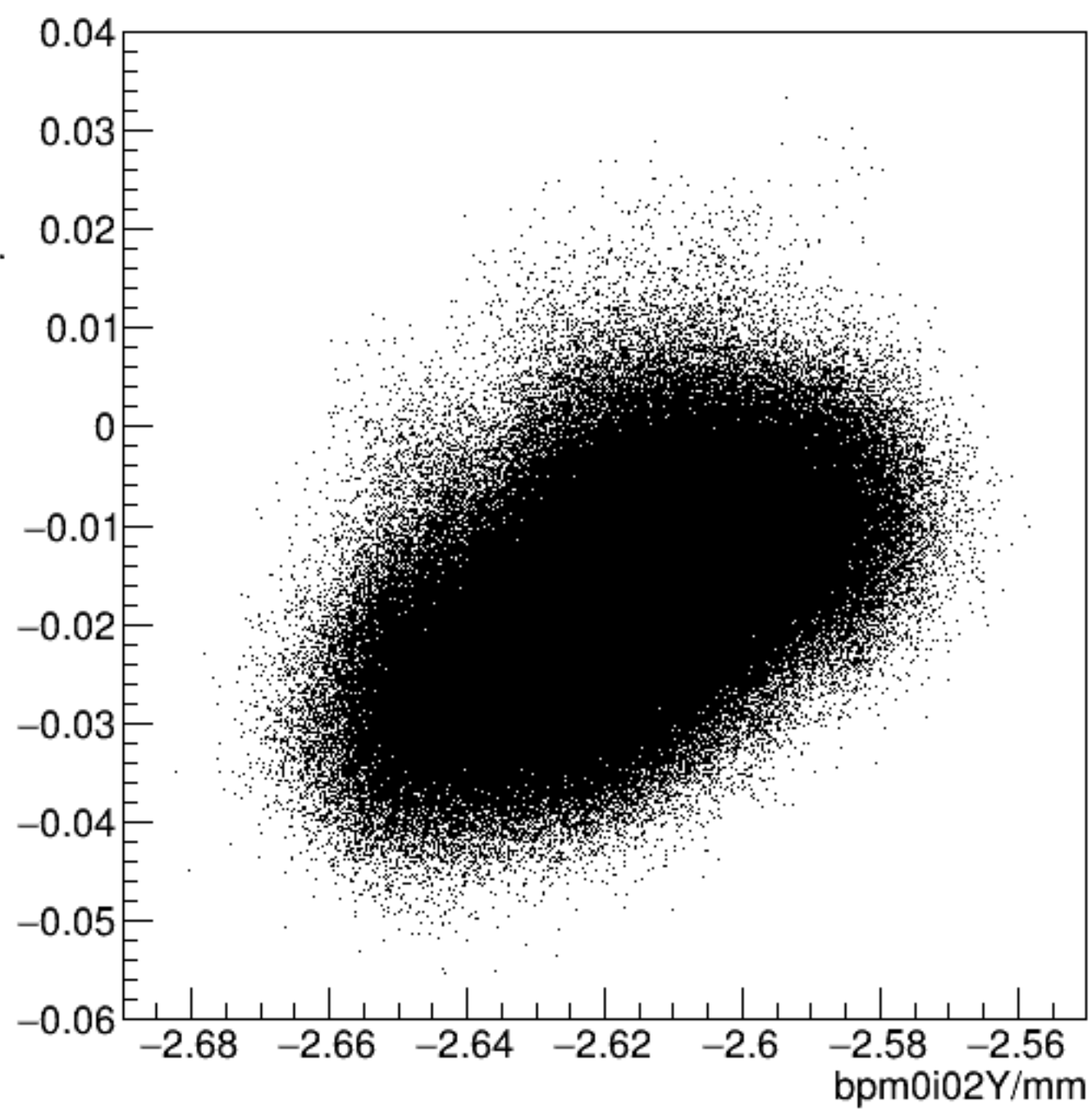
bpm0i02X/mm:bpm0i02Y/mm {ErrorFlag==0}
