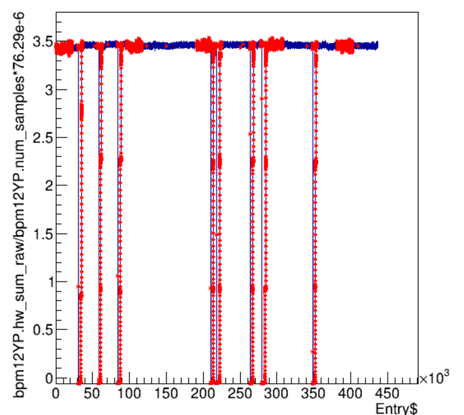
bpm12YP.hw_sum_raw/bpm12YP.num_samples*76.29e-6:Entry$
