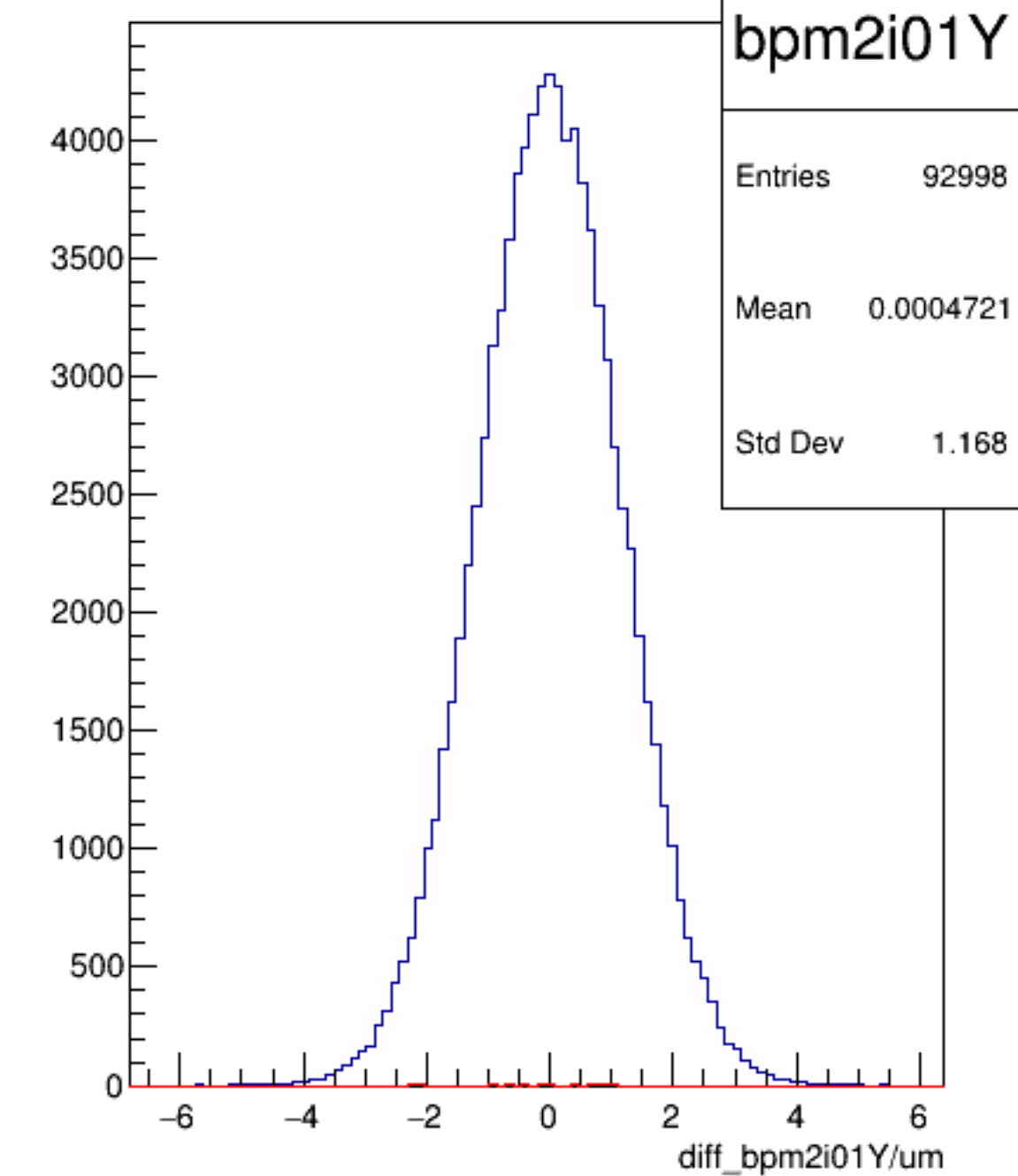
diff_bpm2i01Y/um {ErrorFlag==0}
