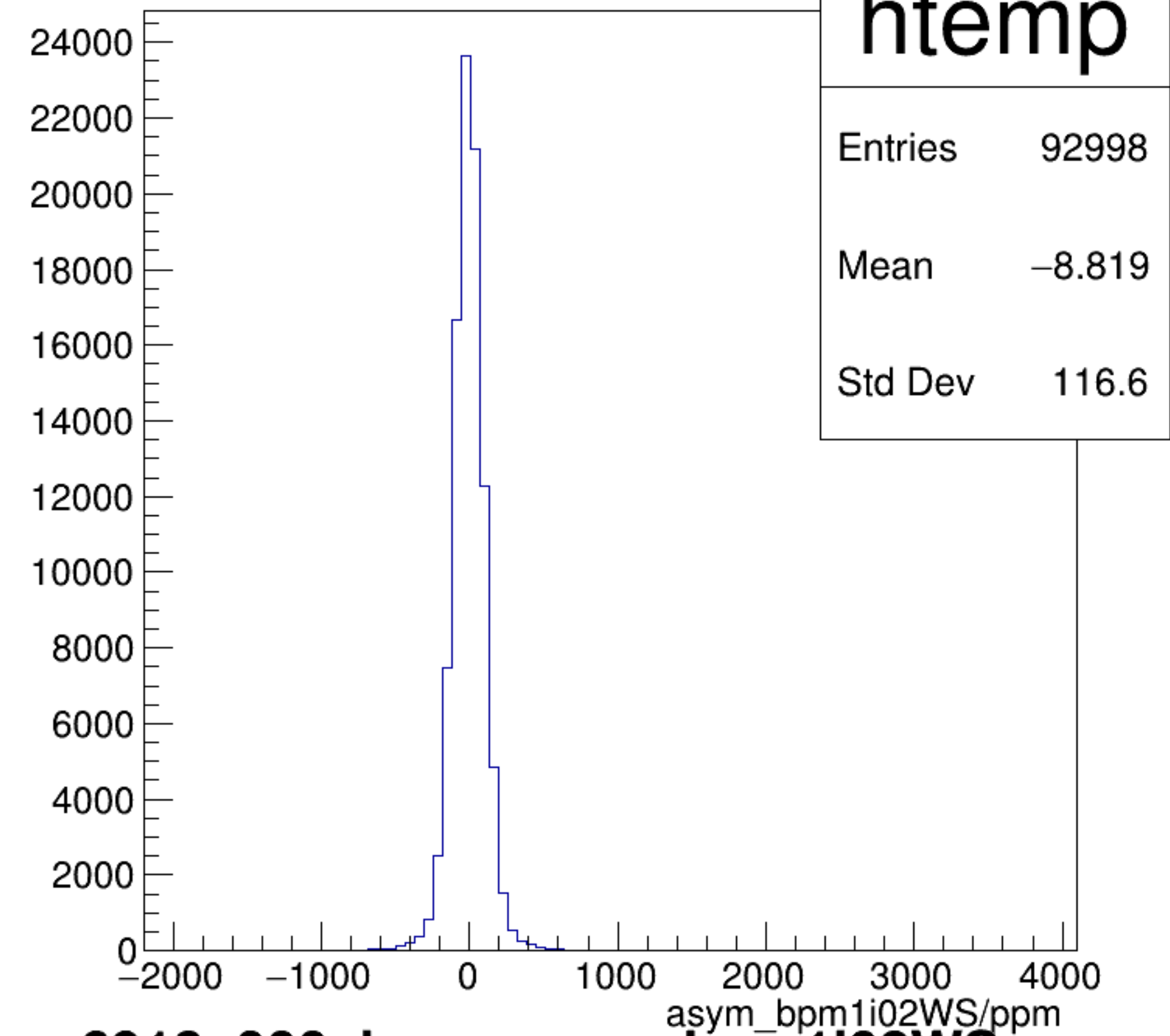
asym_bpm1i02WS/ppm {ErrorFlag==0}
