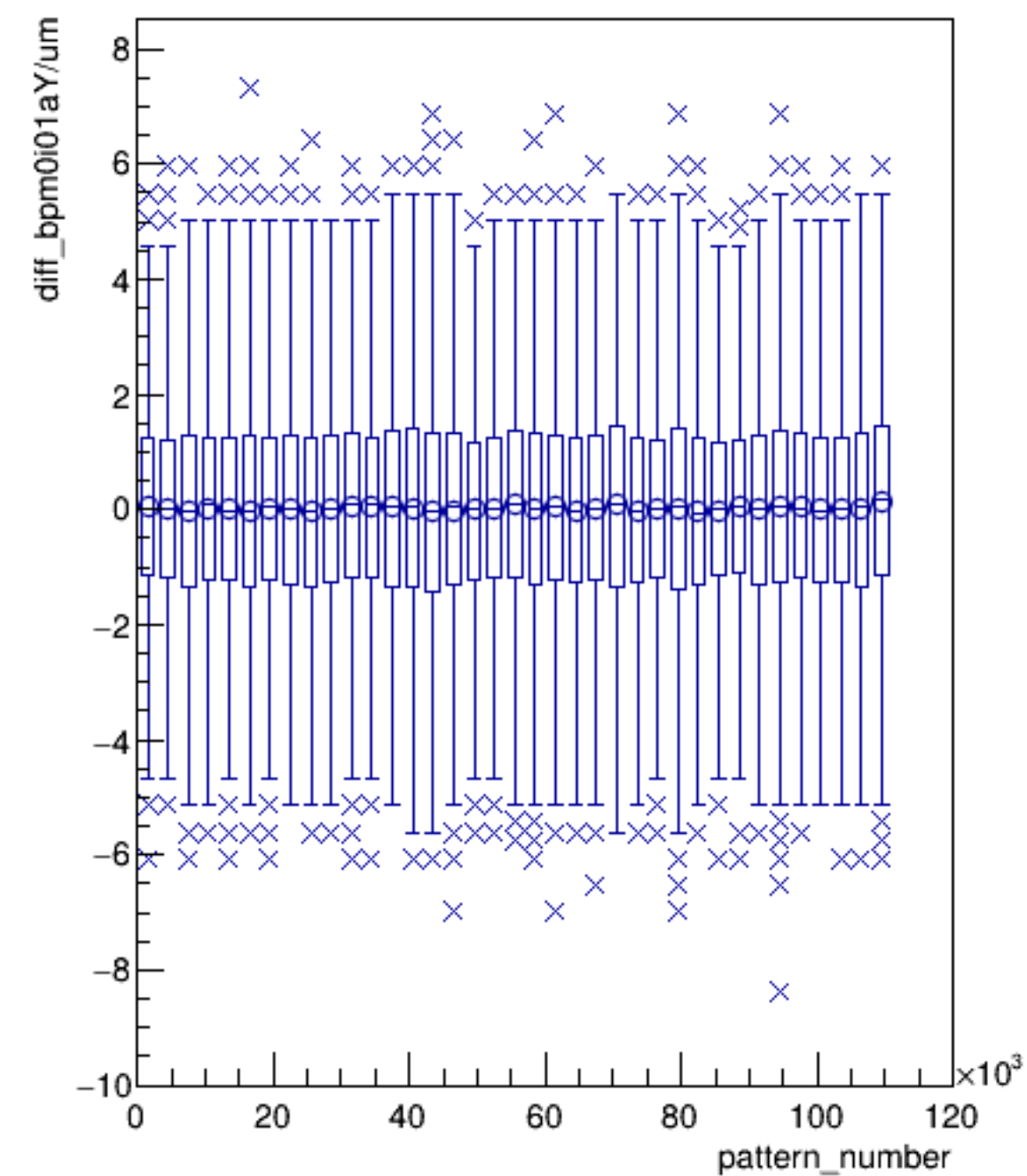
diff_bpm0i01aY/um:pattern_number (ErrorFlag==0)
