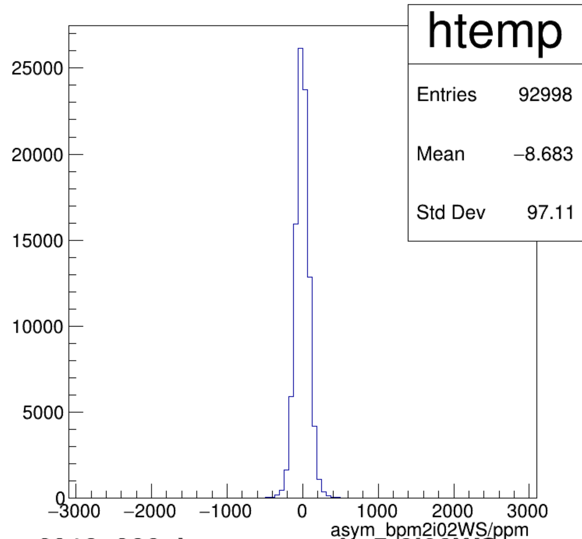
asym_bpm2i02WS/ppm {ErrorFlag==0}
