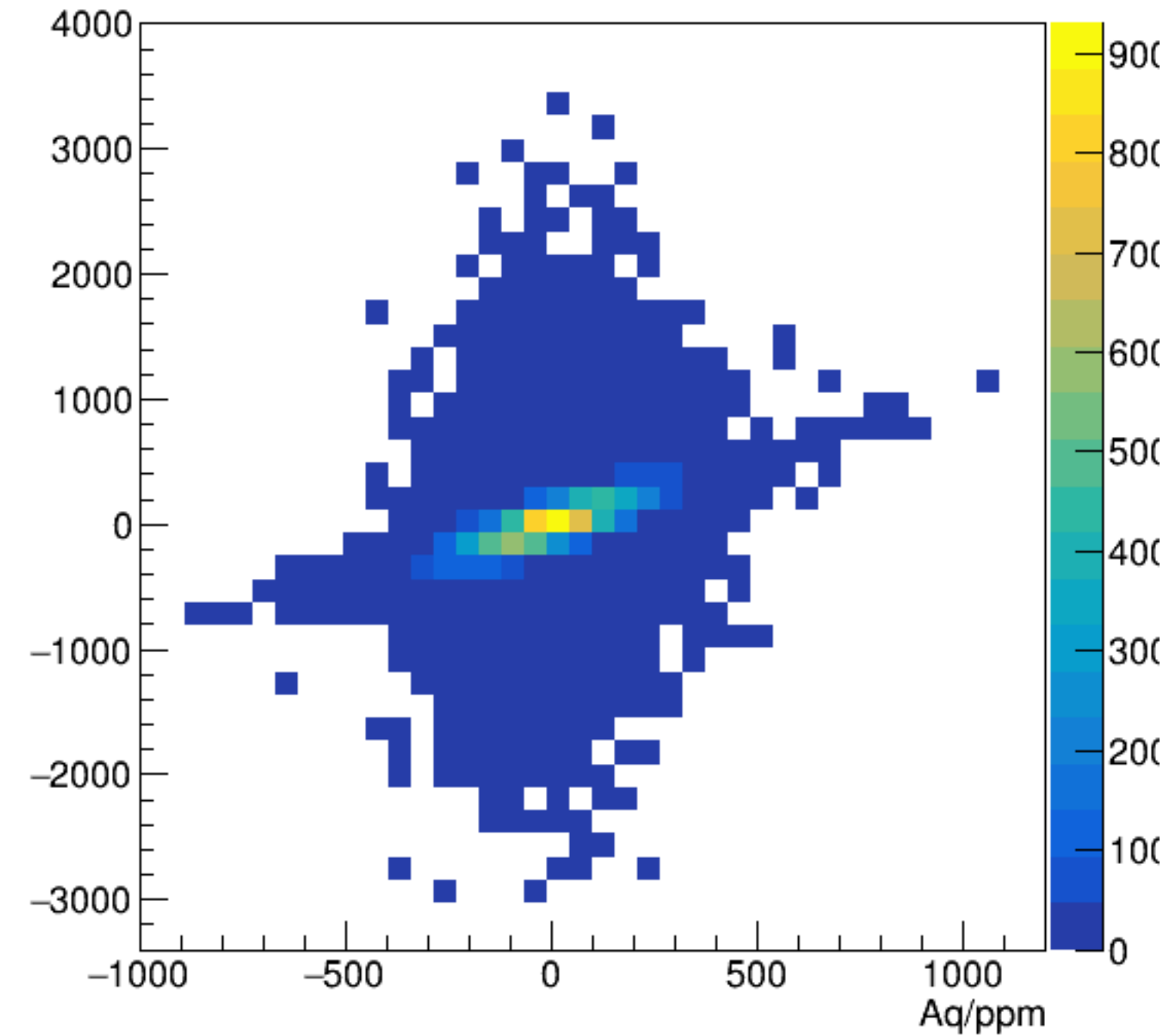
asym_bpm4aWS/ppm:Aq/ppm {ErrorFlag==0}
