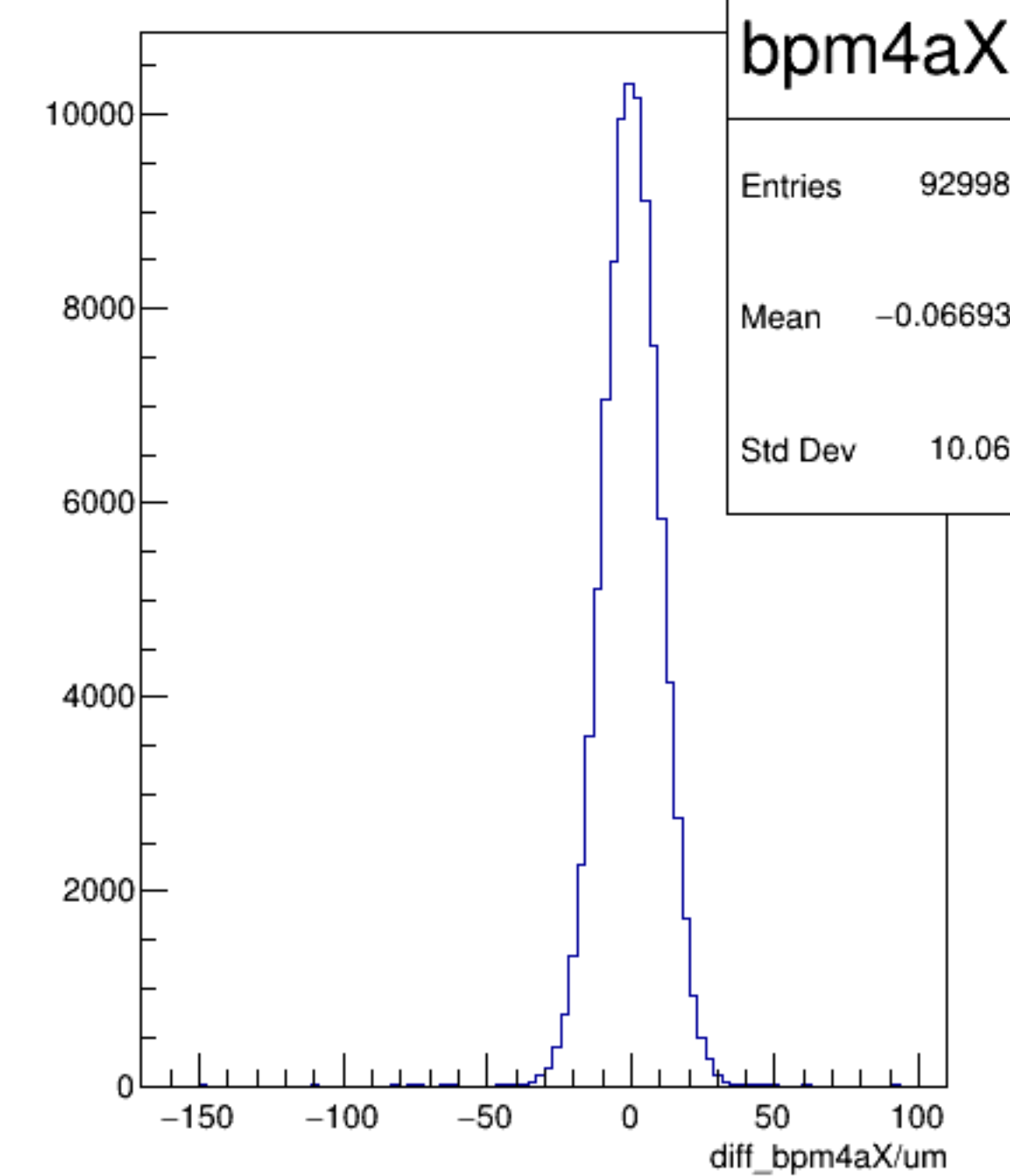
diff_bpm4aX/um {ErrorFlag==0}
