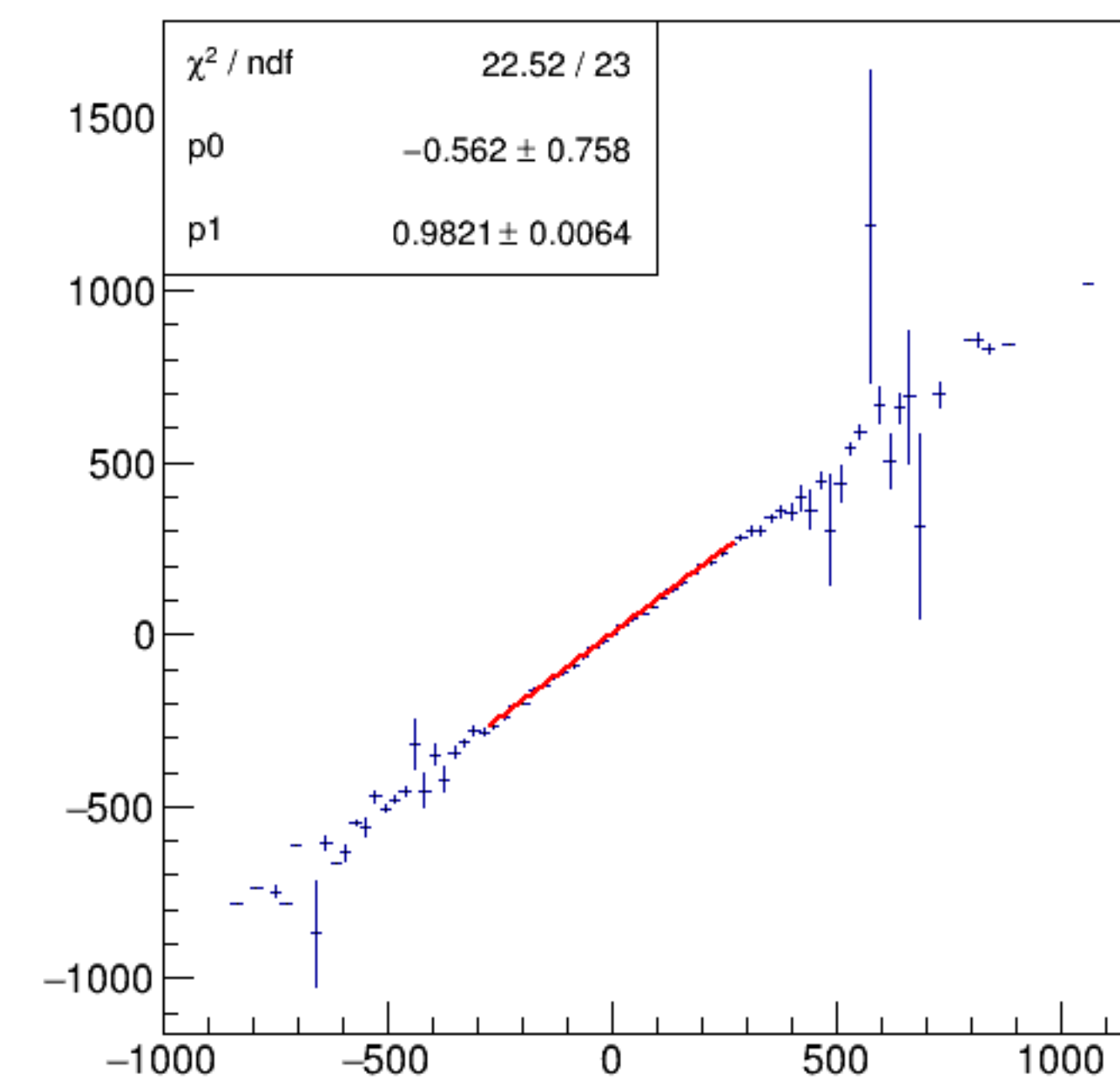
asym_bpm4acWS/ppm:Aq/ppm {ErrorFlag==0}
