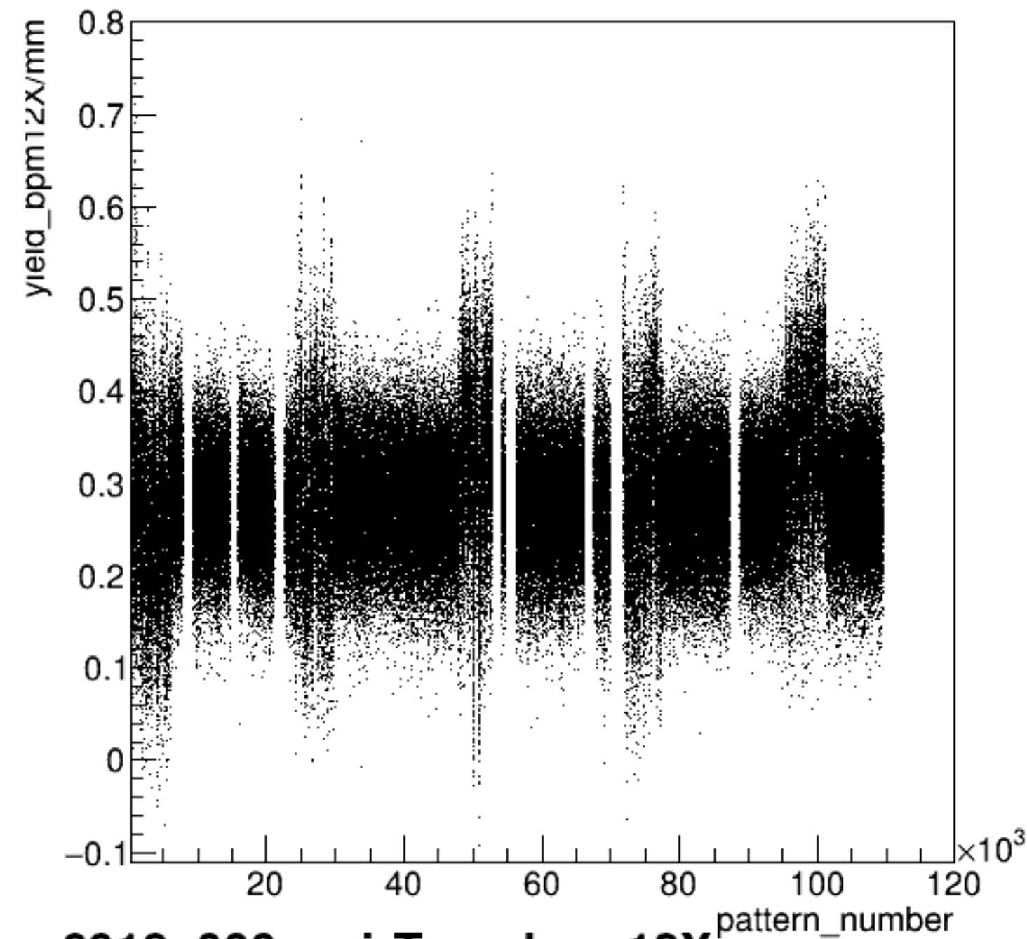
yield_bpm12X/mm:pattern_number {ErrorFlag==0}
