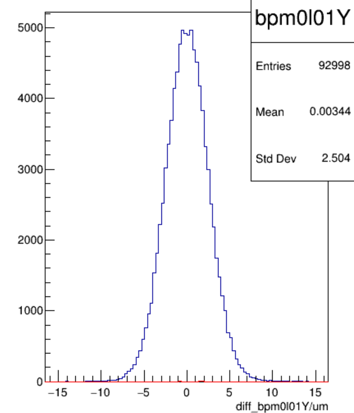
diff_bpm0I01Y/um {ErrorFlag==0}
