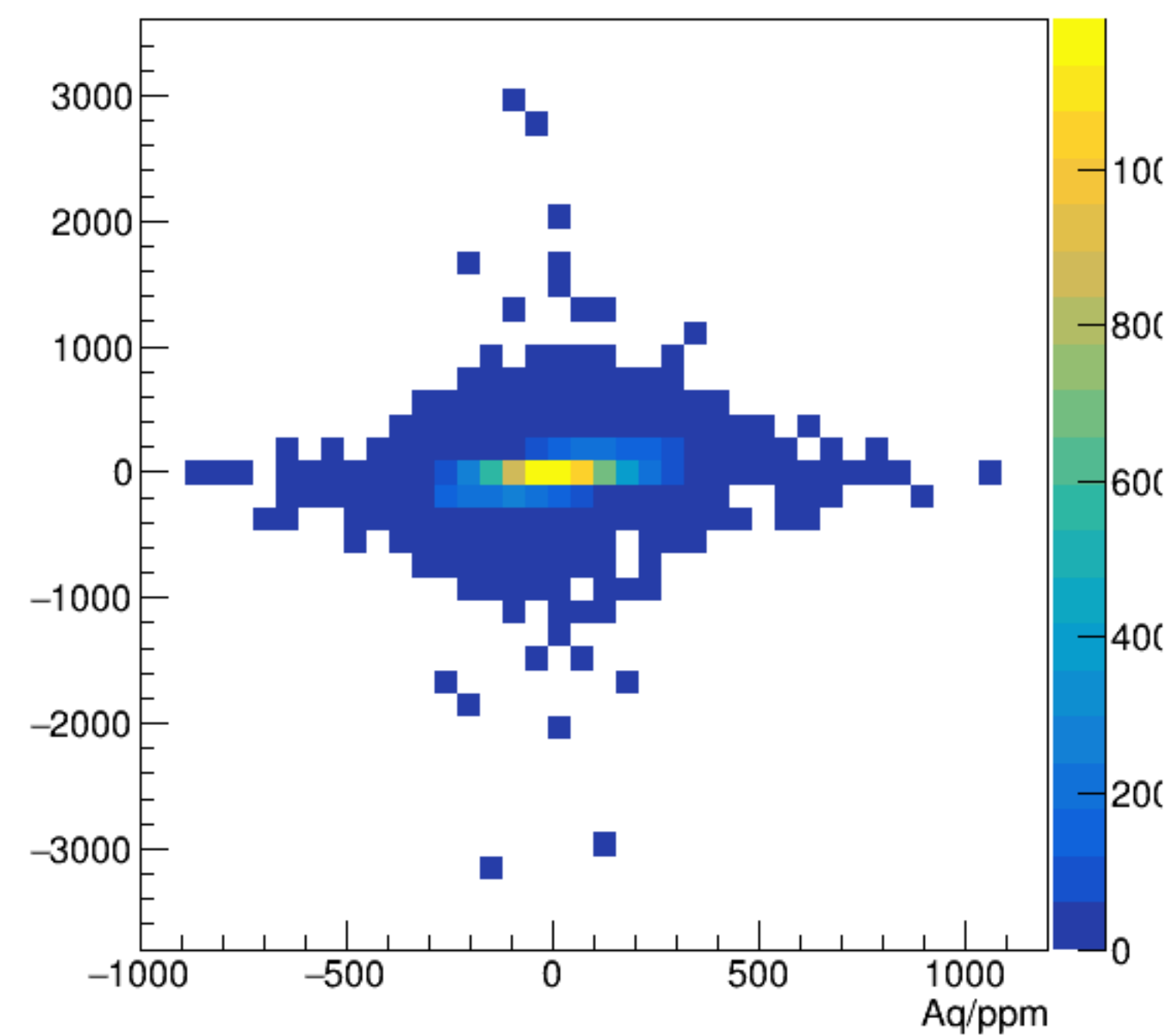
asym_bpm0i01aWS/ppm:Aq/ppm {ErrorFlag==0}
