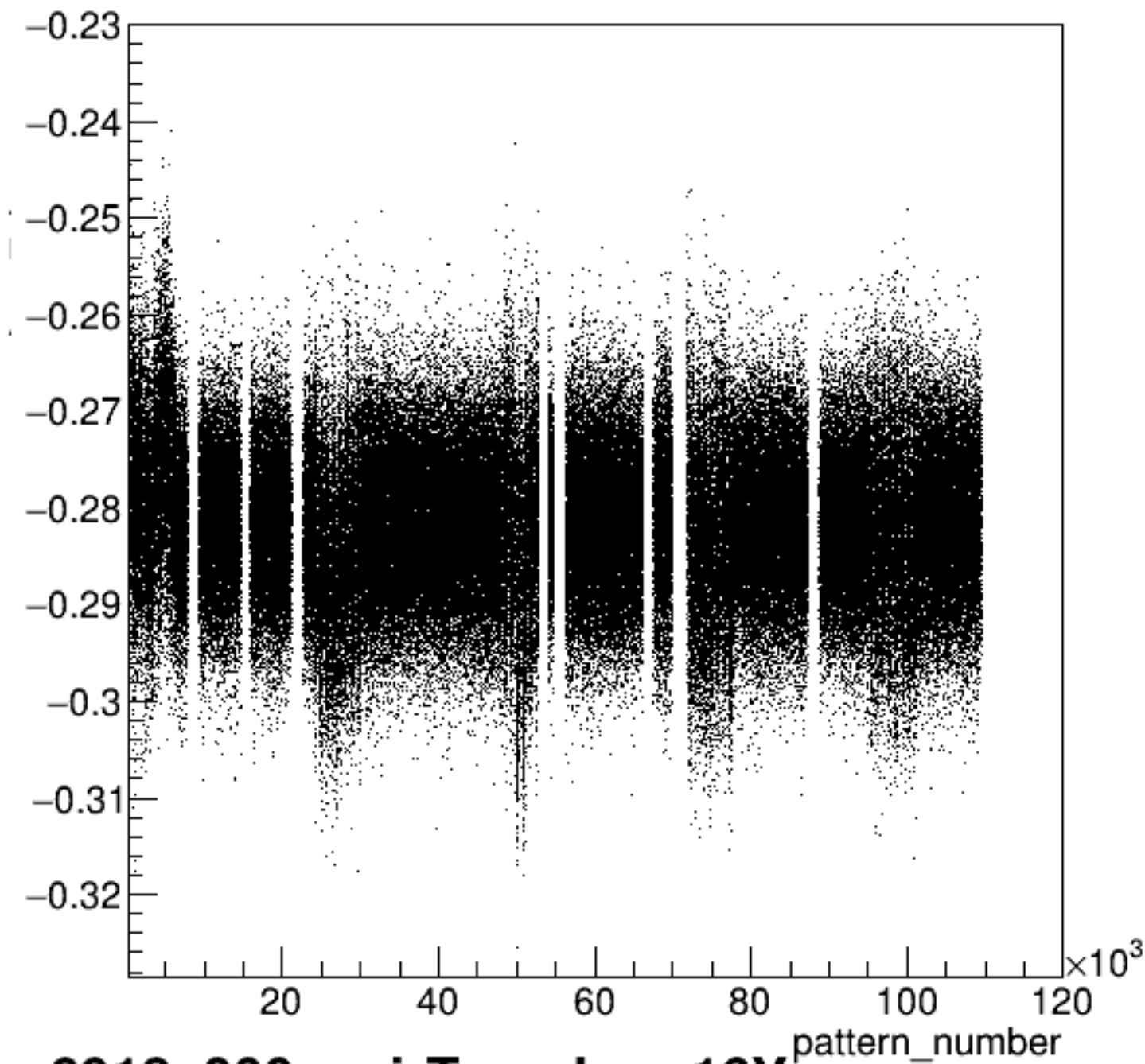
yield_bpm16Y/mm:pattern_number {ErrorFlag==0}
