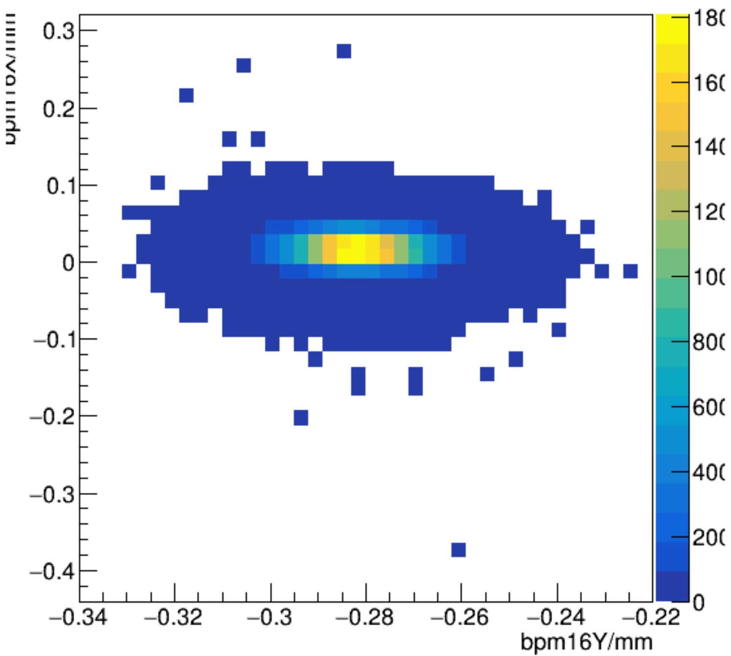
bpm16X/mm:bpm16Y/mm {ErrorFlag==0}
