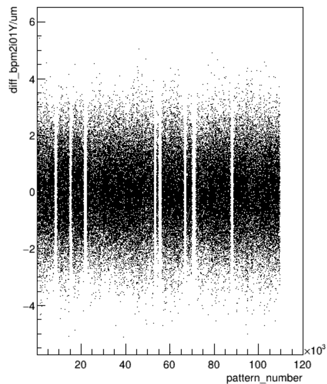
diff_bpm2i01Y/um:pattern_number (ErrorFlag==0)
