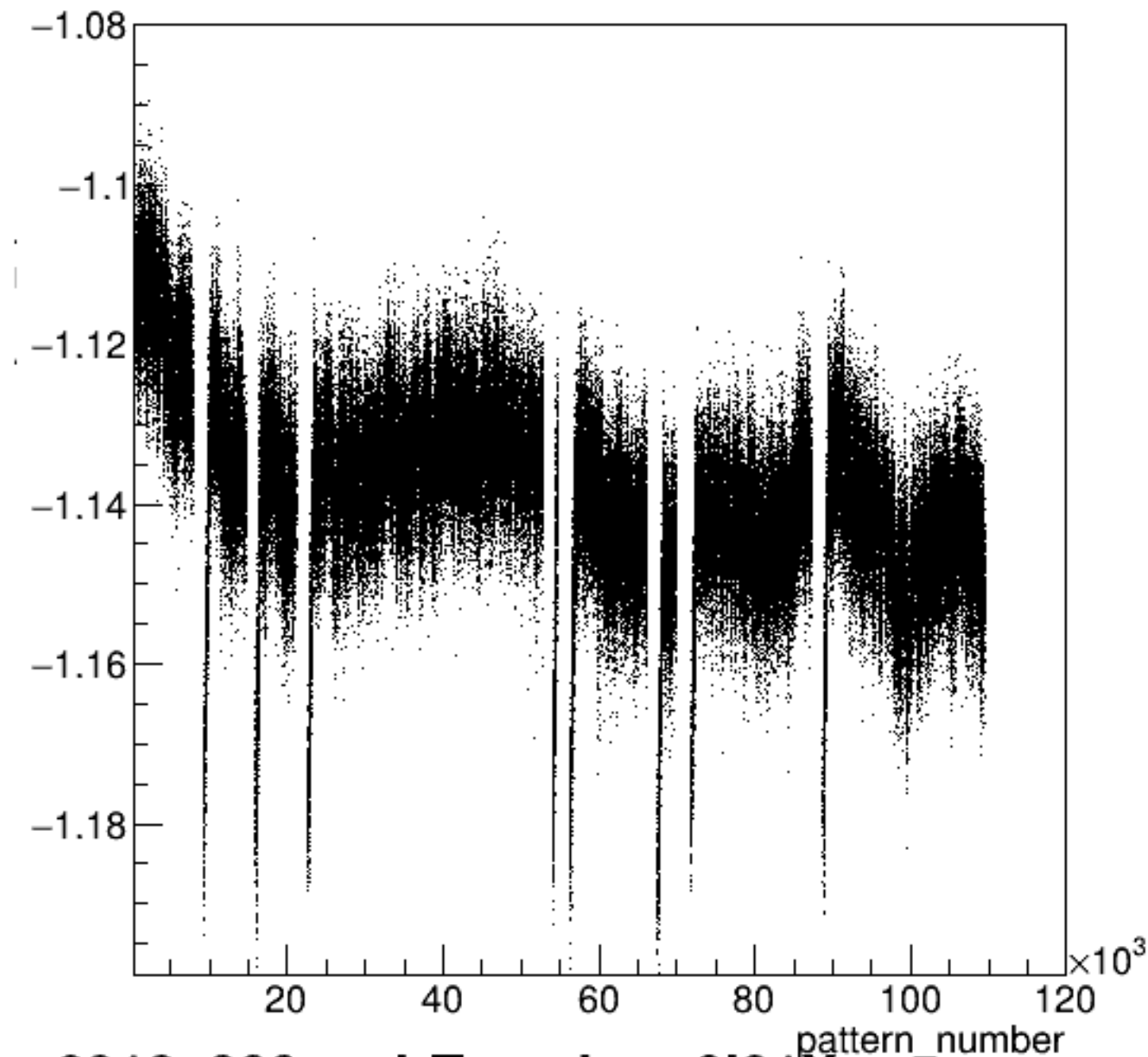
yield_bpm0l01X/mm:pattern_number {ErrorFlag==0}
