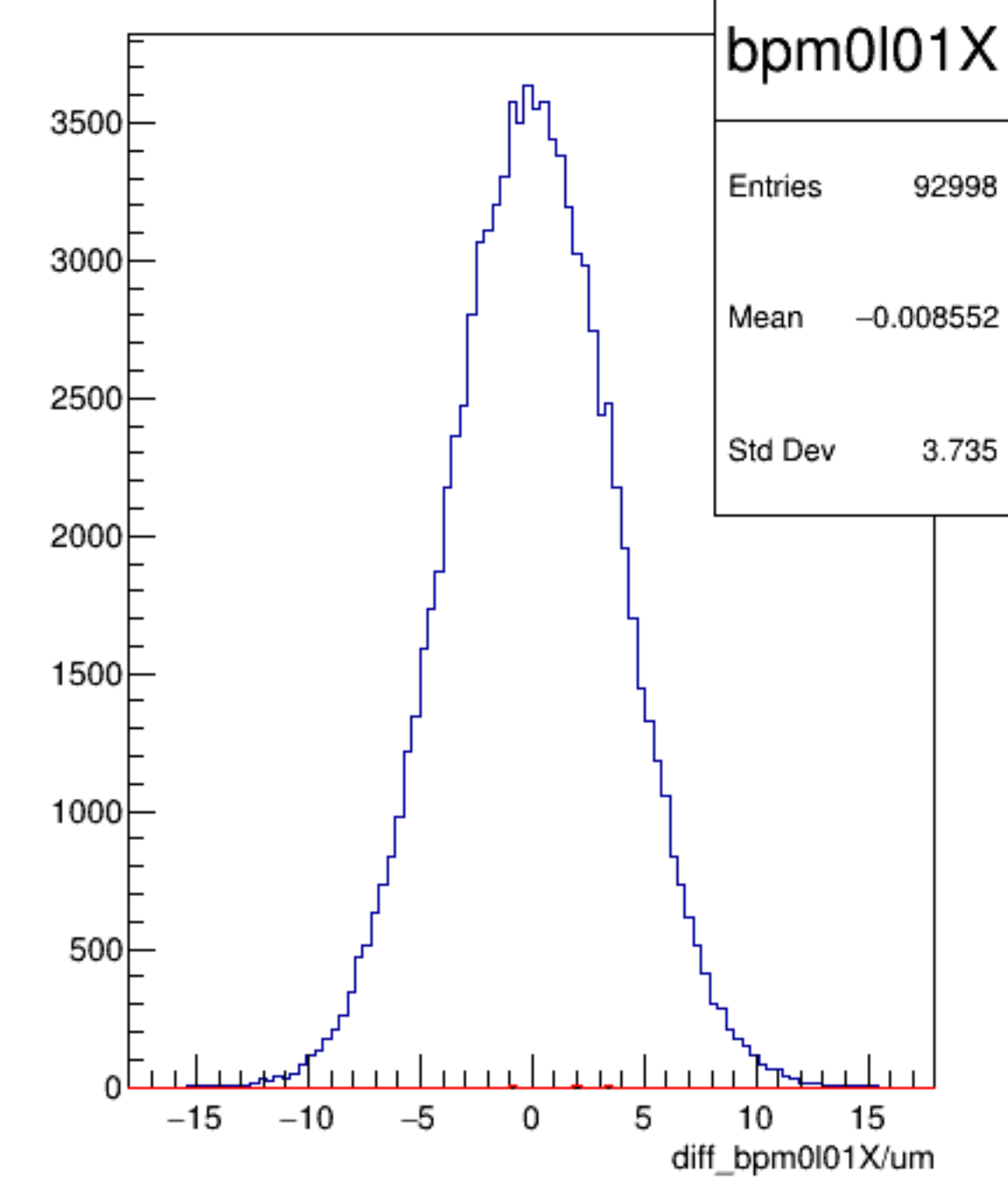
diff_bpm0I01X/um {ErrorFlag==0}
