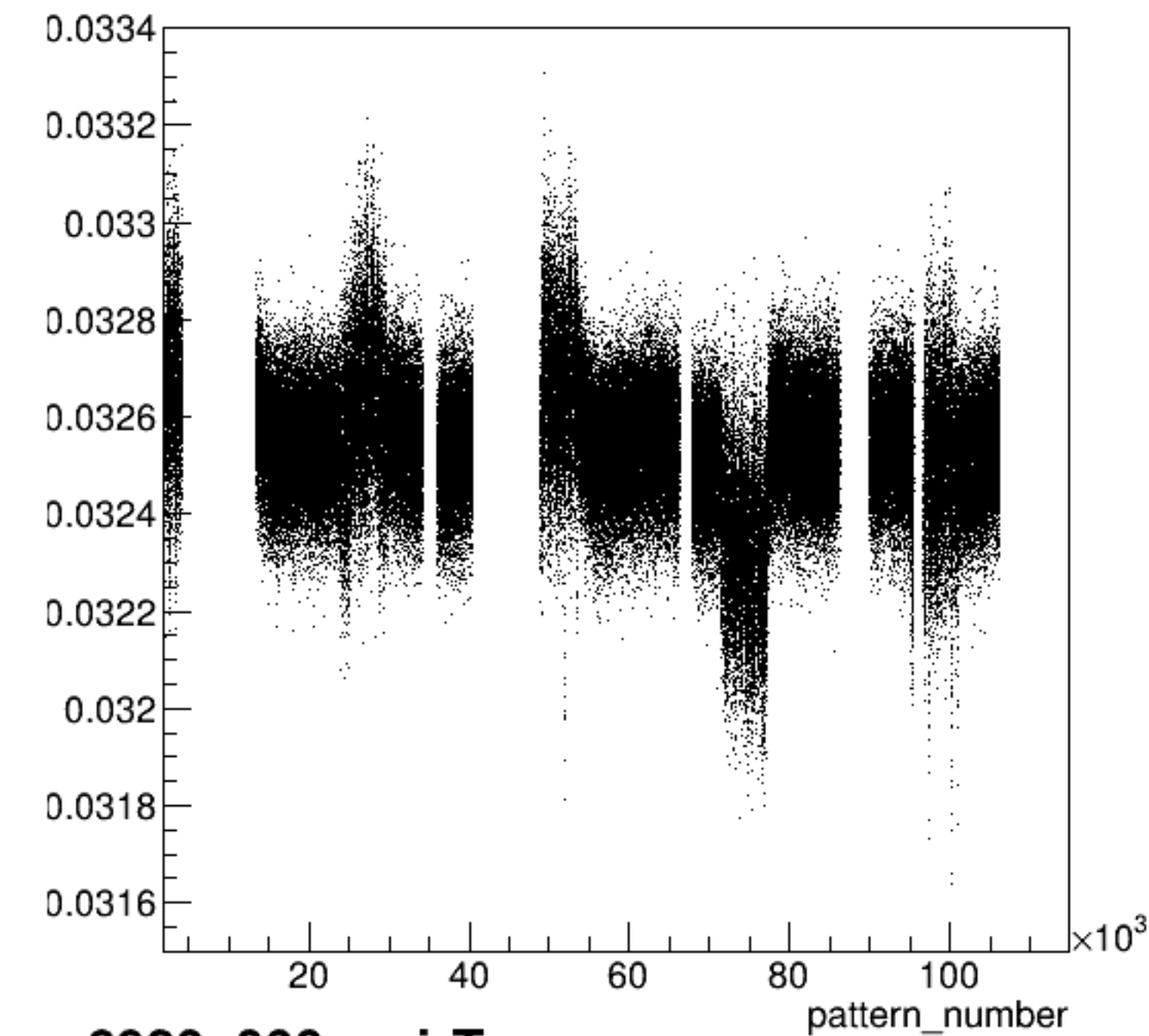
yield_usr:pattern_number {ErrorFlag==0}
