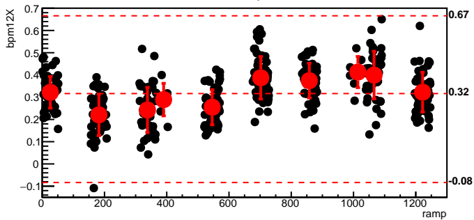
bmod_trim1,cyc=7495
