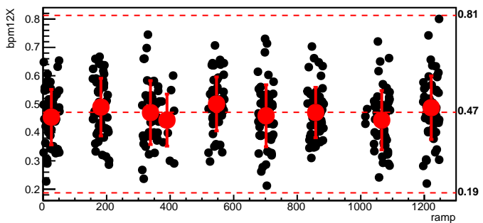
bmod_trim6,cyc=7495
