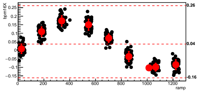
bmod_trim3,cyc=7495
