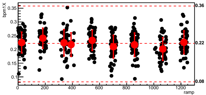
bmod_trim6,cyc=7495
