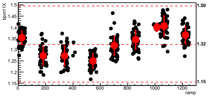
bmod_trim3,cyc=7495
