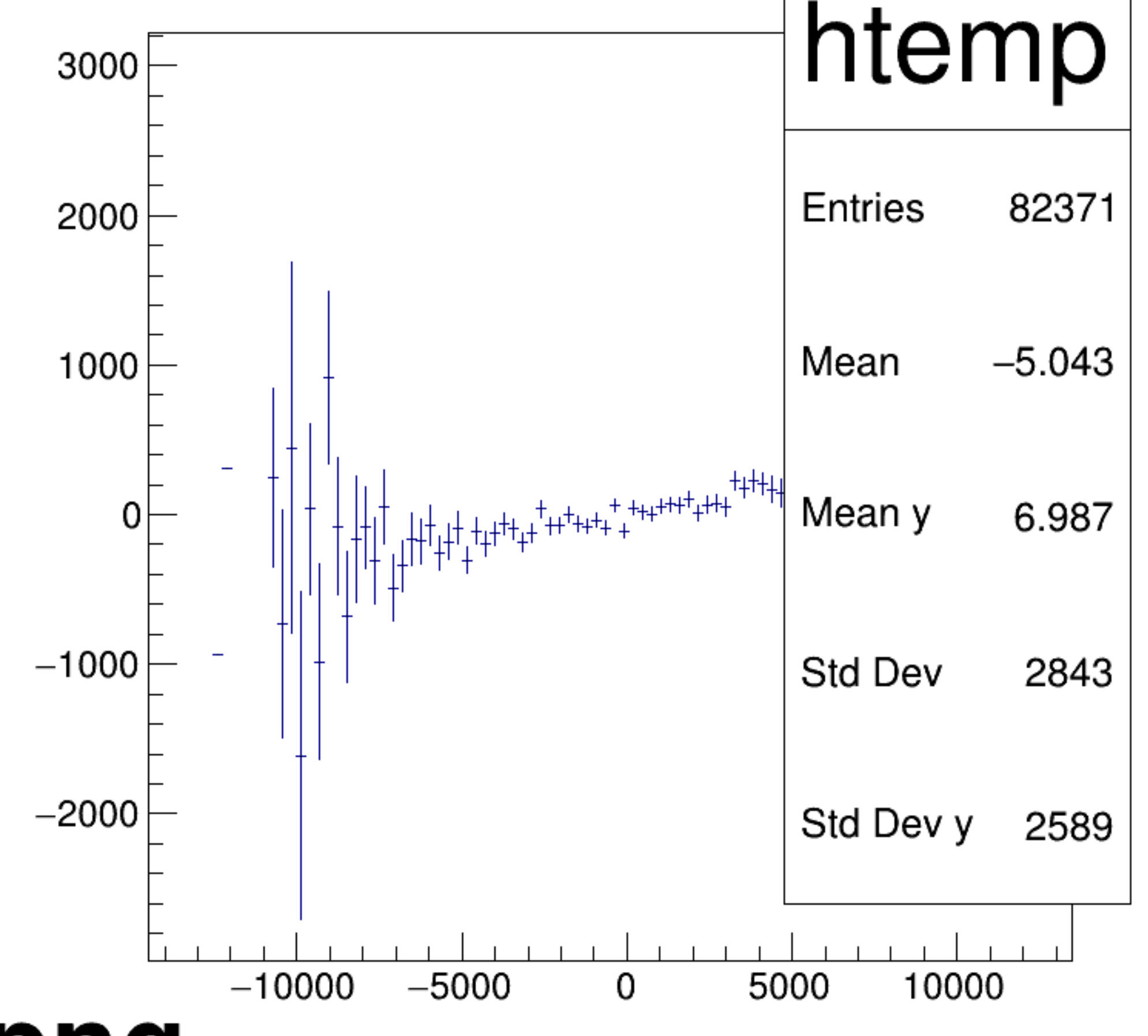
asym_atl1/ppm:asym_atr1/ppm {ok_cut}
