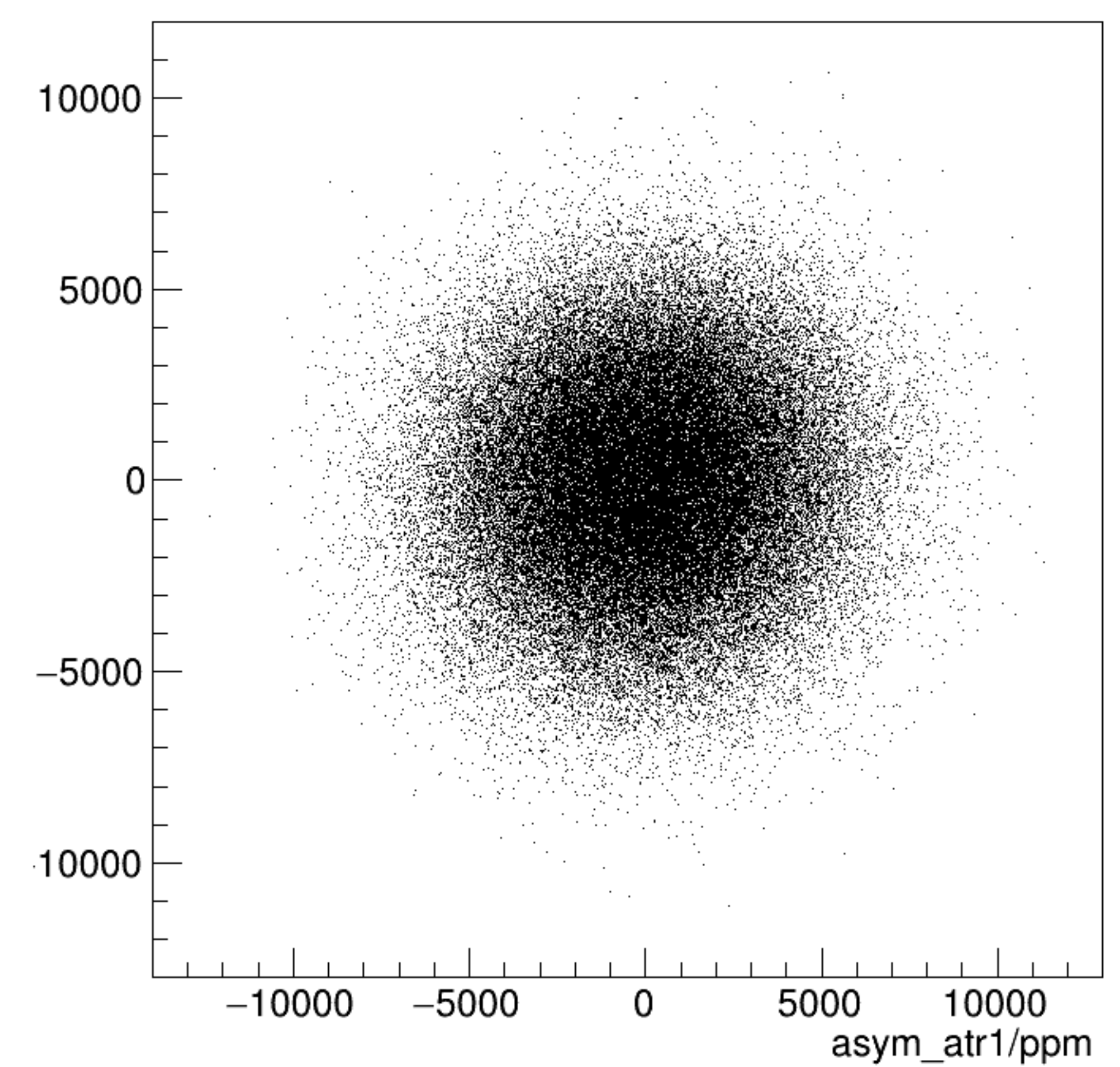
asym_atl1/ppm:asym_atr1/ppm {ok_cut}
