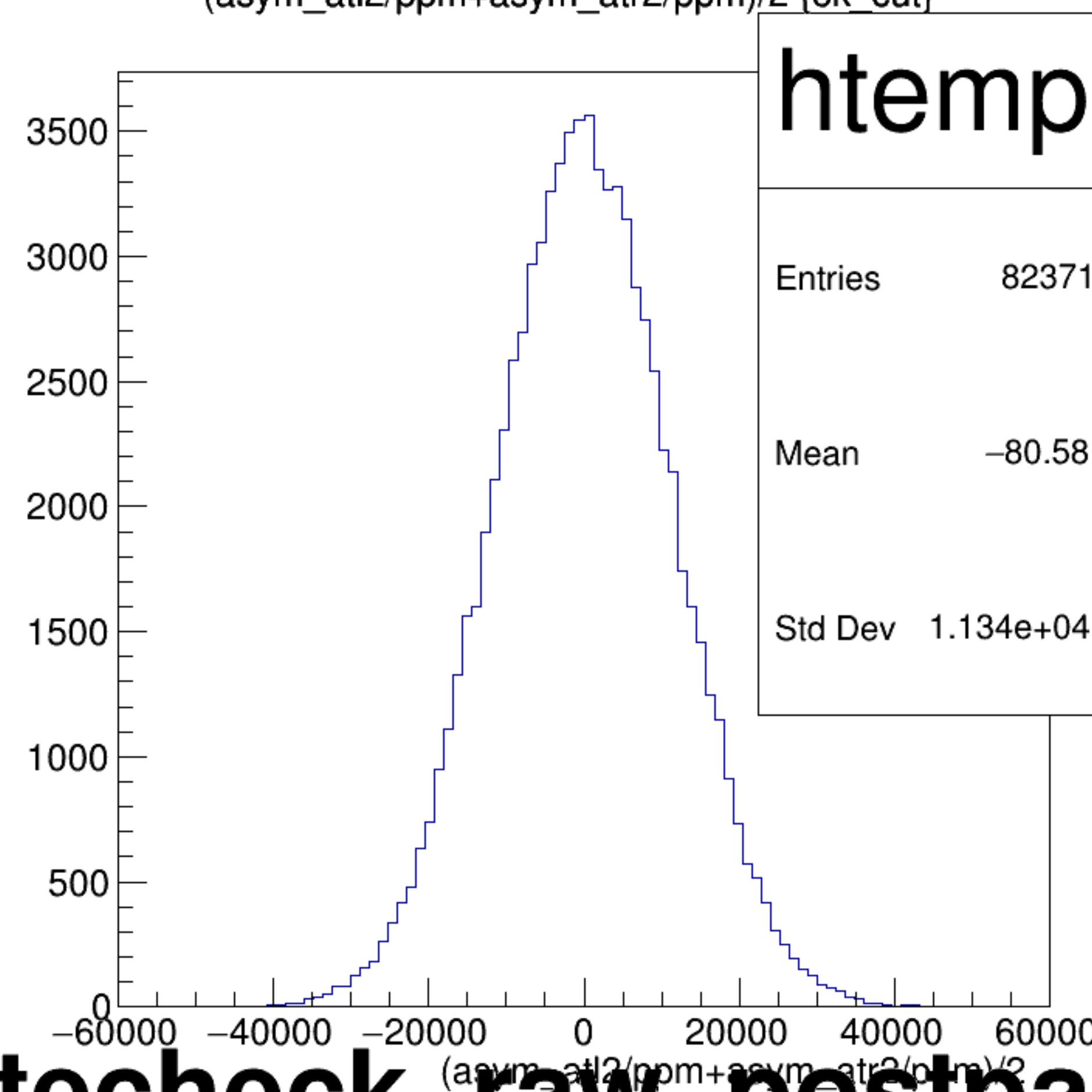
(asym_atl2/ppm+asym_atr2/ppm)/2 {ok_cut}
