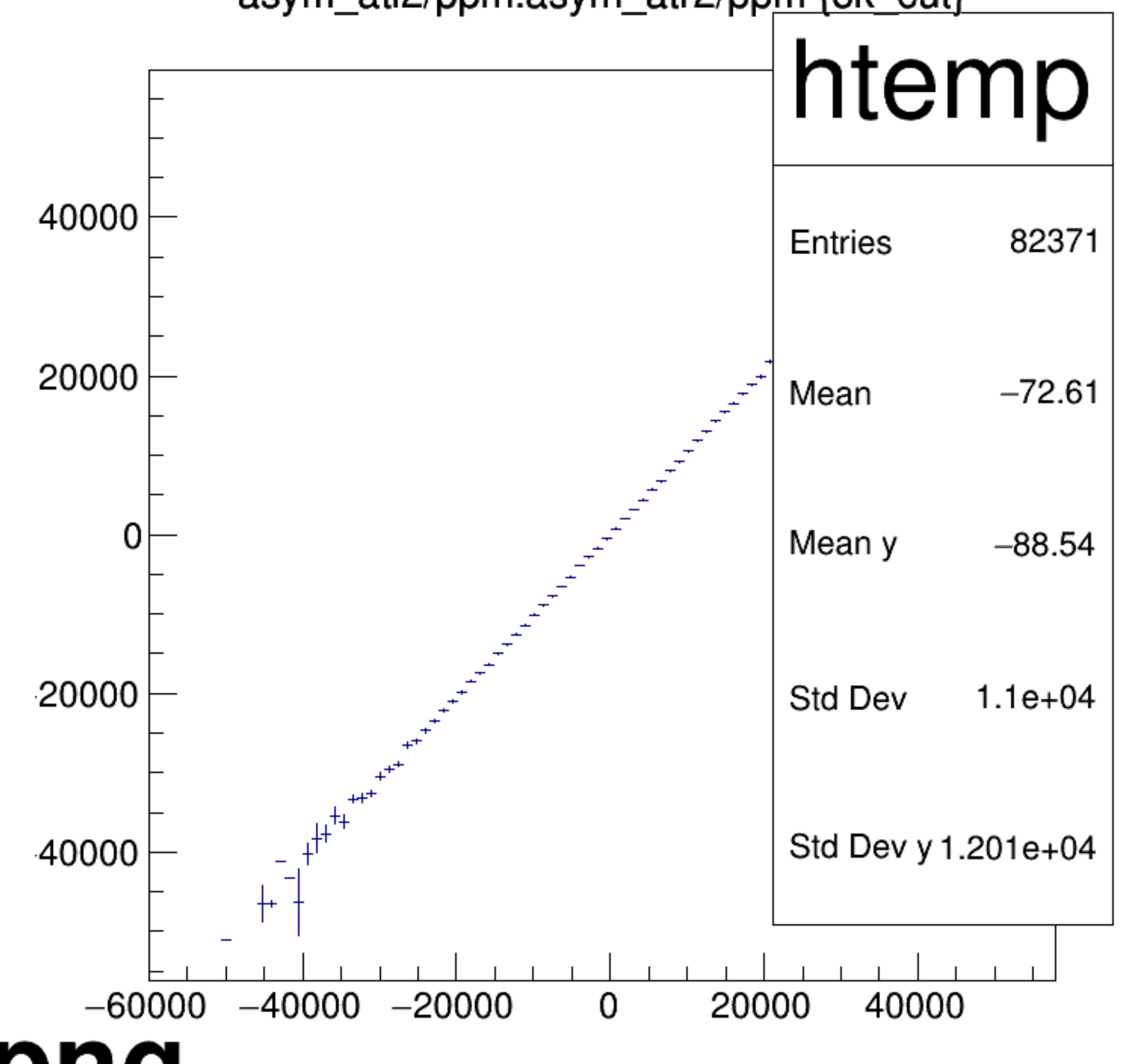
asym_atl2/ppm:asym_atr2/ppm {ok_cut}
