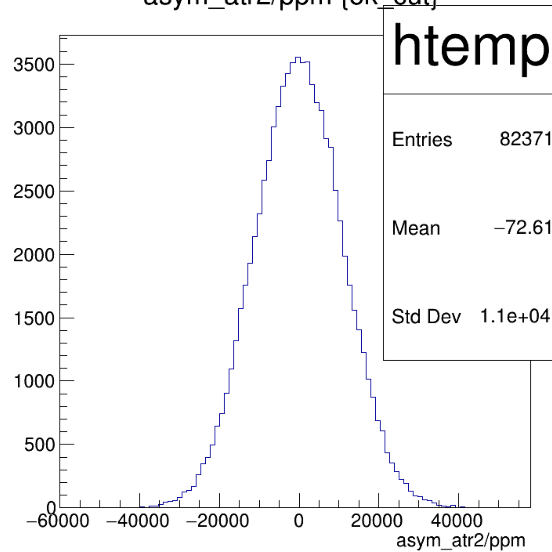
asym_atr2/ppm {ok_cut}
