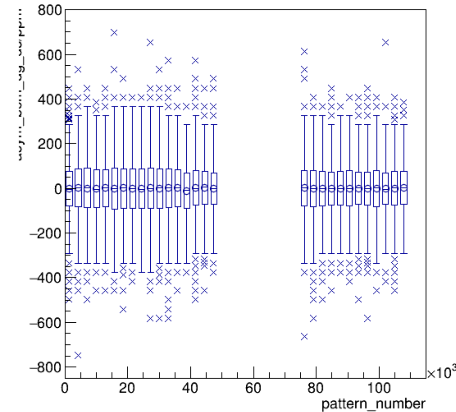
asym_bcm_dg_ds/ppm:pattern_number {ErrorFlag==0}
