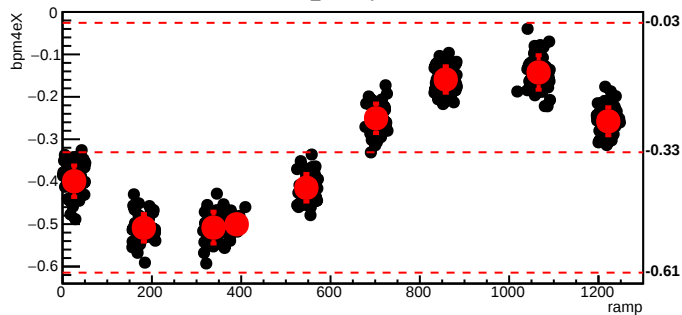
bmod_trim1,cyc=7533
