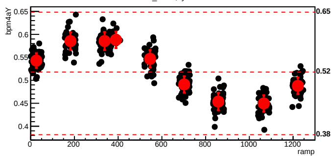
bmod_trim6,cyc=7533
