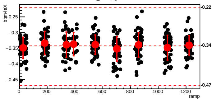
bmod_trim4,cyc=7533
