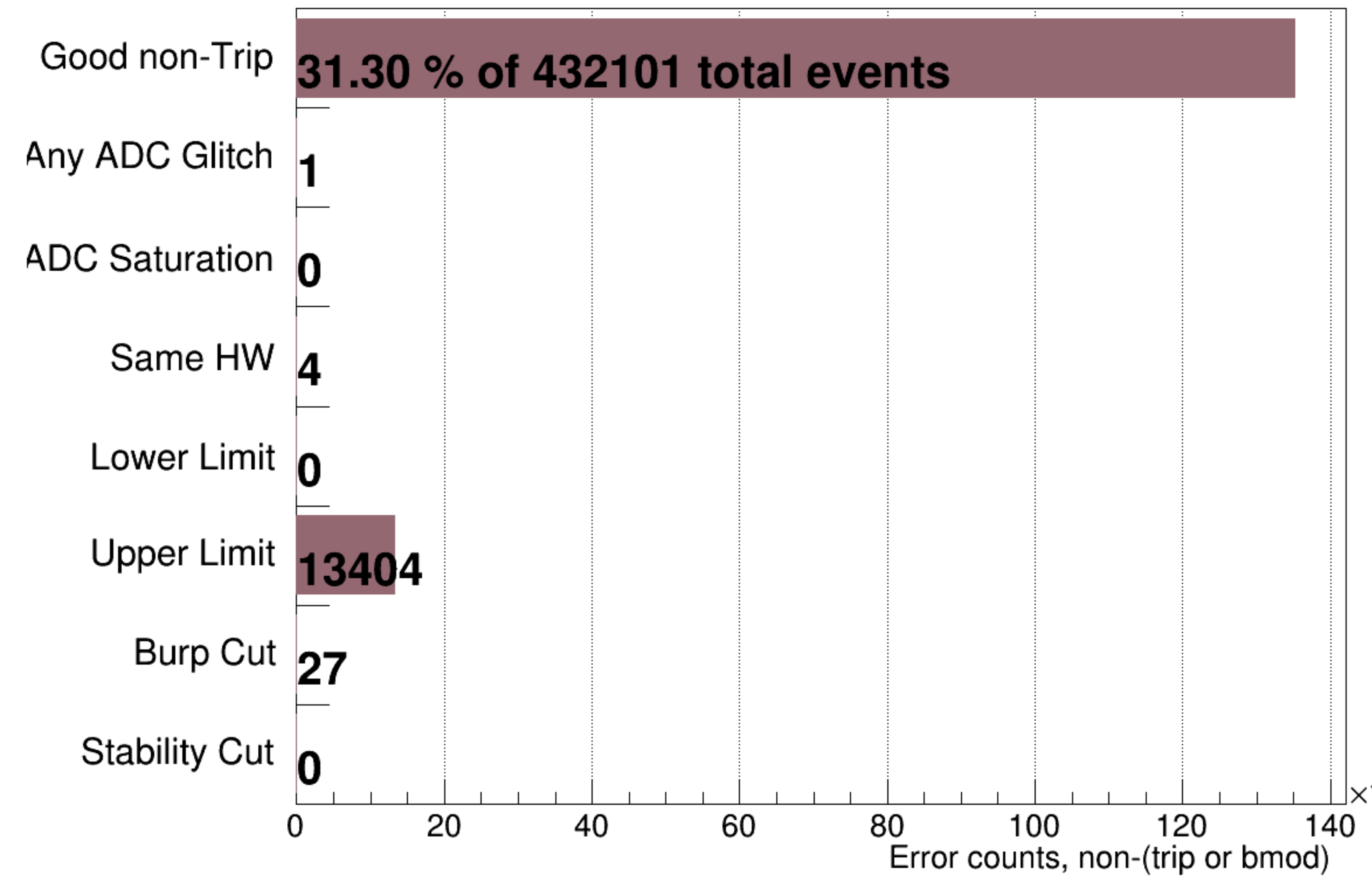
bpm12Y's Device Error Counter && Not (Trip || BMOD)
