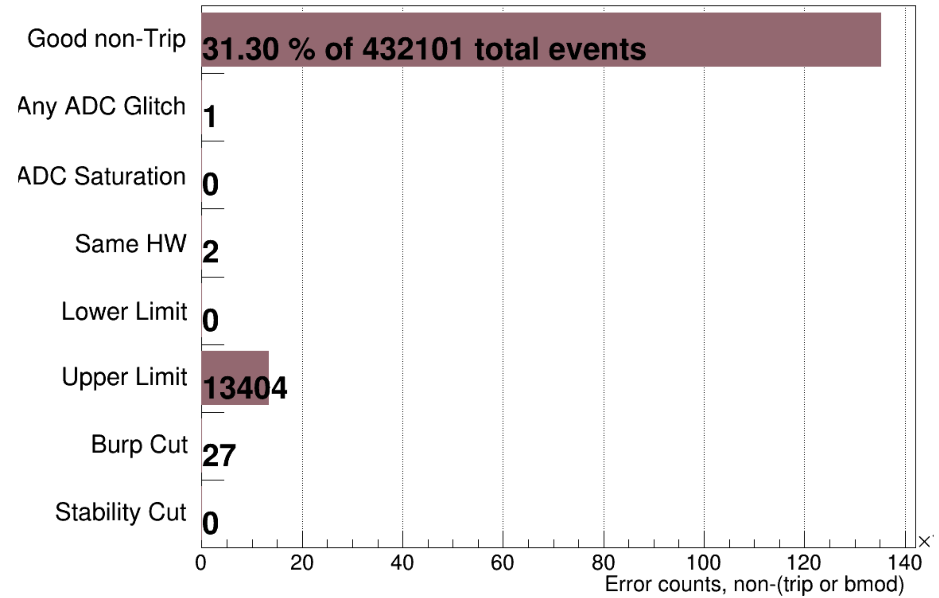
bpm11YM's Device Error Counter && Not (Trip || BMOD)
