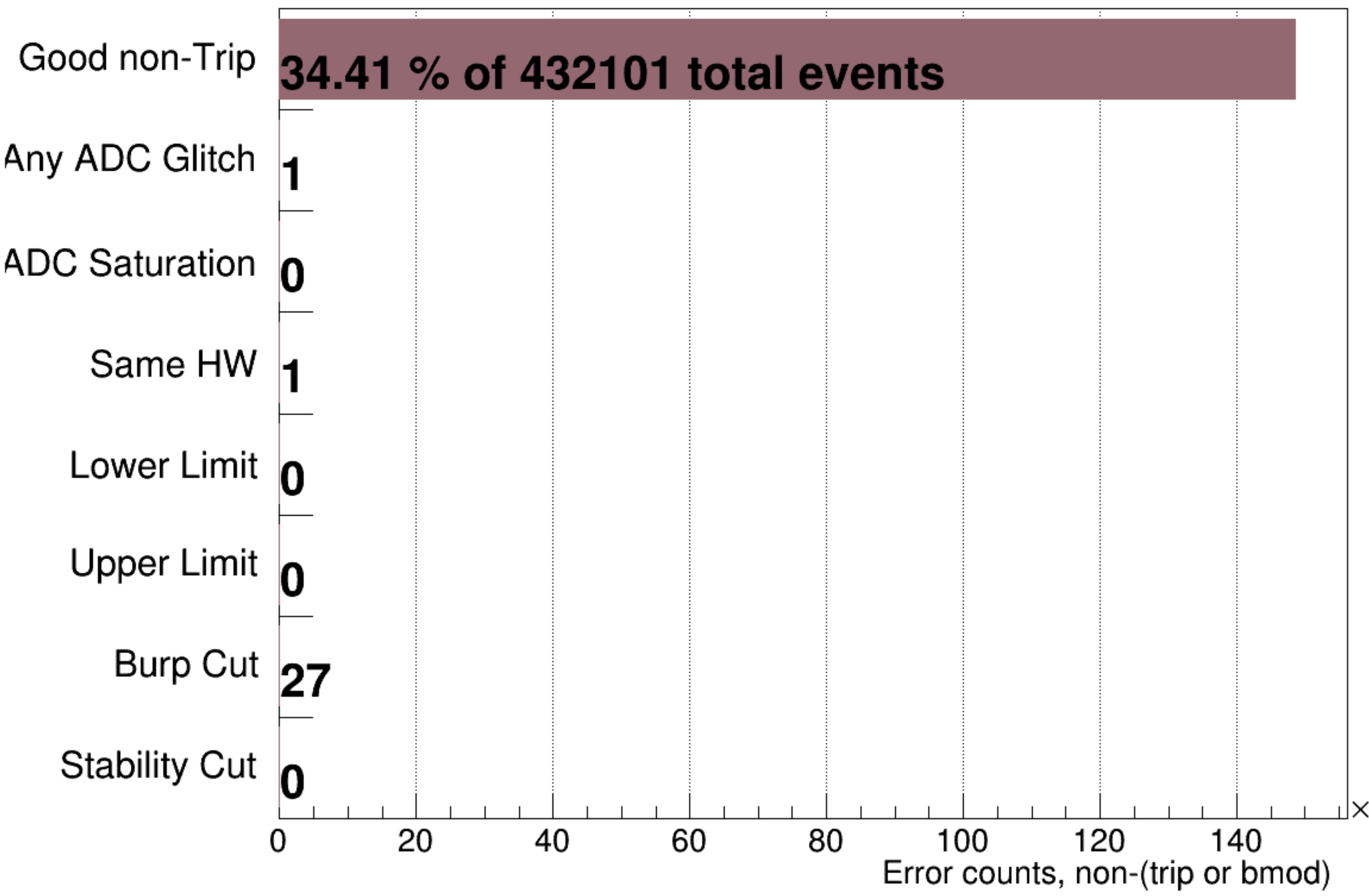
bpm4eYP's Device Error Counter && Not (Trip || BMOD)
