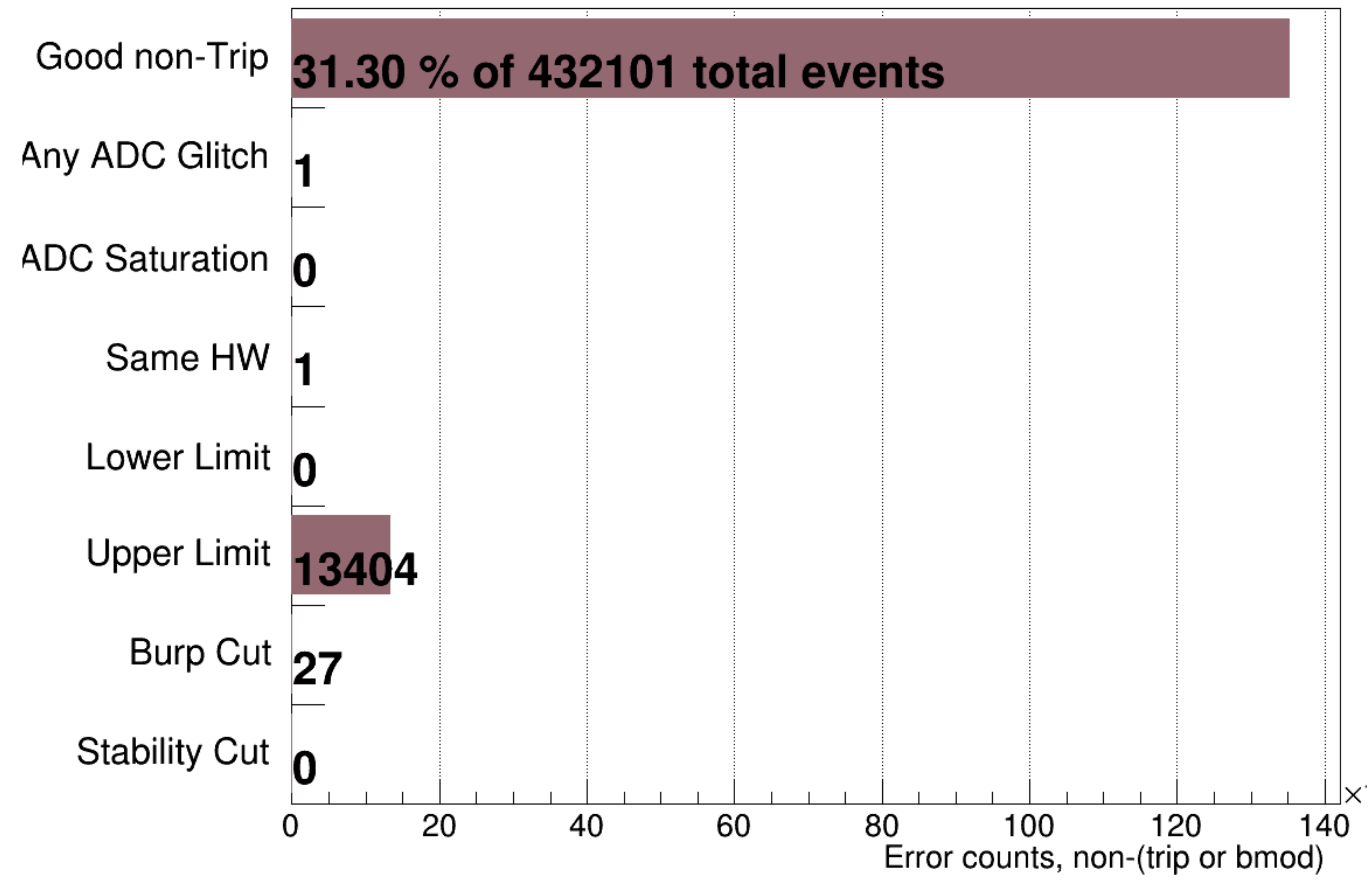
bpm12XP's Device Error Counter && Not (Trip || BMOD)
