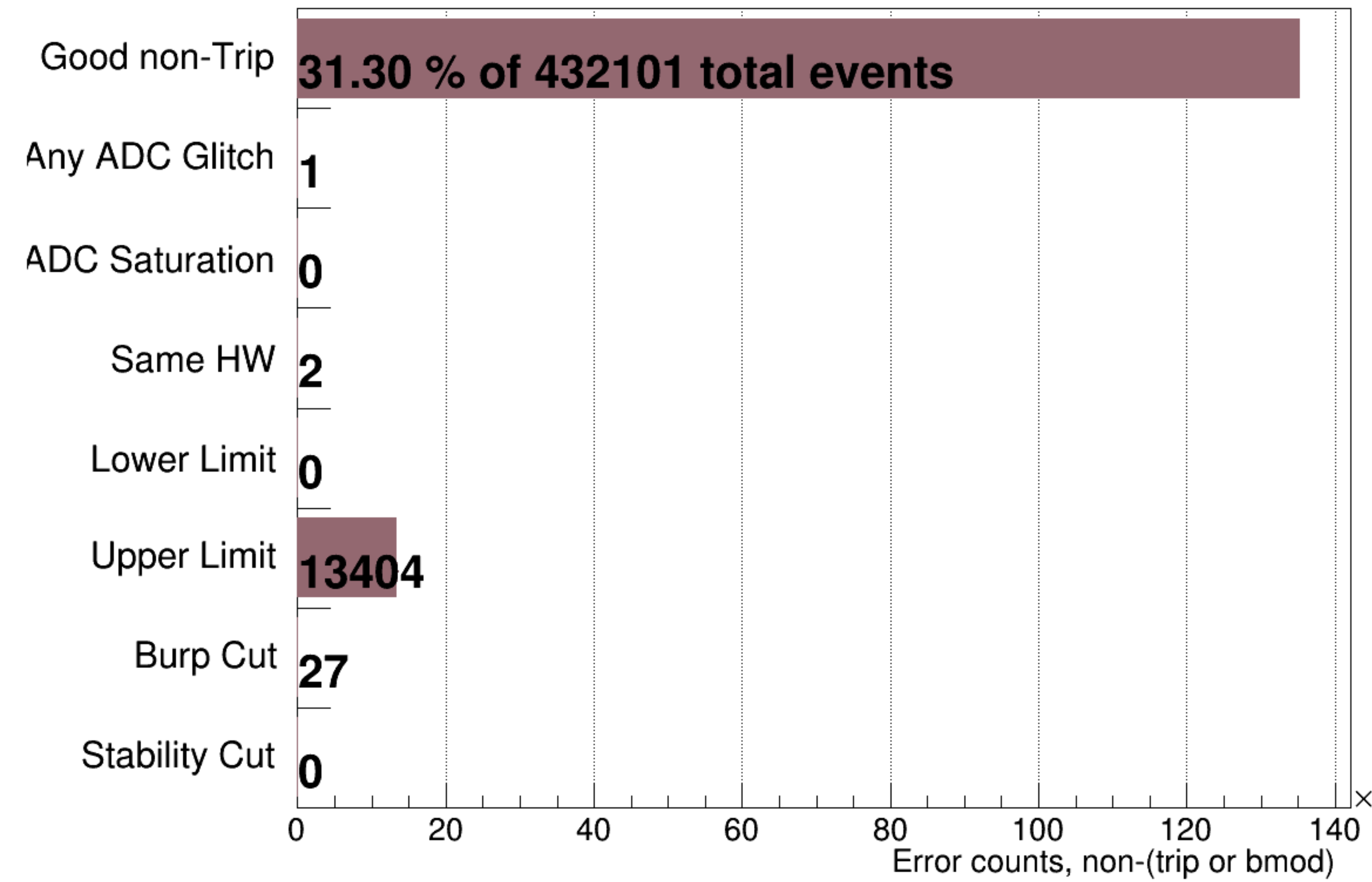
bpm11X's Device Error Counter && Not (Trip || BMOD)
