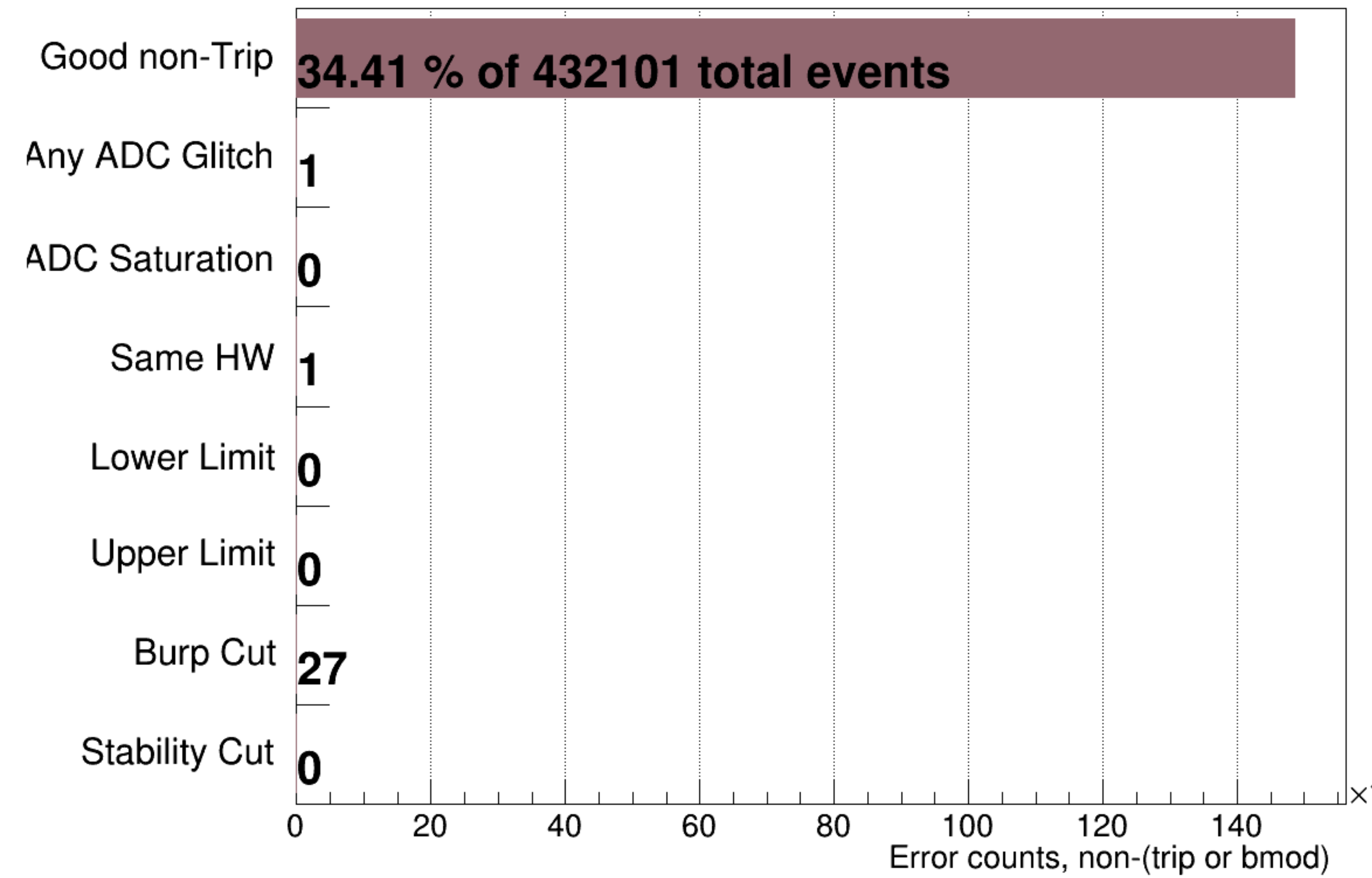
bpm4aYM's Device Error Counter && Not (Trip || BMOD)
