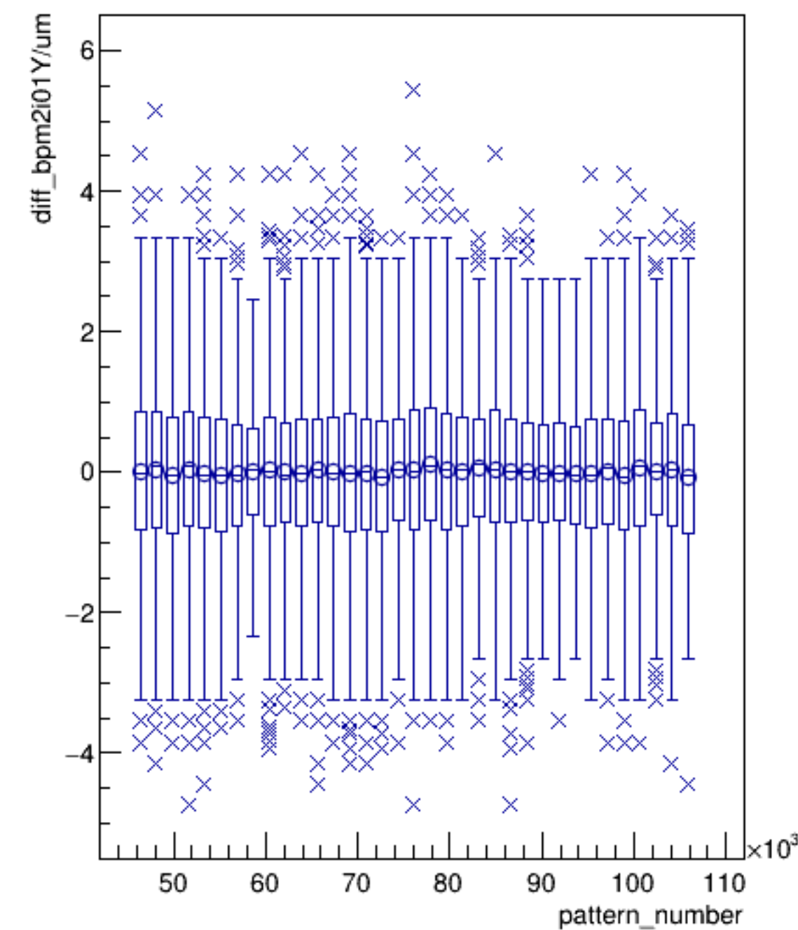
diff_bpm2i01Y/um:pattern_number (ErrorFlag==0)
