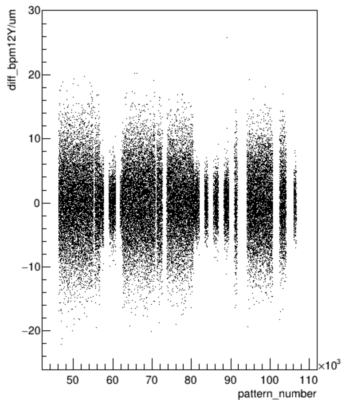
diff_bpm12Y/um:pattern_number {ErrorFlag==0}
