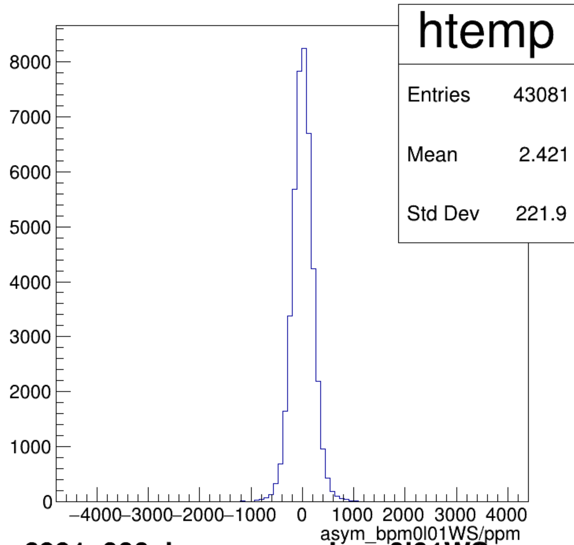
run6991_000_bpm_asym_bpm0l01WS.png
