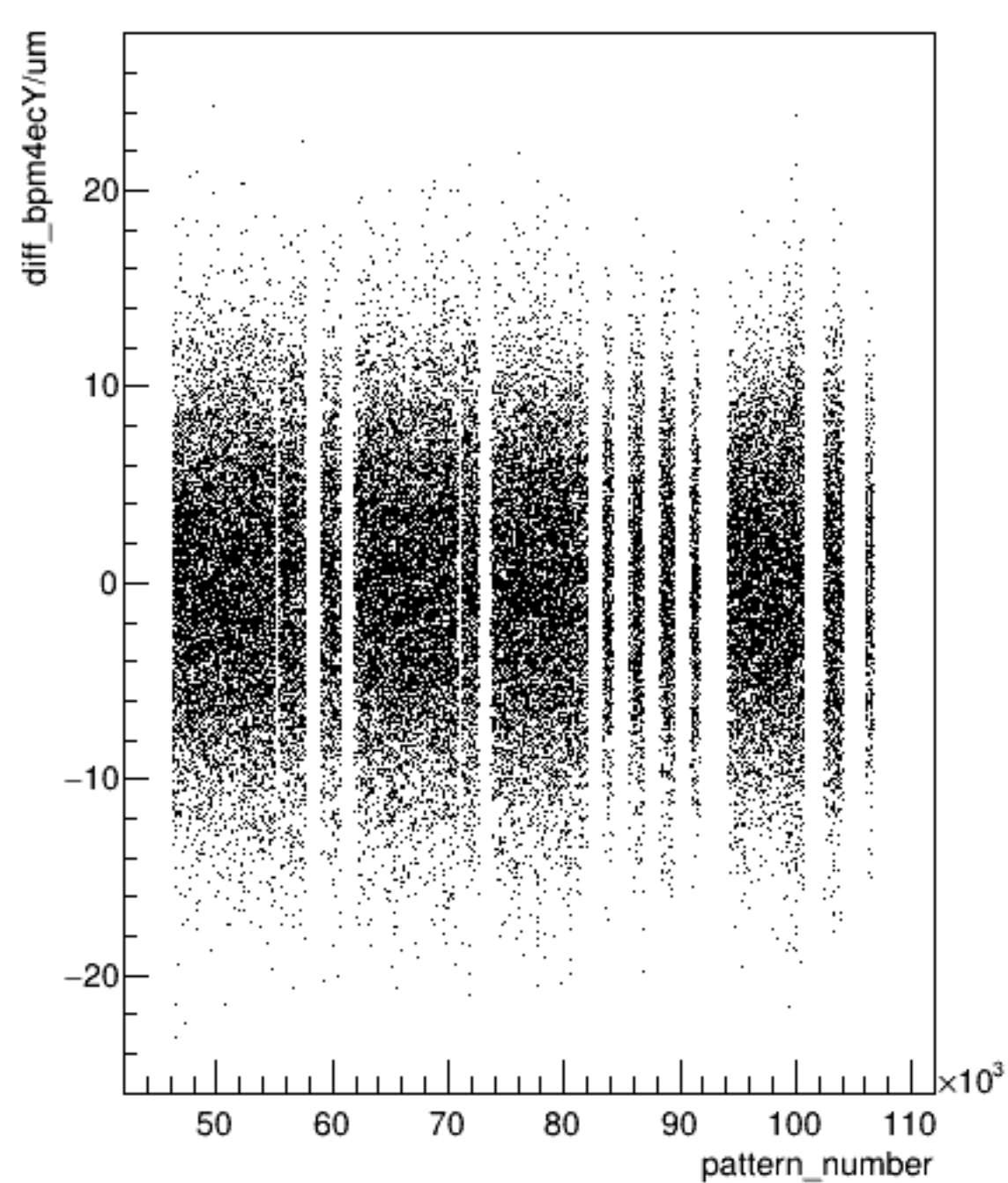
diff_bpm4ecY/um:pattern_number (ErrorFlag==0)
