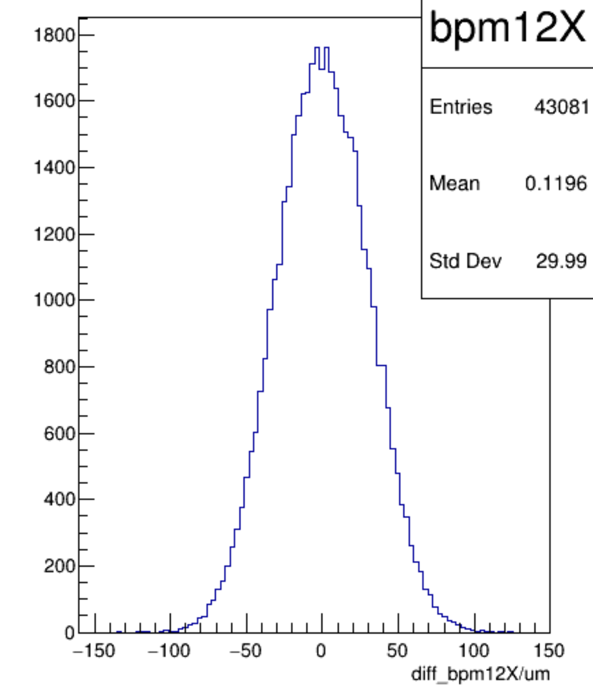
diff_bpm12X/um {ErrorFlag==0}
