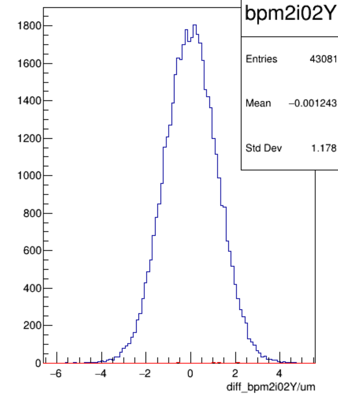
diff_bpm2i02Y/um {ErrorFlag==0}
