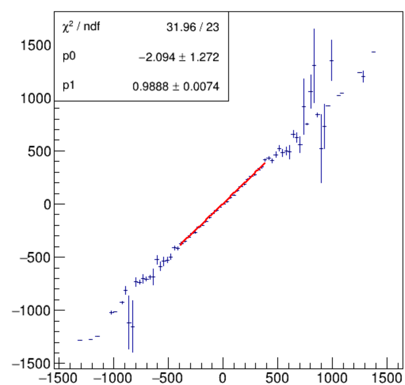
asym_bpm4ecWS/ppm:Aq/ppm {ErrorFlag==0}
