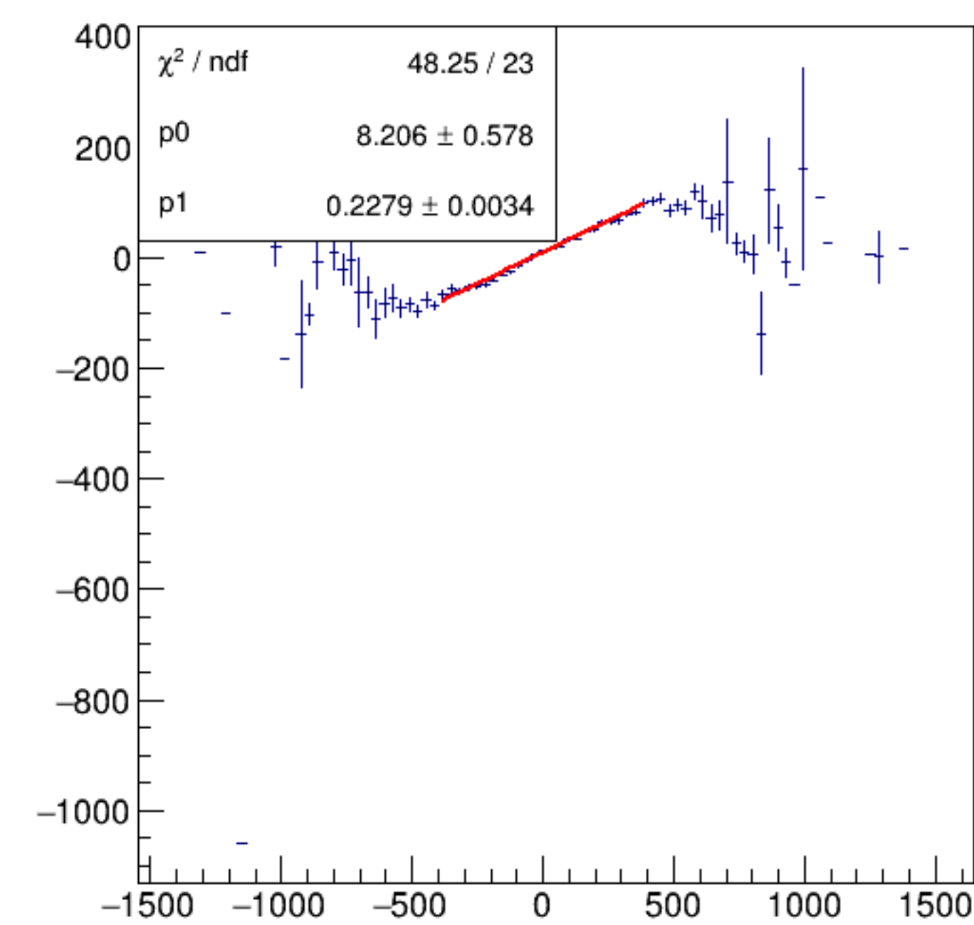
asym_bpm0i01aWS/ppm:Aq/ppm {ErrorFlag==0}
