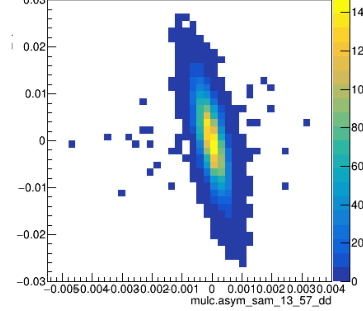
asym_sam_13_57_dd
