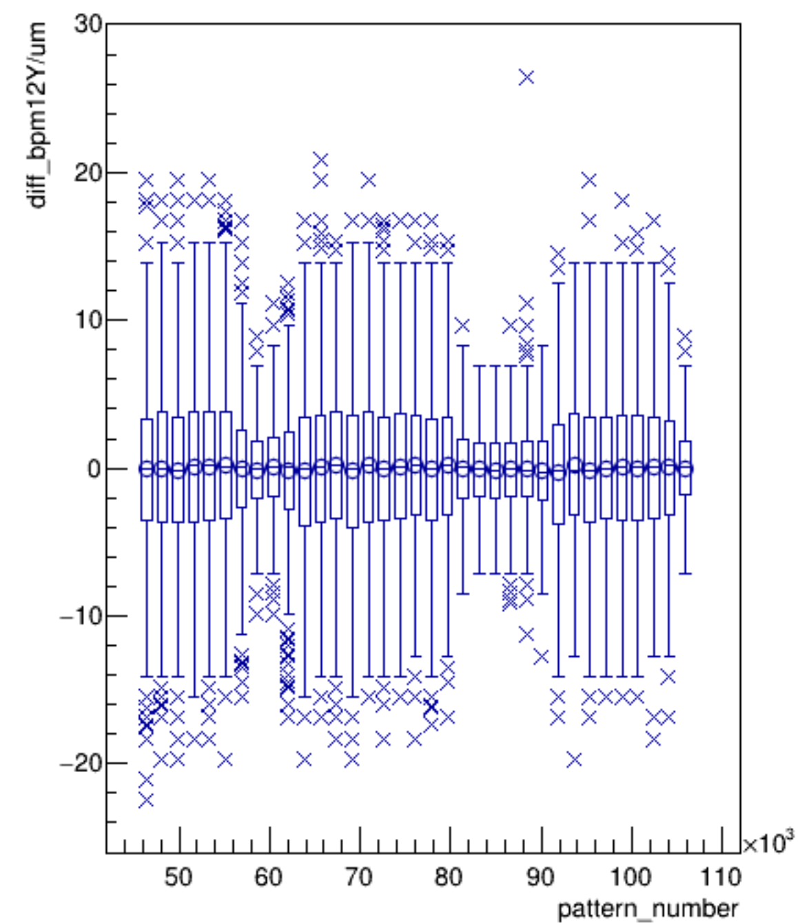
diff_bpm12Y/um:pattern_number {ErrorFlag==0}
