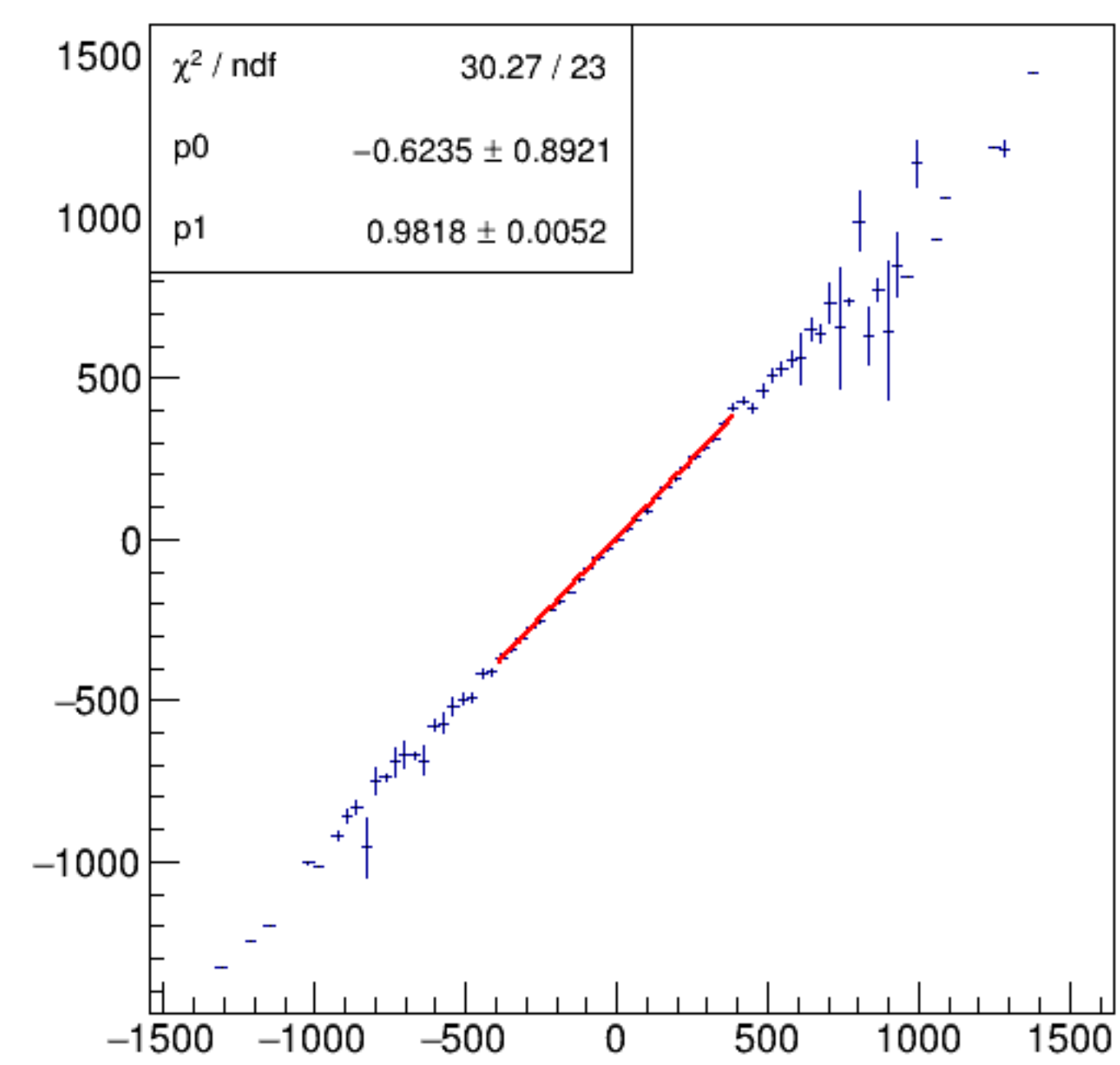
asym_bpm4eWS/ppm:Aq/ppm {ErrorFlag==0}
