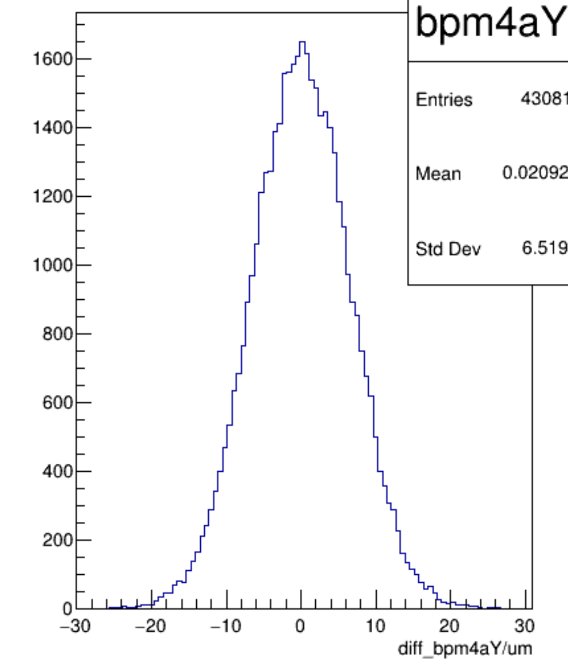
diff_bpm4aY/um {ErrorFlag==0}
