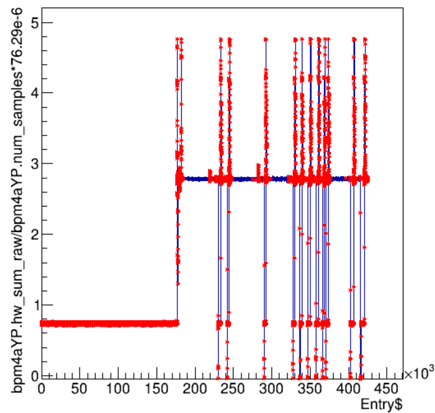
bpm4aYP.hw_sum_raw/bpm4aYP.num_samples*76.29e-6:Entry$
