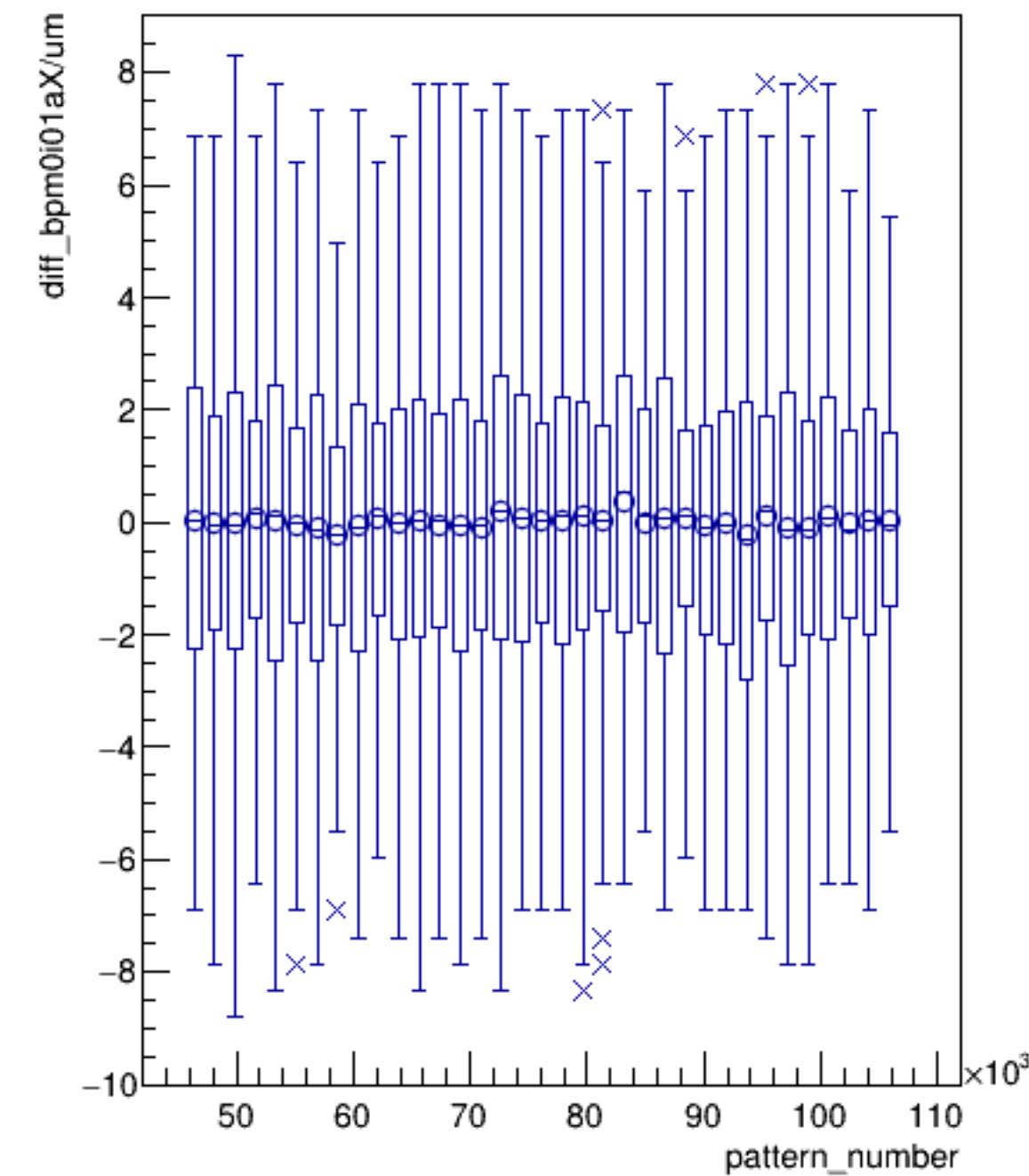
diff_bpm0i01aX/um:pattern_number (ErrorFlag==0)
