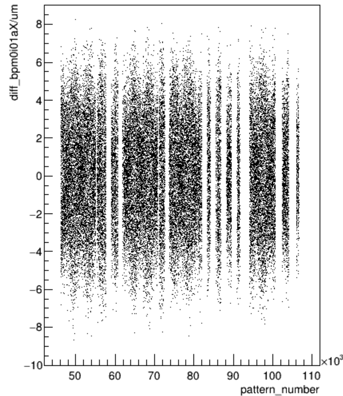
diff_bpm0i01aX/um:pattern_number (ErrorFlag==0)
