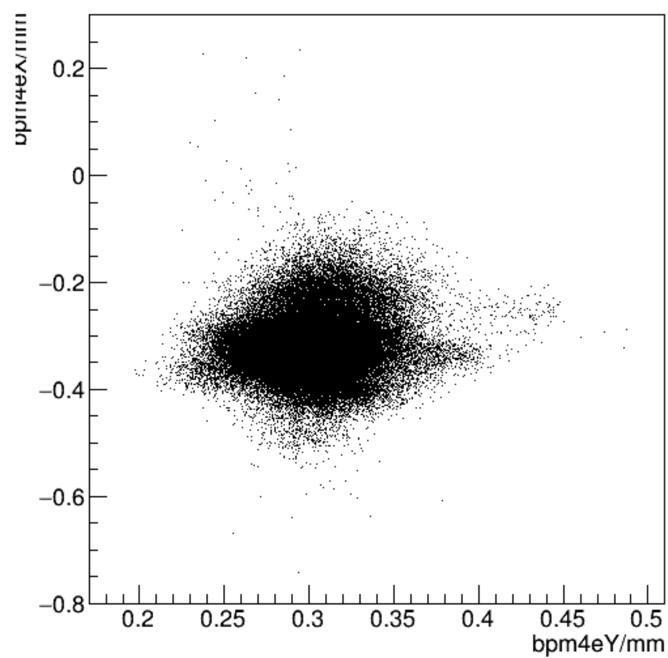
bpm4eX/mm:bpm4eY/mm {ErrorFlag==0}
