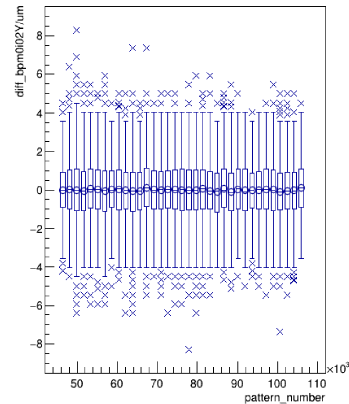
diff_bpm0i02Y/um:pattern_number (ErrorFlag==0)
