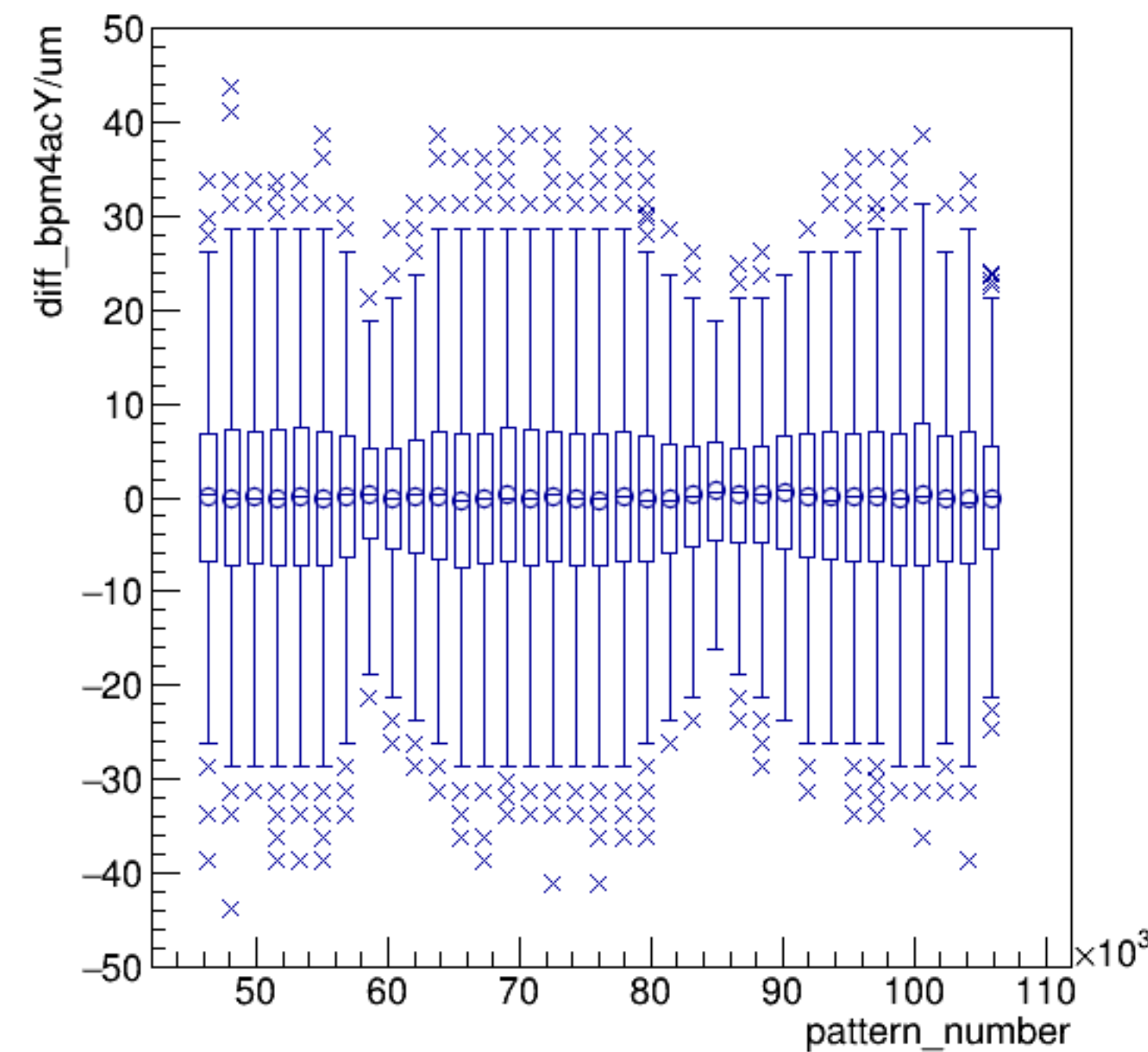
diff_bpm4acY/um:pattern_number {ErrorFlag==0}
