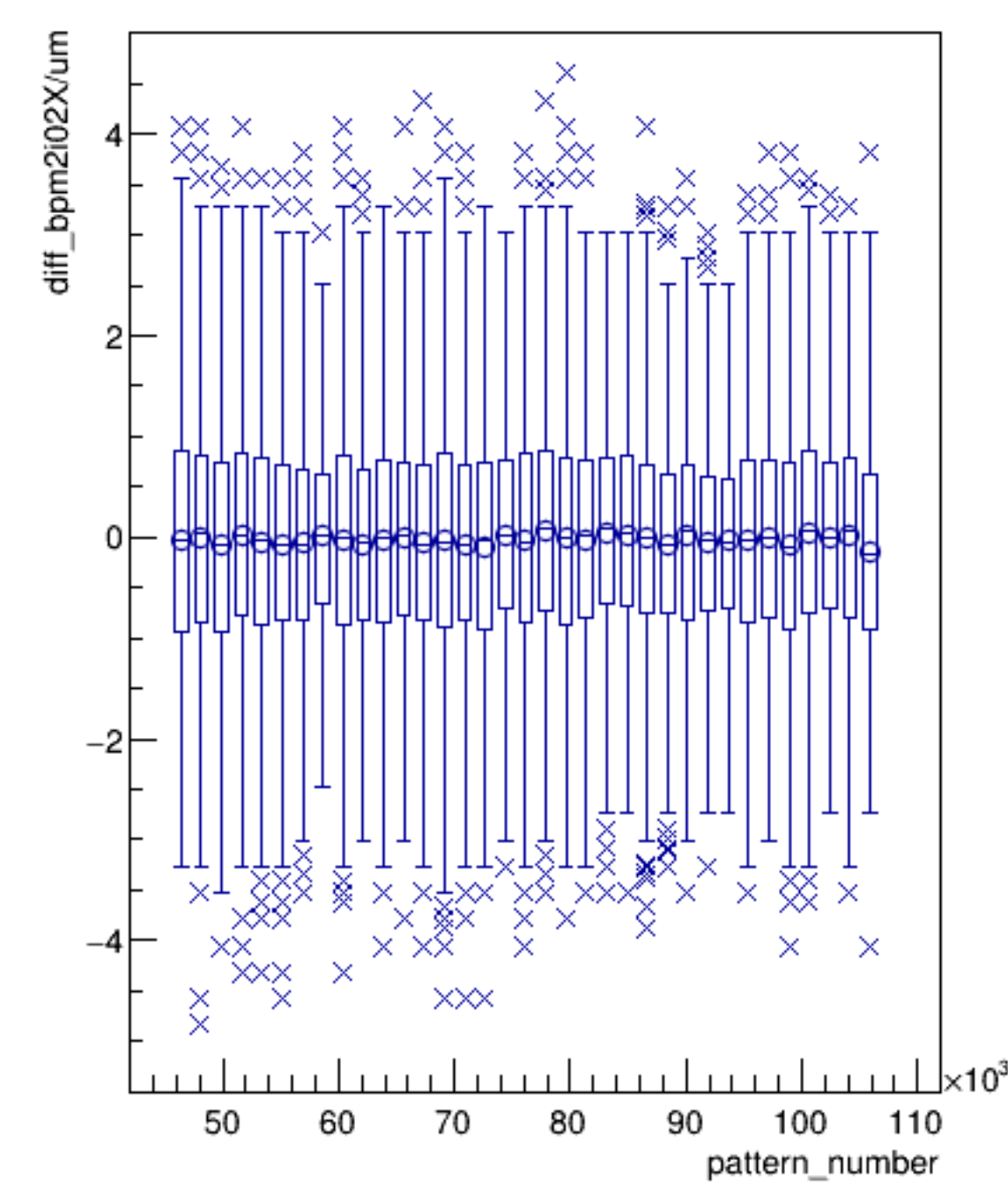
diff_bpm2i02X/um:pattern_number (ErrorFlag==0)
