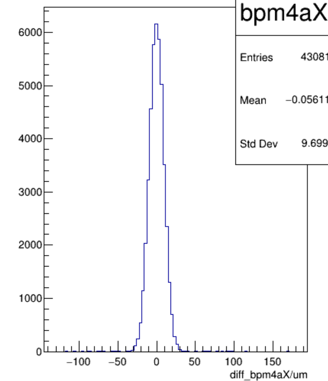
diff_bpm4aX/um {ErrorFlag==0}
