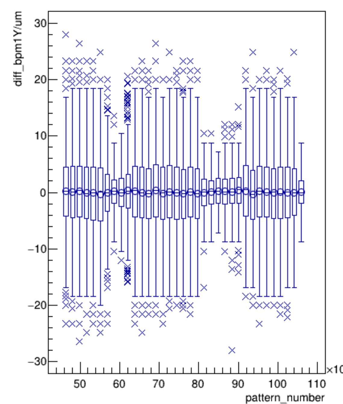
diff_bpm1Y/um:pattern_number {ErrorFlag==0}
