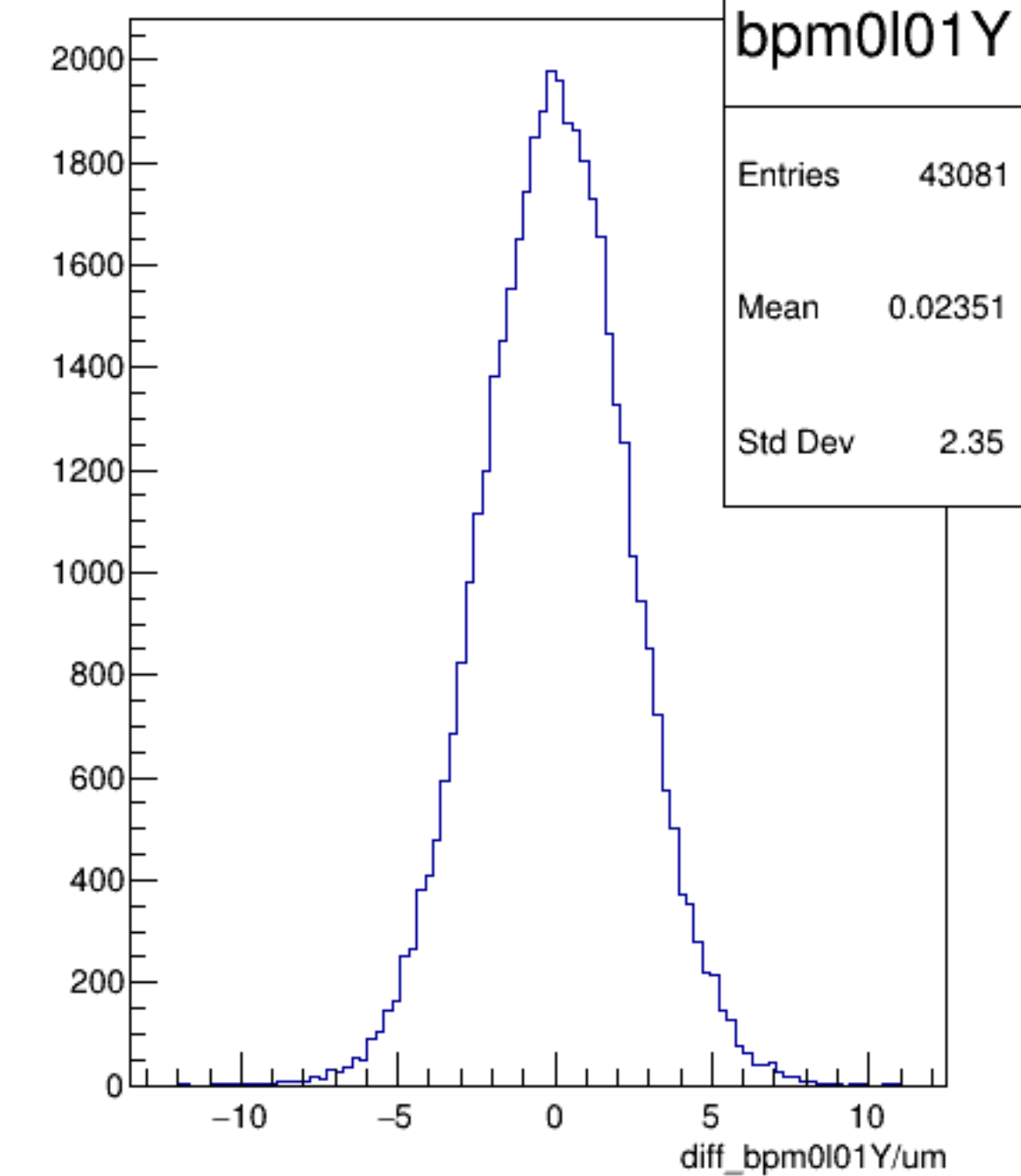
diff_bpm0l01Y/um {ErrorFlag==0}
