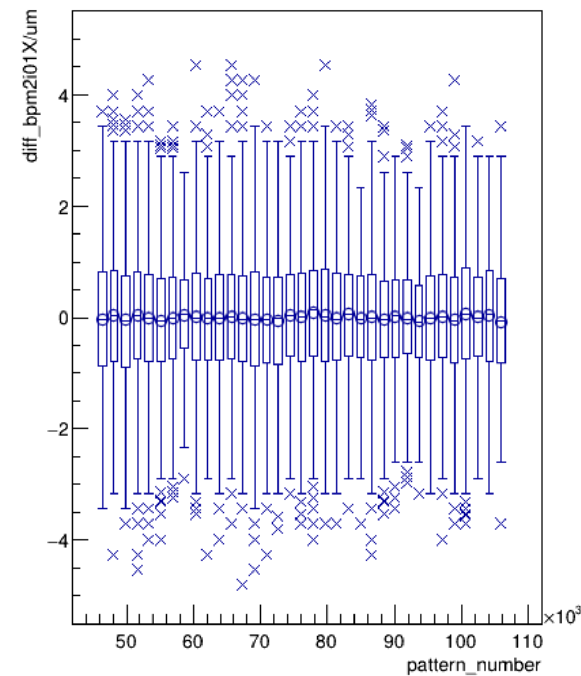
diff_bpm2i01X/um:pattern_number (ErrorFlag==0)
