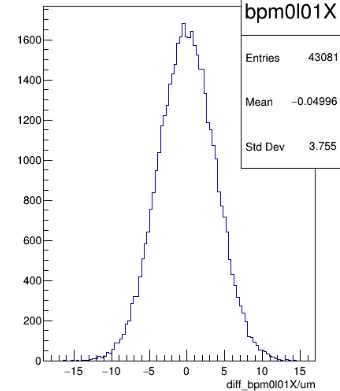
diff_bpm0l01X/um {ErrorFlag==0}
