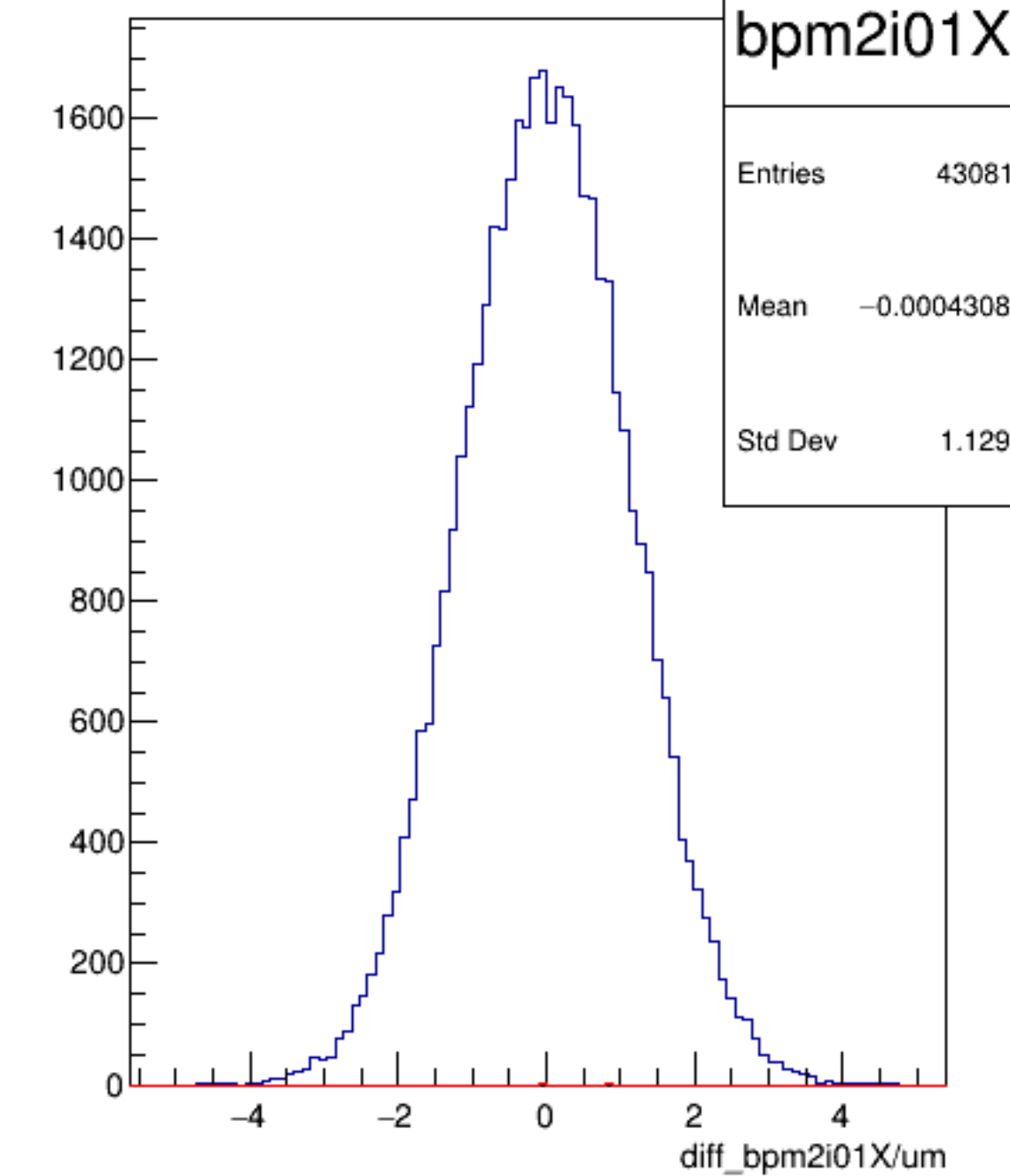
diff_bpm2i01X/um {ErrorFlag==0}
