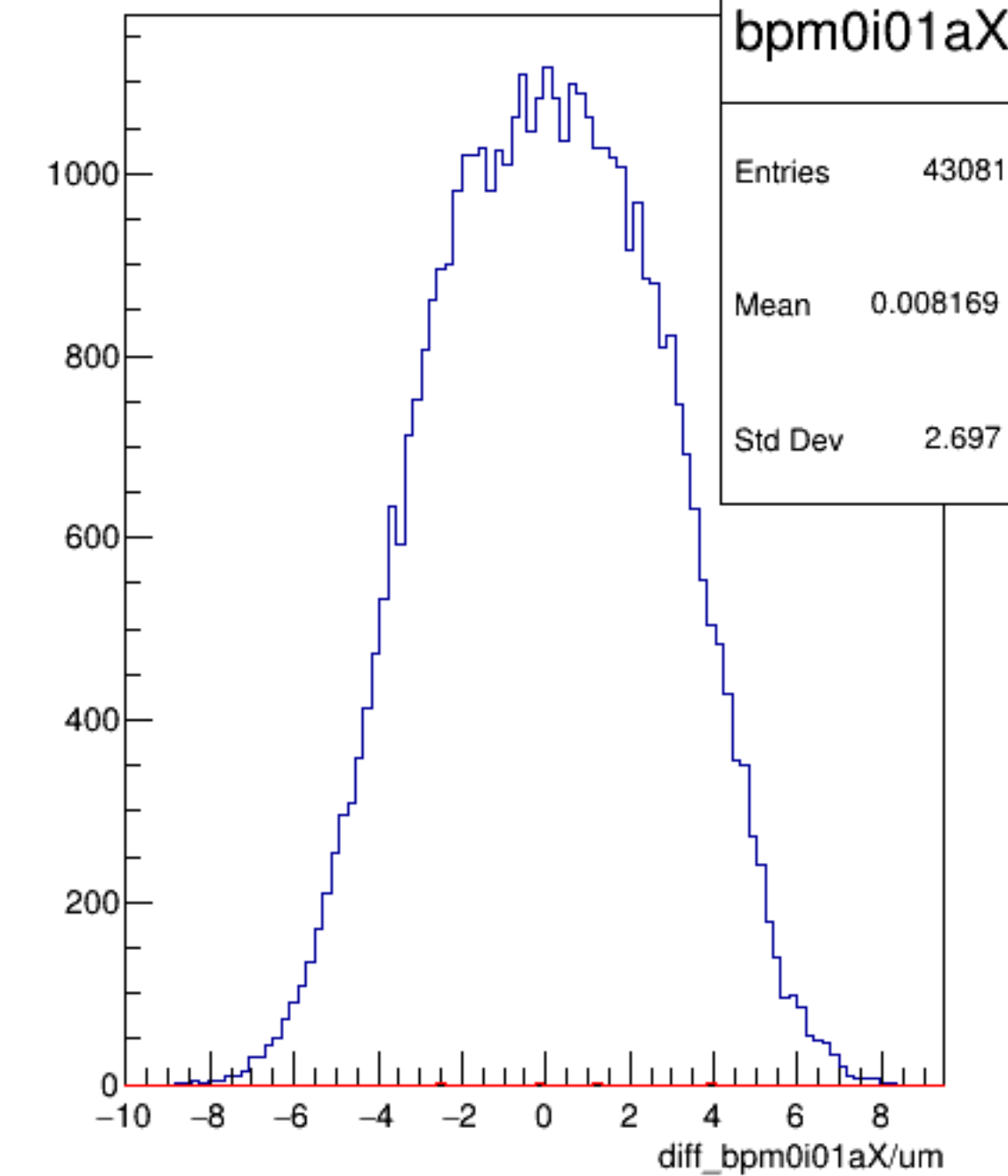
diff_bpm0i01aX/um {ErrorFlag==0}
