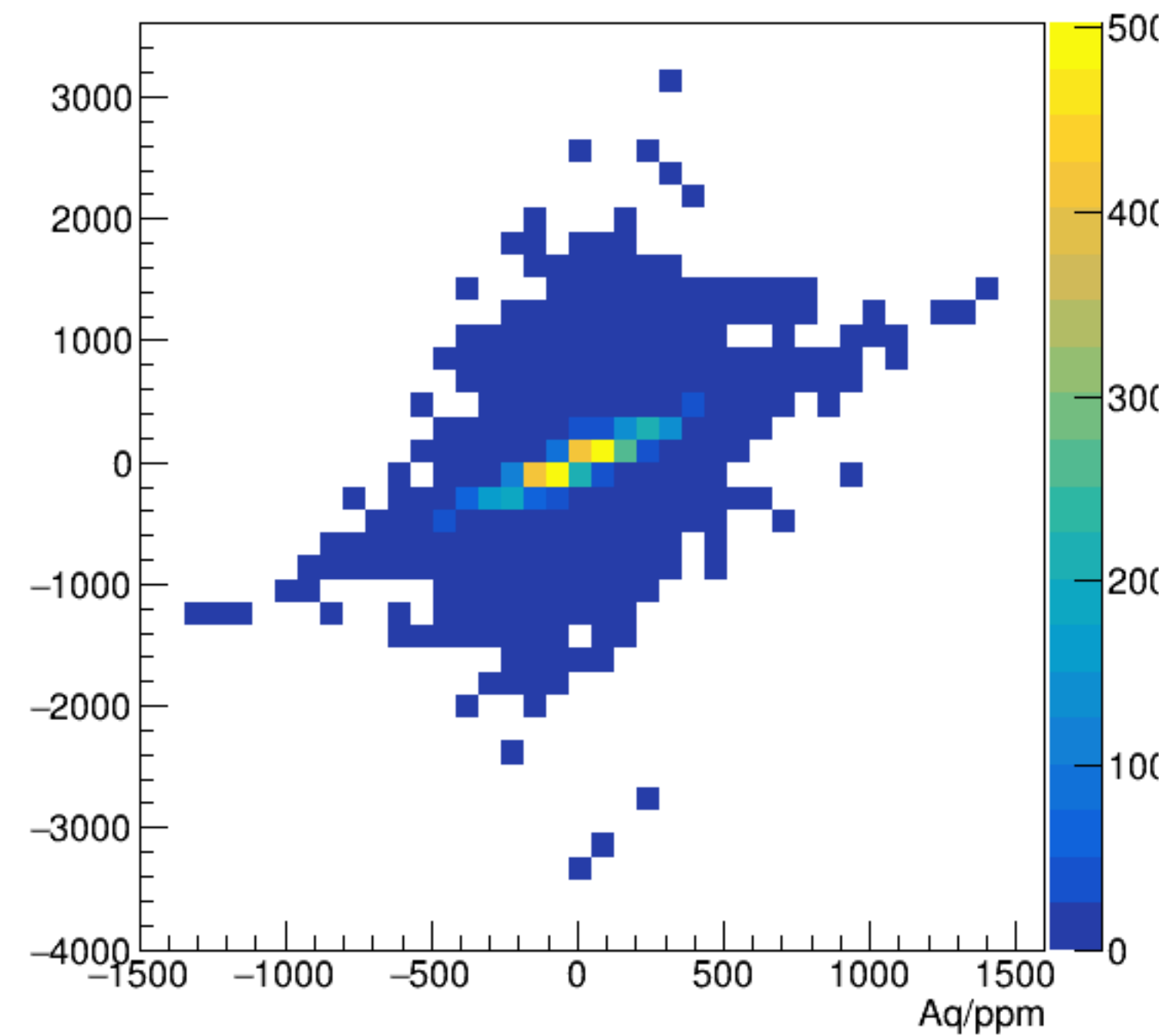
asym_bpm4eWS/ppm:Aq/ppm {ErrorFlag==0}
