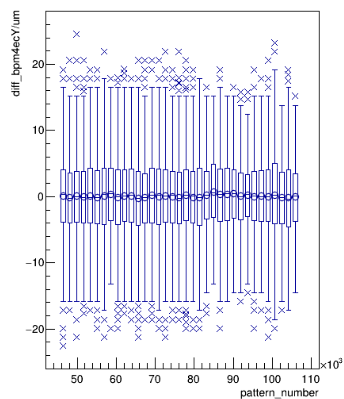
diff_bpm4ecY/um:pattern_number (ErrorFlag==0)
