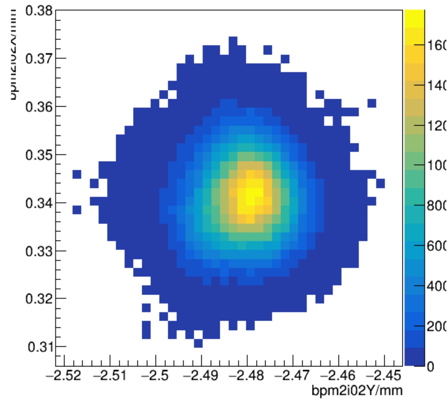
bpm2i02X/mm:bpm2i02Y/mm {ErrorFlag==0}
