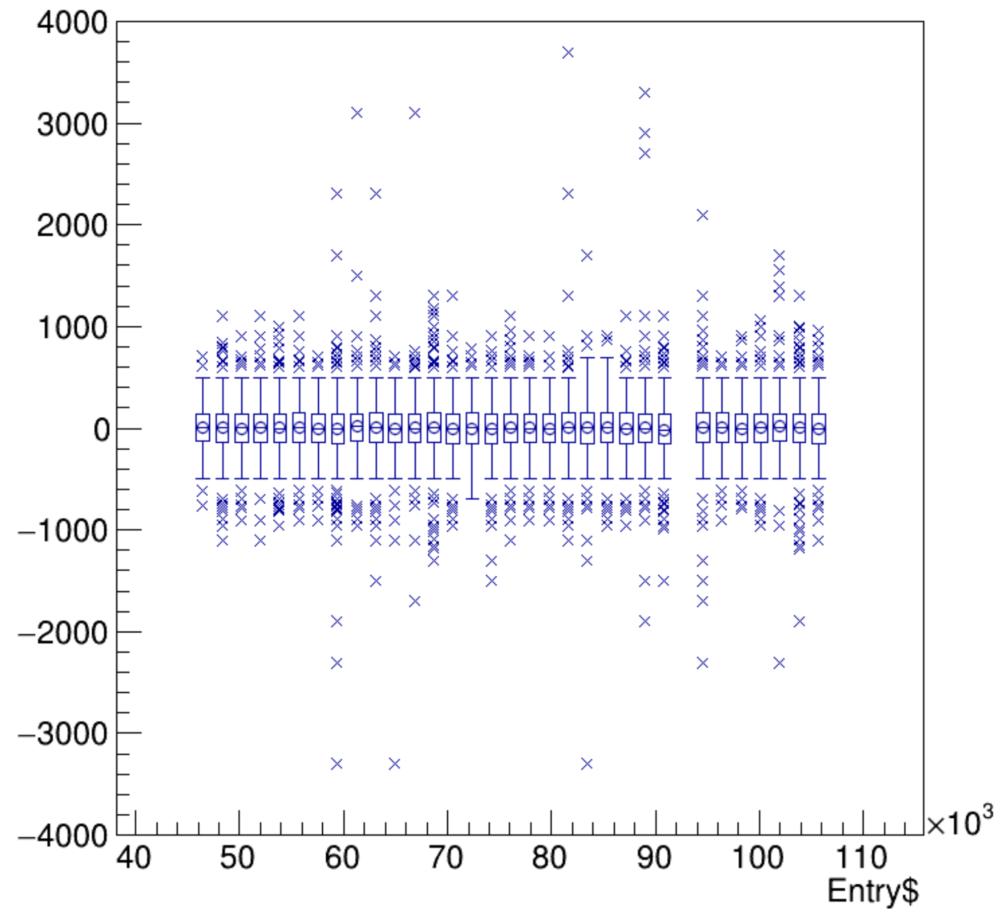
asym_bpm0i07WS/ppm:Entry$ {ErrorFlag==0}
