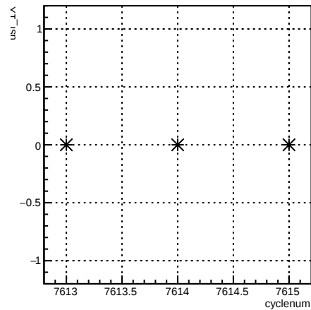
usr_4eY:cyclenum {run == 6994}
