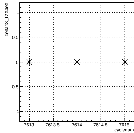
delta13_12X4eX:cyclenum {run == 6994}
