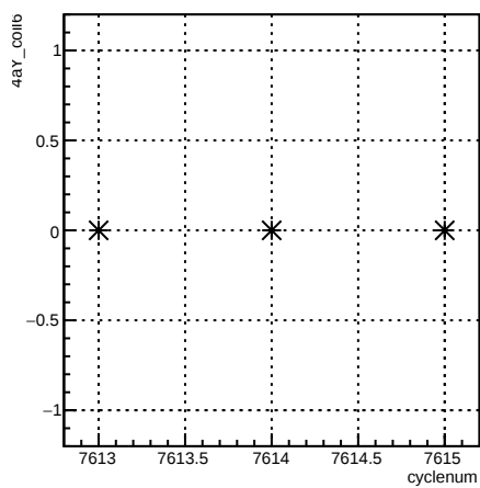
4aY_coil6:cyclenum {run == 6994}
