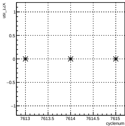
usl_12X:cyclenum {run == 6994}
