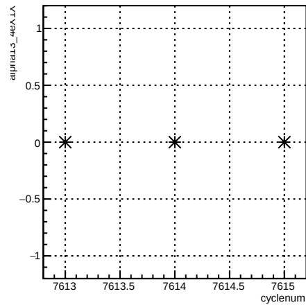
alpha13_4eX1X:cyclenum {run == 6994}
