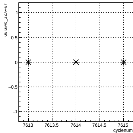
delta46_12X4eY:cyclenum {run == 6994}
