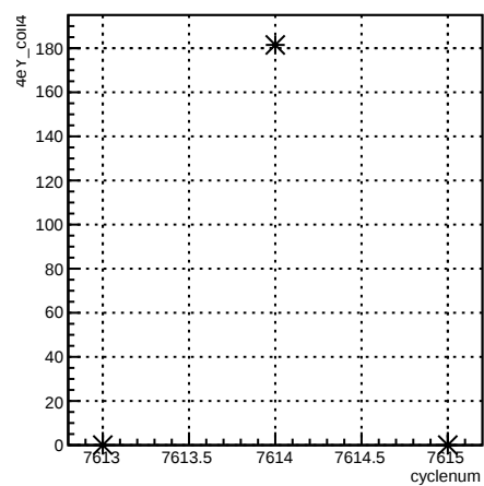
4eY_coil4:cyclenum {run == 6994}
