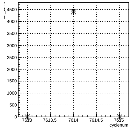
run:cyclenum {run == 6994}
