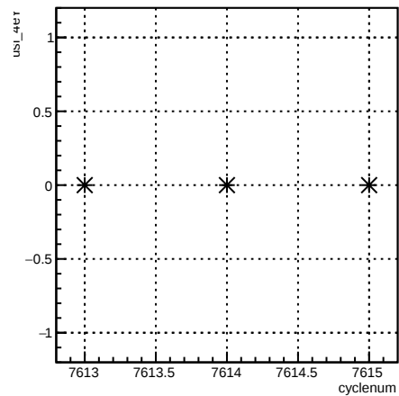
usl_4eY:cyclenum {run == 6994}
