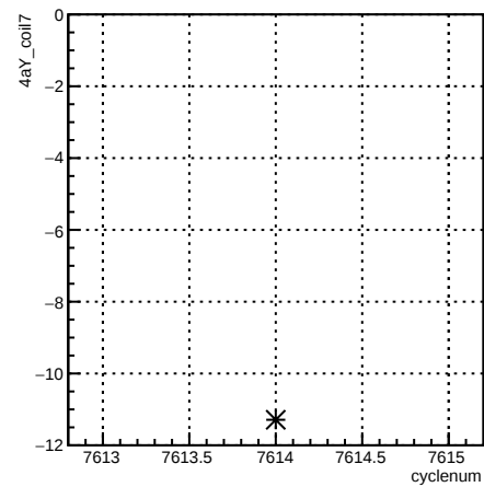
4aY_coil7:cyclenum {run == 6994}
