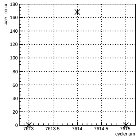
4aY_coil4:cyclenum {run == 6994}
