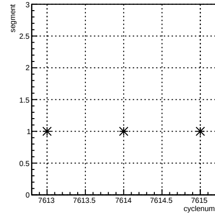
segment:cyclenum {run == 6994}
