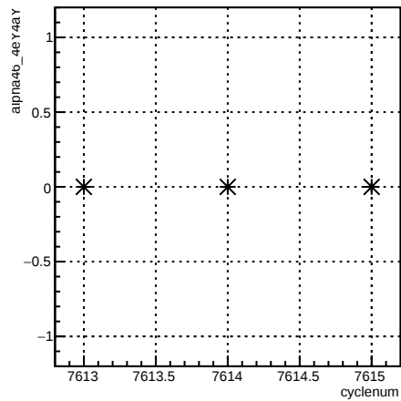
alpha46_4eY4aY:cyclenum {run == 6994}
