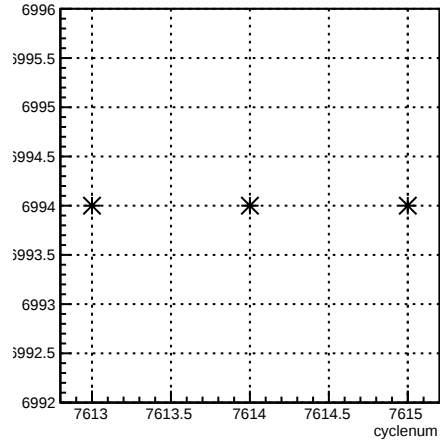
run:cyclenum {run == 6994}
