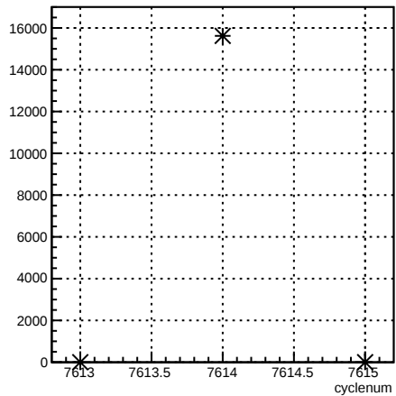
usl_coil7:cyclenum {run == 6994}
