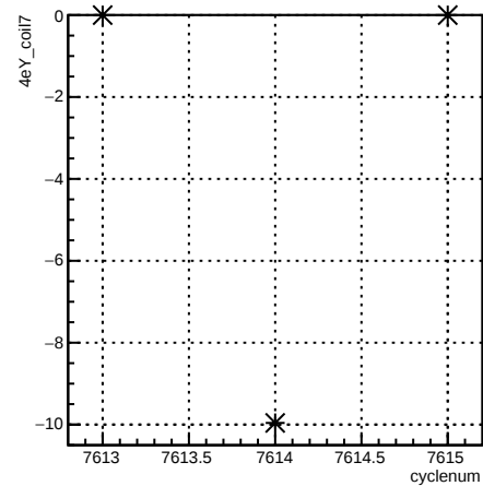
4eY_coil7:cyclenum {run == 6994}
