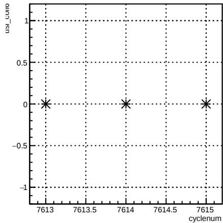
usl_coil6:cyclenum {run == 6994}
