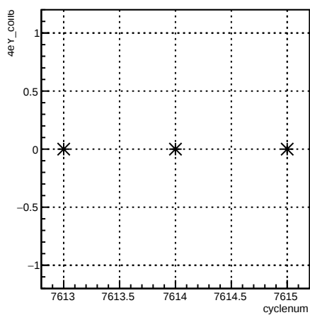
4eY_coil6:cyclenum {run == 6994}
