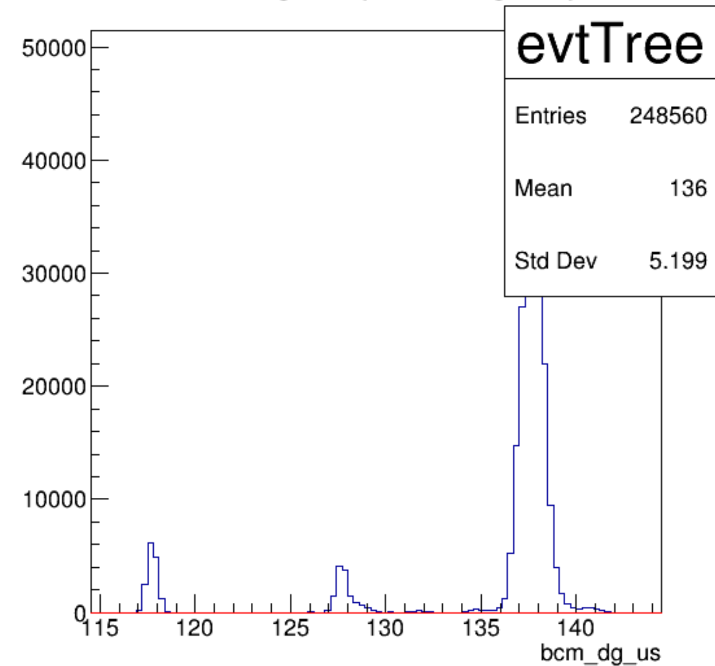
bcm_dg_us {ErrorFlag==0}
