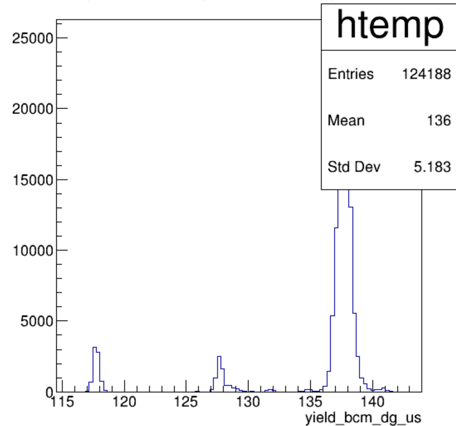
yield_bcm_dg_us {ErrorFlag==0}
