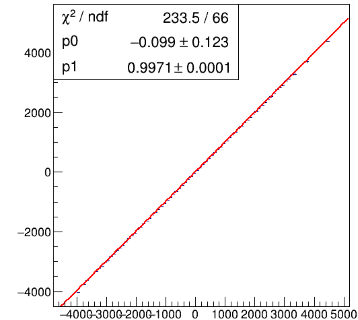
run6997_000_asym_bcm_an_us_vs_asym_bcm_an_ds3_pr.png
