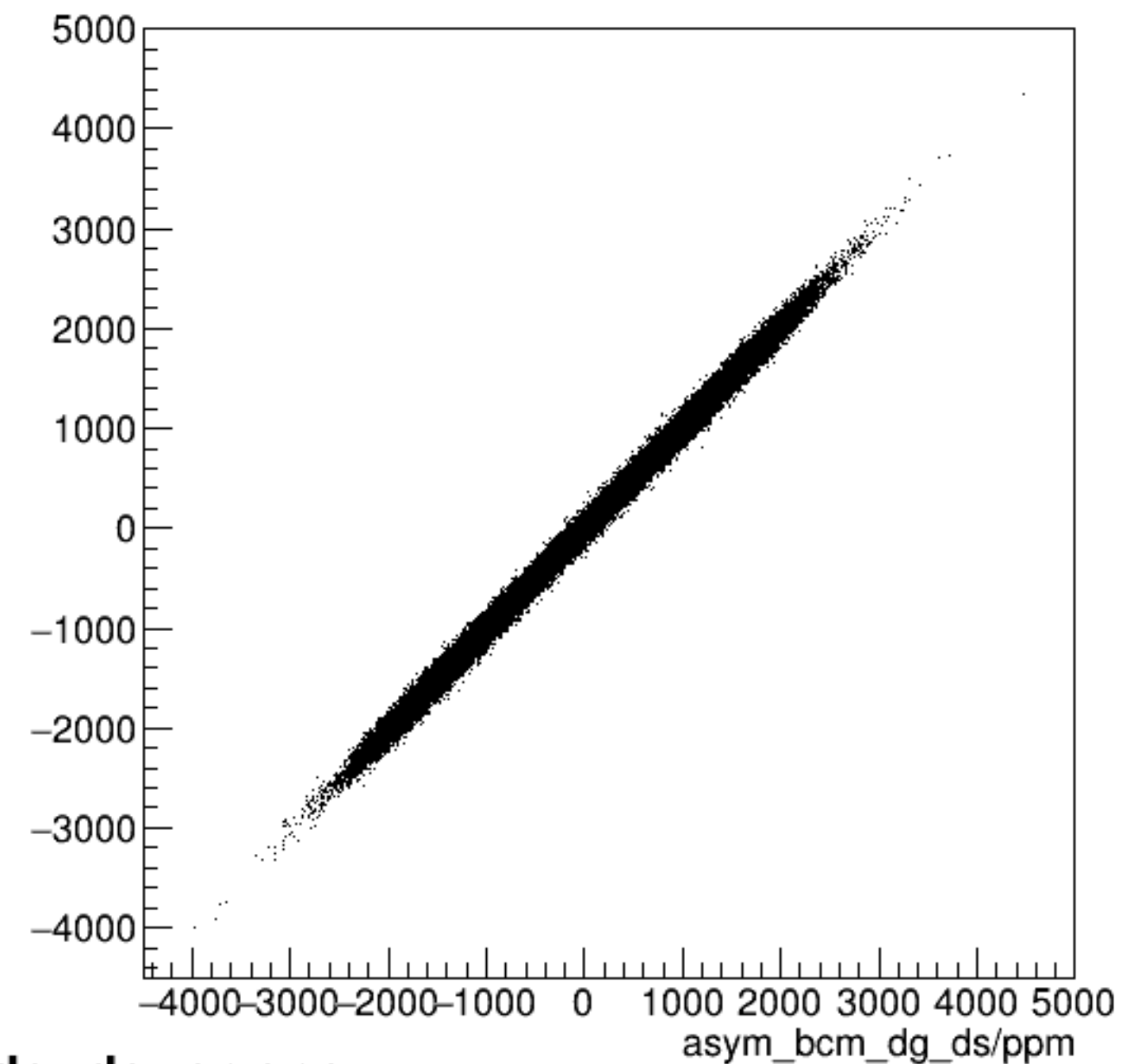
run6997_000_asym_bcm_dg_us_vs_asym_bcm_dg_ds_pr.png
