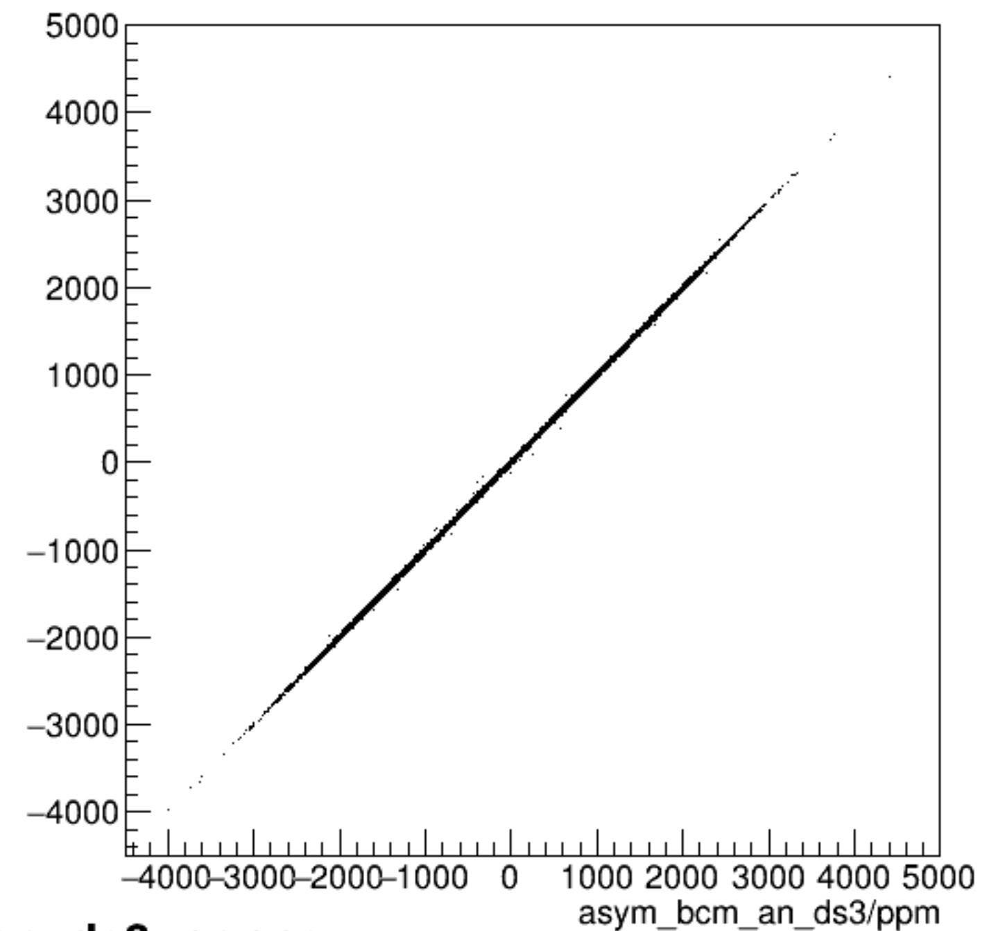
run6997_000_asym_bcm_an_ds_vs_asym_bcm_an_ds3_pr.png
