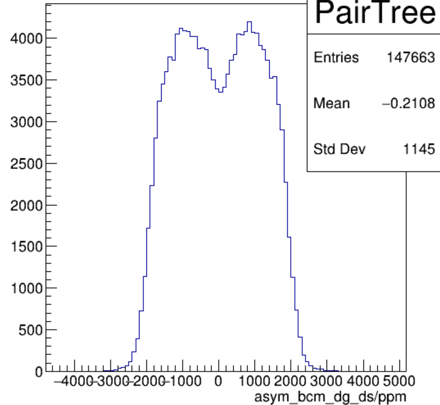
asym_bcm_dg_ds/ppm {ErrorFlag==0}
