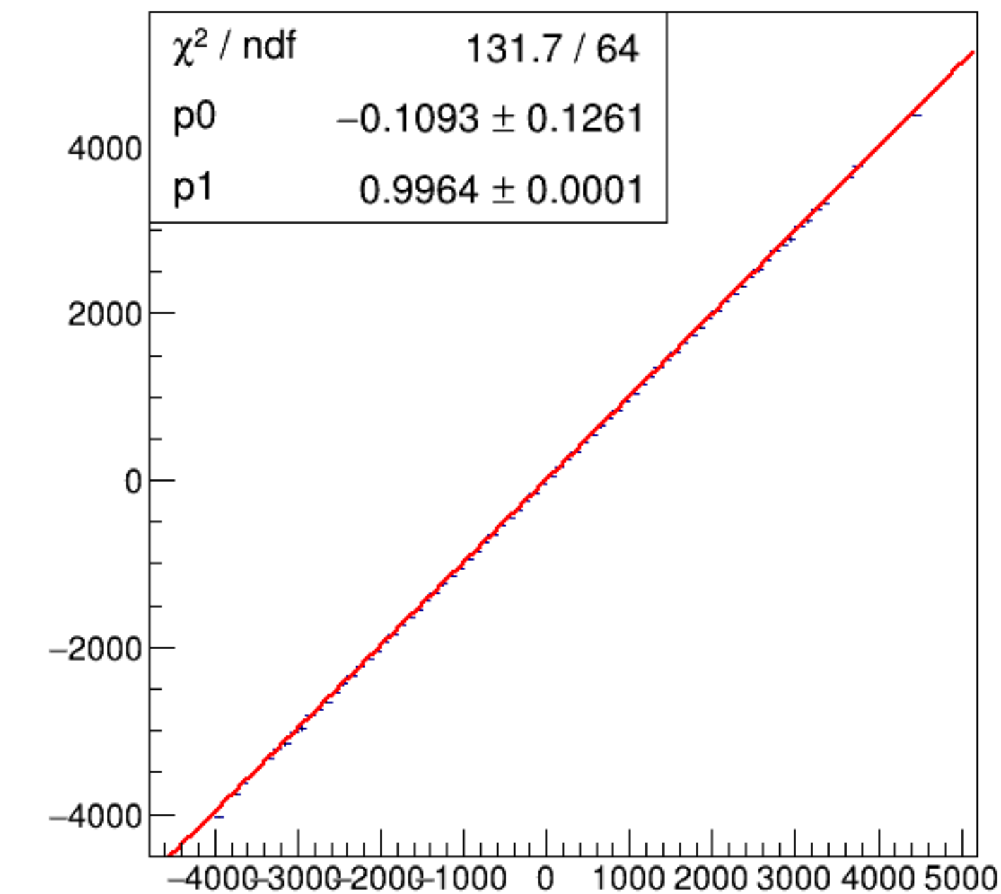
run6997_000_asym_bcm_an_us_vs_asym_bcm_an_ds_pr.png
