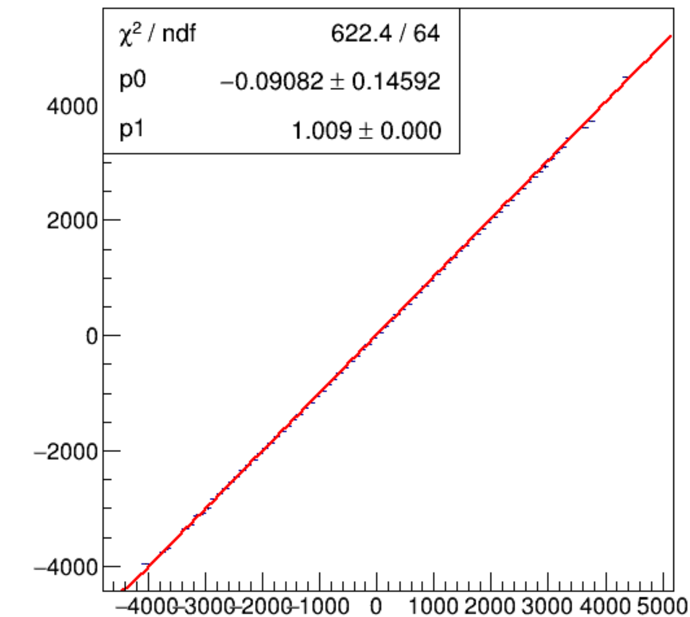
run6997_000_asym_bcm_dg_ds_vs_asym_bcm_an_us_pr.png
