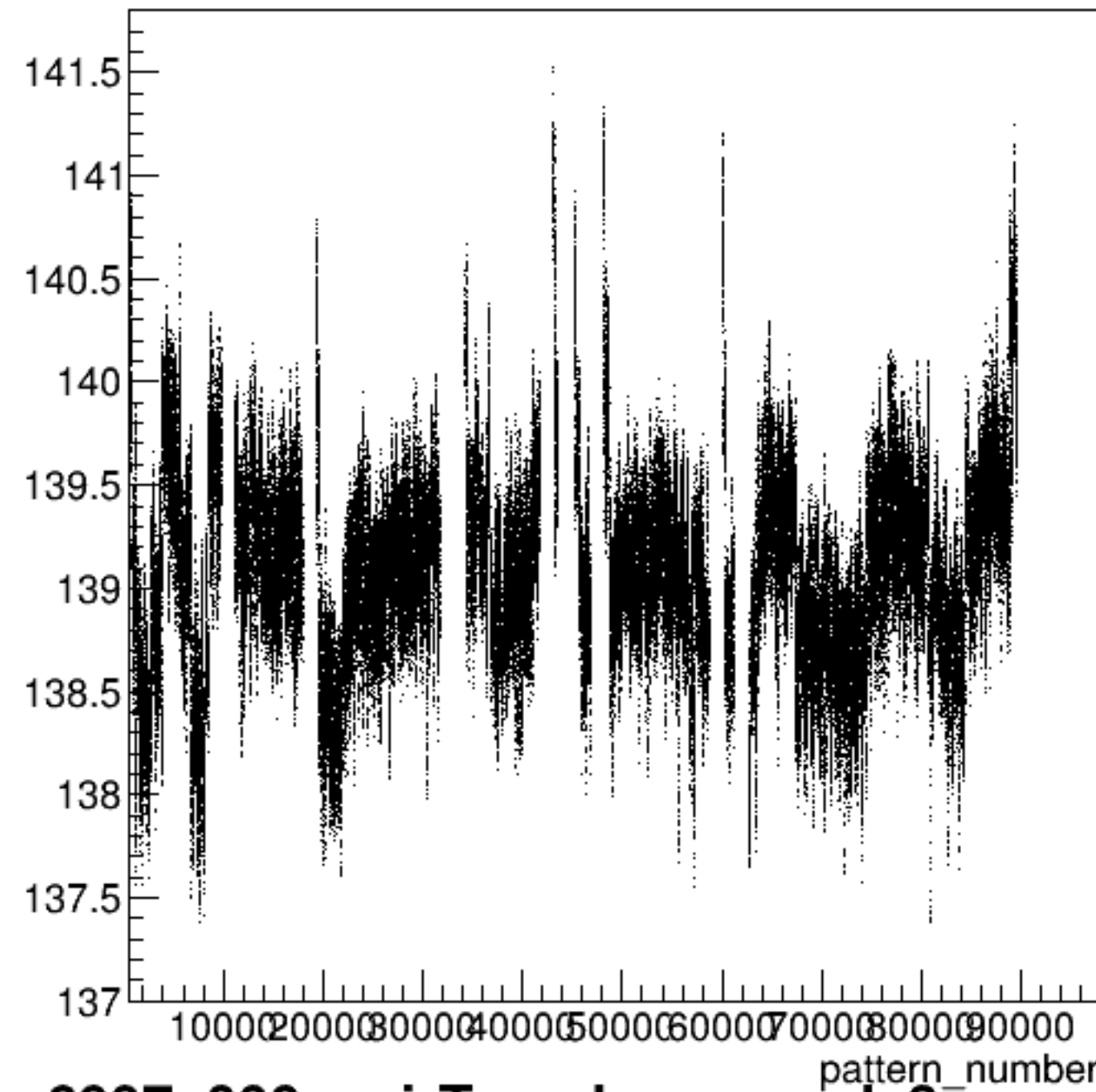
yield_bcm_an_ds3:pattern_number {ErrorFlag==0}
