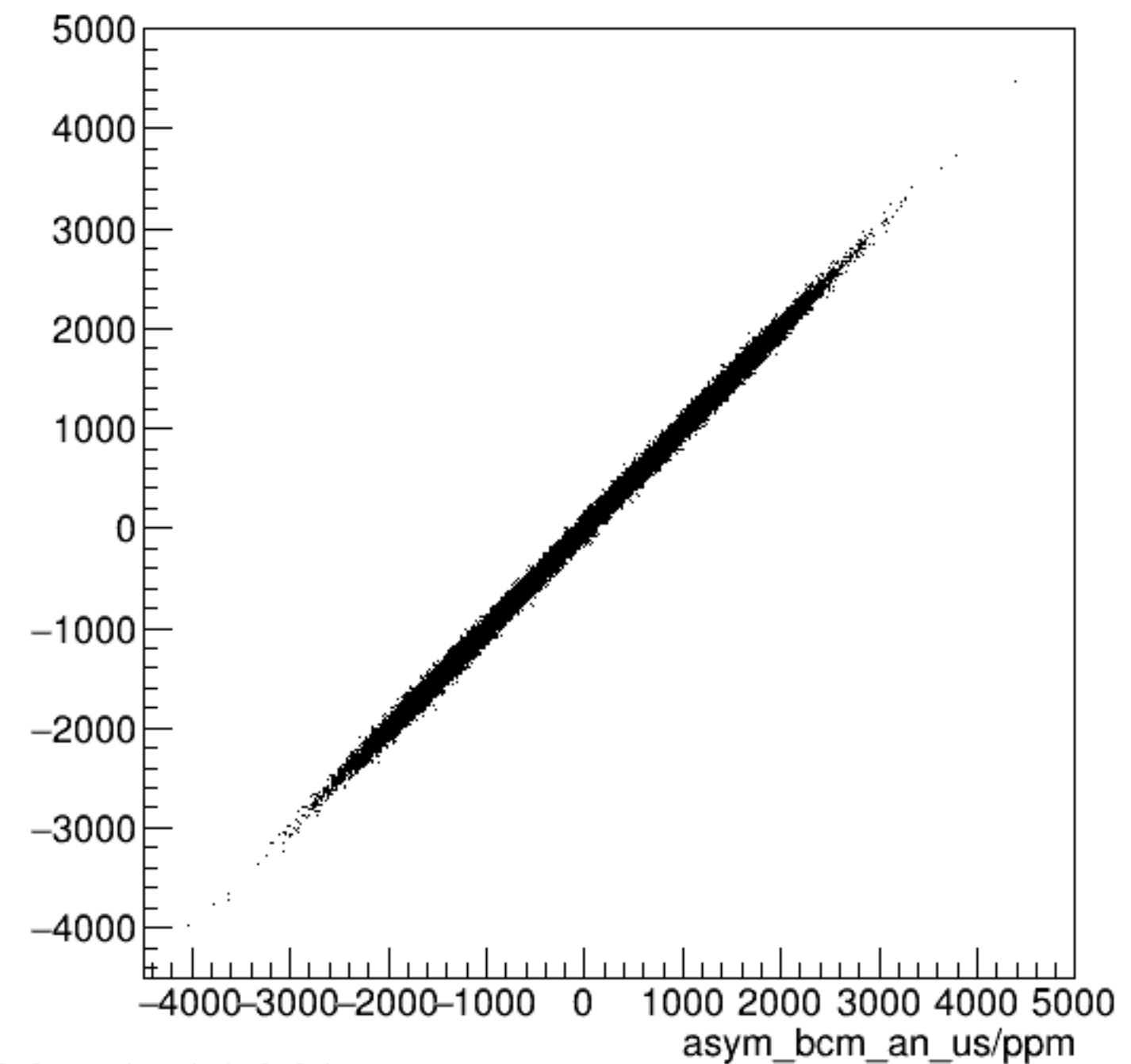
run6997_000_asym_bcm_dg_ds_vs_asym_bcm_an_us_pr.png
