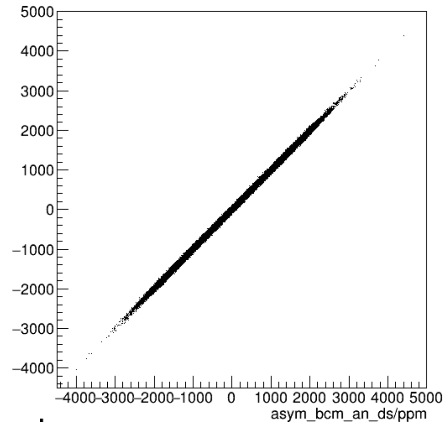
run6997_000_asym_bcm_an_us_vs_asym_bcm_an_ds_pr.png
