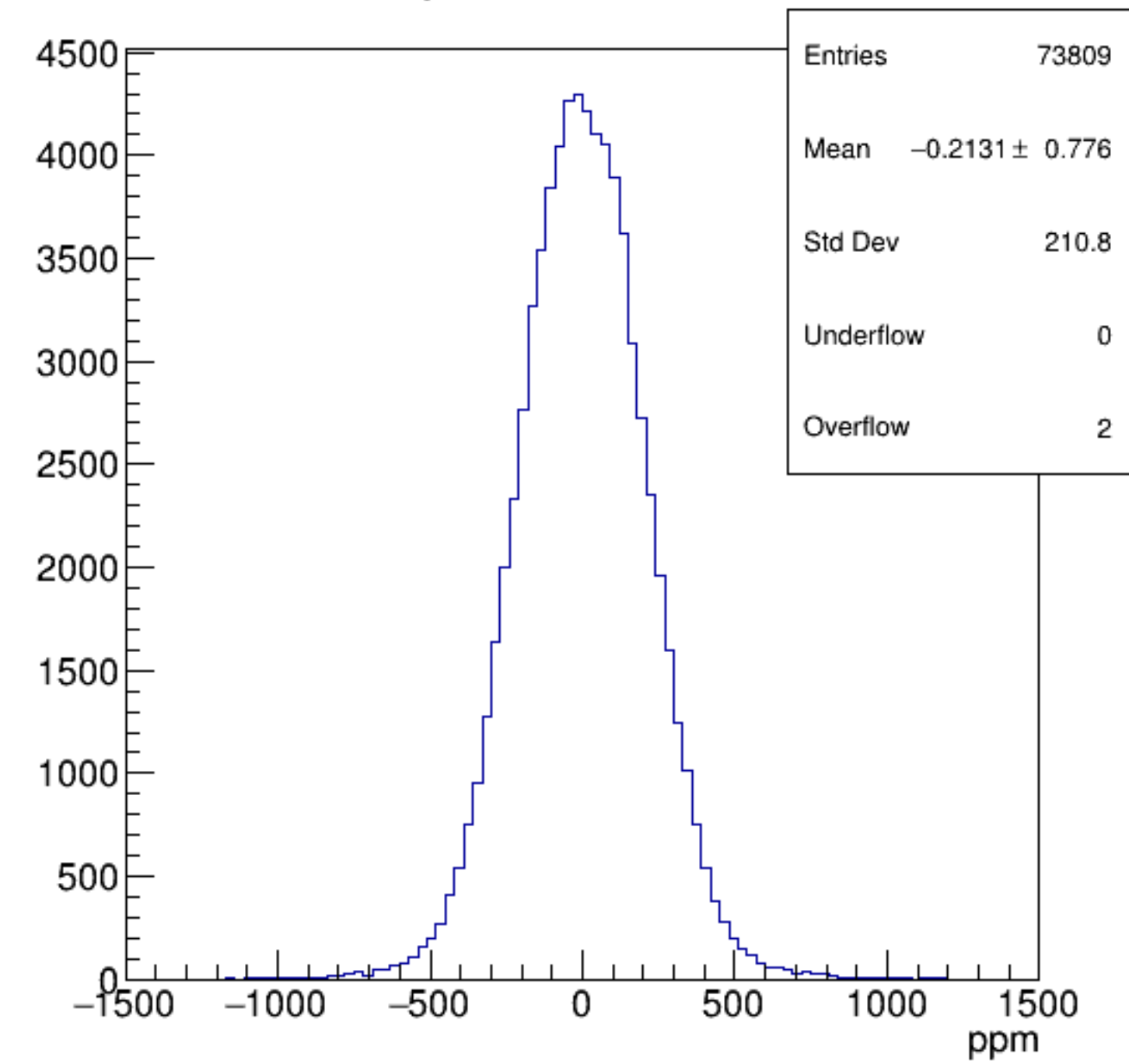
asym_bcm_an_us
