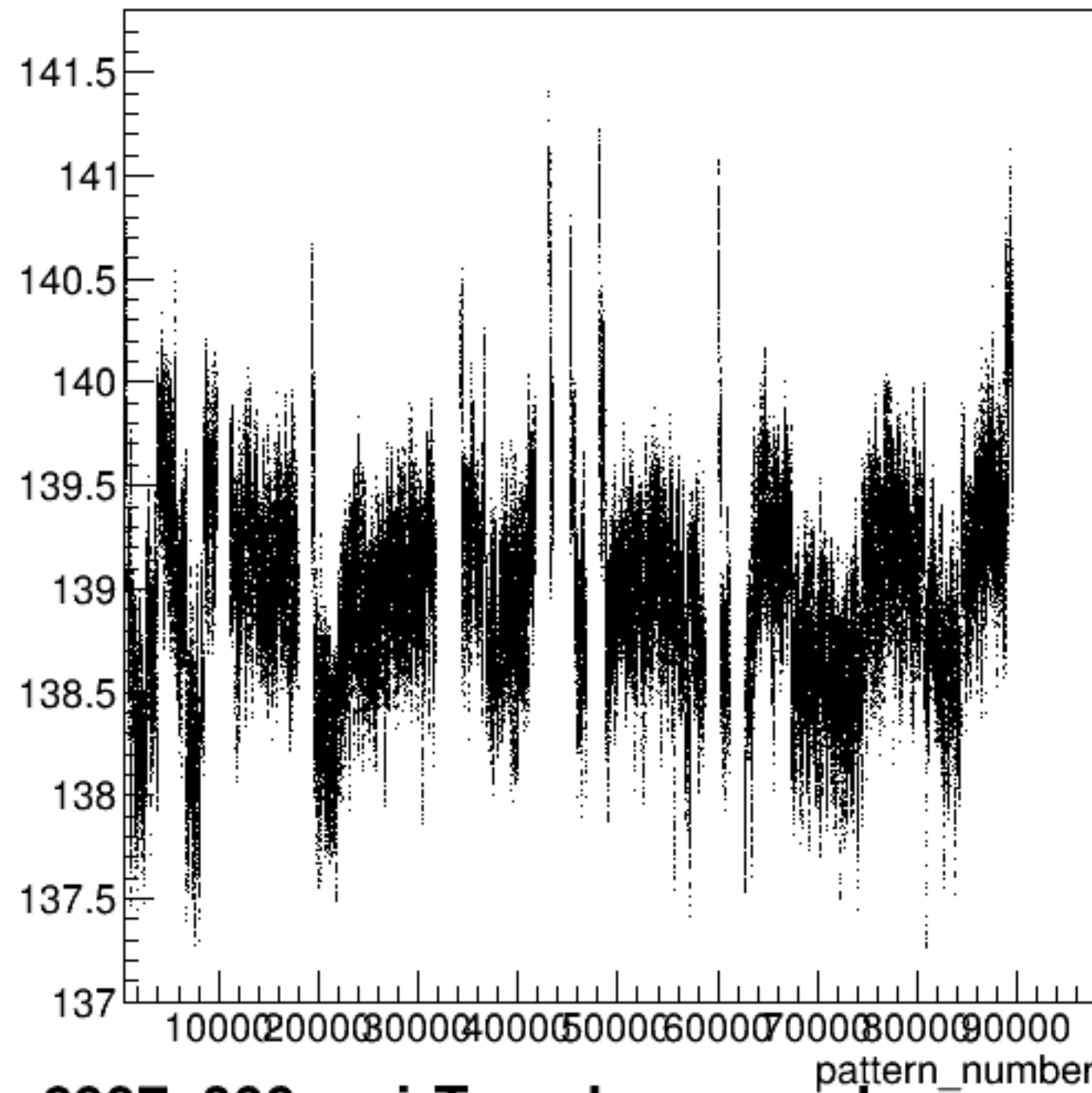
yield_bcm_an_ds:pattern_number {ErrorFlag==0}
