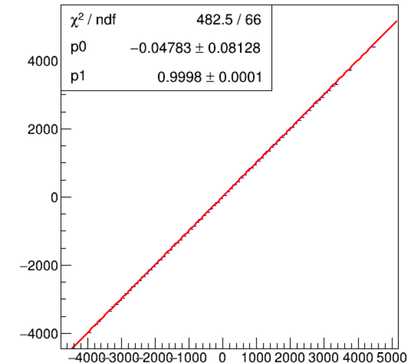
run6997_000_asym_bcm_an_ds_vs_asym_bcm_an_ds3_pr.png
