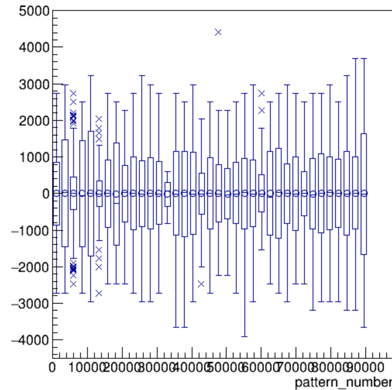
asym_bcm_an_ds/ppm:pattern_number {ErrorFlag==0}
