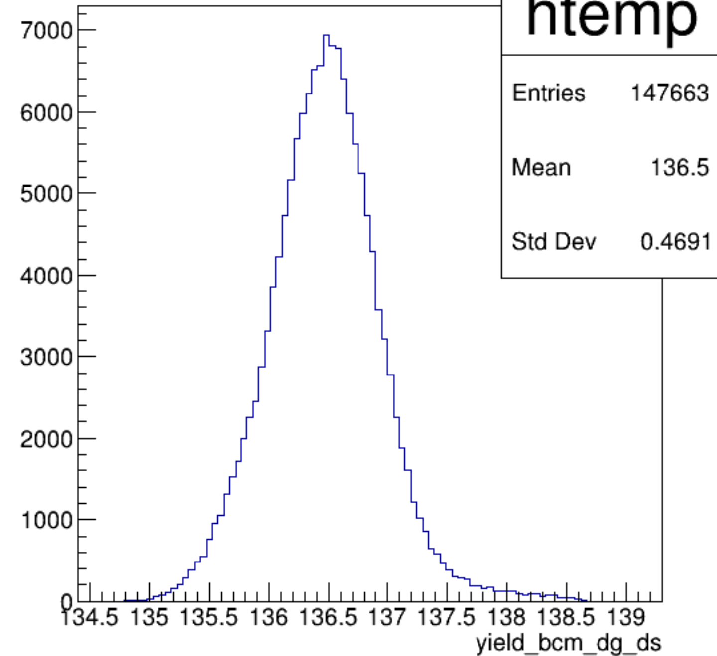
yield_bcm_dg_ds {ErrorFlag==0}
