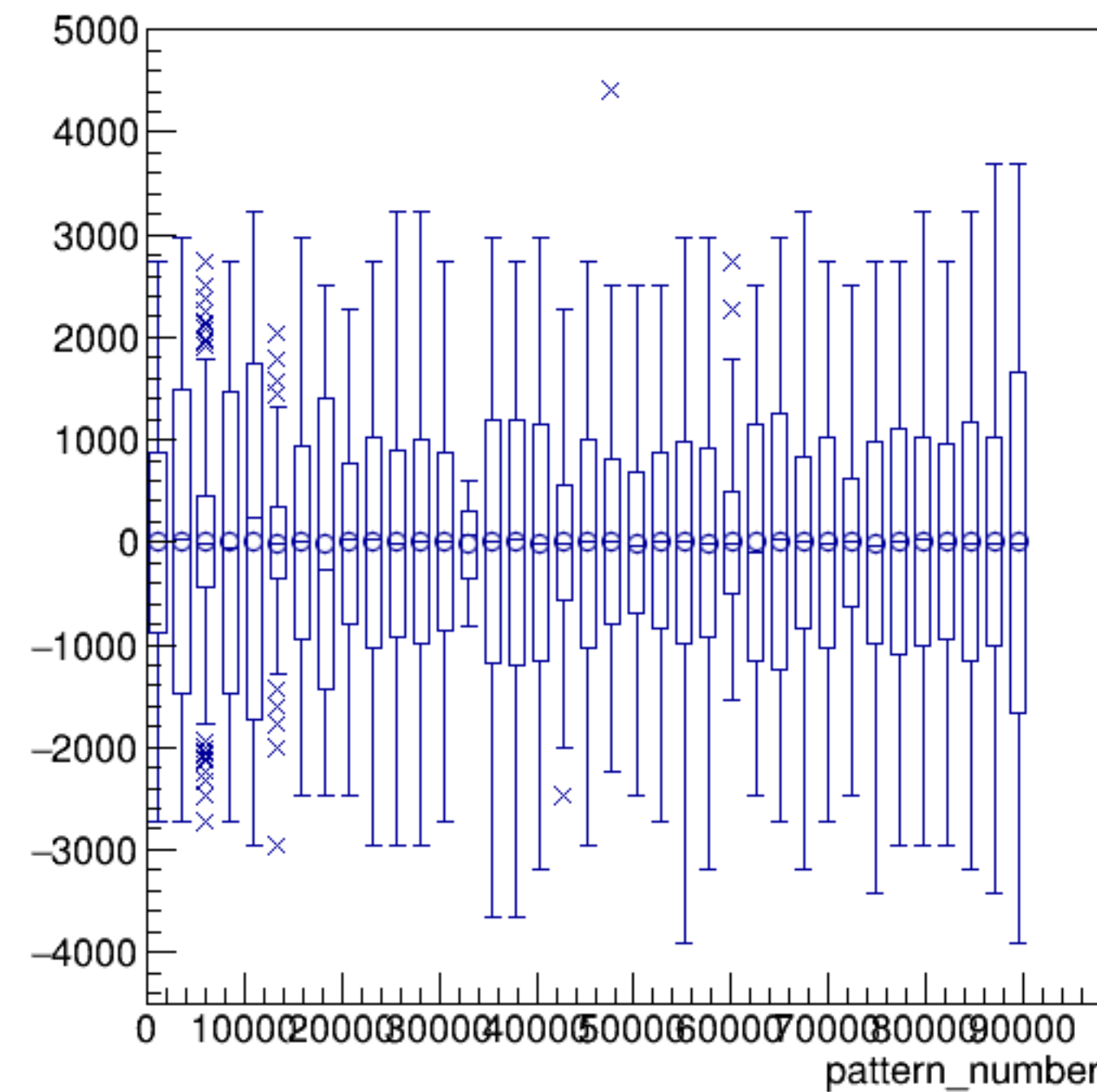
asym_bcm_dg_us/ppm:pattern_number {ErrorFlag==0}
