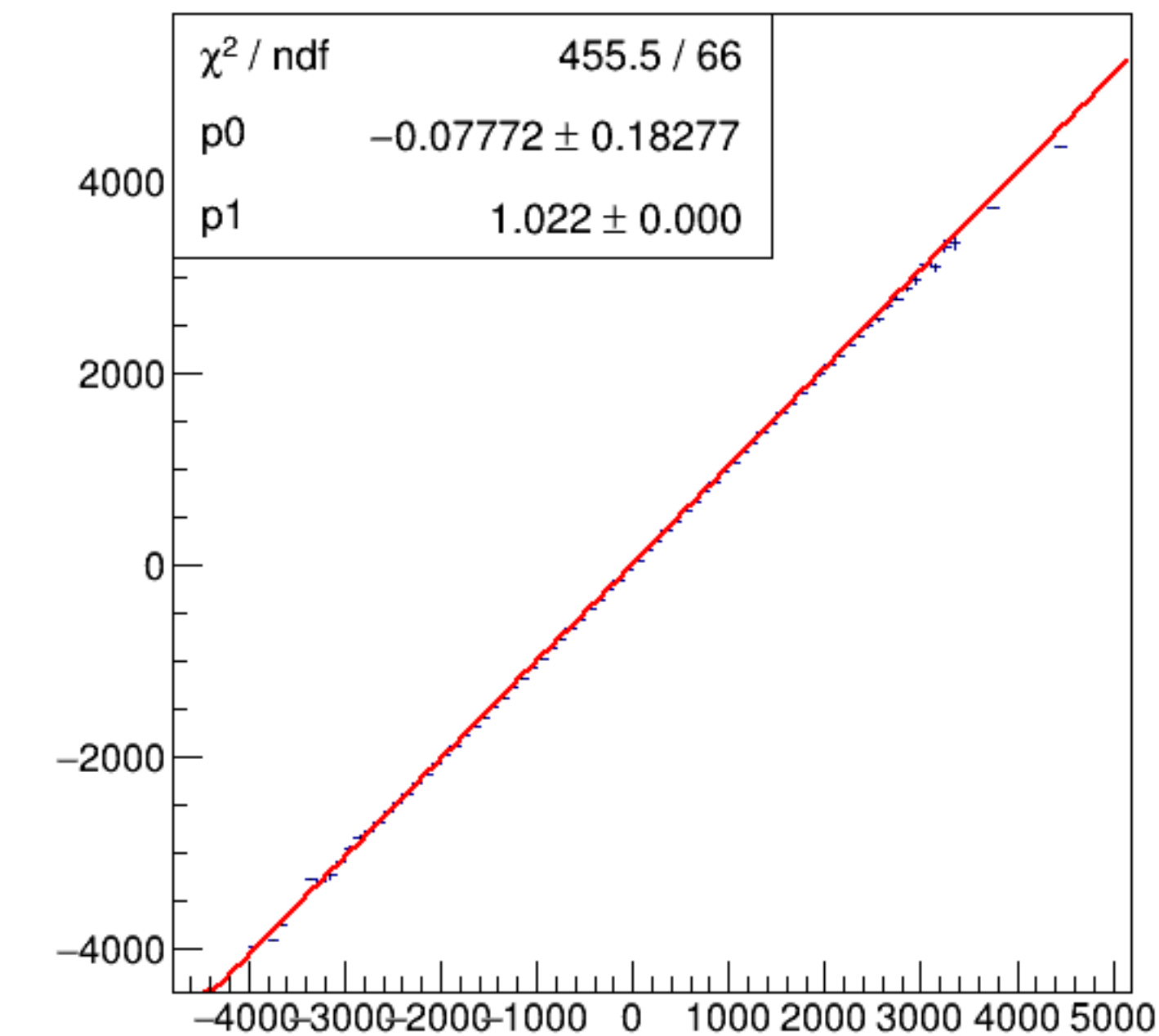
run6997_000_asym_bcm_dg_us_vs_asym_bcm_an_ds3_pr.png
