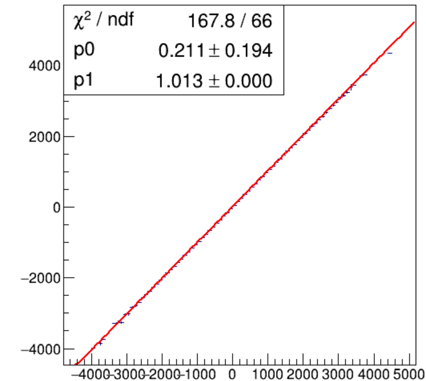
run6997_000_asym_bcm_dg_us_vs_asym_bcm_dg_ds_pr.png
