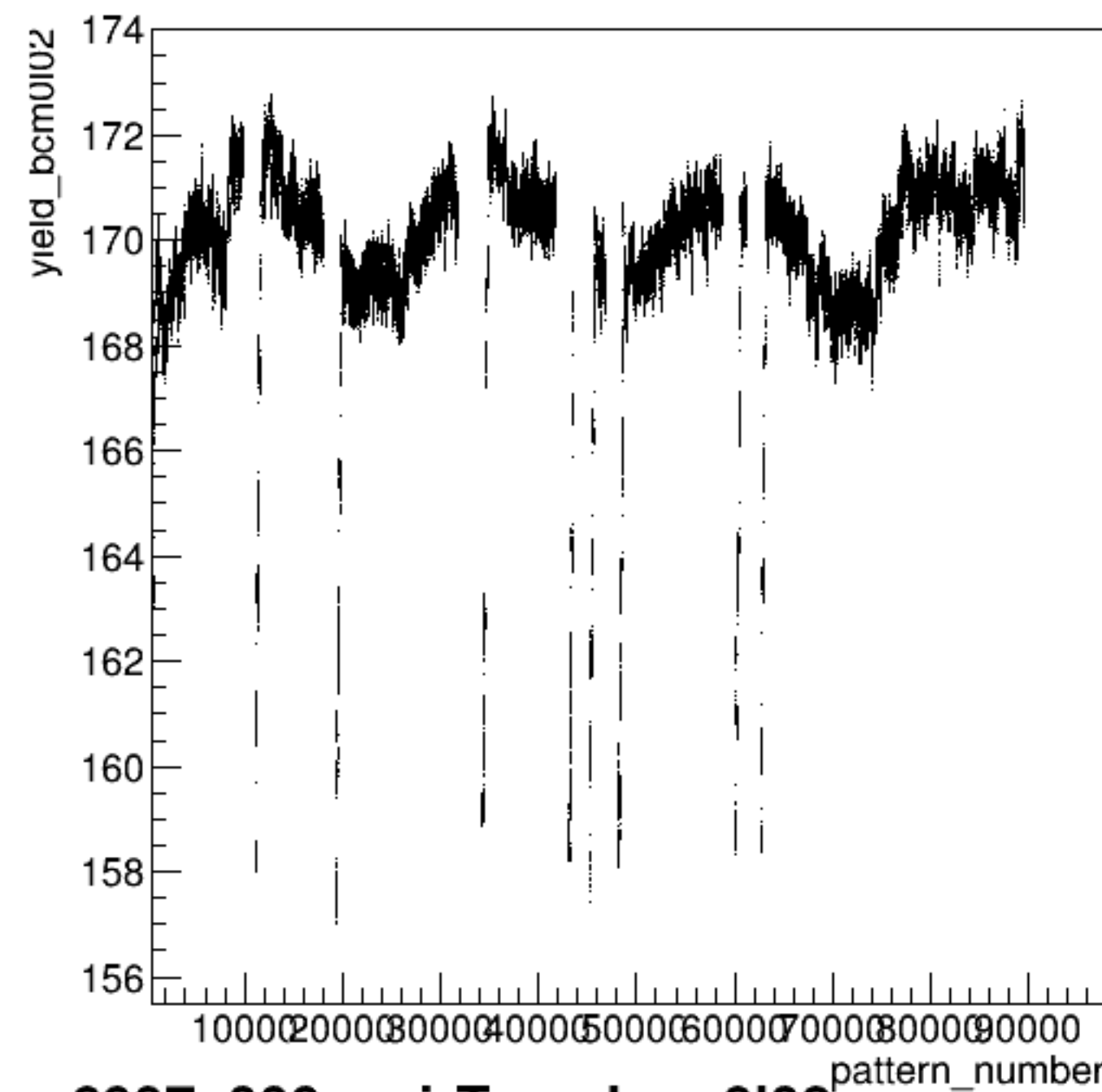
yield_bcm0l02:pattern_number {ErrorFlag==0}
