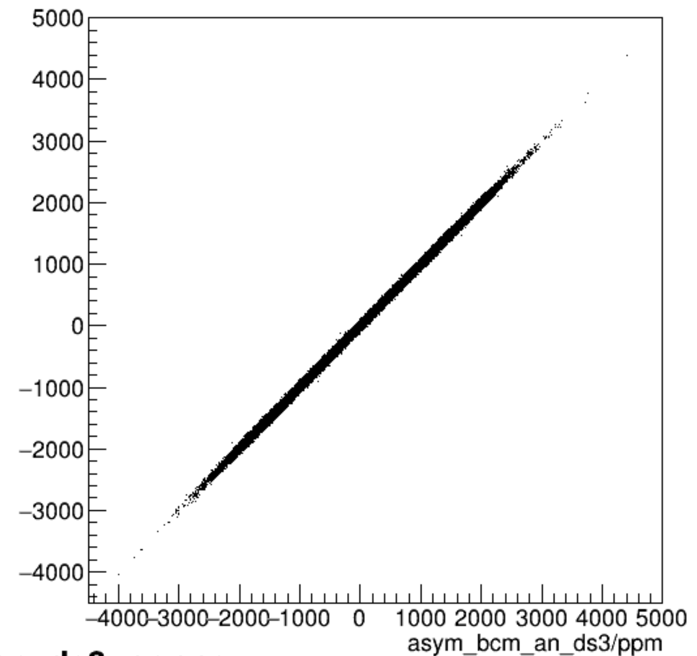
run6997_000_asym_bcm_an_us_vs_asym_bcm_an_ds3_pr.png
