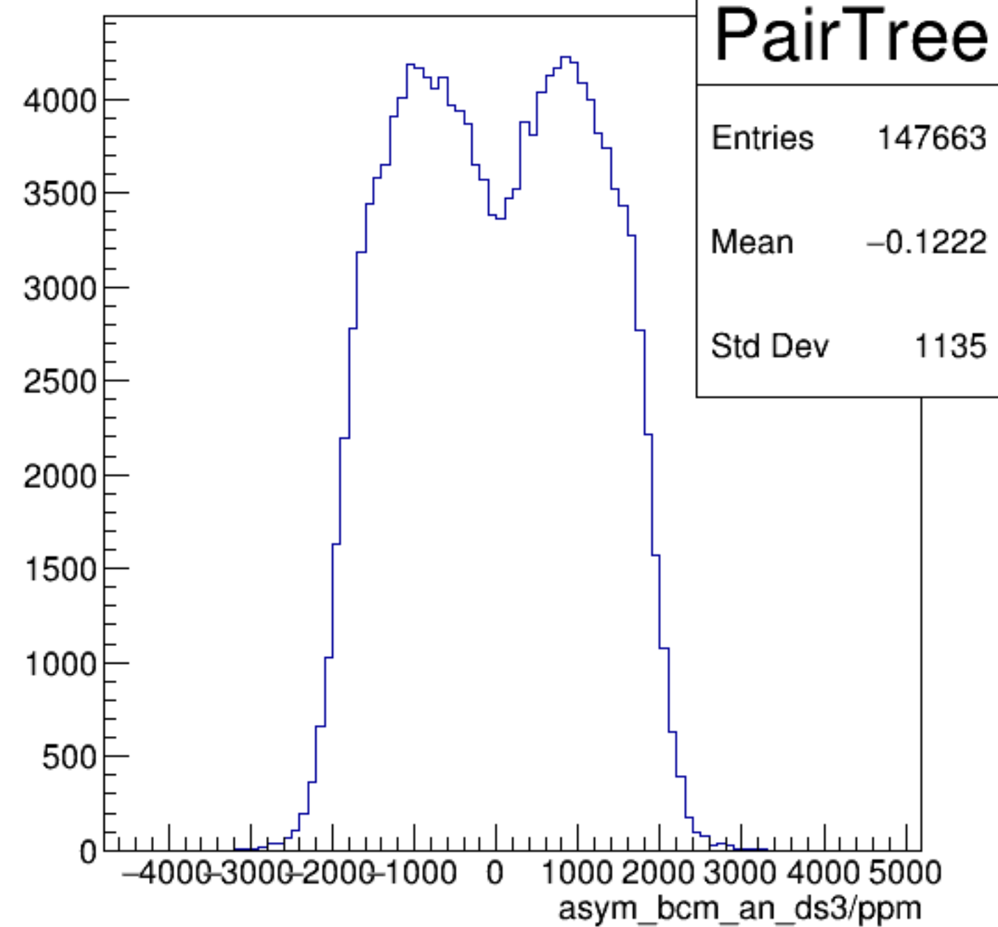
asym_bcm_an_ds3/ppm {ErrorFlag==0}
