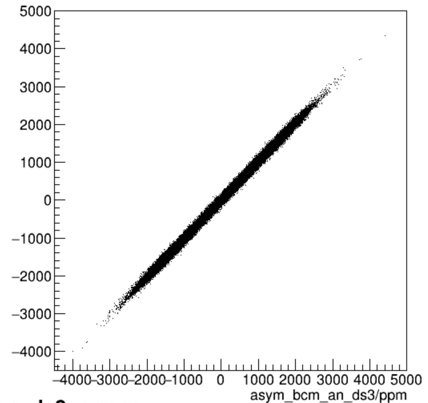
run6997_000_asym_bcm_dg_us_vs_asym_bcm_an_ds3_pr.png
