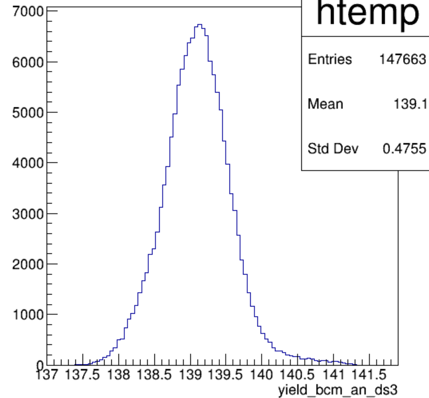
yield_bcm_an_ds3 {ErrorFlag==0}
