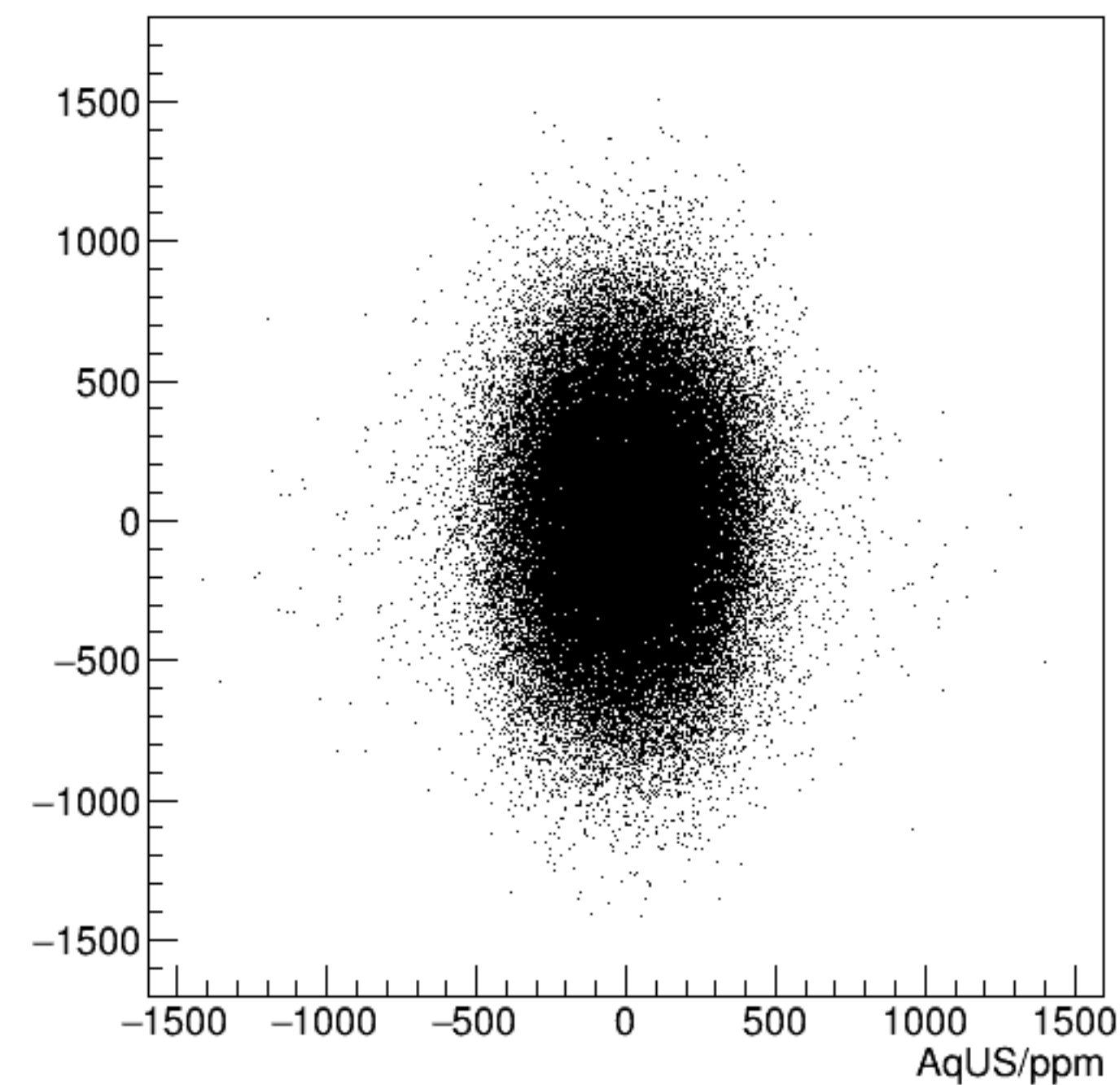
reg_asym_dsl/ppm:AqUS/ppm {ok_cut}
