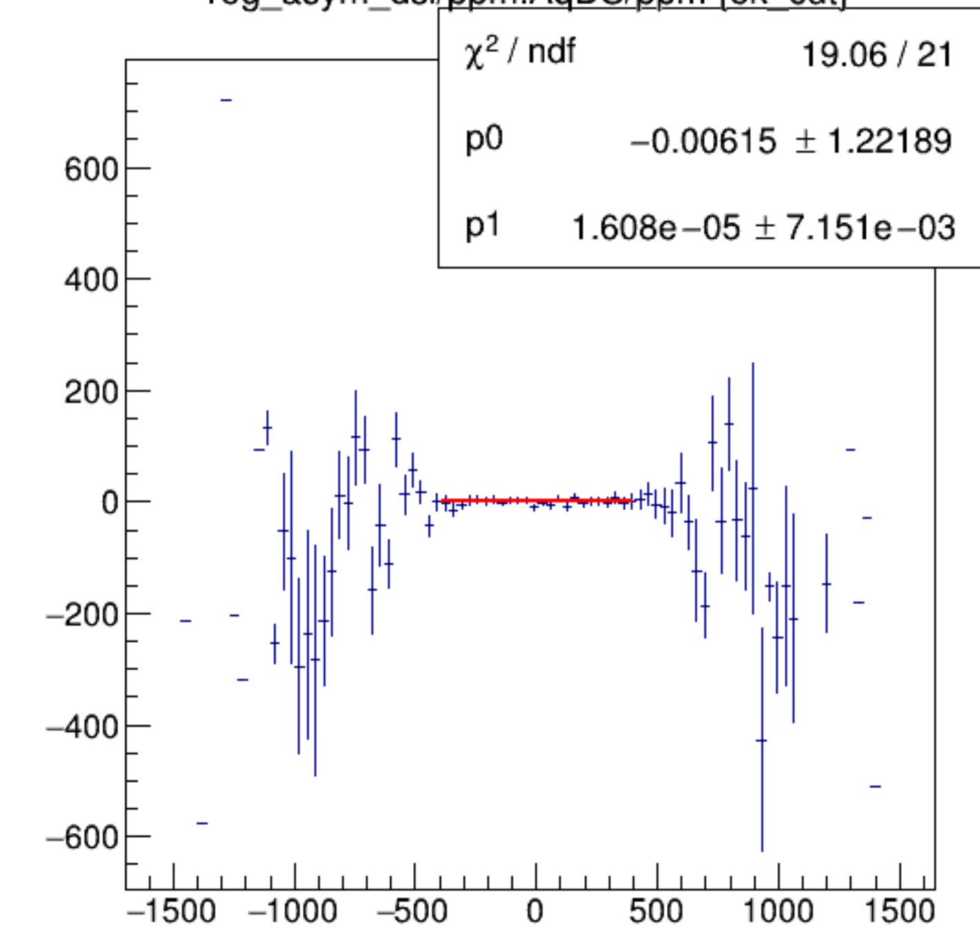
reg_asym_dsl/ppm:AqDS/ppm {ok_cut}
