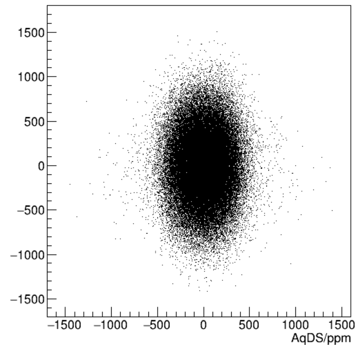
reg_asym_dsl/ppm:AqDS/ppm {ok_cut}
