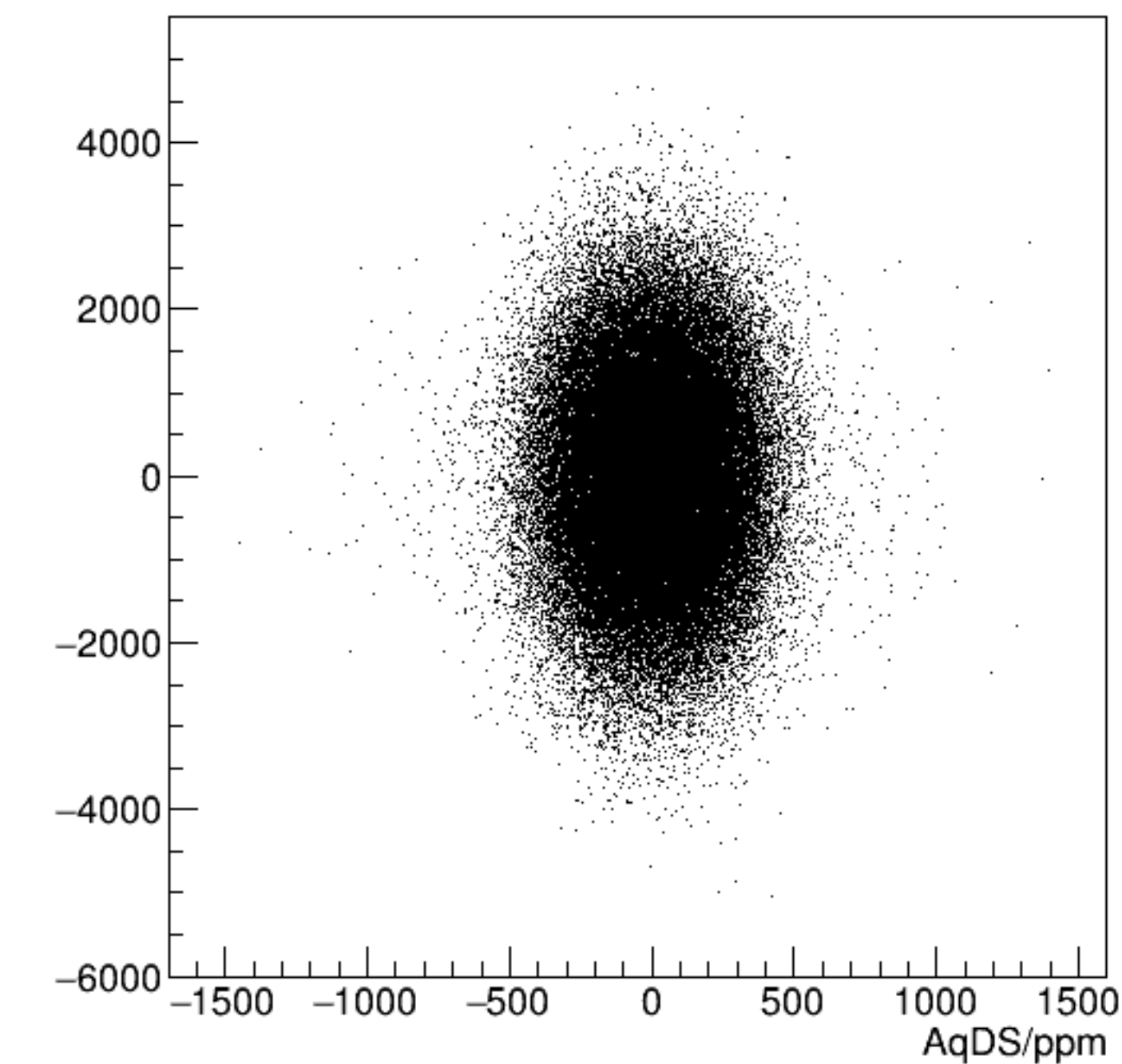
reg_asym_usl/ppm:AqDS/ppm {ok_cut}
