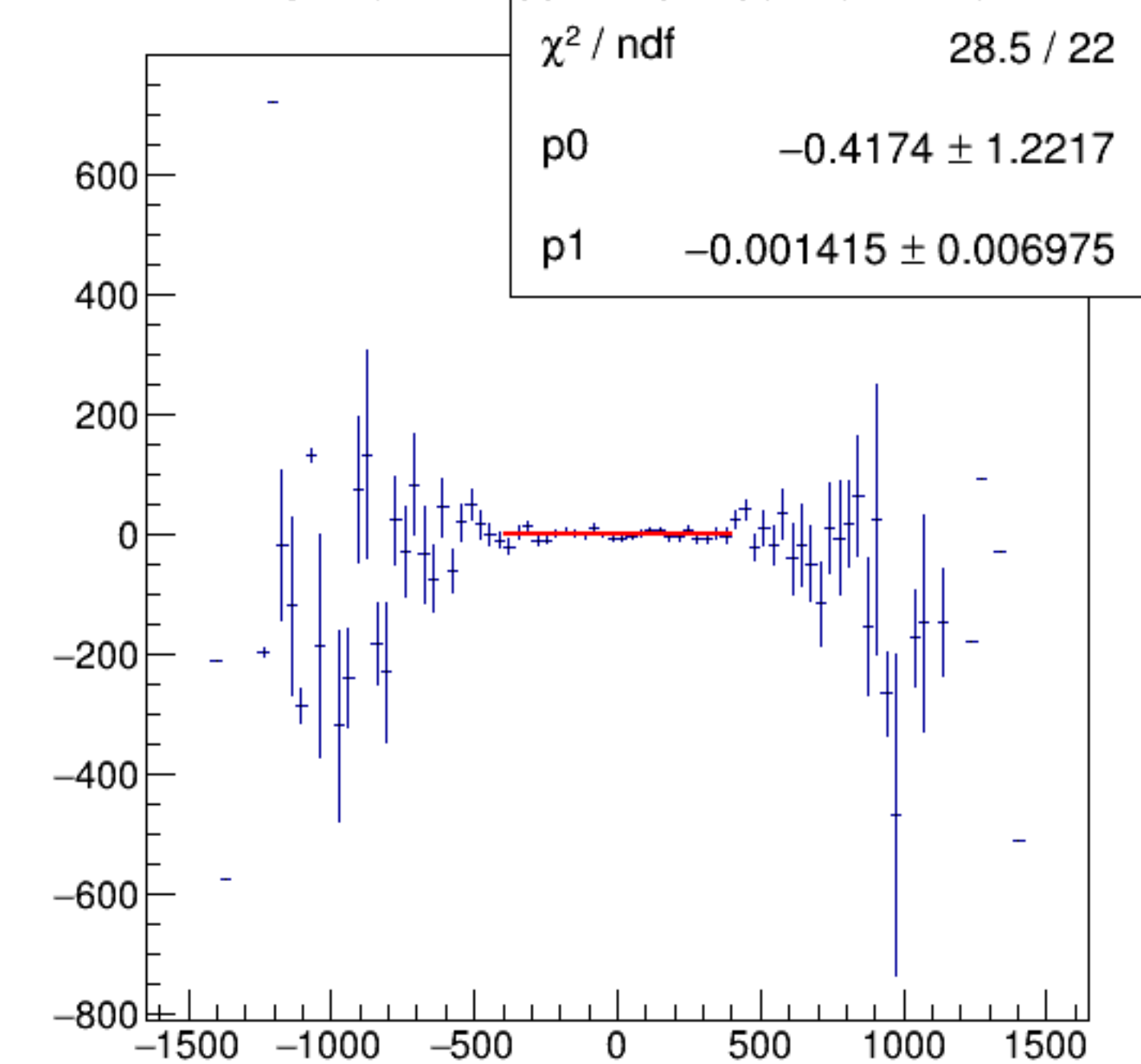
reg_asym_dsl/ppm:AqUS/ppm {ok_cut}
