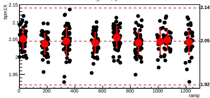
bmod_trim4,cyc=7662
