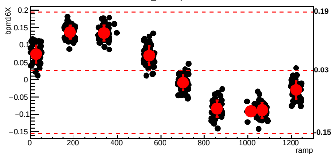
bmod_trim1,cyc=7662
