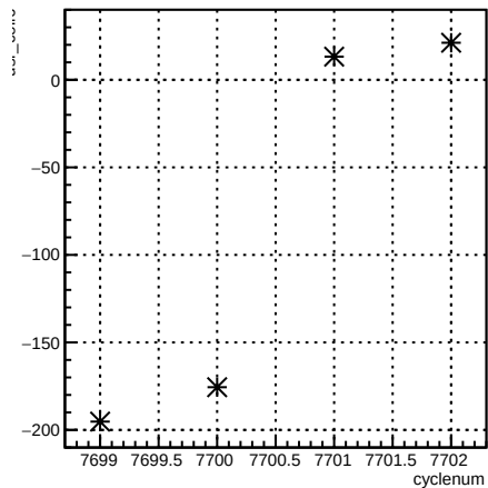
usr_coil6:cyclenum {run == 7014}
