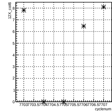
12X_coil6:cyclenum {run == 7015}
