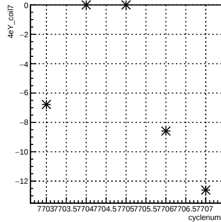
4eY_coil7:cyclenum {run == 7015}
