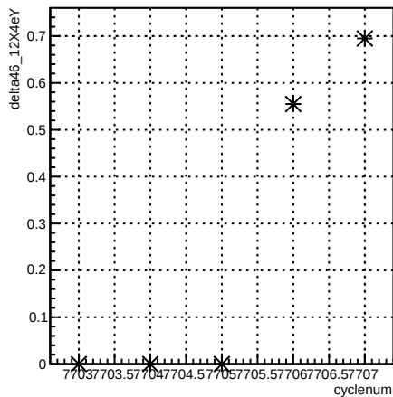
delta46_12X4eY:cyclenum {run == 7015}
