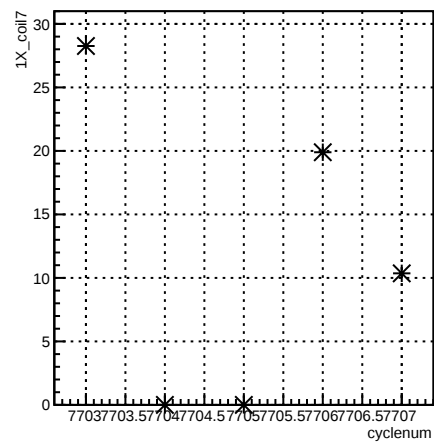
1X_coil7:cyclenum {run == 7015}
