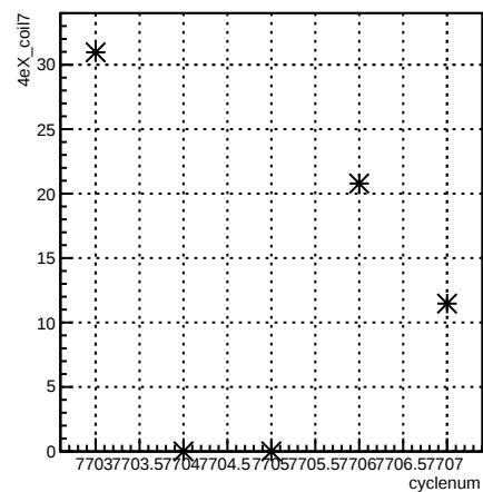
4eX_coil7:cyclenum {run == 7015}
