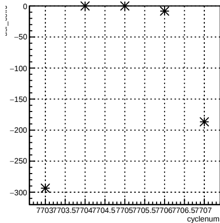
usr_coil6:cyclenum {run == 7015}
