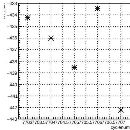
1X_coil1:cyclenum {run == 7015}
