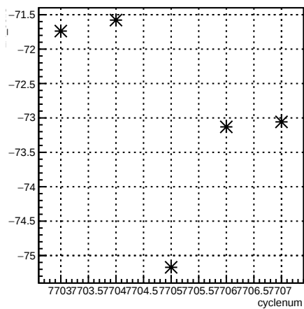
1X_coil3:cyclenum {run == 7015}
