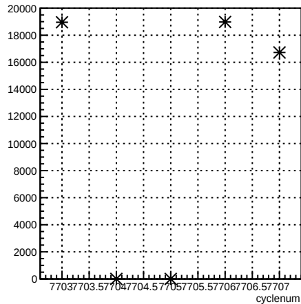
usr_coil7:cyclenum {run == 7015}
