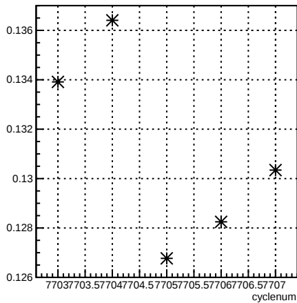
delta46_12X4eY:cyclenum {run == 7015}
