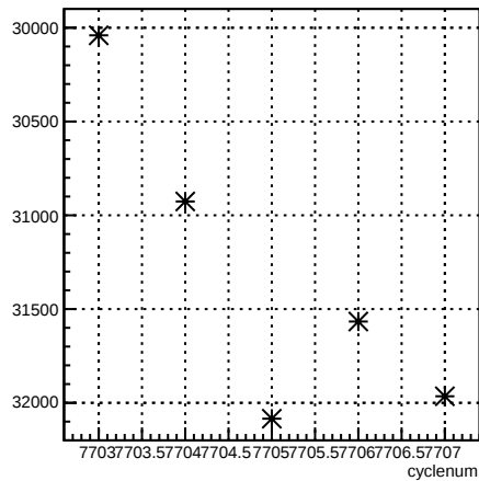
usr_coil6:cyclenum {run == 7015}
