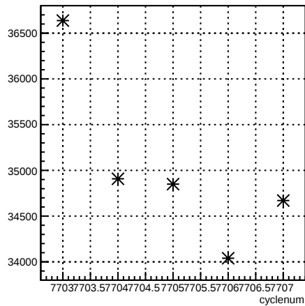
usl_coil6:cyclenum {run == 7015}
