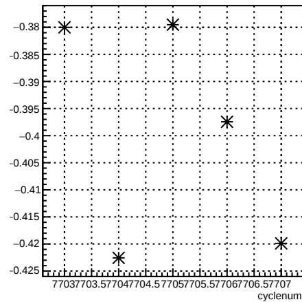
segment:cyclenum {run == 7015}
