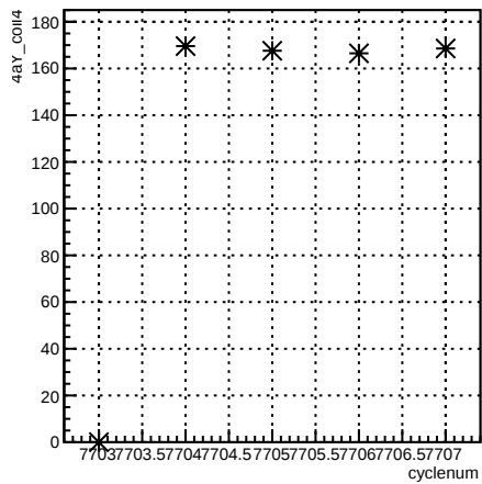
4eY_coil4:cyclenum {run == 7015}
