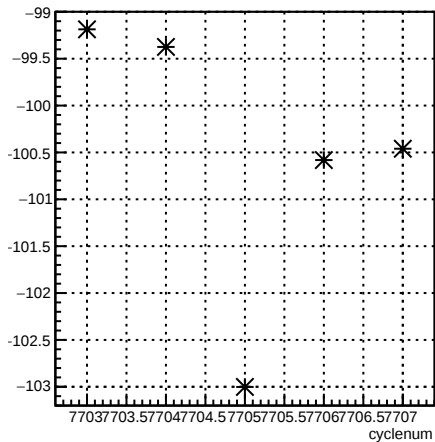
4eX_coil3:cyclenum {run == 7015}
