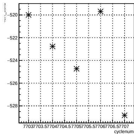
4eX_coil1:cyclenum {run == 7015}
